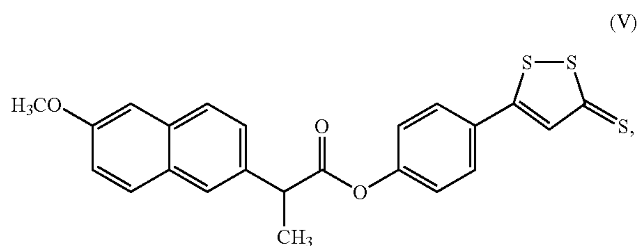
2-(6-Methoxy-naphthalen-2-yl)-propionic acid 4-(5-thioxo-5H-[1,2]dithiol-3-yl)-phenyl ester
