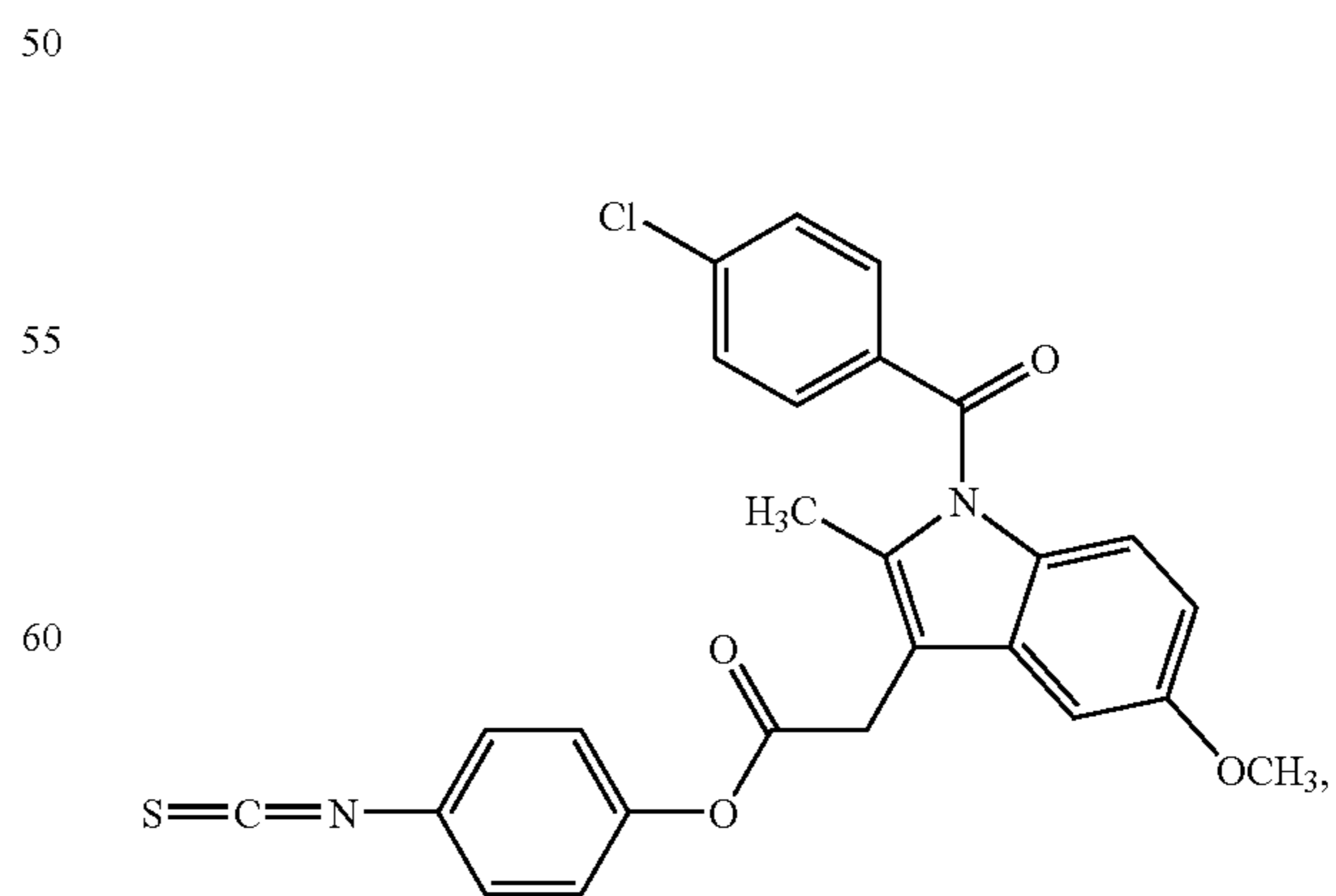
4-(isothiocyano)-phenyl -2-[1-(4-chlorobenzoyl)-5-methoxy-2-methyl-indol-3-yl]-acetate (XXXIV)
