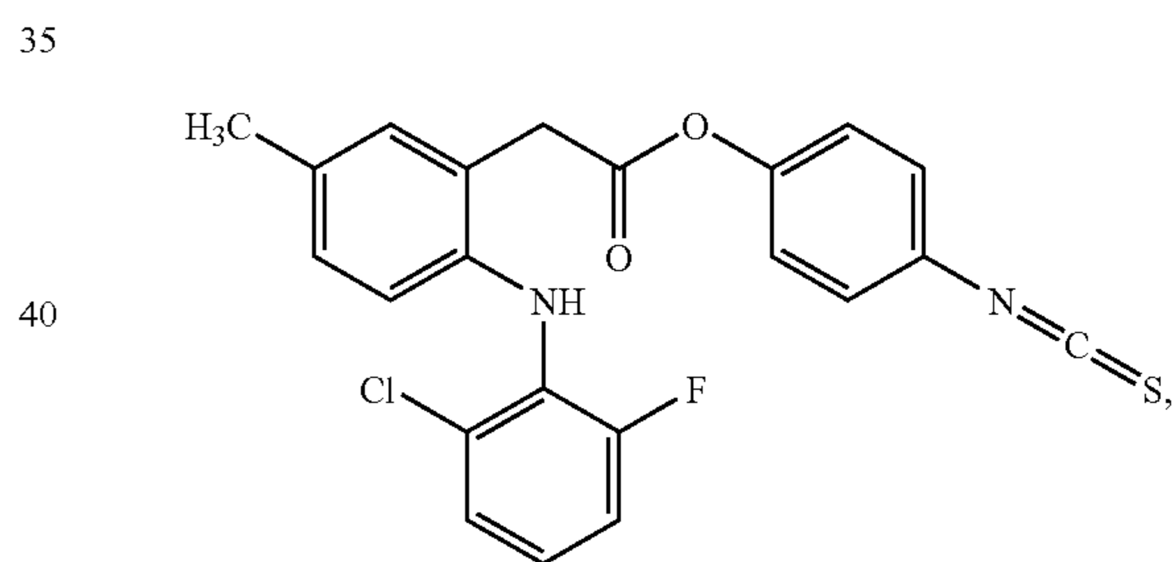
4-isothiocyanatophenyl 2-(2-(2-chloro-6-fluorophenylamino)-5-methylphenyl)acetate (XXIII)
