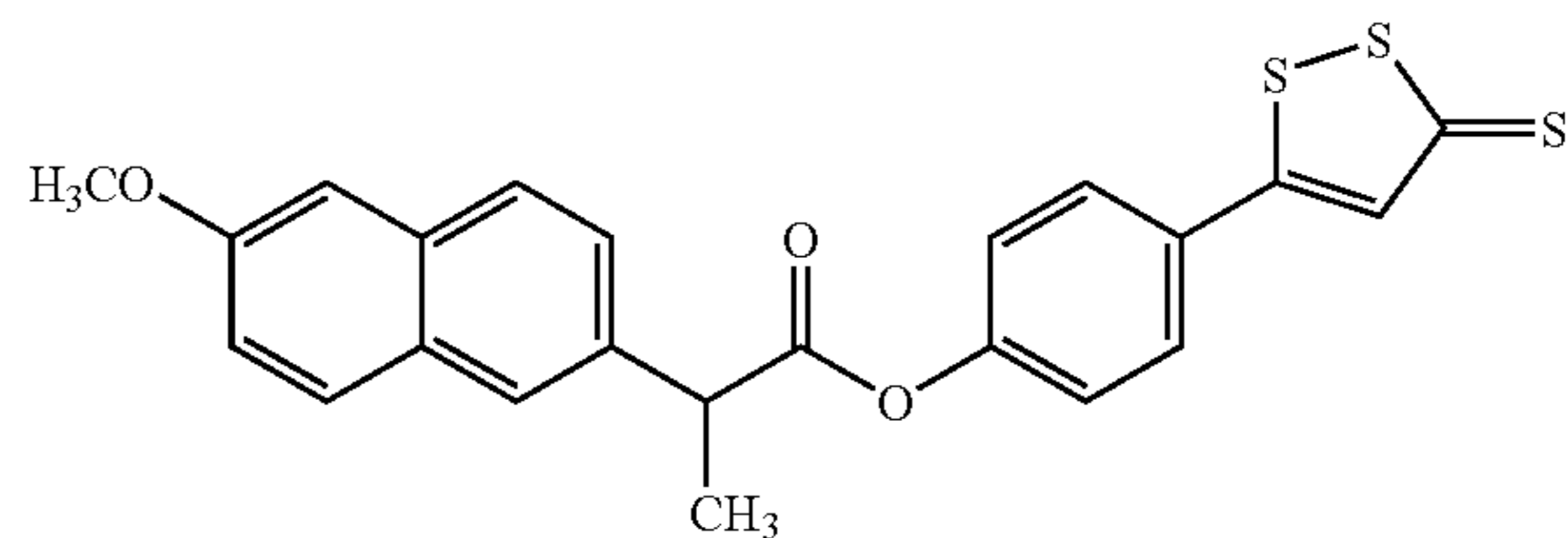
2-(6-Methoxy-naphthalen-2-yl)-propionic acid 4-(5-thio-5H-[1,2]dithiol-3-yl)-phenyl ester (V)
