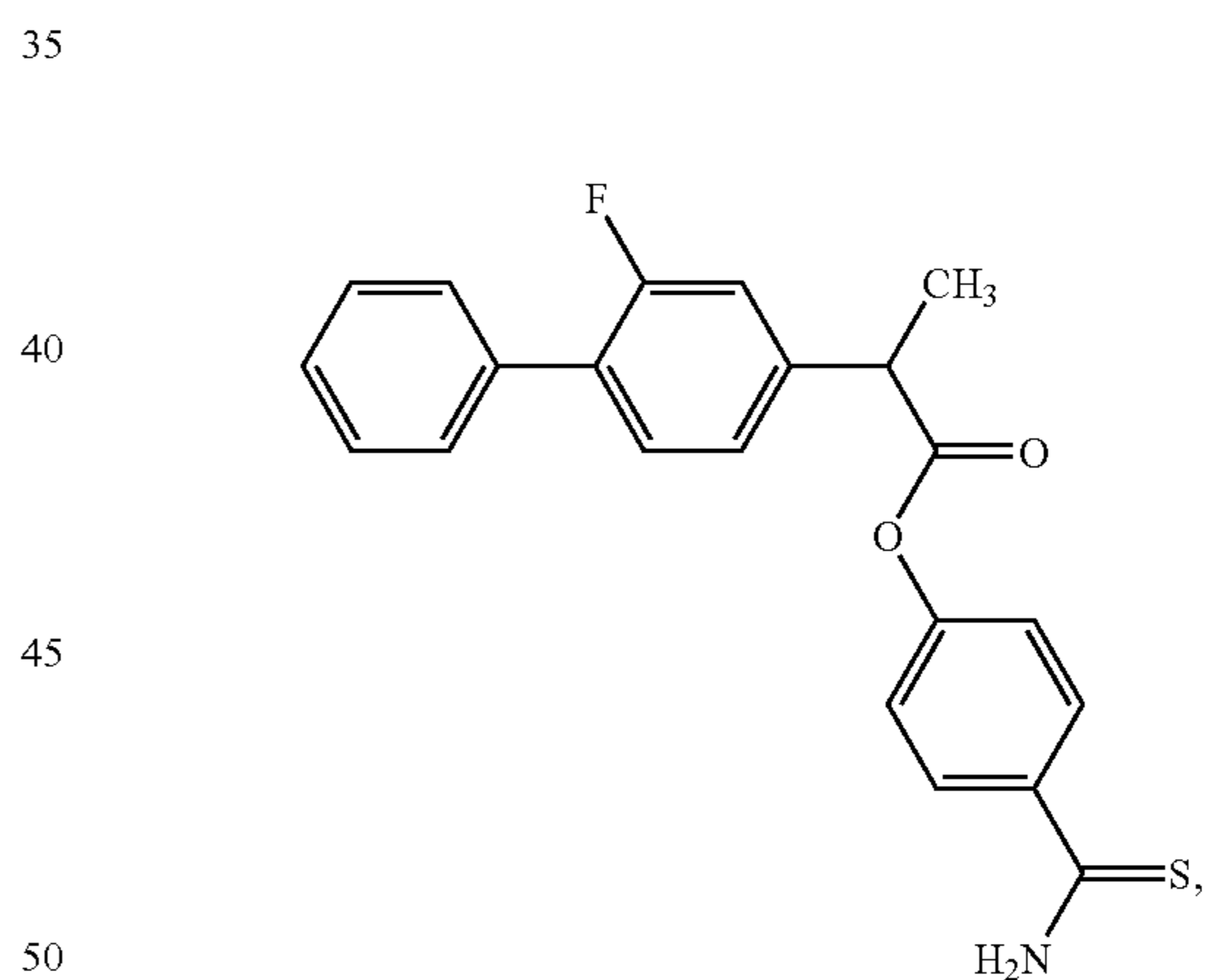
4-thiocarbamoylphenyl 2-(2-Fluoro-4-biphenyl)propanoate (XXXI)
