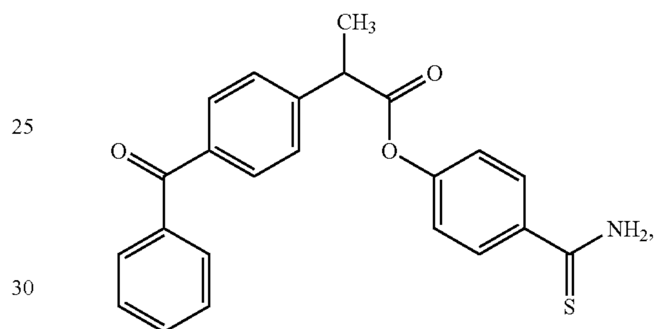
4-thiocarbamoylphenyl 2-(4-oxophenyl)phenyl propanoate (XXX)
