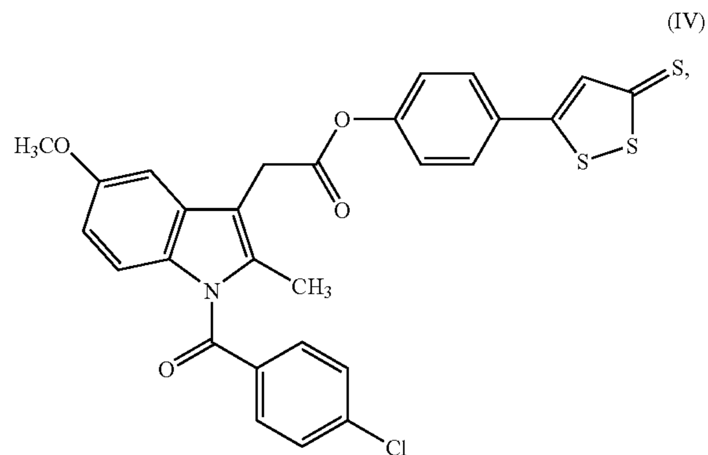
[1-(4-Chloro-benzoyl)-5-methoxy-2-methyl-1H-indol-3-yl]-acetic acid 4-(5-thioxo-5H-[1,2]dithiol-3-yl)-phenyl ester
