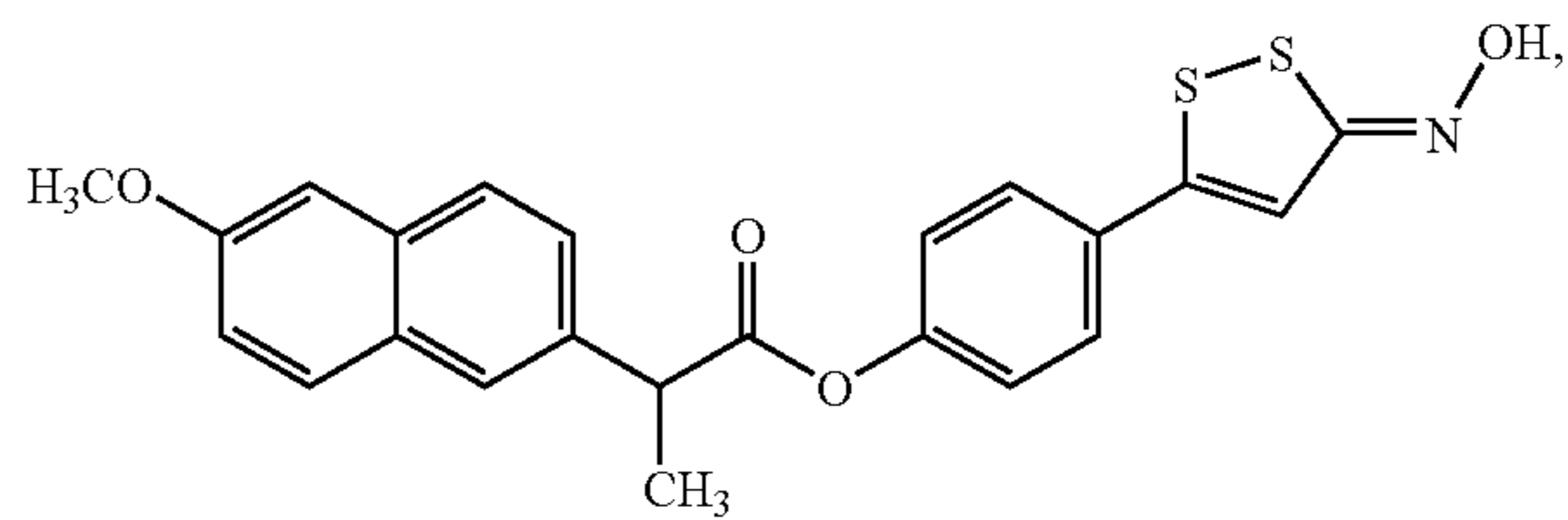
2-(6-Methoxy-naphthalen-2-yl)-propionic acid 4-(5-hydroxyimino-5H-[1,2]dithiol-3-yl)-phenyl ester (XV)
