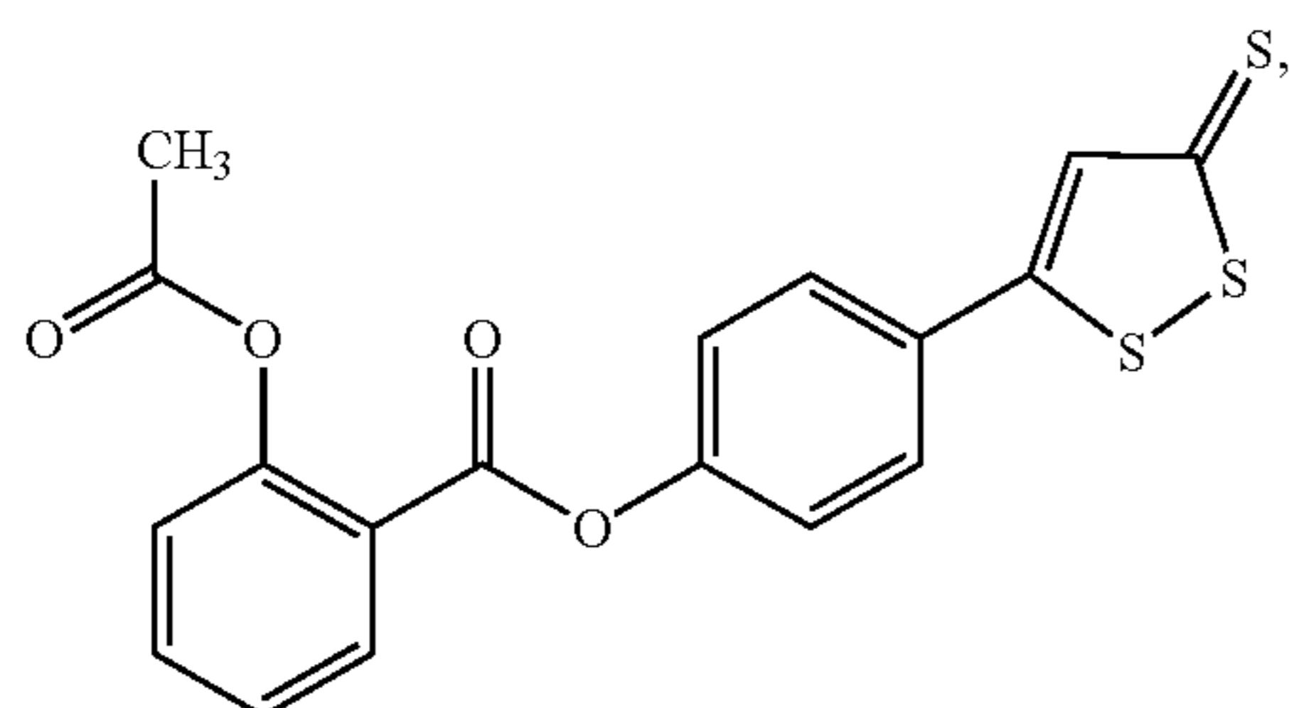
4-(5-thio-5H-1,2-dithiol-3-yl)-phenyl 2-acetoxybenzoate (I)
