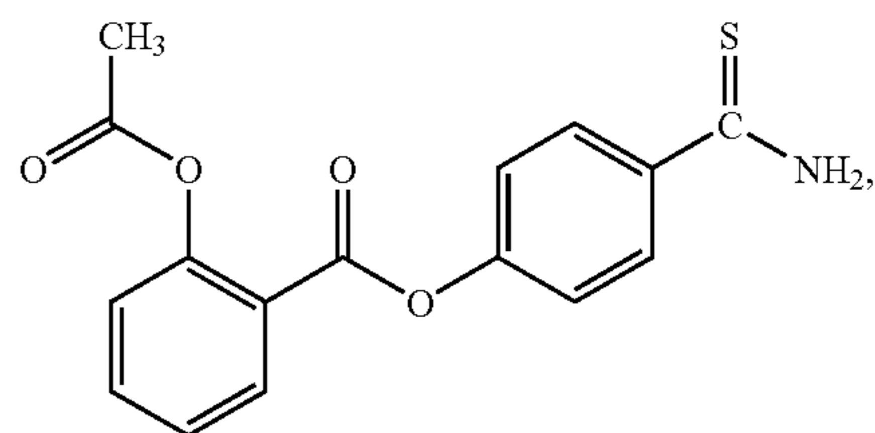
2-Acetoxy-benzoic acid 4-thiocarbamoyl-phenyl ester (XVI)
