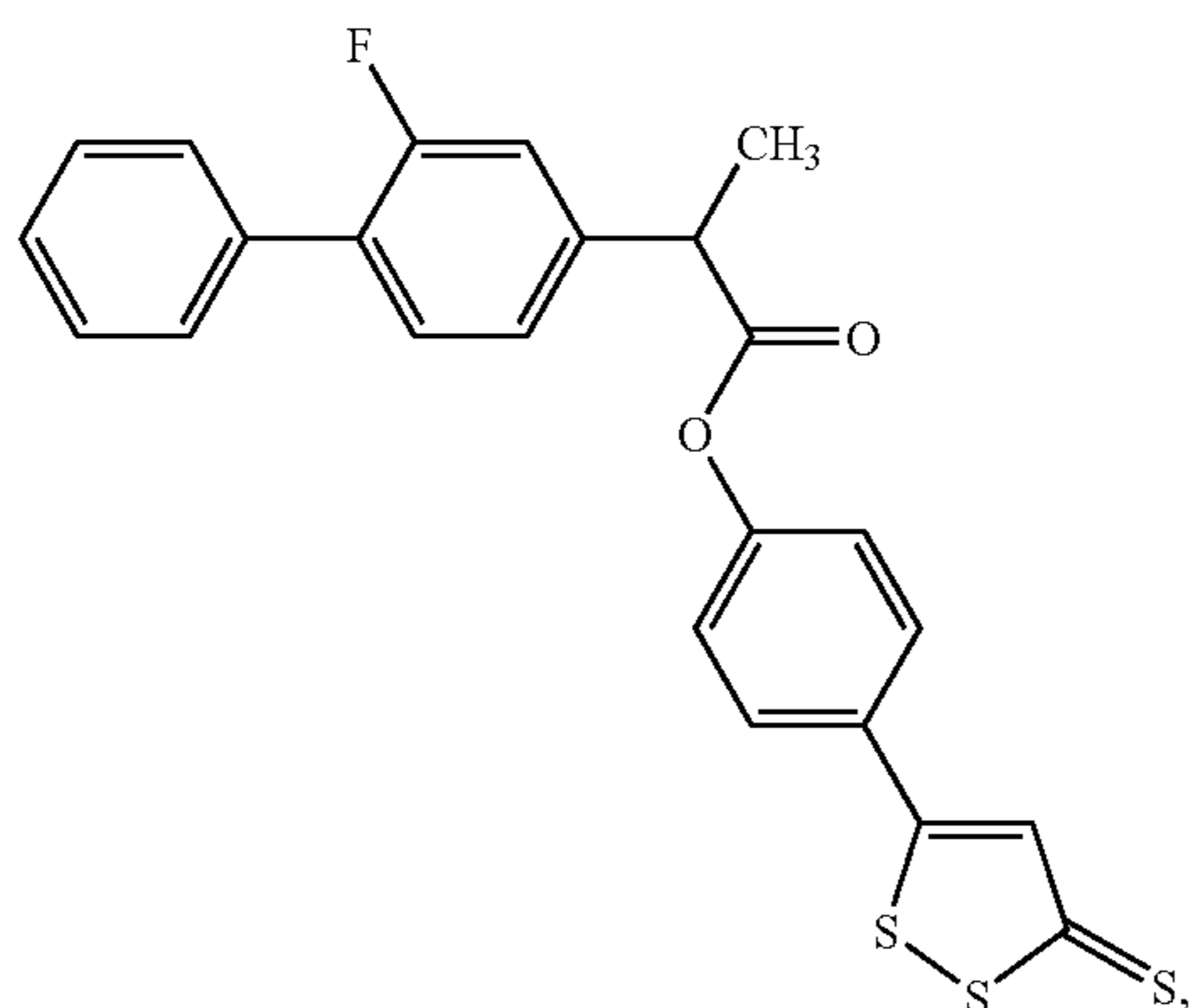
4-(5-thioxo-5H-1,2-dithiol-3-yl)phenyl 2-(2-Fluoro-4-biphenyl)propanoate (XXVIII)
