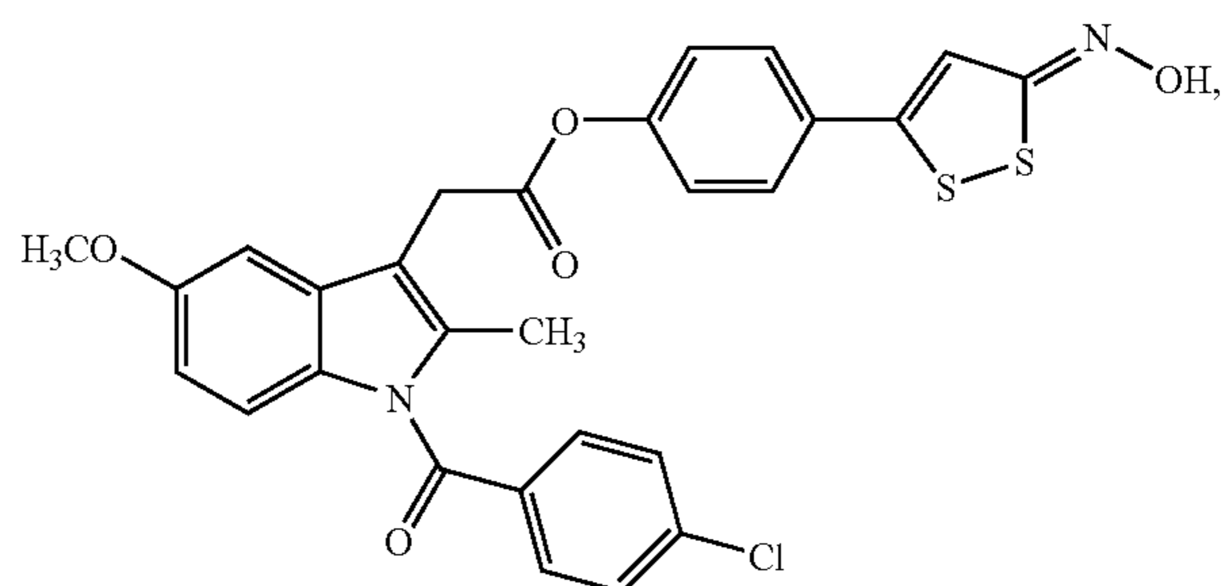
[1-(4-Chloro-benzoyl)-5-methoxy-2-methyl-1H-indol-3-yl]-acetic acid 4-(5-hydroxyimino-5H-[1,2]dithiol-3-yl)-phenyl ester (XIV)
