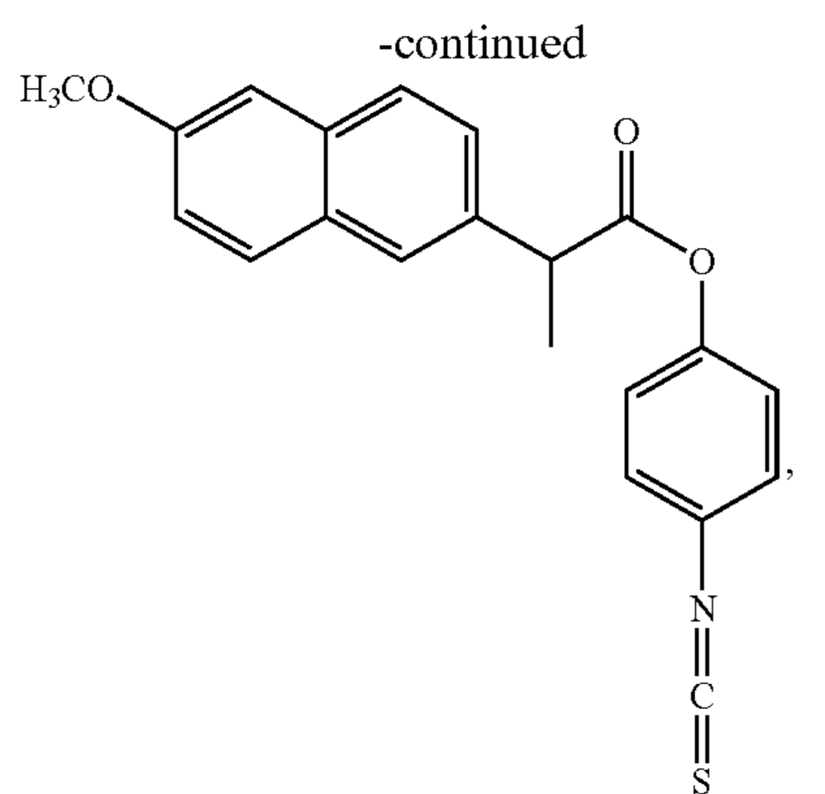
4-isothiocyanatophenyl 2-(2-methoxynaphthalen-6-yl)propanoate (XXV)
