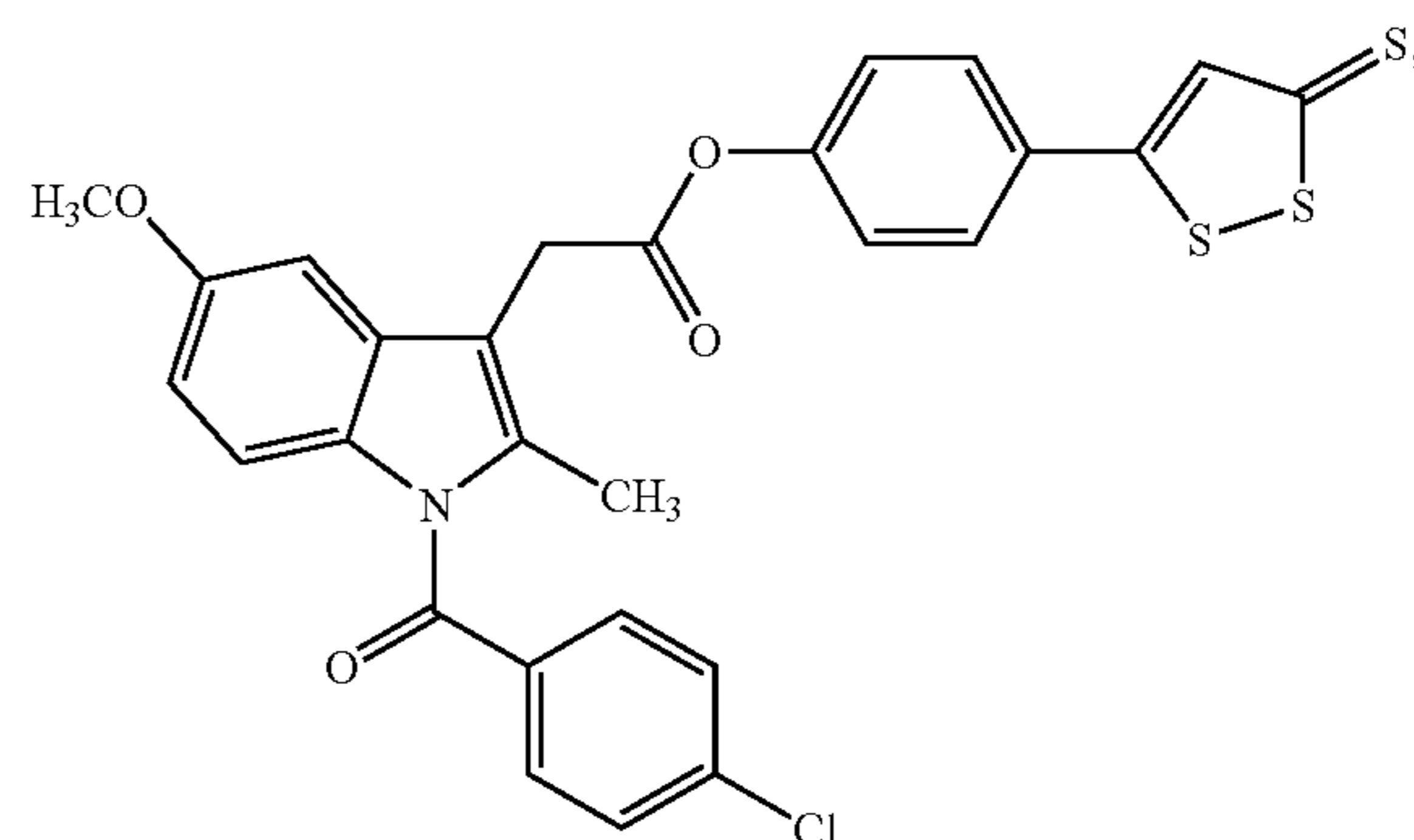
[1-(4-Chloro-benzoyl)-5-methoxy-2-methyl-1H-indol-3-yl]-acetic acid 4-(5-thio-5H-[1,2]dithiol-3-yl)-phenyl ester (IV)
