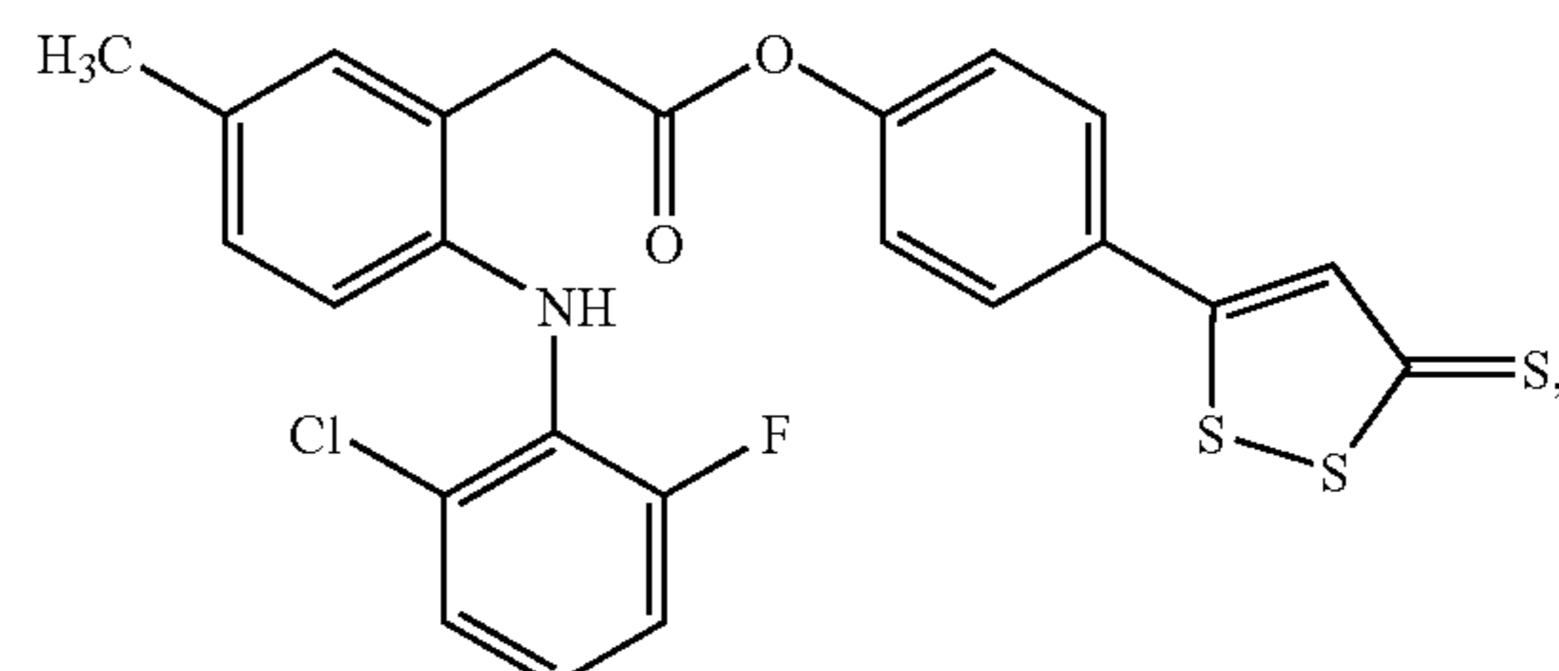
4-(5-thio-5H-1,2-dithiol-3-yl)phenyl 2-(2-(2-chloro-6-fluorophenylamino)-5-methylphenyl)acetate (III)
