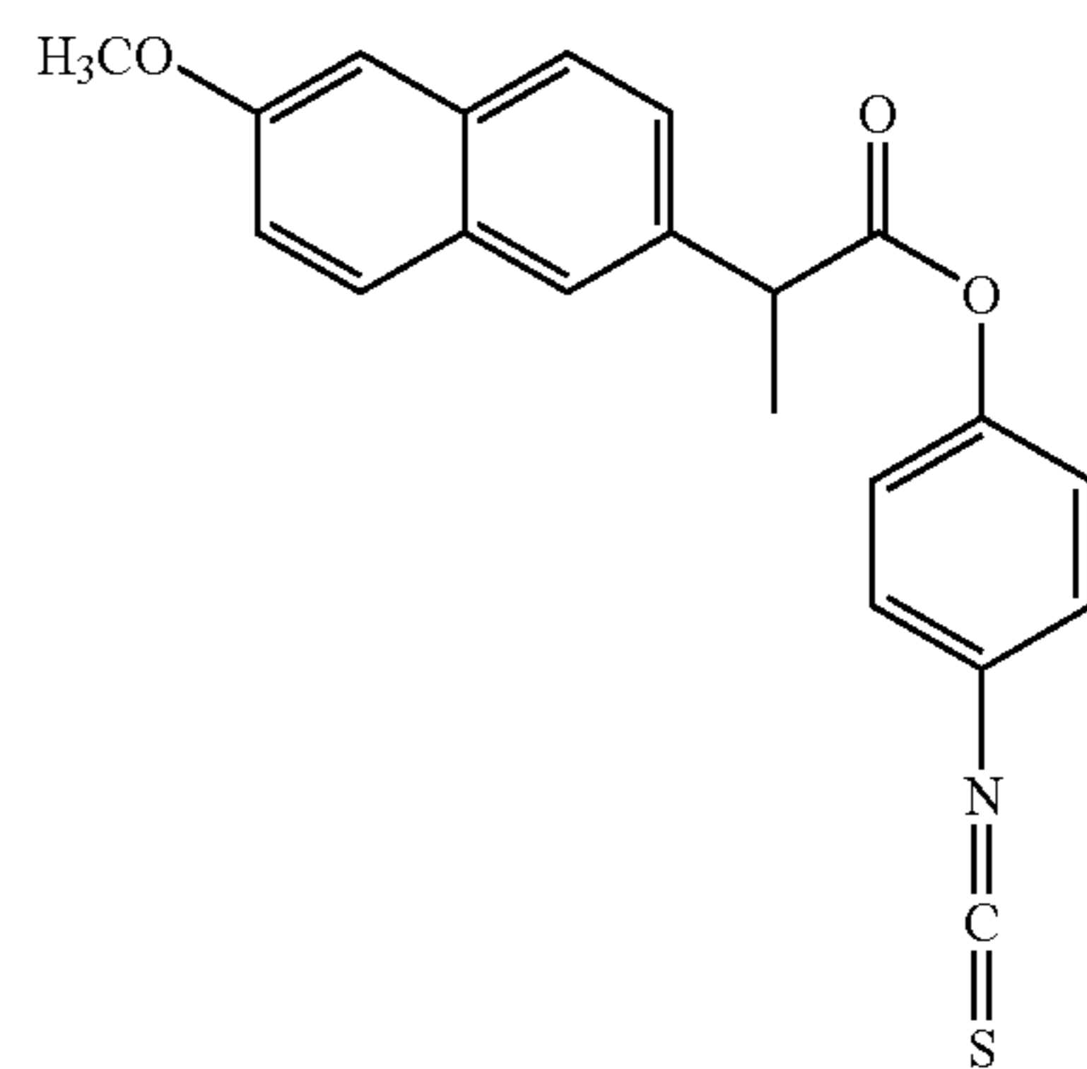
4-isothiocyanatophenyl 2-(2-methoxynaphthalen-6-yl) propanoate
