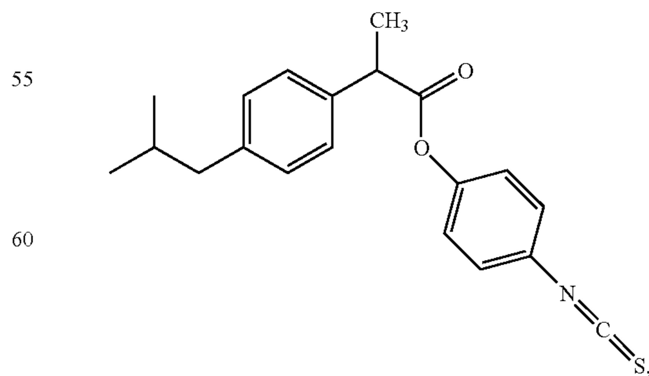
4-isothiocyanatophenyl 2-(4-isobutylphenyl)propanoate (XXXII)
