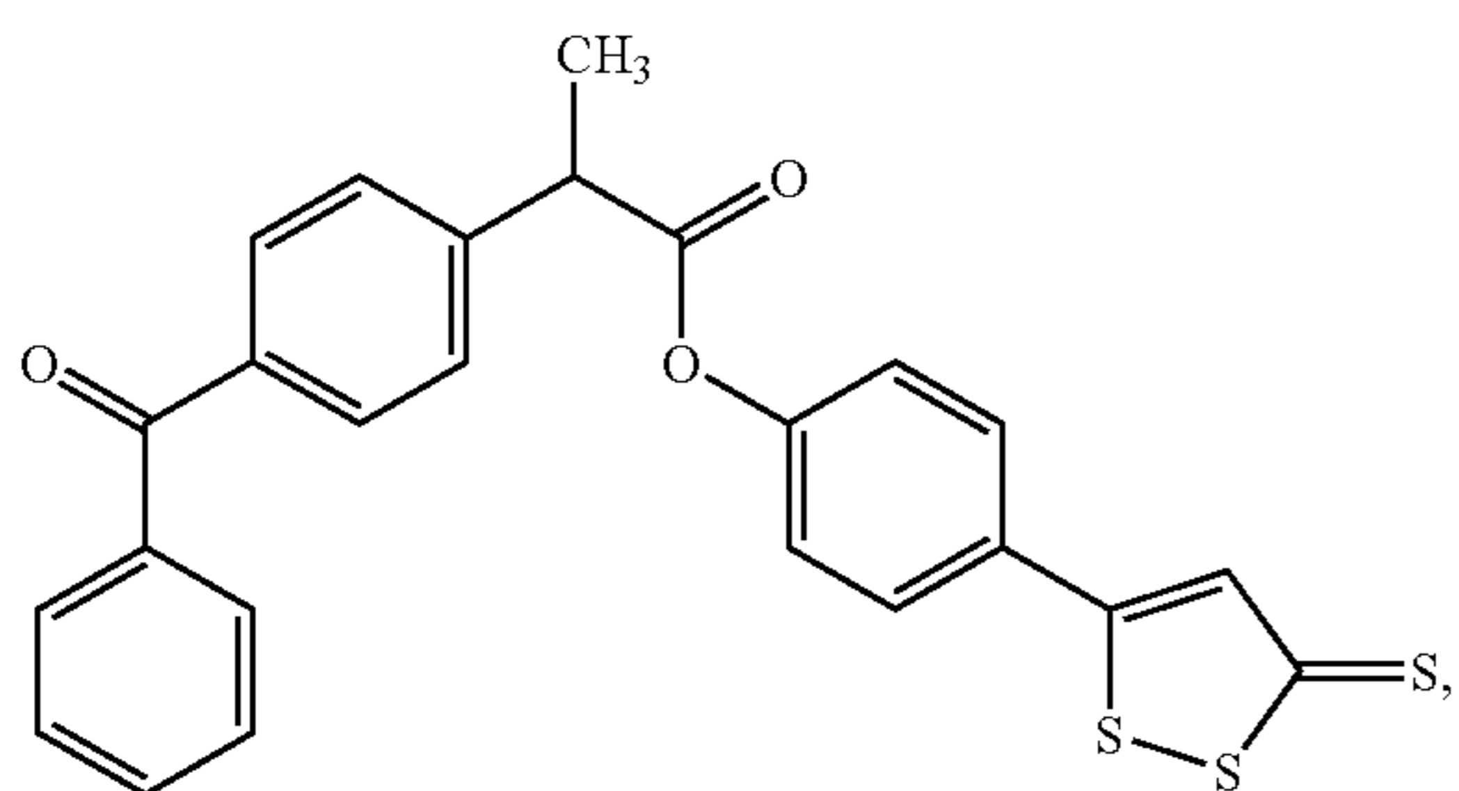
4-(5-thioxo-5H-1,2-dithiol-3-yl)phenyl 2-(3-benzoylphenyl)propanoate (XXVII)
