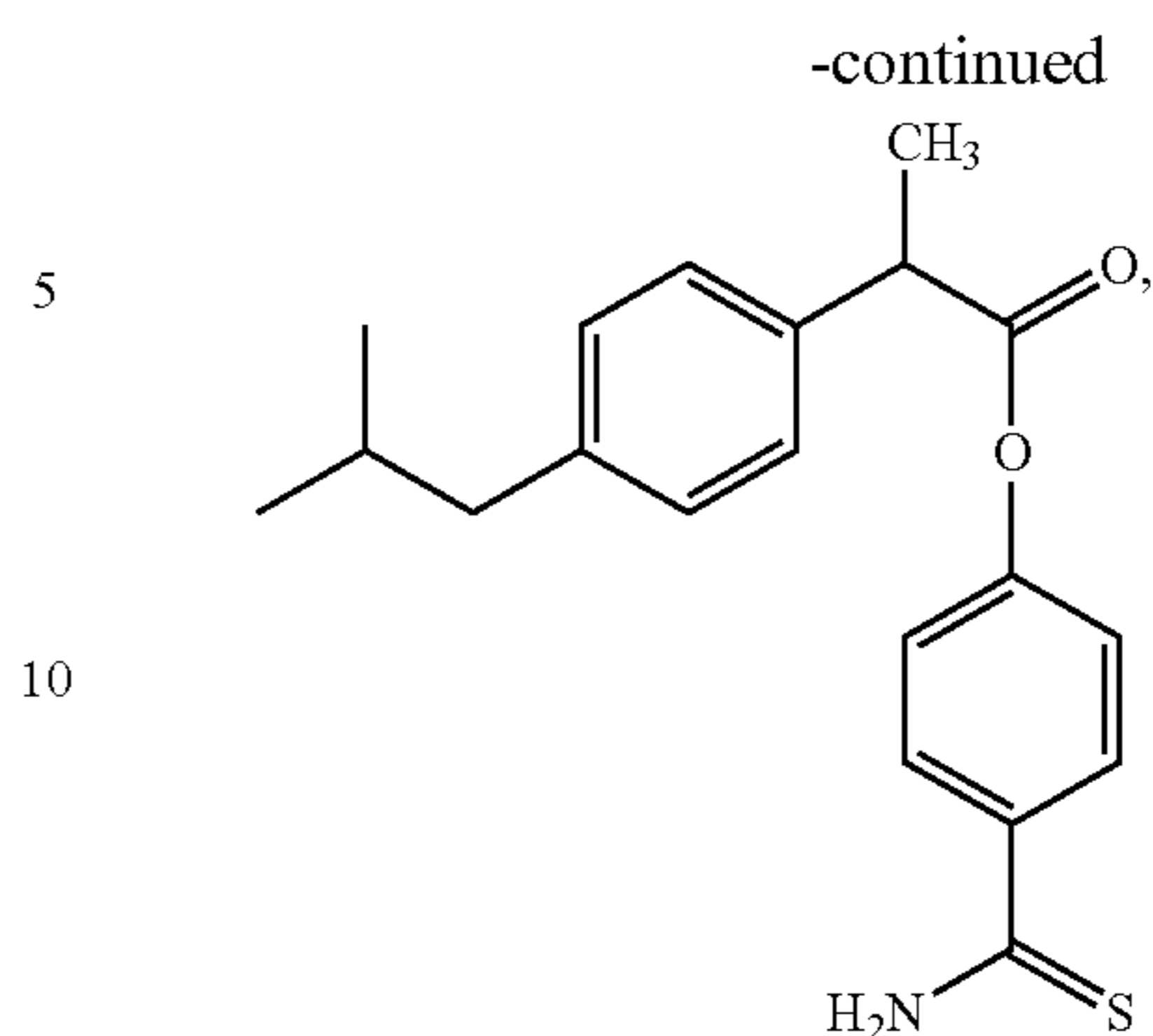
4-thiocarbamoylphenyl 2-(4-isobutylphenyl)propanoate (XXIX)
