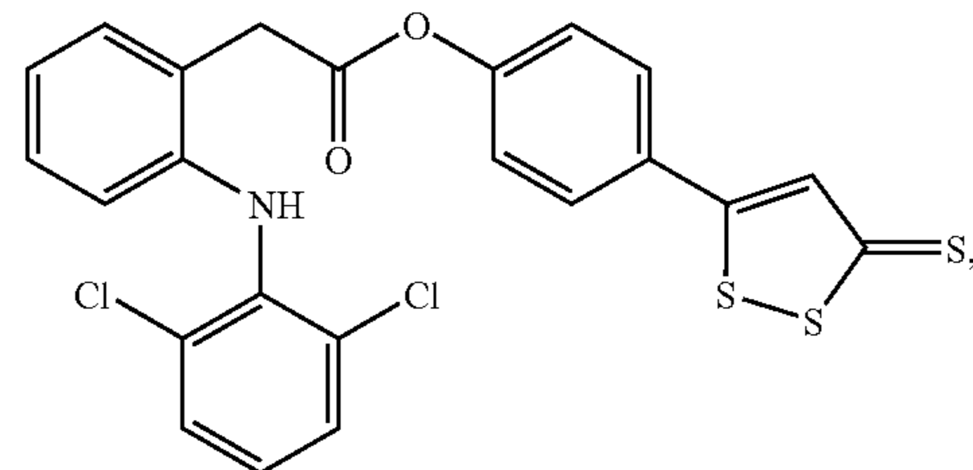
4-(5-thio-5H-1,2-dithiol-3-yl)phenyl 2-(2-(2,6-dichlorophenylamino)phenyl)acetate (II)
