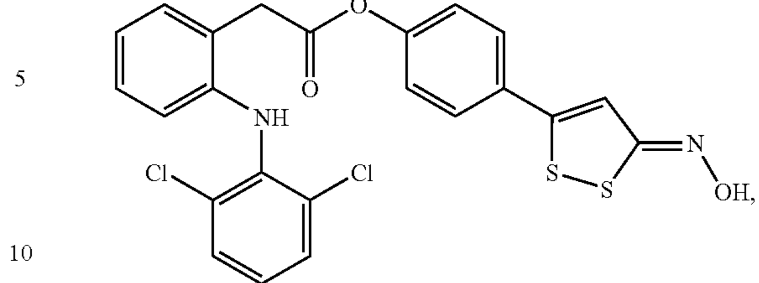
[2-(2,6-Dichloro-phenylamino)-phenyl]-acetic acid 4-(5-hydroxyimino-5H-[1,2]dithiol-3-yl)-phenyl ester (XII)
