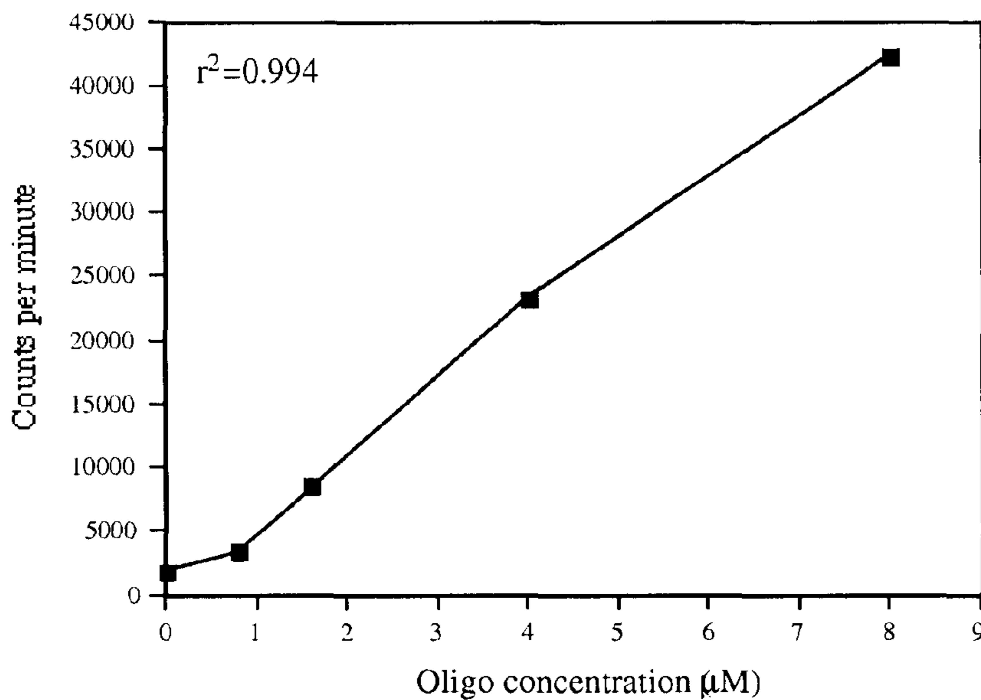
Chart 2. Increase in hybridisation signal of labelled probe is proportional to attached template concentration. (sample washes in 1xTth ligation buffer; 0.1%SDS at 22°C)
