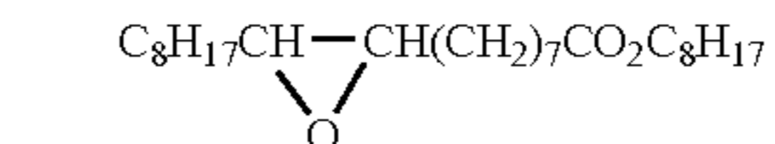
(Solv-2)
