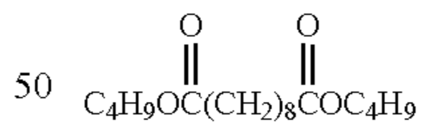
(Solv-4)
