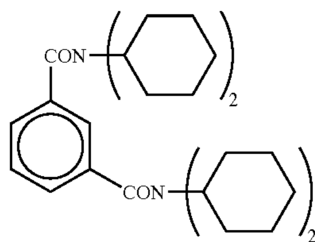
(Cpd-14)
