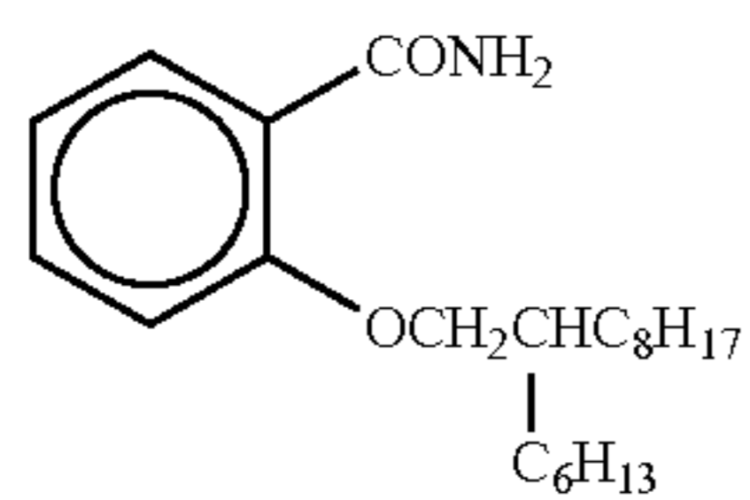
(Cpd-16)
