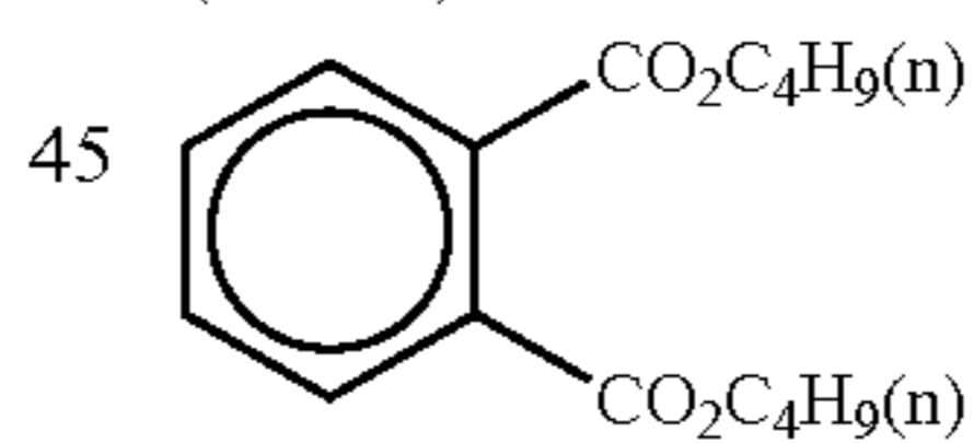
(Solv-3)
