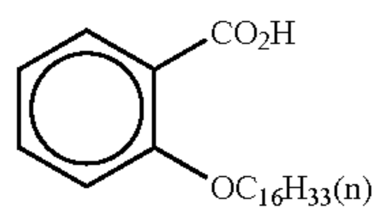
(Cpd-17)
