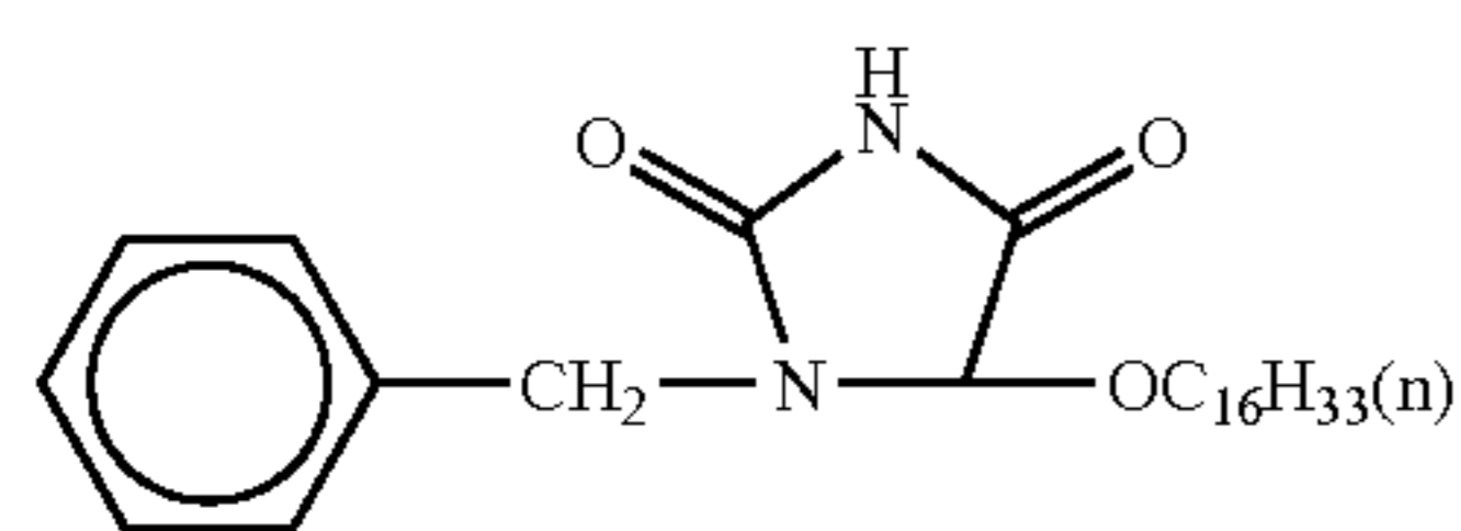
(Cpd-18)
