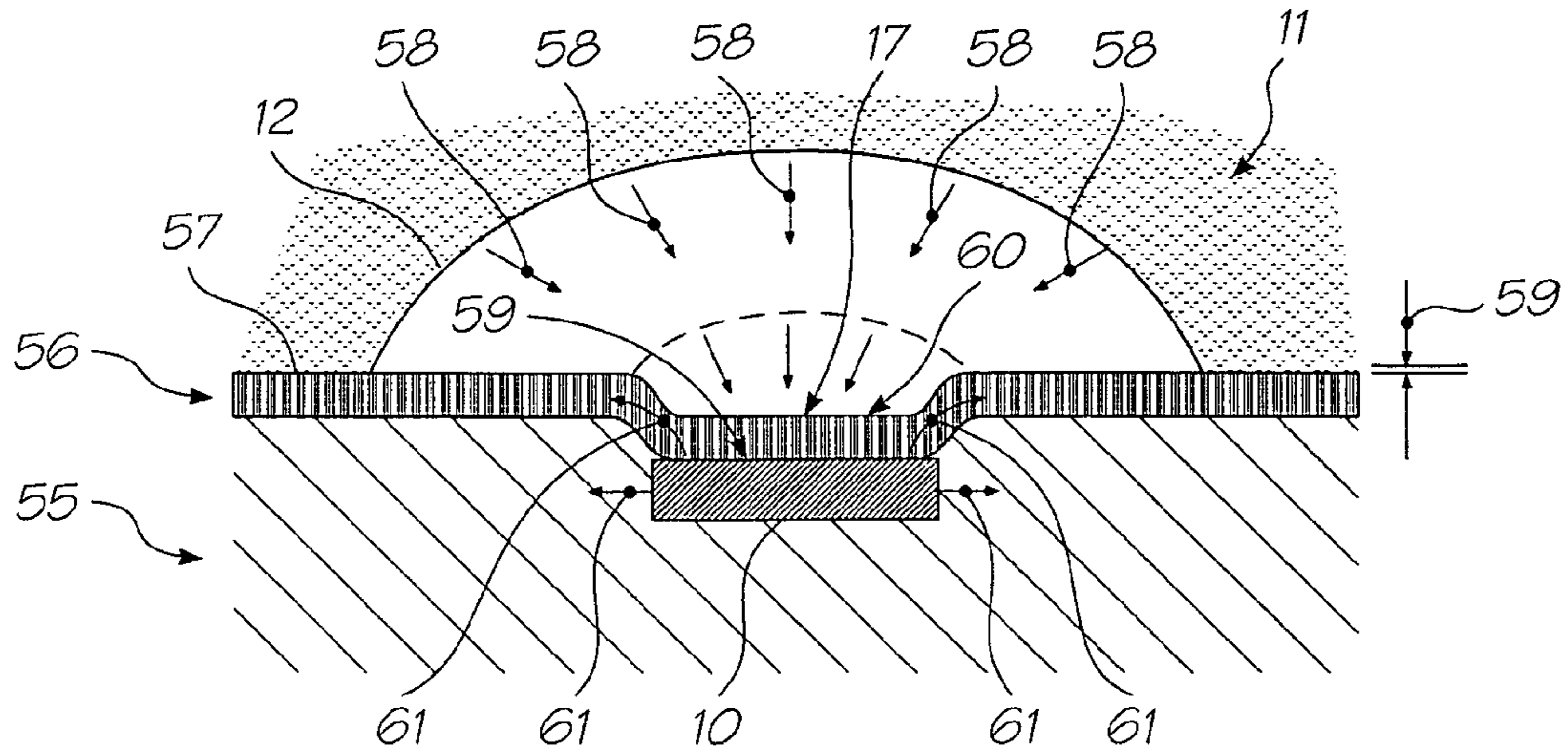
FIG. 47 (PRIOR ART)
