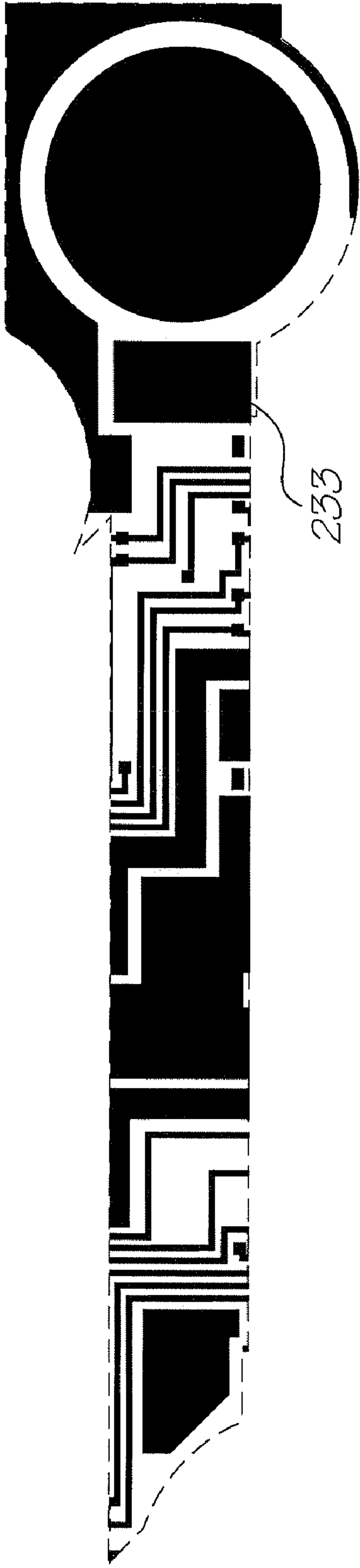
Metal 2 mask
