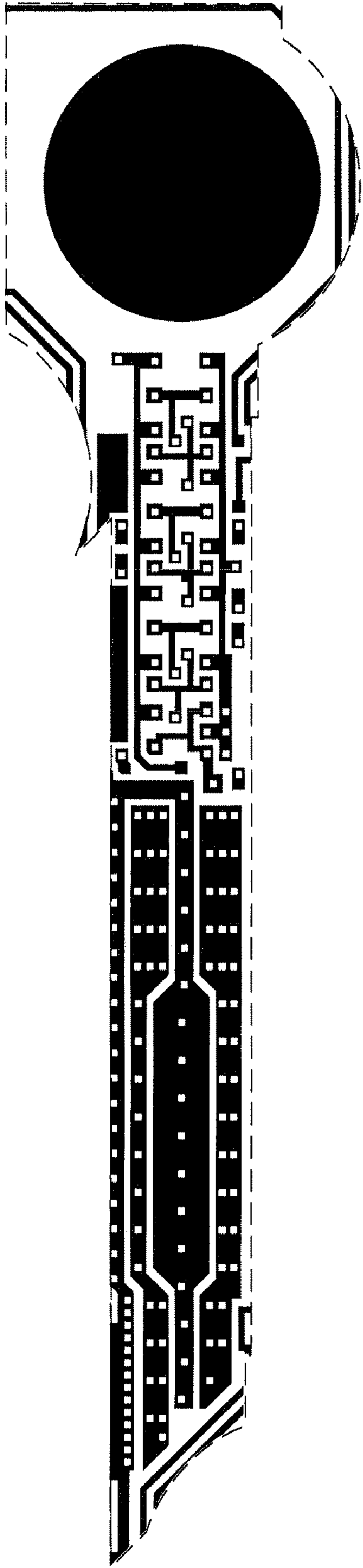
Metal 1 mask
