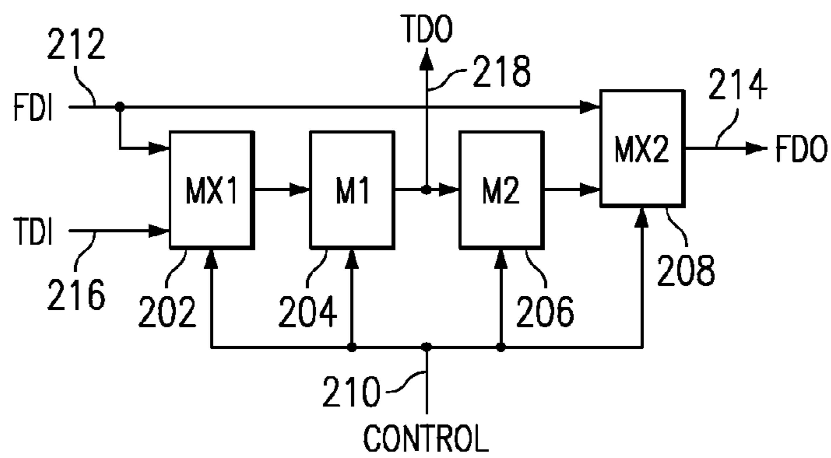
FIG. 2 (PRIOR ART)
