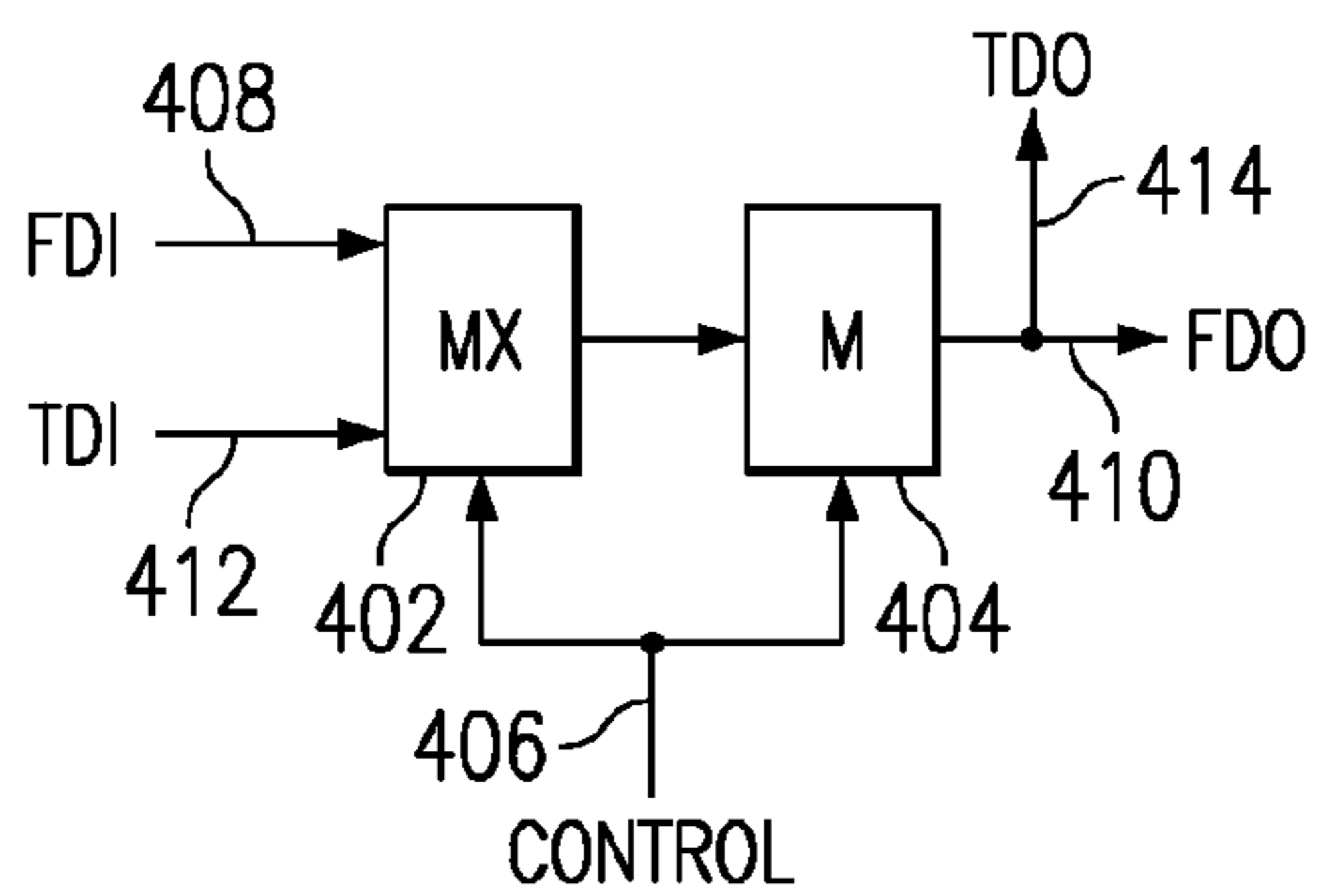
FIG. 4 (PRIOR ART)
