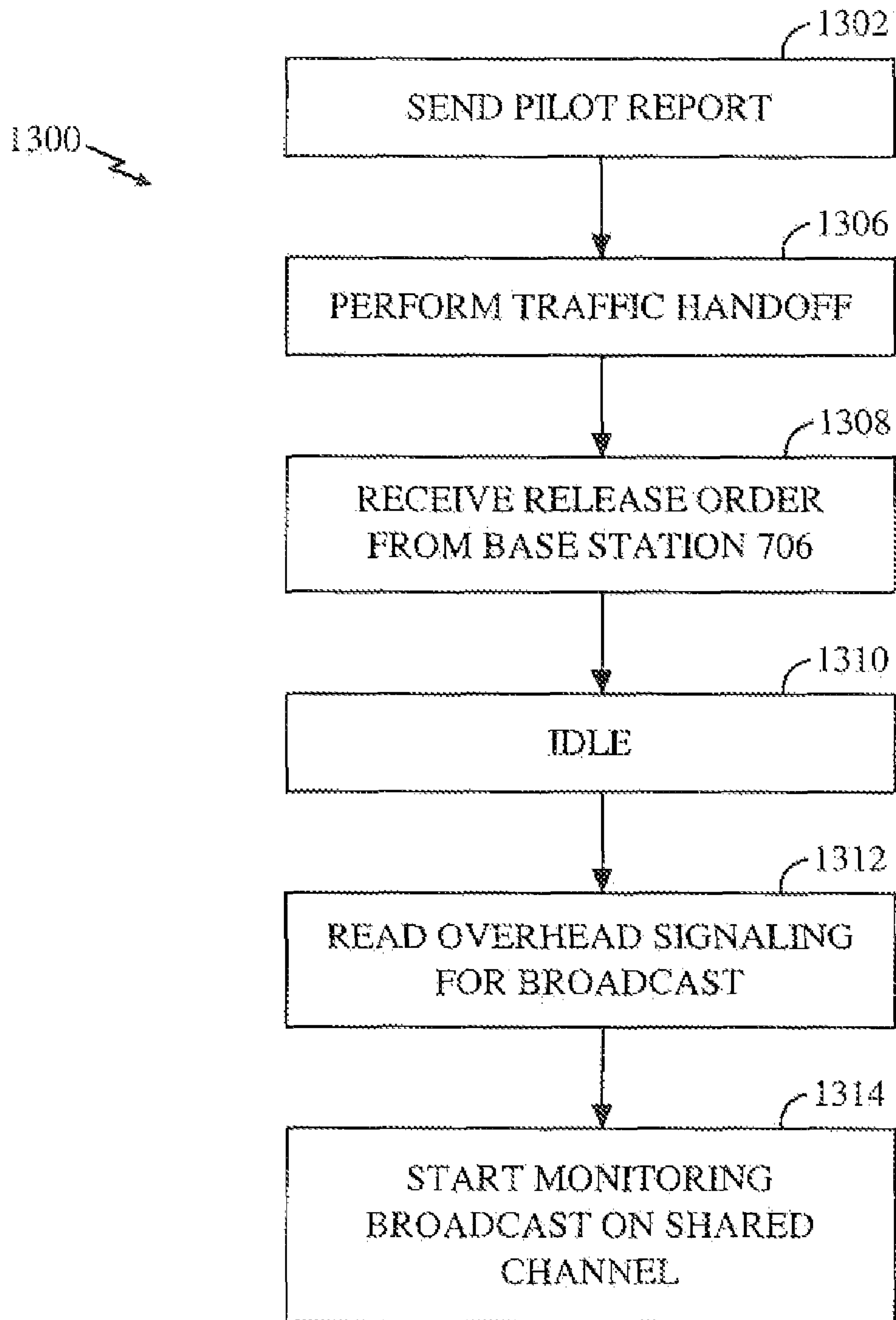
INDIVIDUAL-TO-SHARED HANDOFF OPERATION OF REMOTE (SECOND EMBODIMENT)
