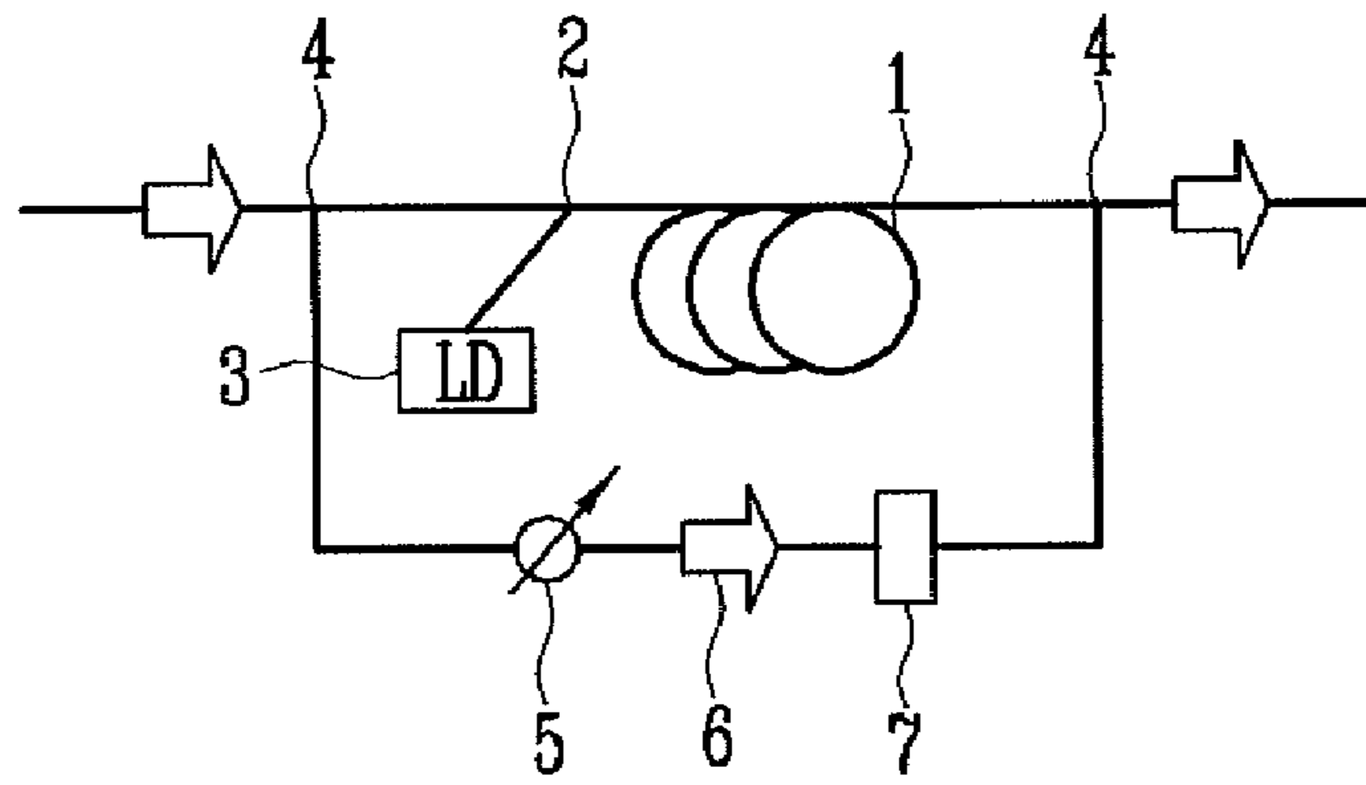
FIG. 1 (PRIOR ART)
