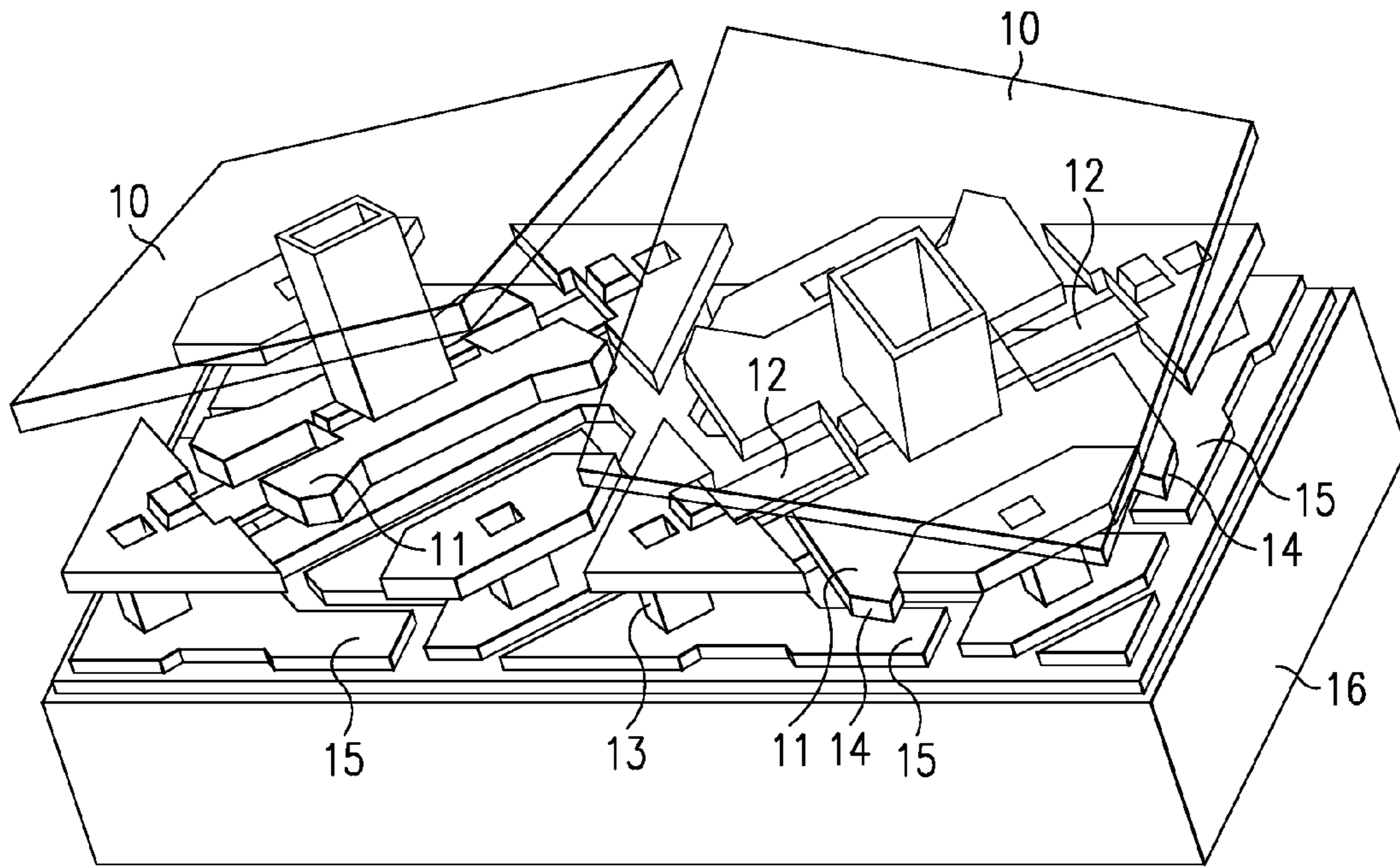
FIG. 1 (PRIOR ART)
