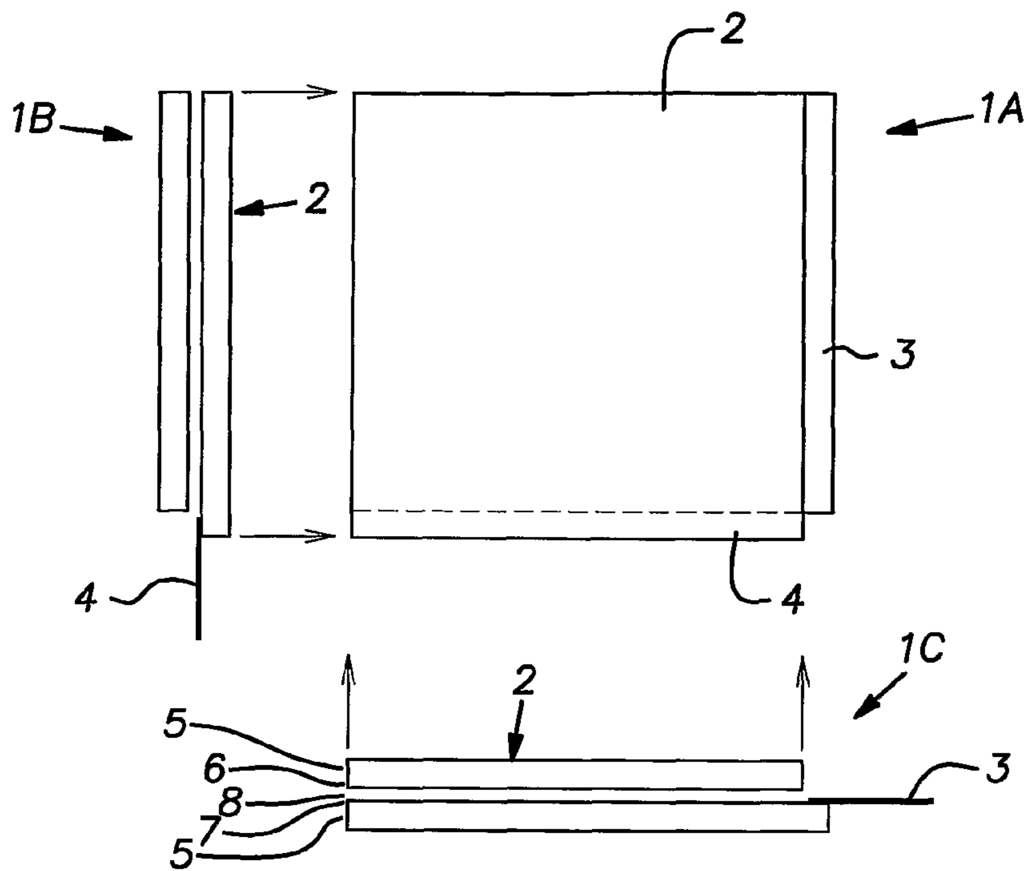
FIG. 1 PRIOR ART
