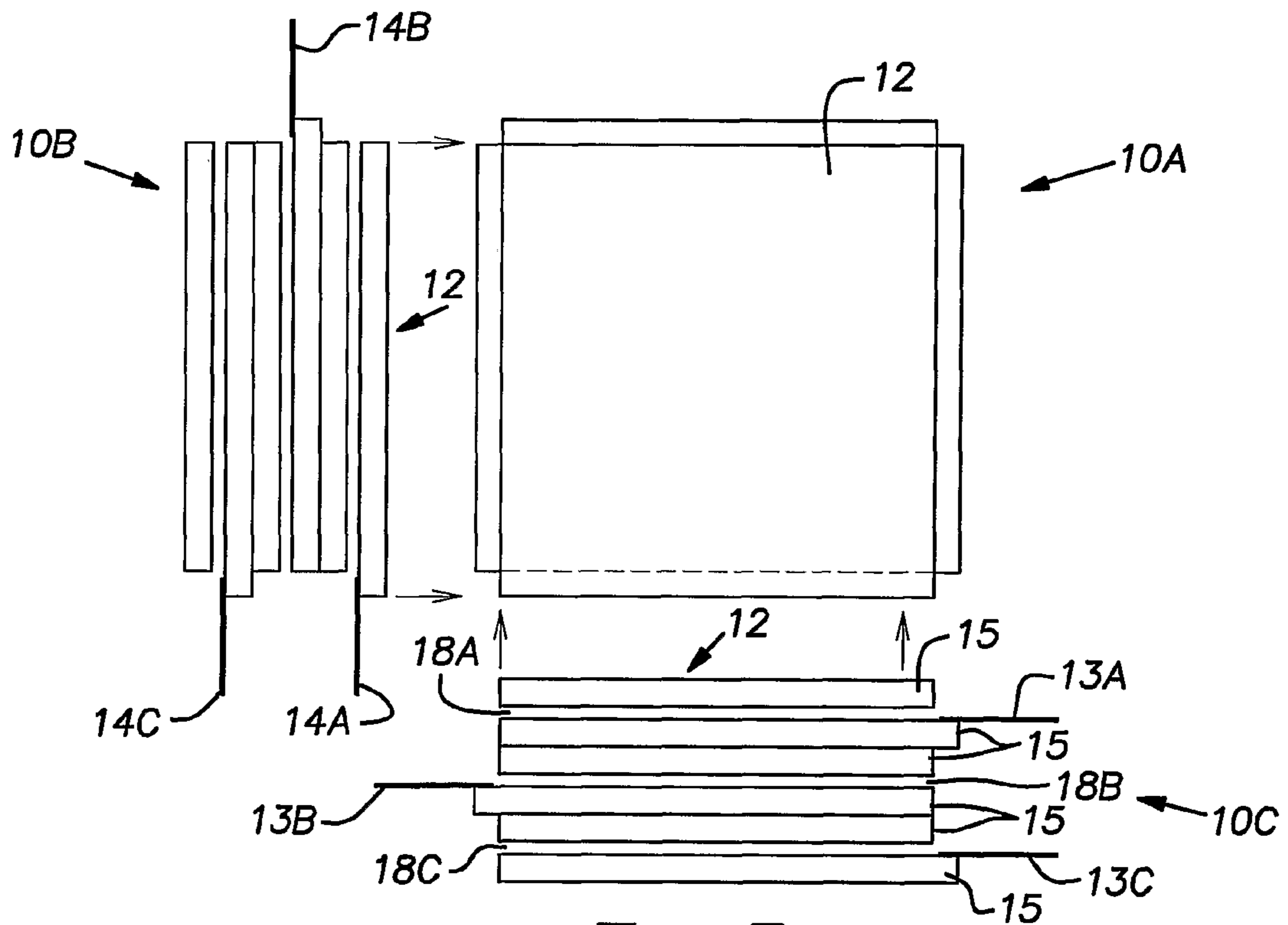
FIG. 2 PRIOR ART
