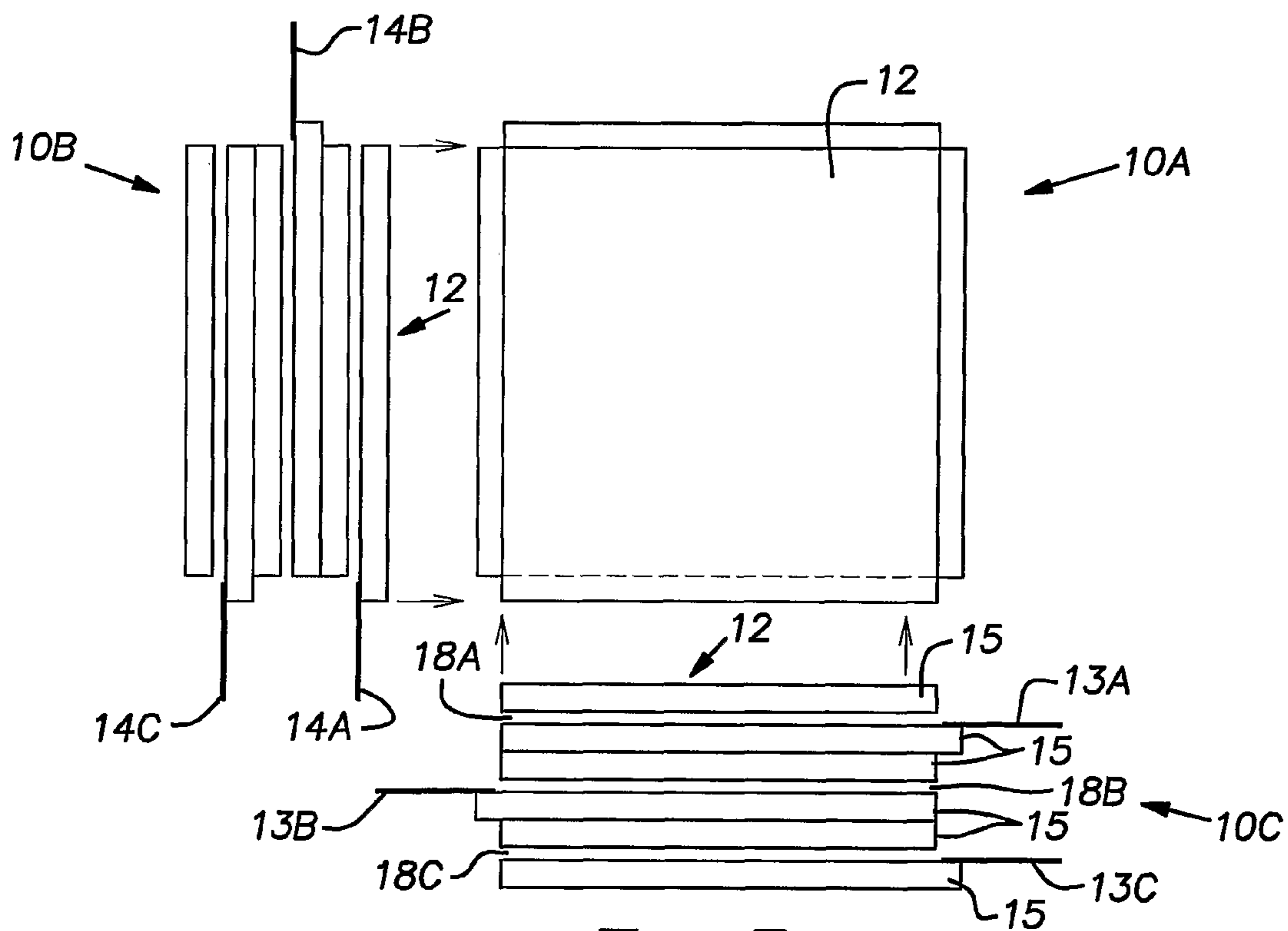
FIG. 2 PRIOR ART
