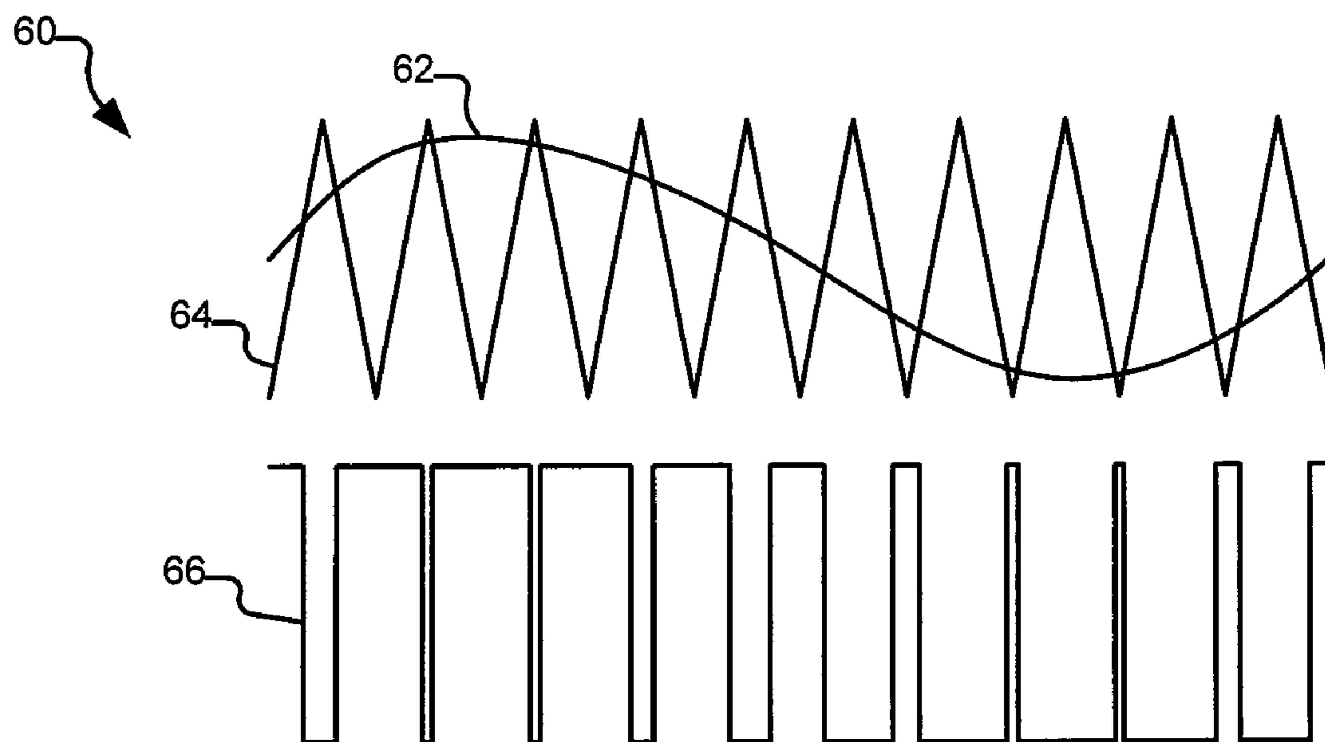
FIG. 4 (PRIOR ART)
