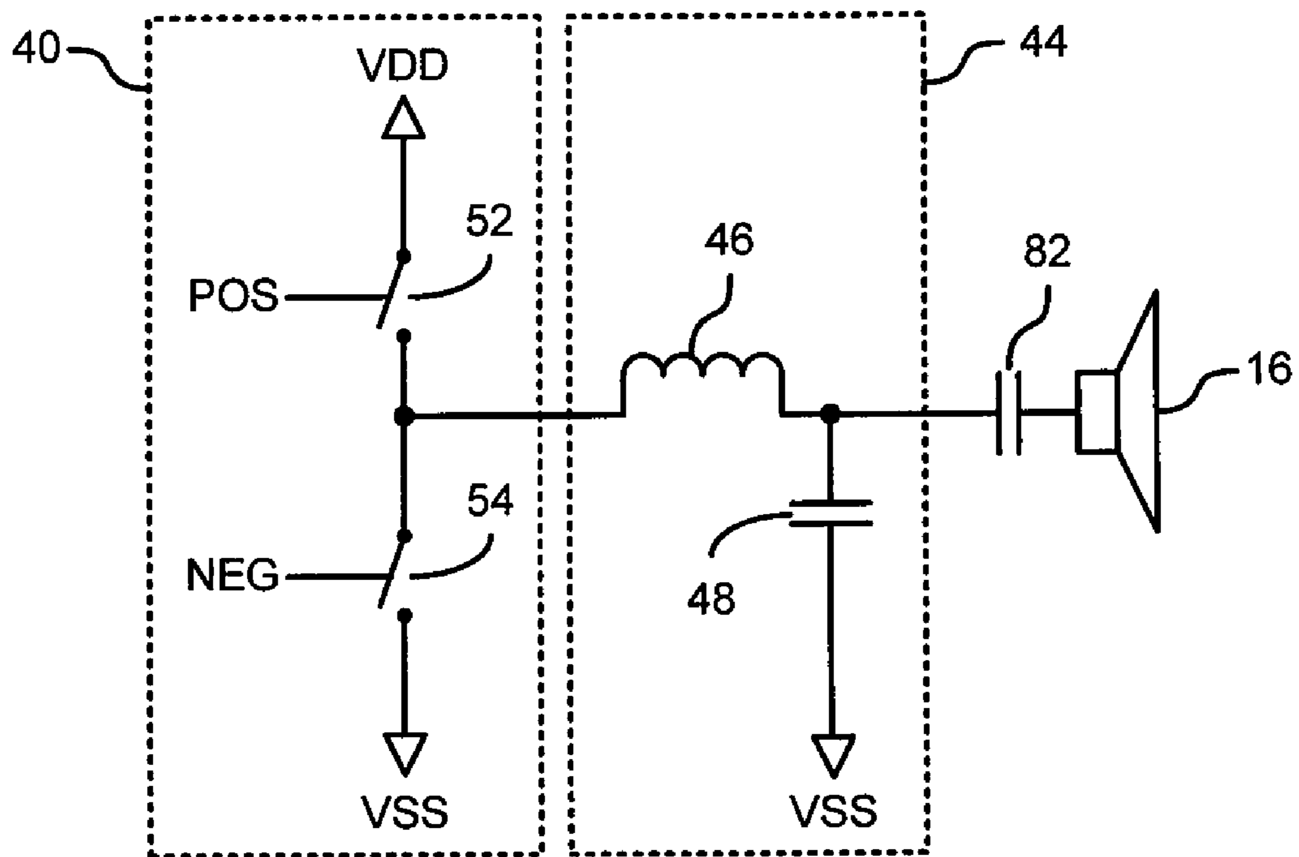
FIG. 3 (PRIOR ART)
