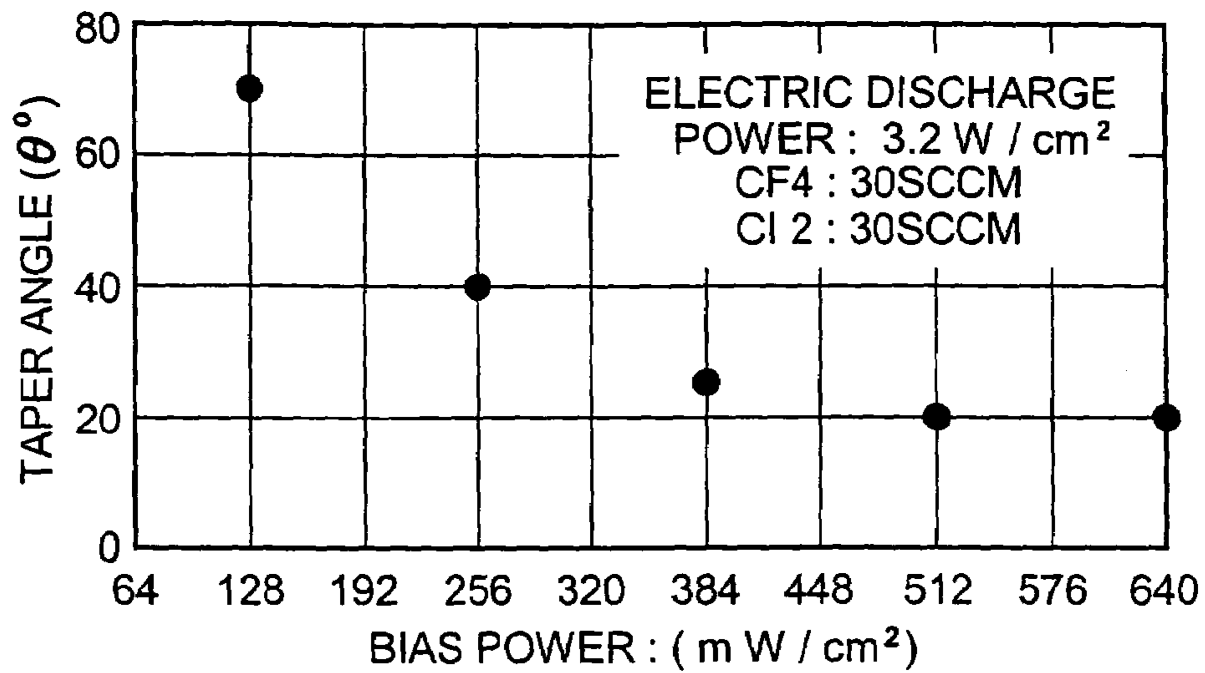
DEPENDENCE OF TAPER ANGLE ON BIAS POWER
