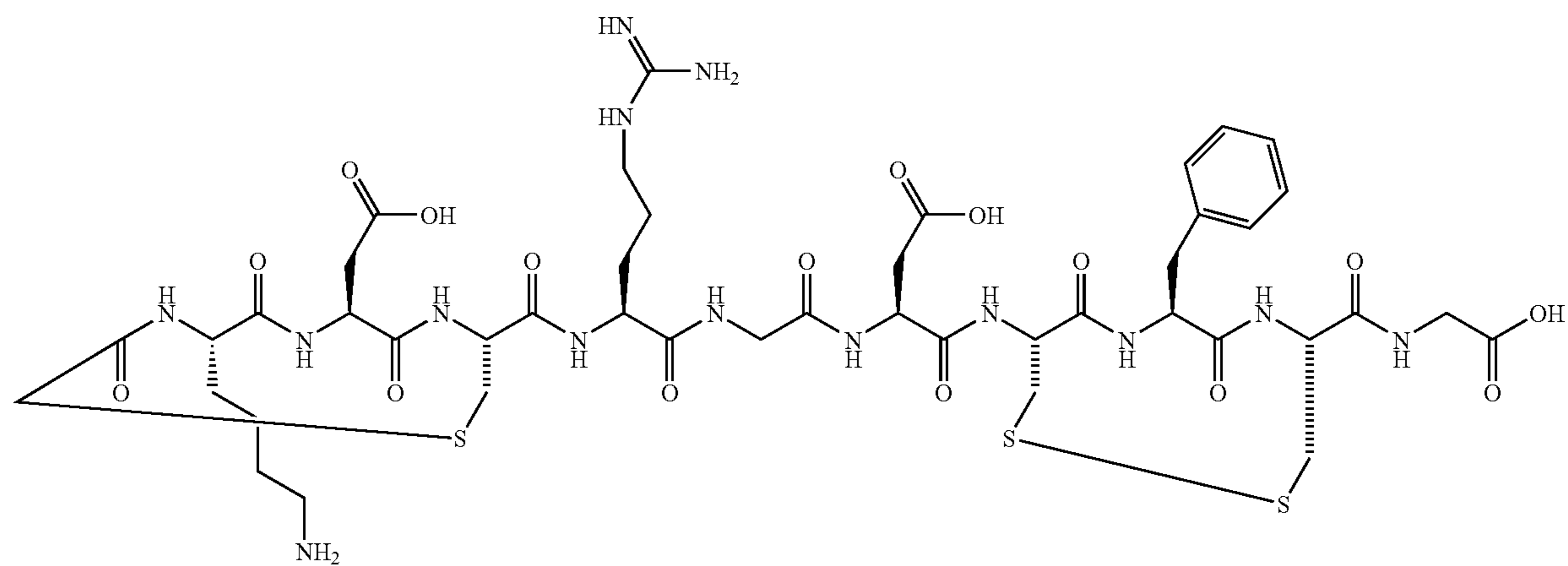
Compound 2: Vector
