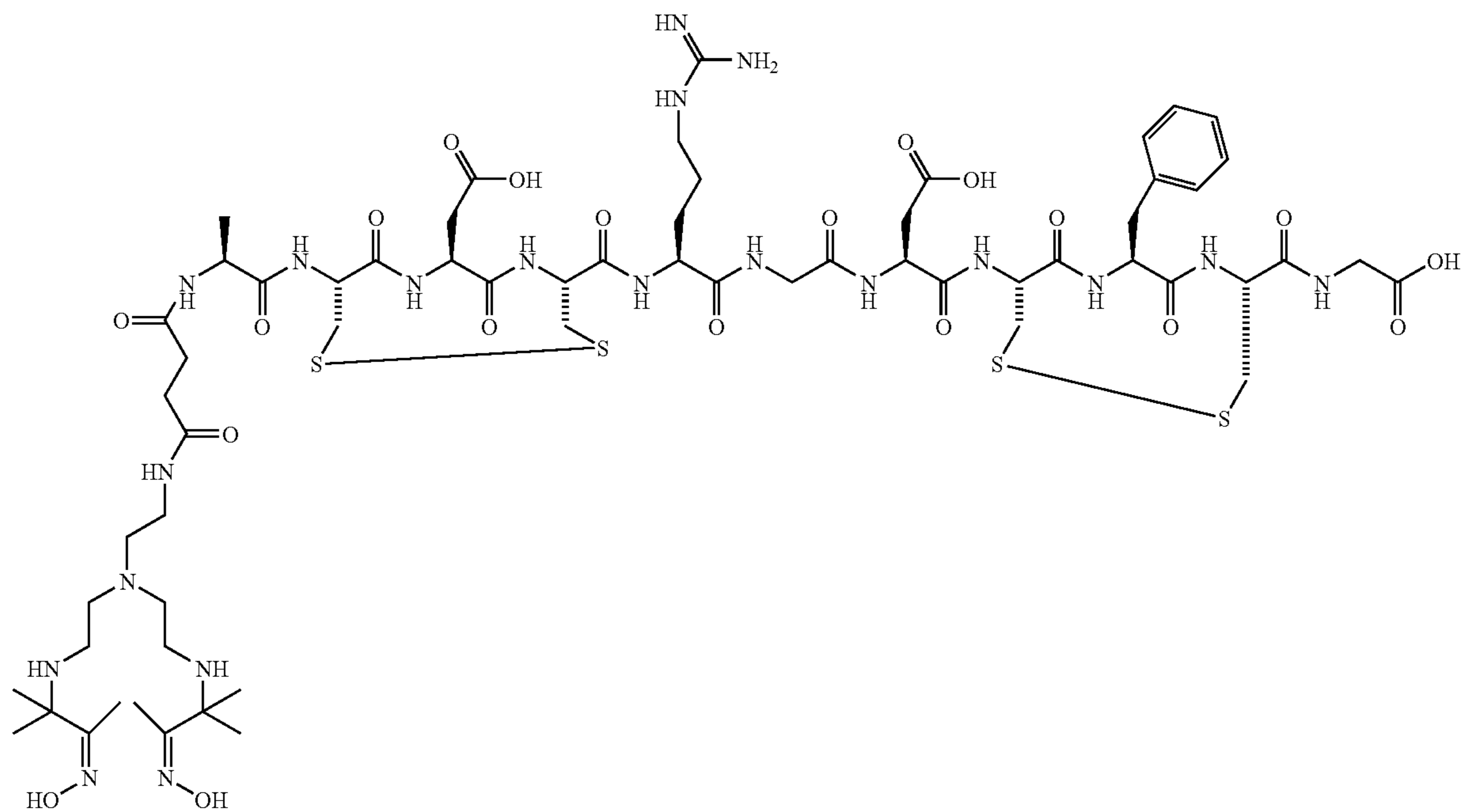
Compound 1:
