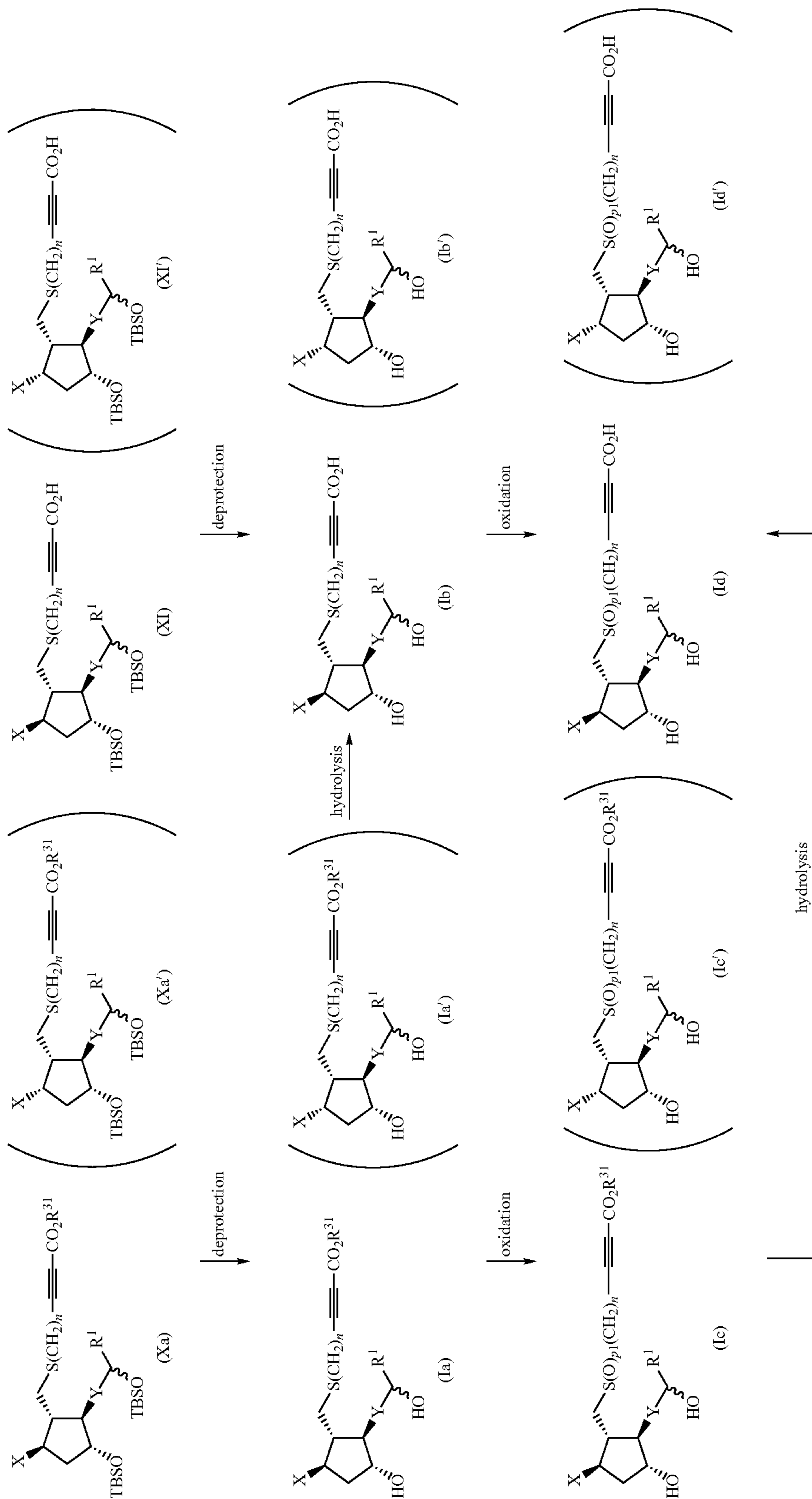
Reaction Scheme 2
