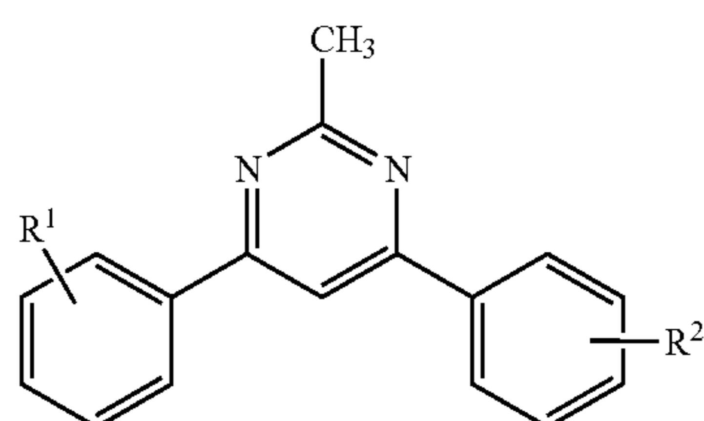
LC-MS analysis of methylpyrimidines (9).
