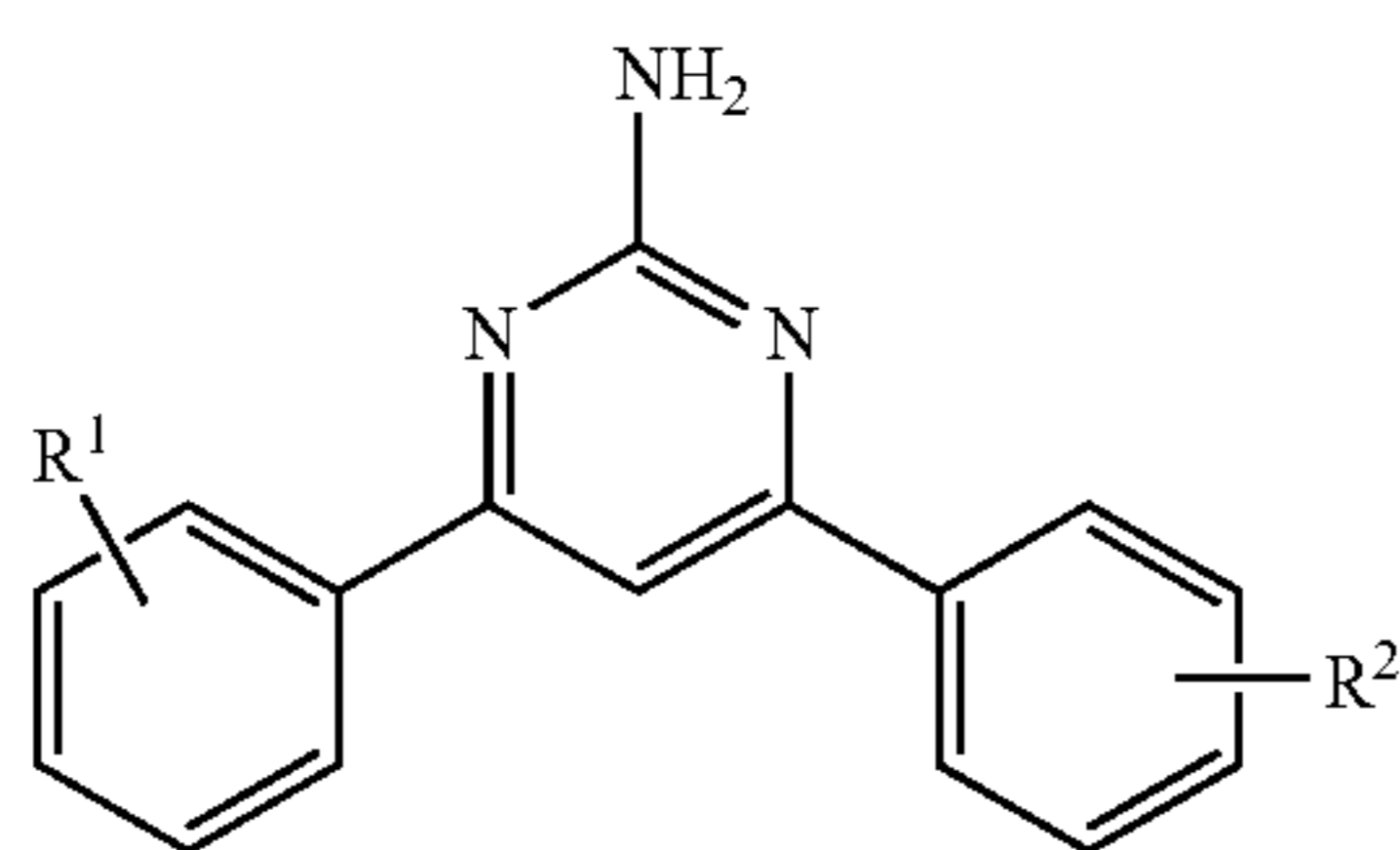
LC-MS analysis of aminopyrimidines (10).
