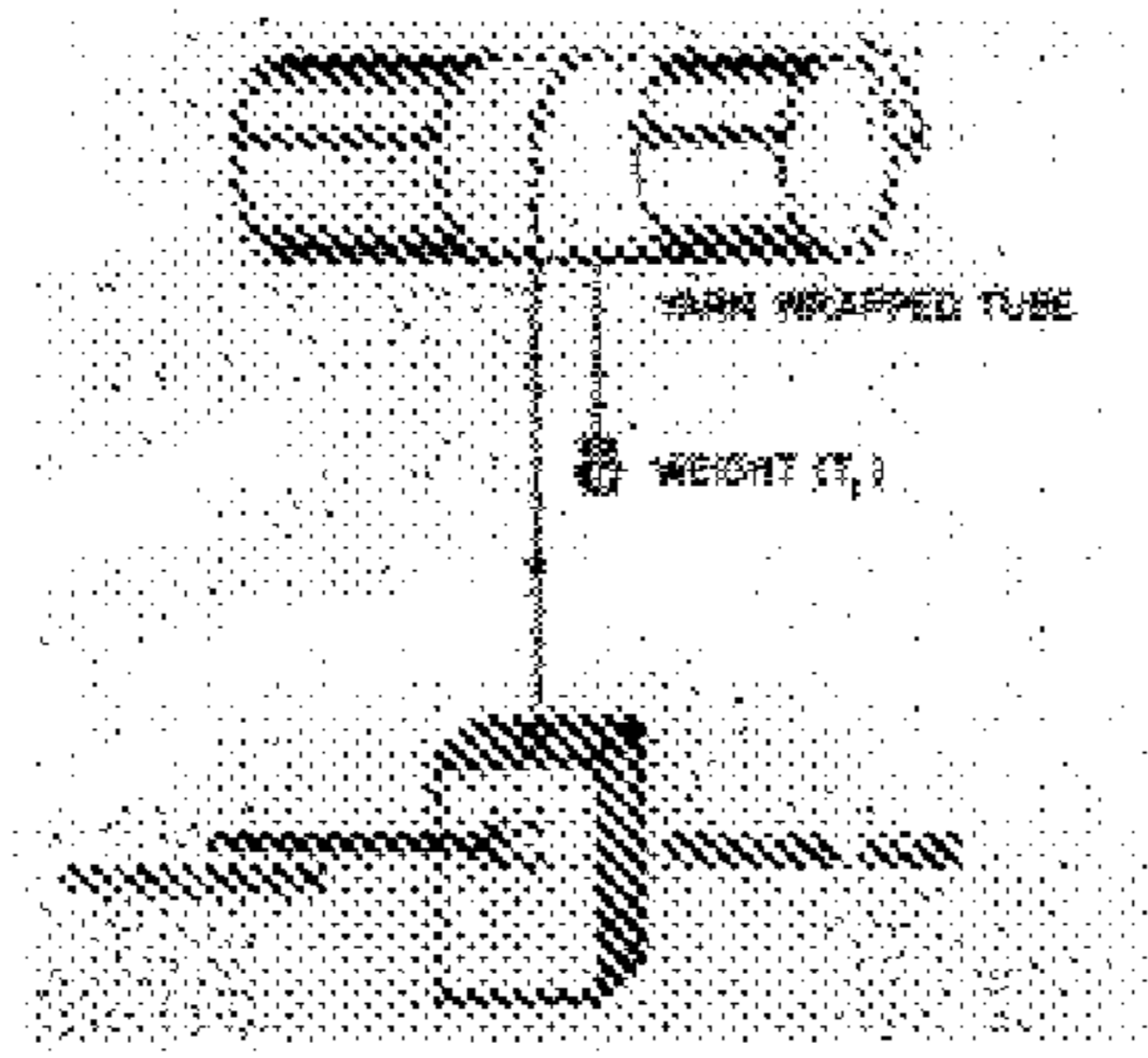
Figure 7: Capstan Yarn Friction Apparatus
