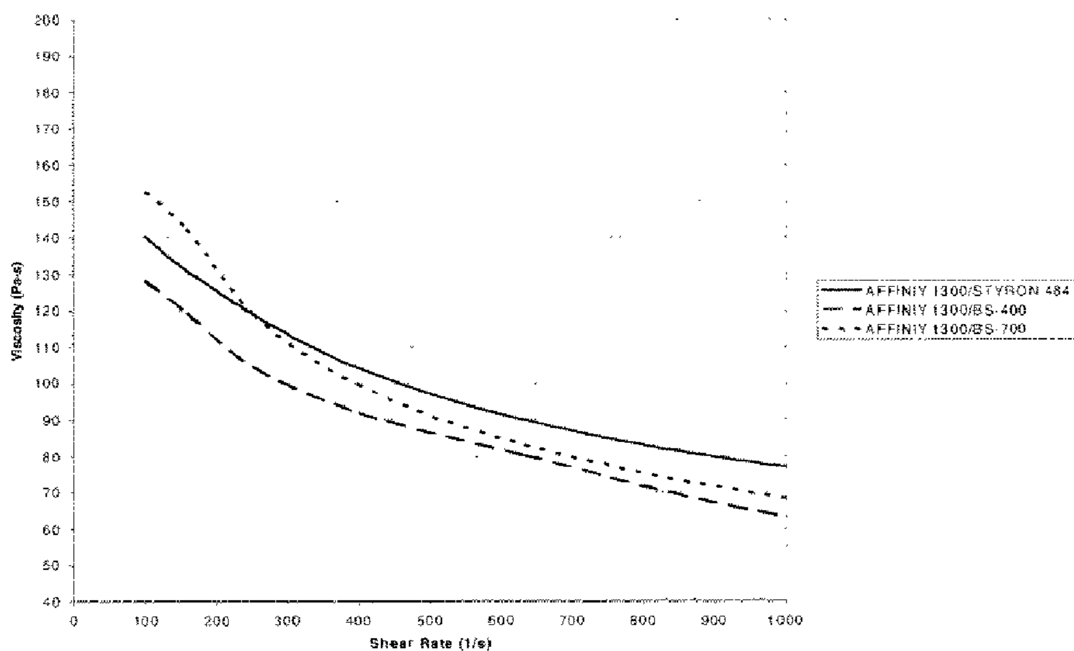
Figure 11: Viscosities of ASPUN Blends at 250°C
