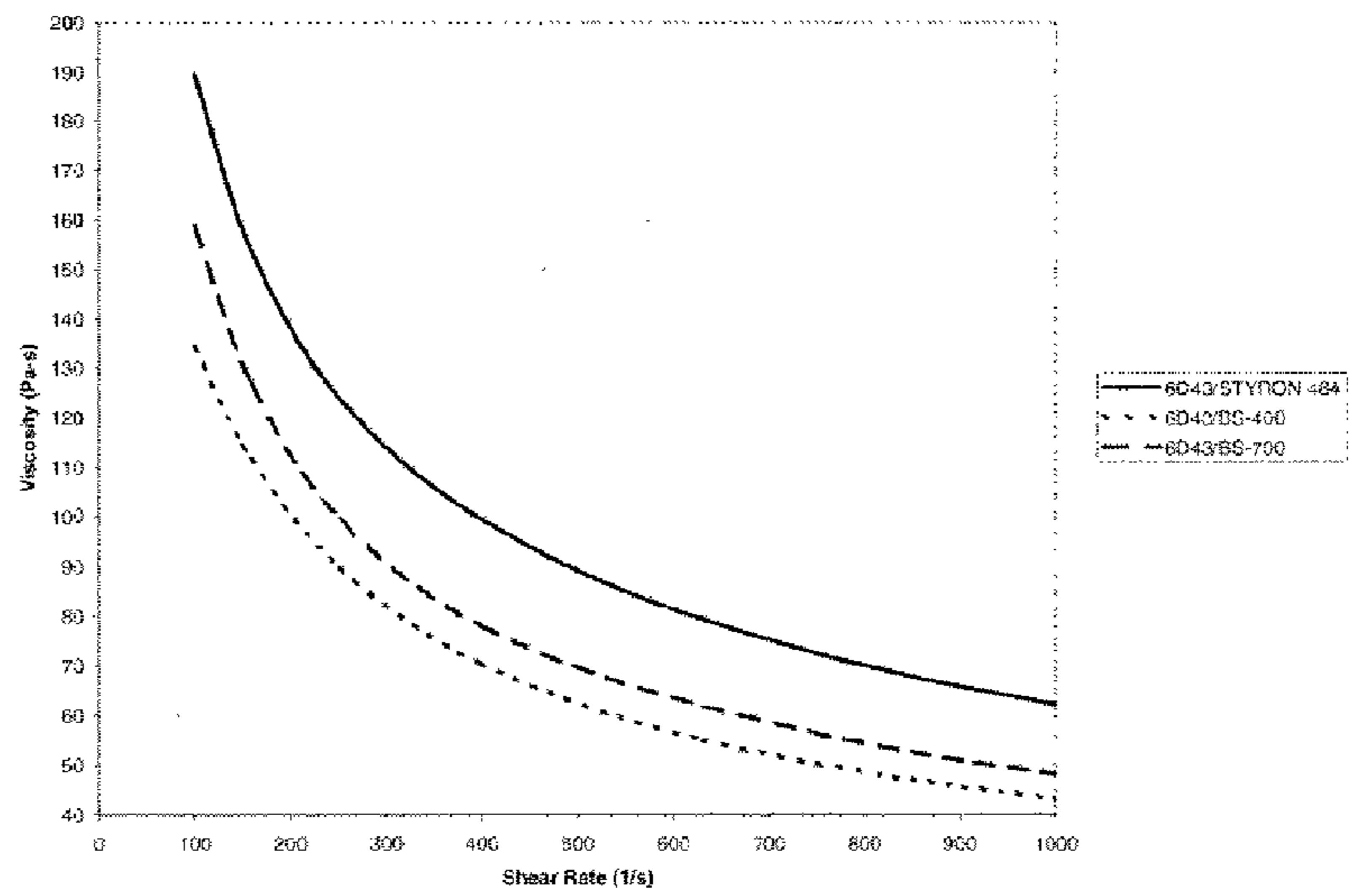
Figure 10: Viscosities of 6D43 Blends at 250°C
