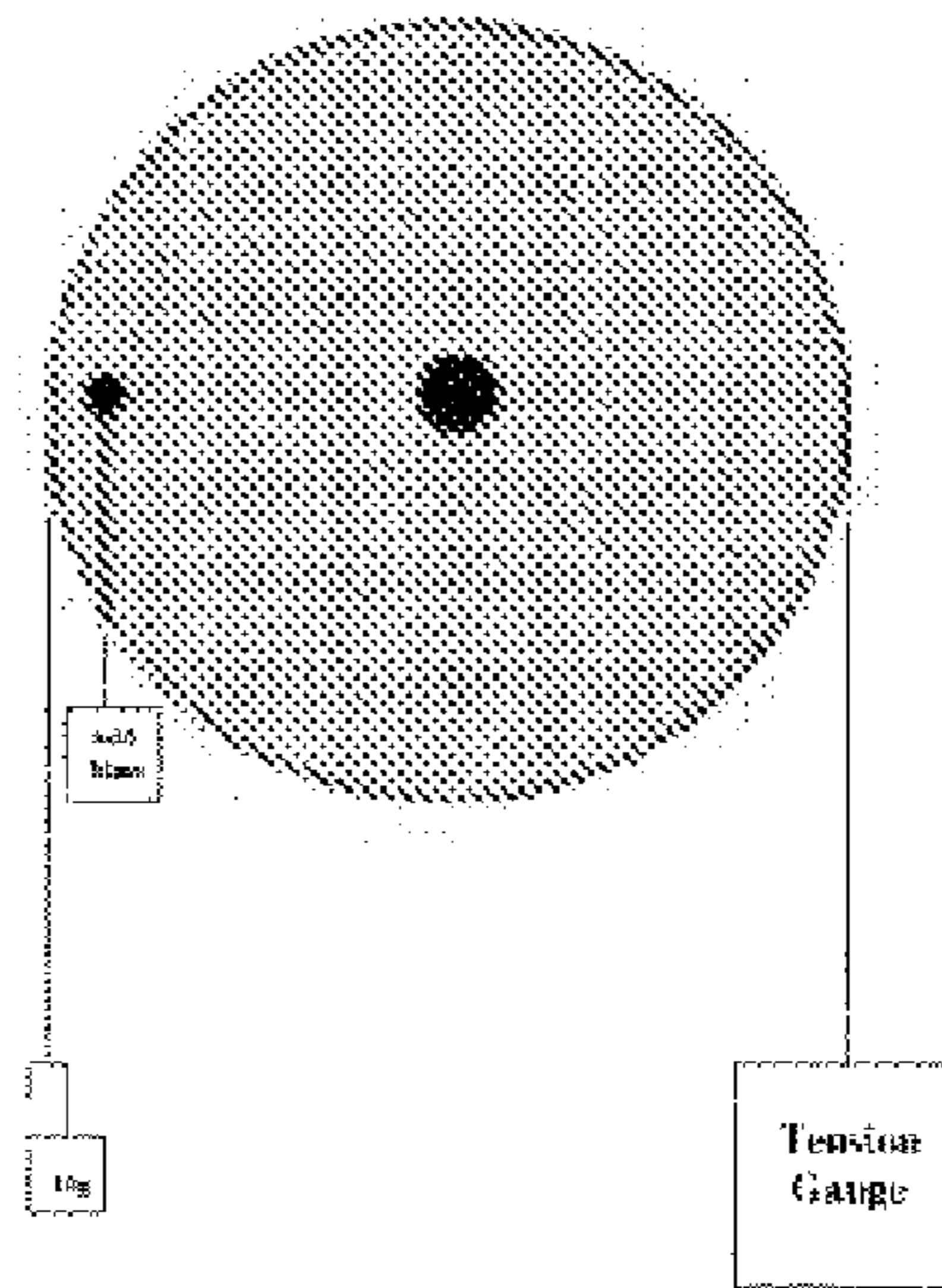
Figure 8: Static Friction Test Set-up
