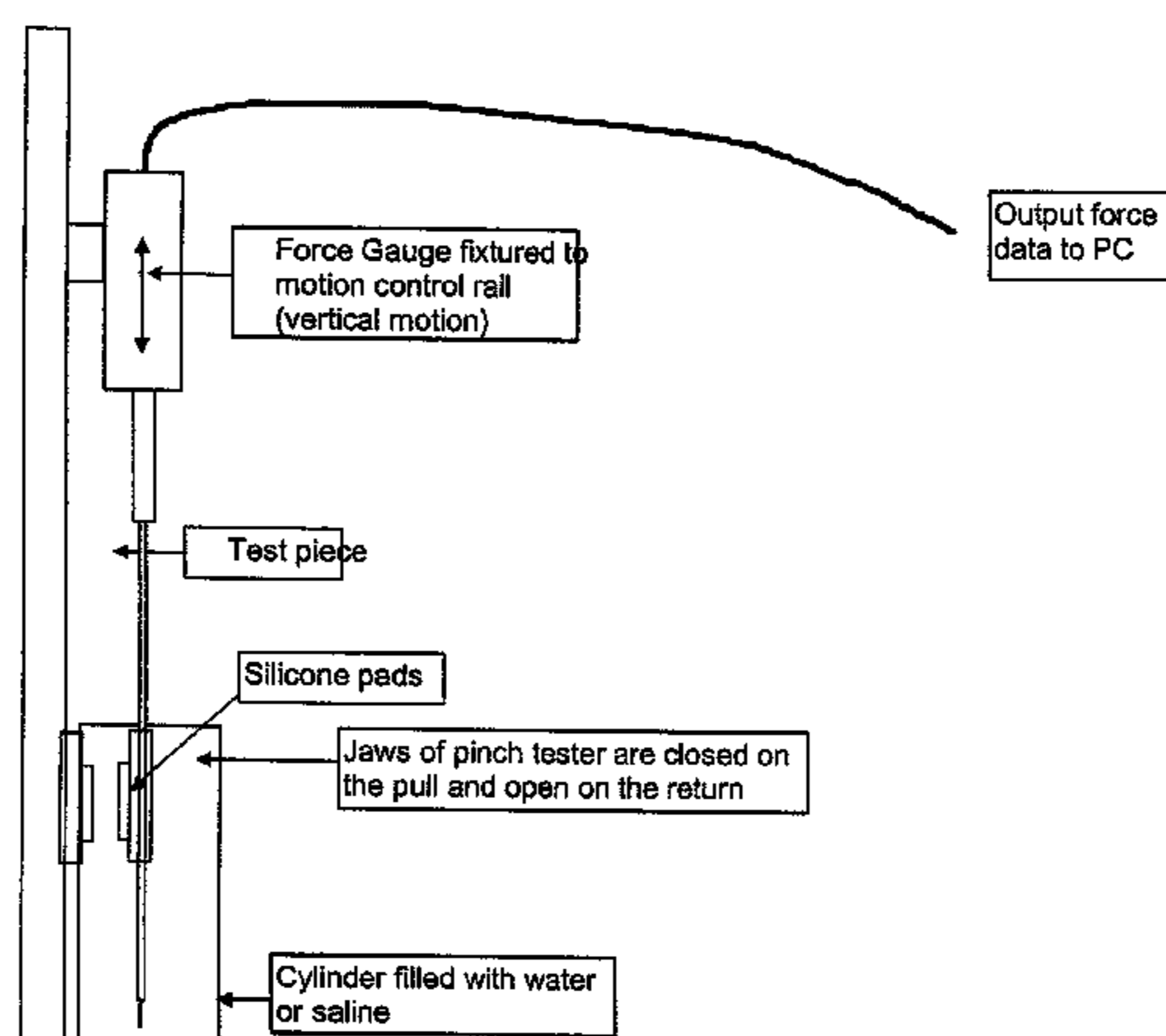
Friction Measurements by Vertical Pinch Method
