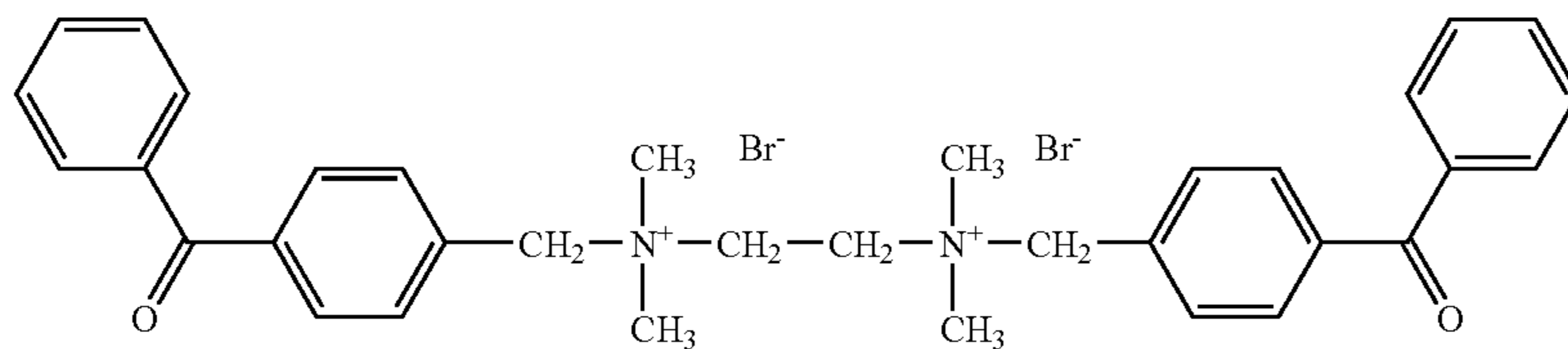
Ethylenebis(4-benzoylbenzyl)dimethylammonium) Dibromide
