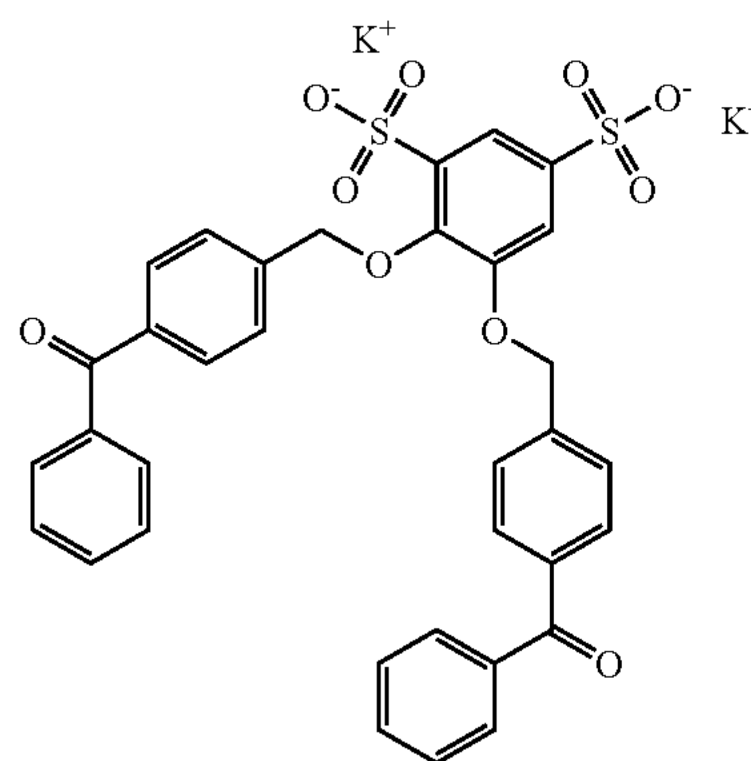
4,5-bis(4-benzoyl-phenylmethylenoxy) benzene-1,3-disulfonic acid dipotassium salt (DBDS)
