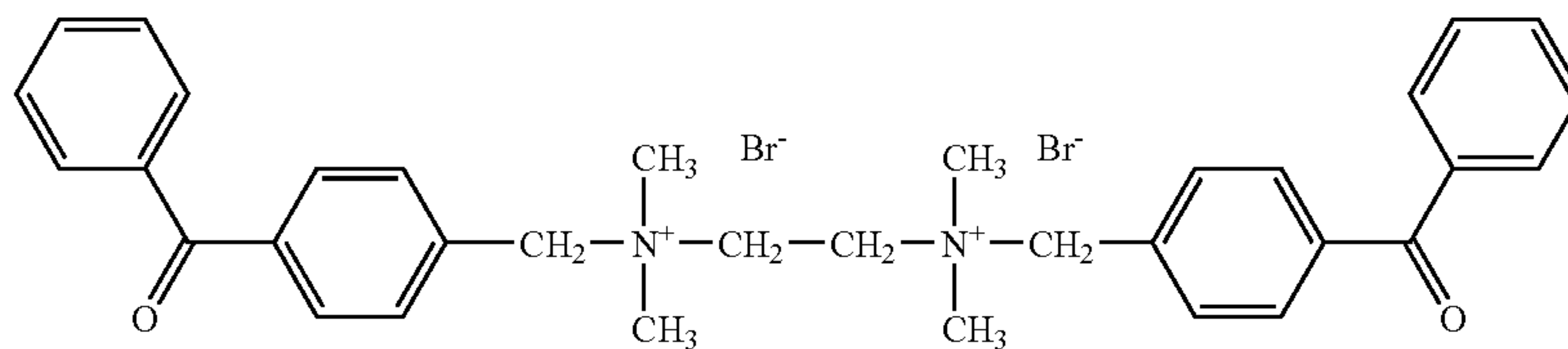
Ethylenebis(4-benzoylbenzyl)dimethylammonium) Dibromide
