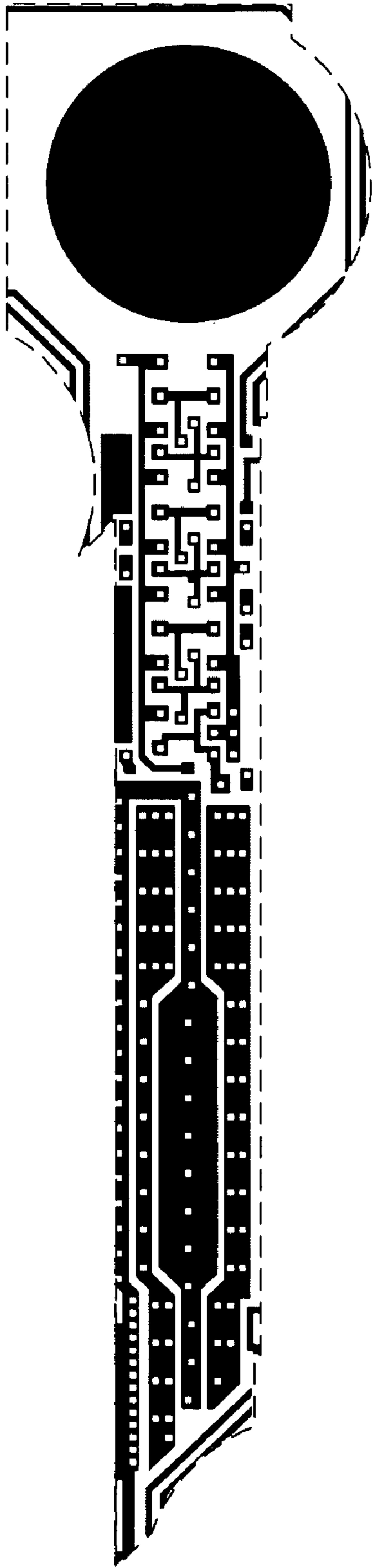
Metal 1 mask
