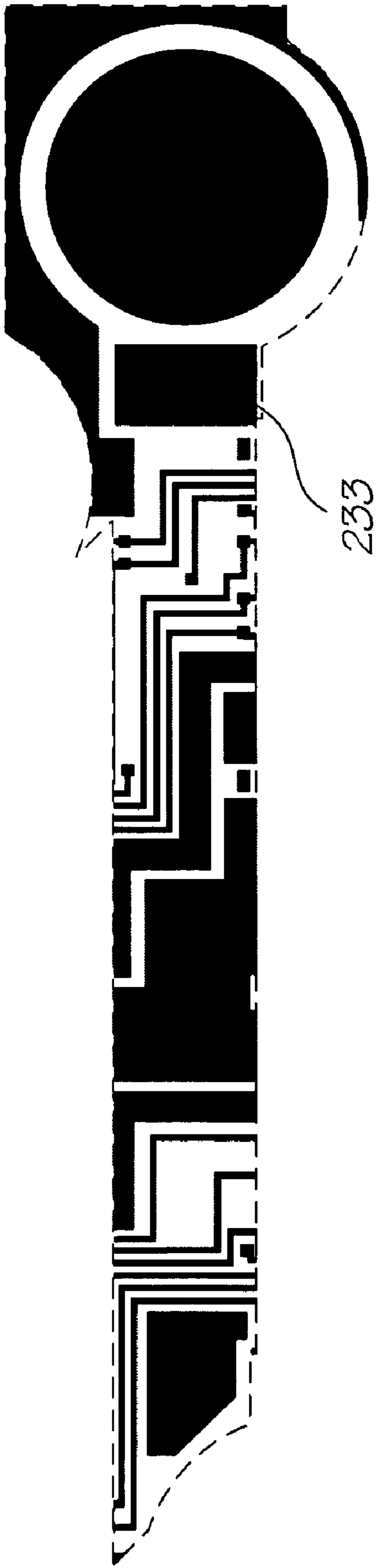
Metal 2 mask
