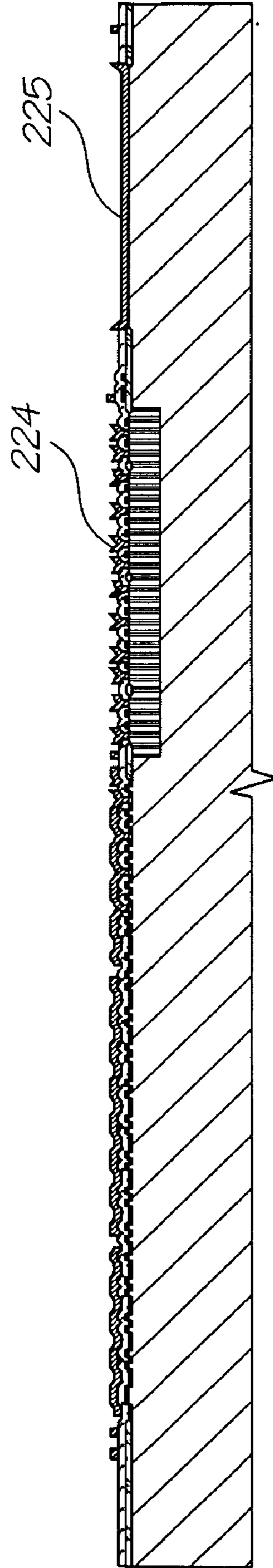
Deposit Metal 1
