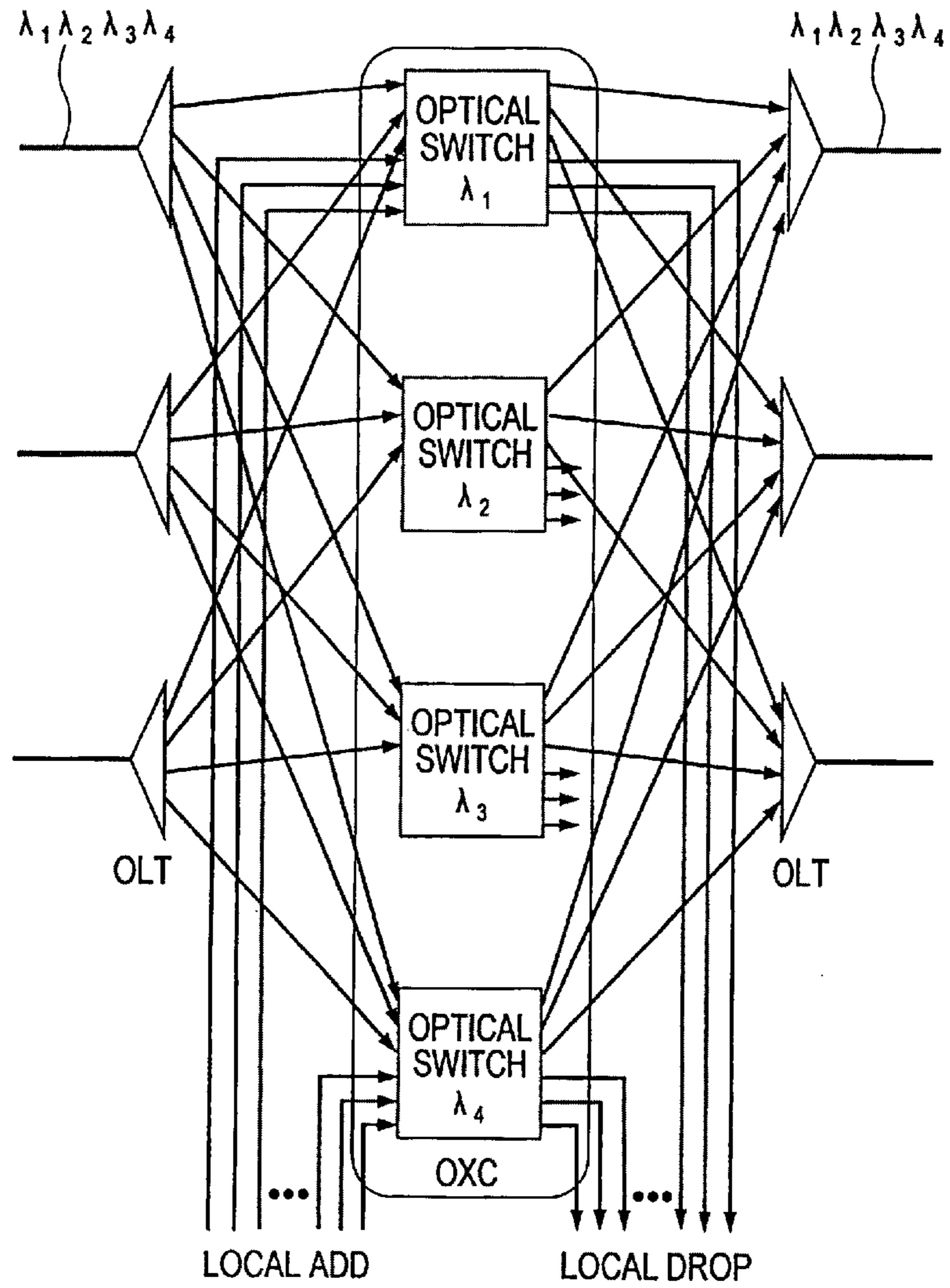
FIG. 13I PRIOR ART
