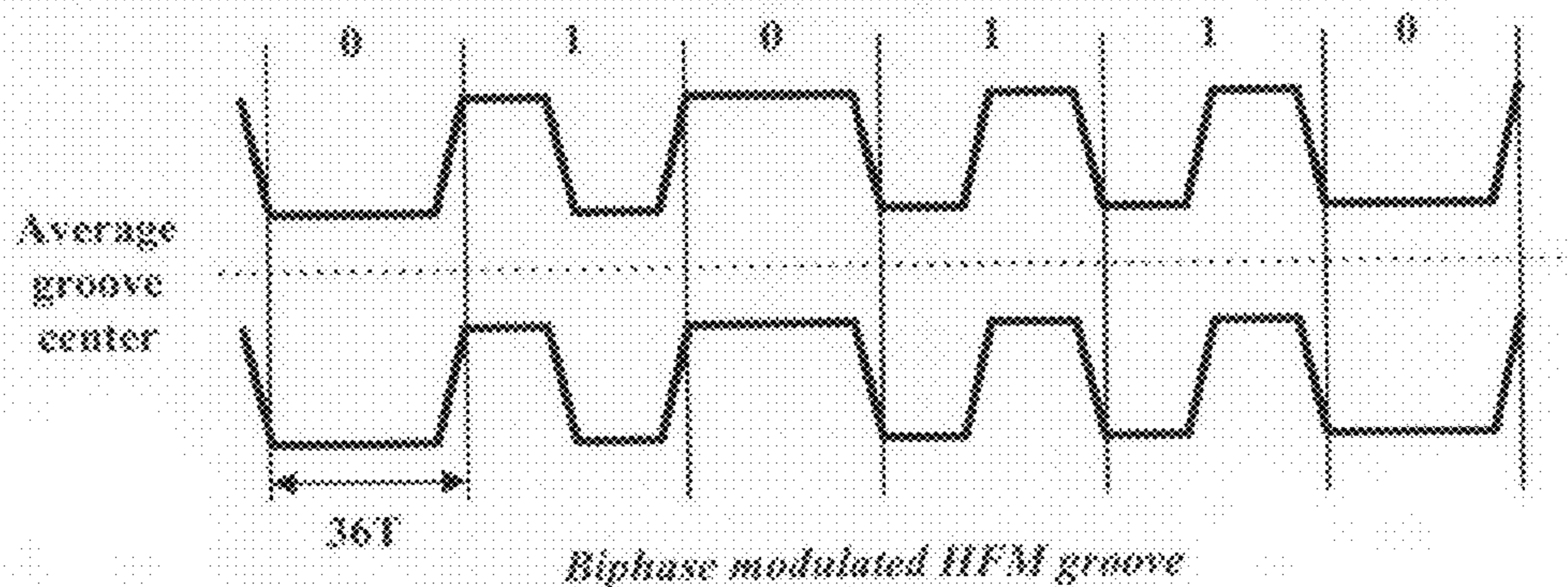
FIG. 2 (Prior Art)
