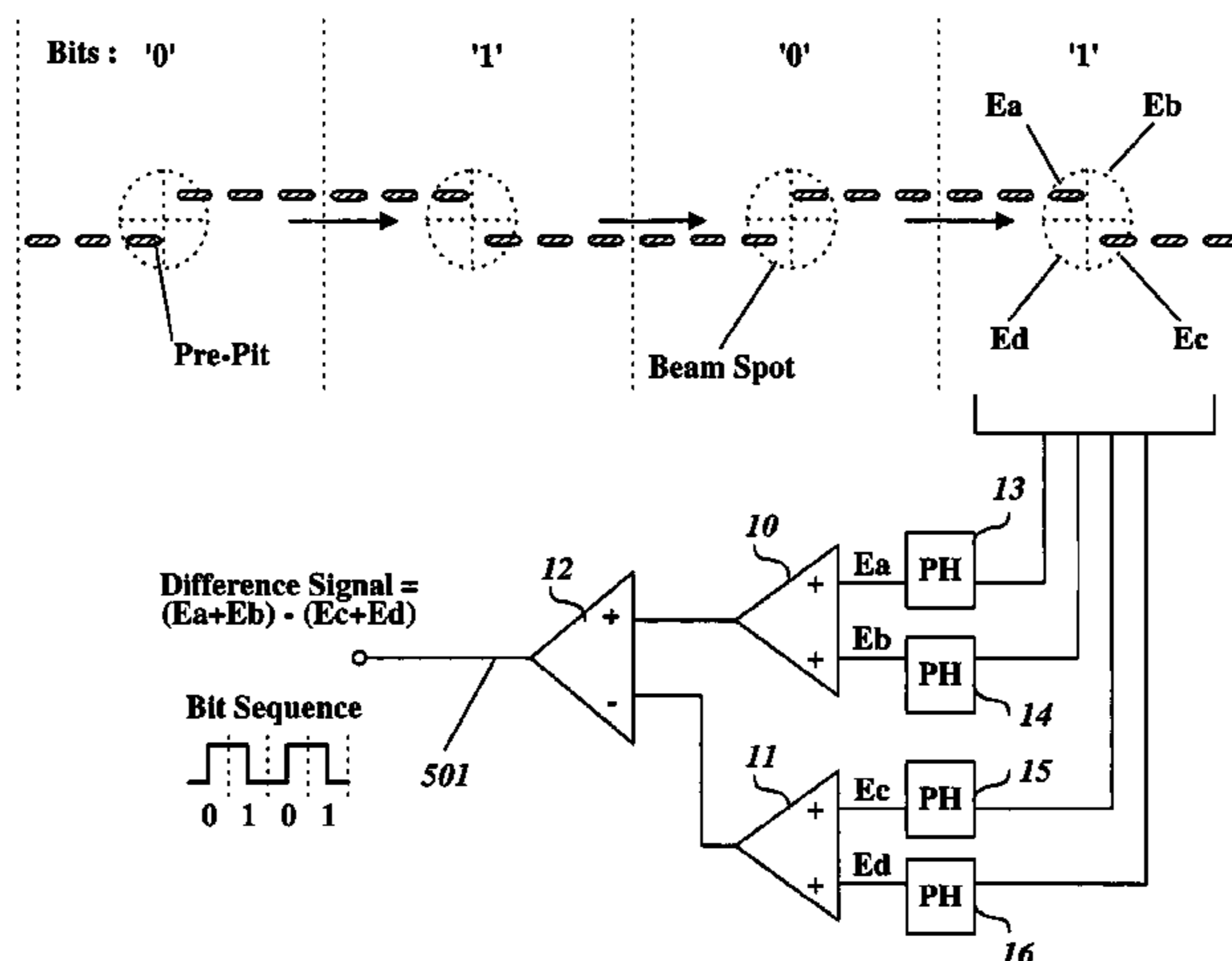
Data encoded in Wobbled Pits by Bi-Phase Modulation
