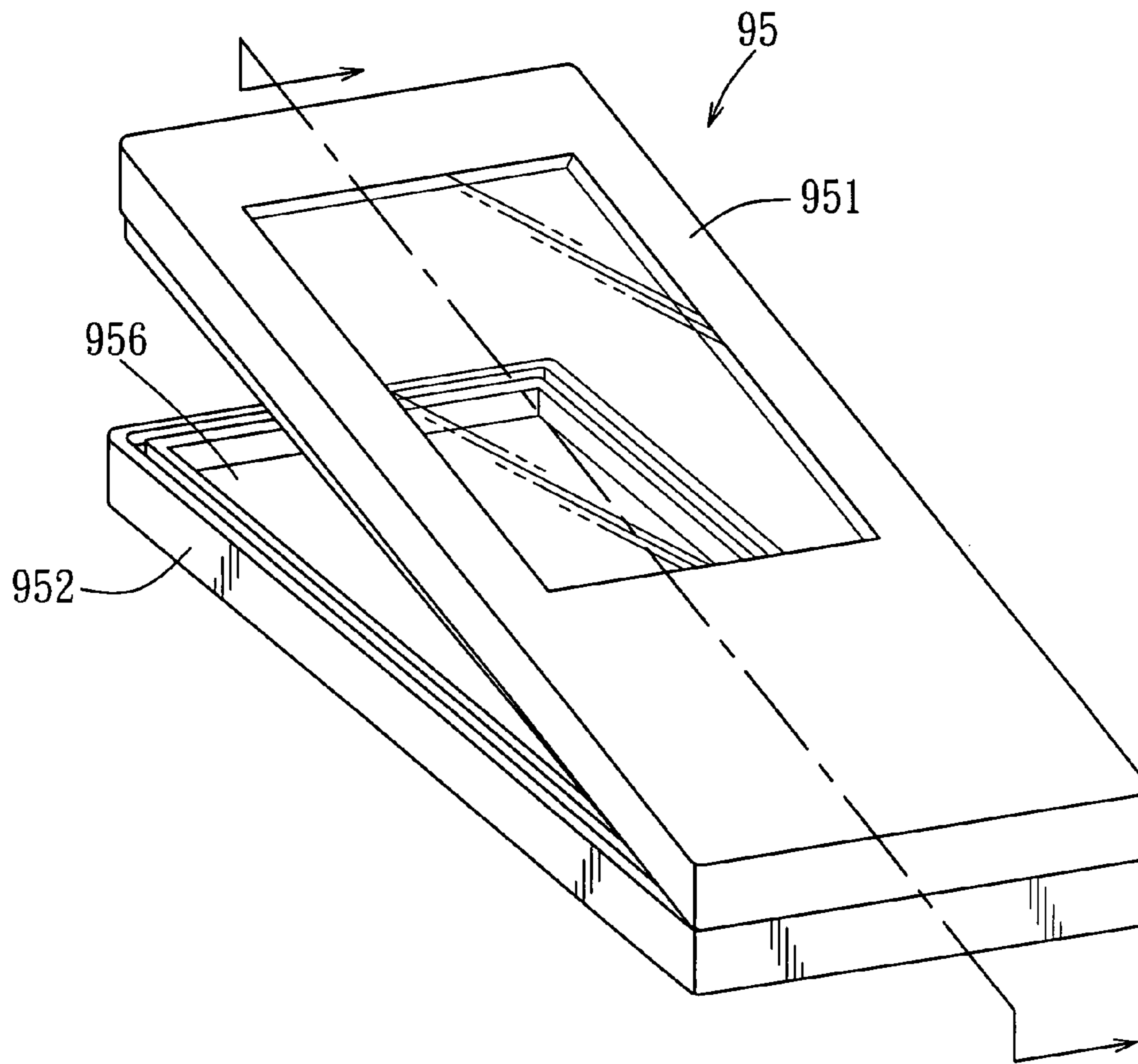
FIG. 5 PRIOR ART
