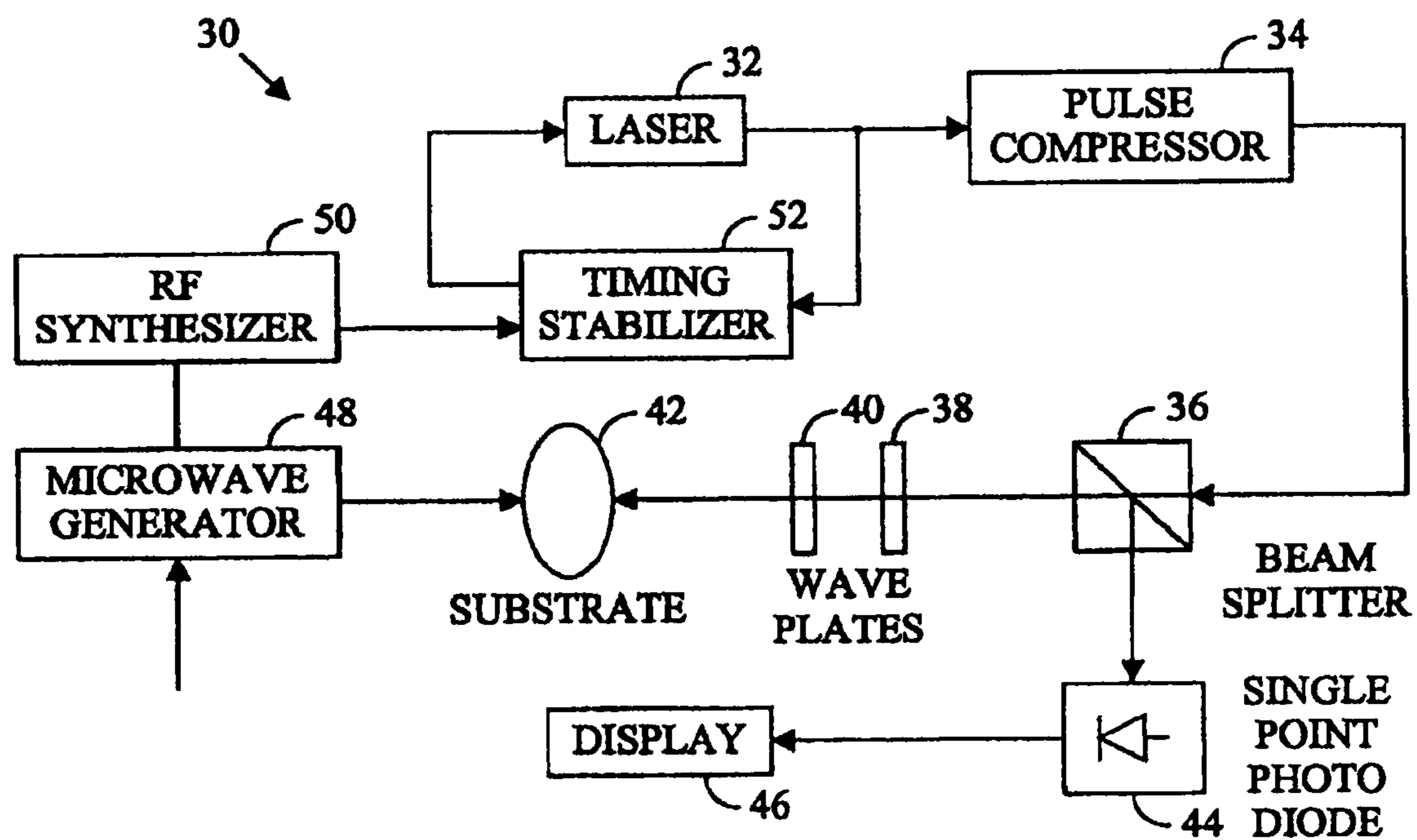
FIG. 1 PRIOR ART
