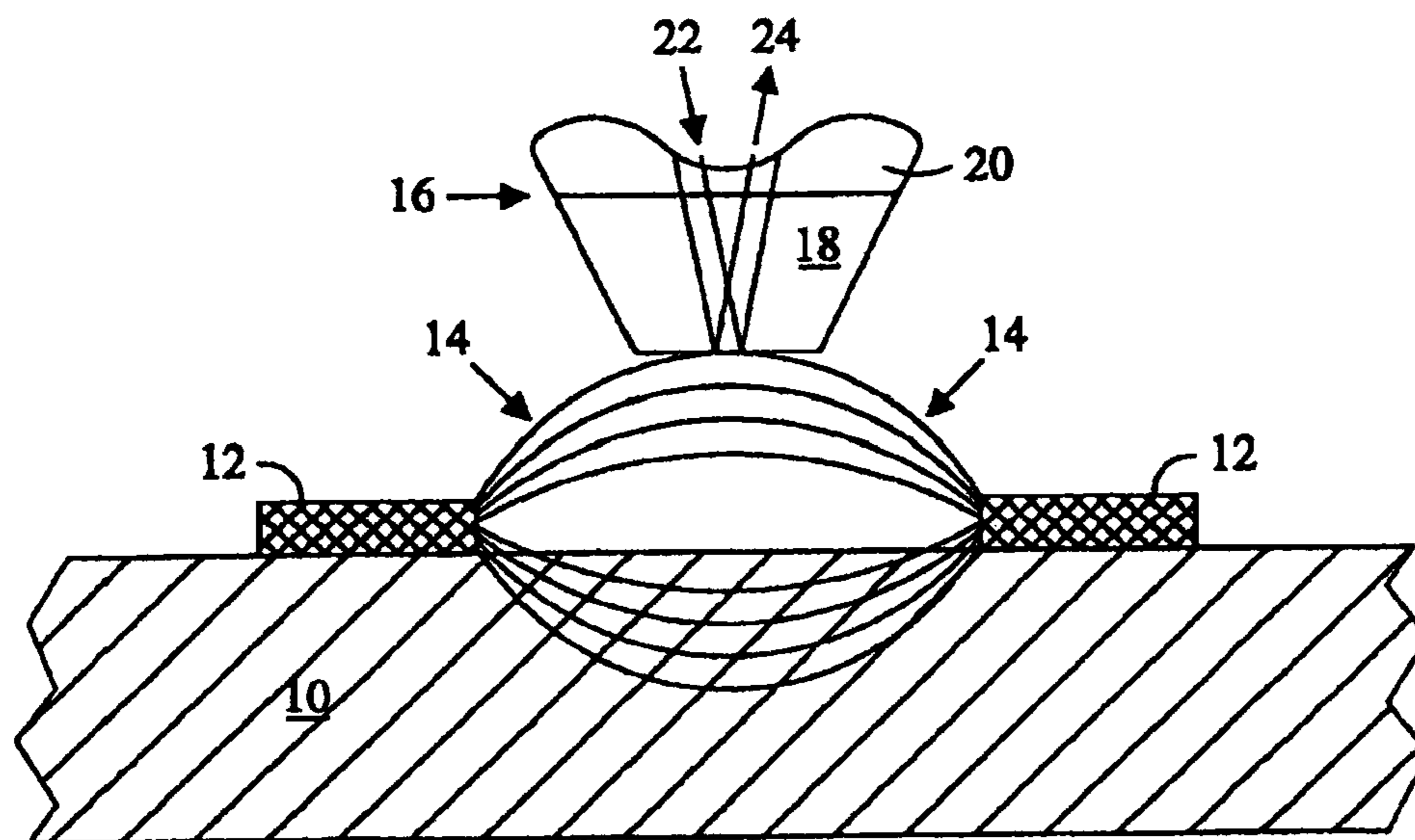
FIG. 1 PRIOR ART
