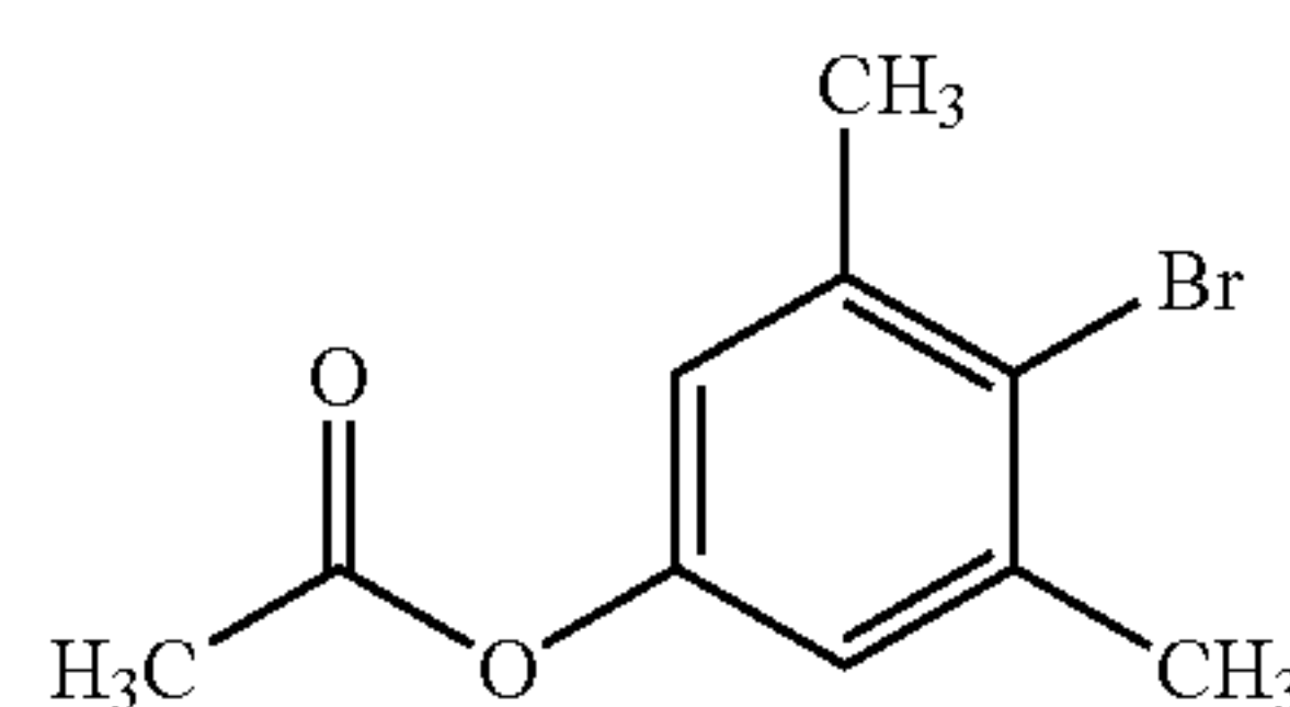
4-bromo-3,5-dimethylphenyl acetate
