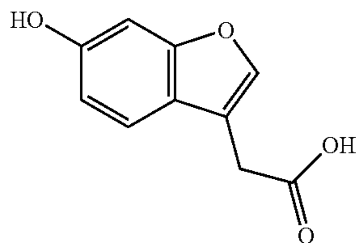
(6-hydroxy-1-benzofuran-3-yl)acetic acid
