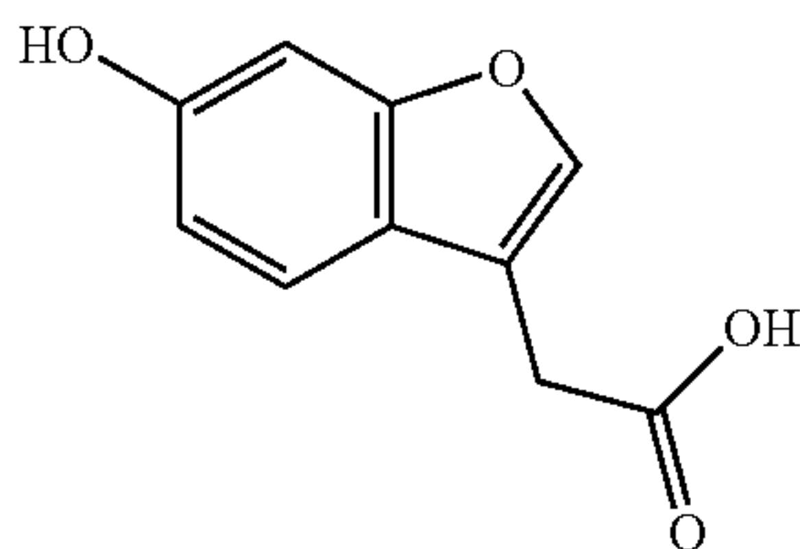
(6-hydroxy-1-benzofuran-3-yl)acetic acid
