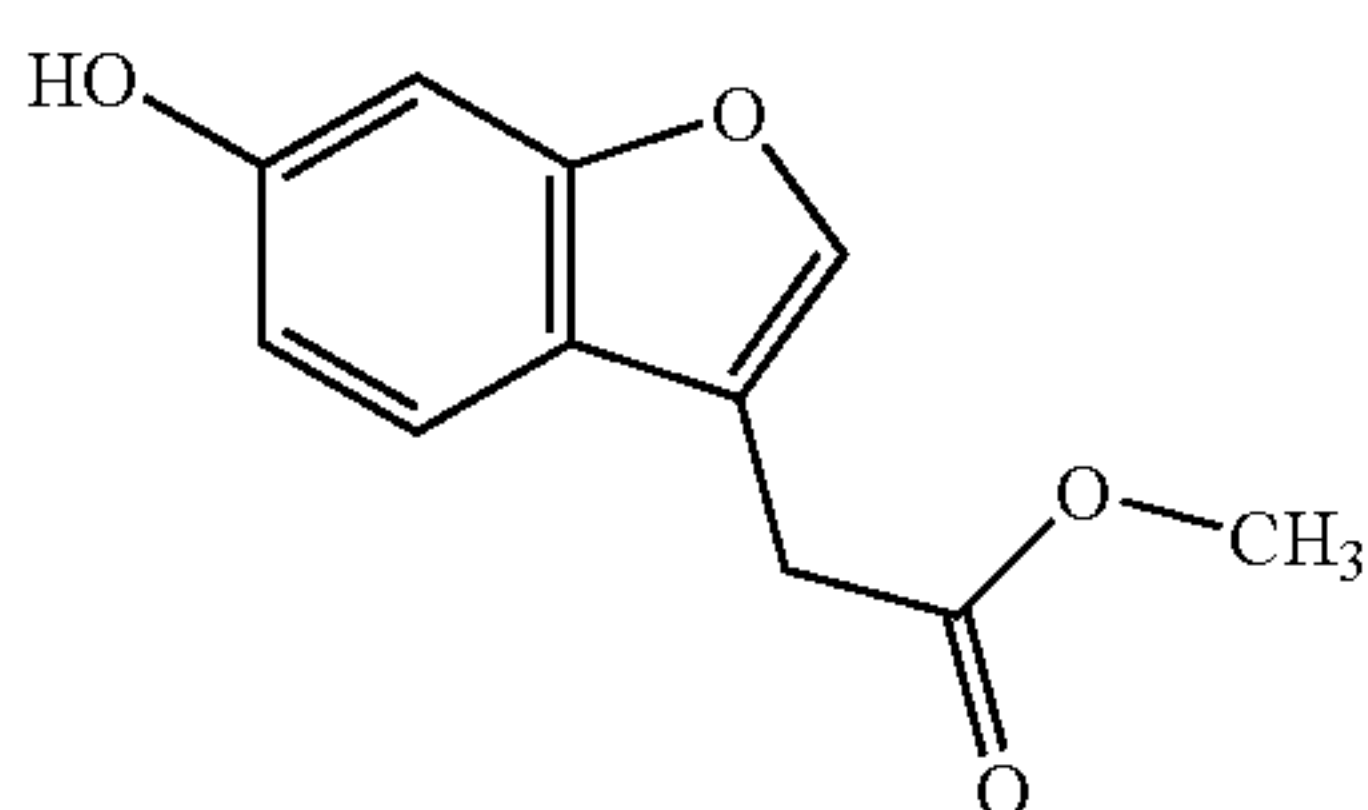
Methyl(6-hydroxy-2,3-dihydro-1-benzofuran-3-yl)acetate
