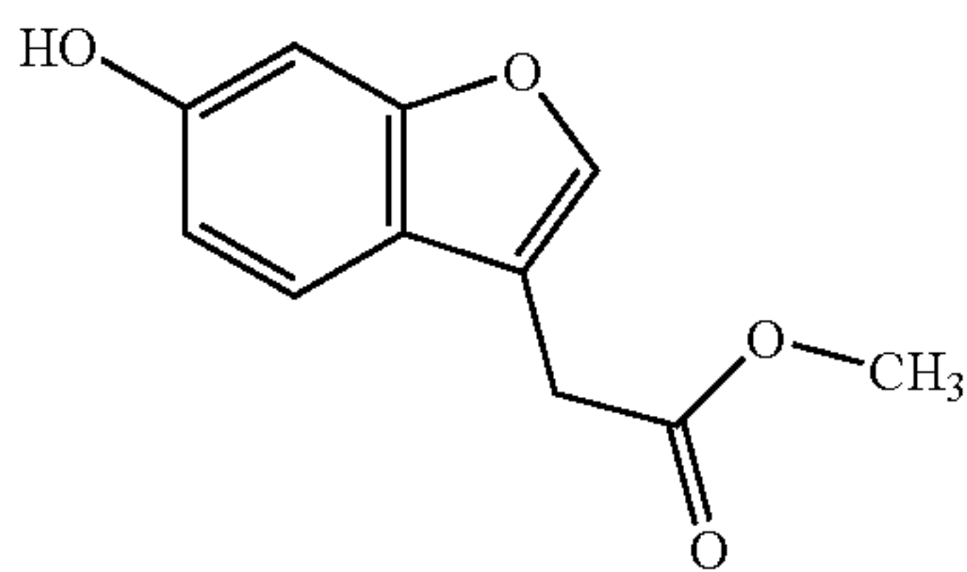
Methyl(6-hydroxy-1-benzofuran-3-yl)acetate
