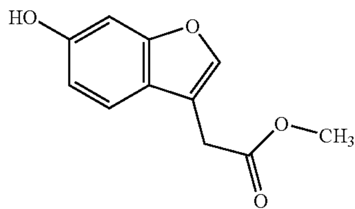
Methyl(6-hydroxy-1-benzofuran-3-yl)acetate
