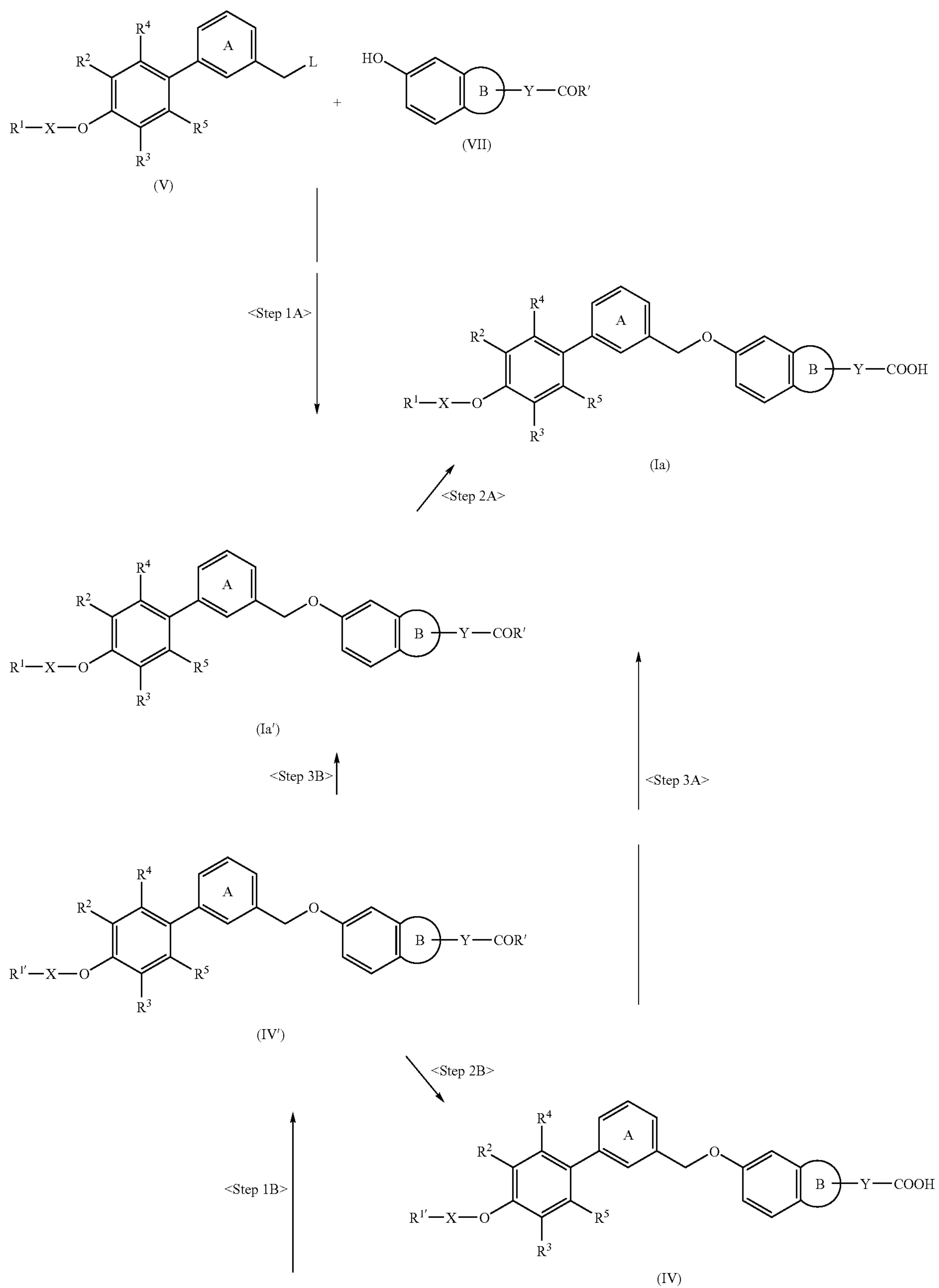
Scheme 1
