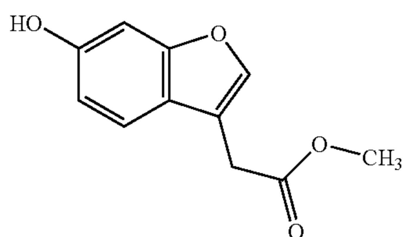
Methyl(6-hydroxy-2,3-dihydro-1-benzofuran-3-yl)acetate
