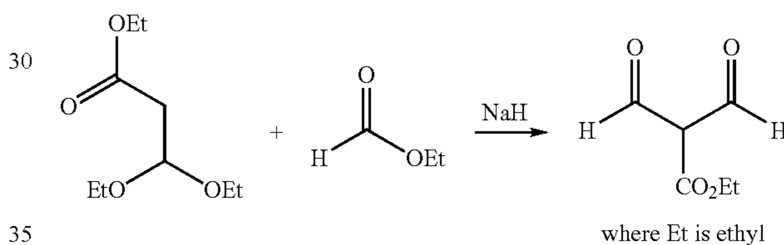
REACTION SCHEME II
