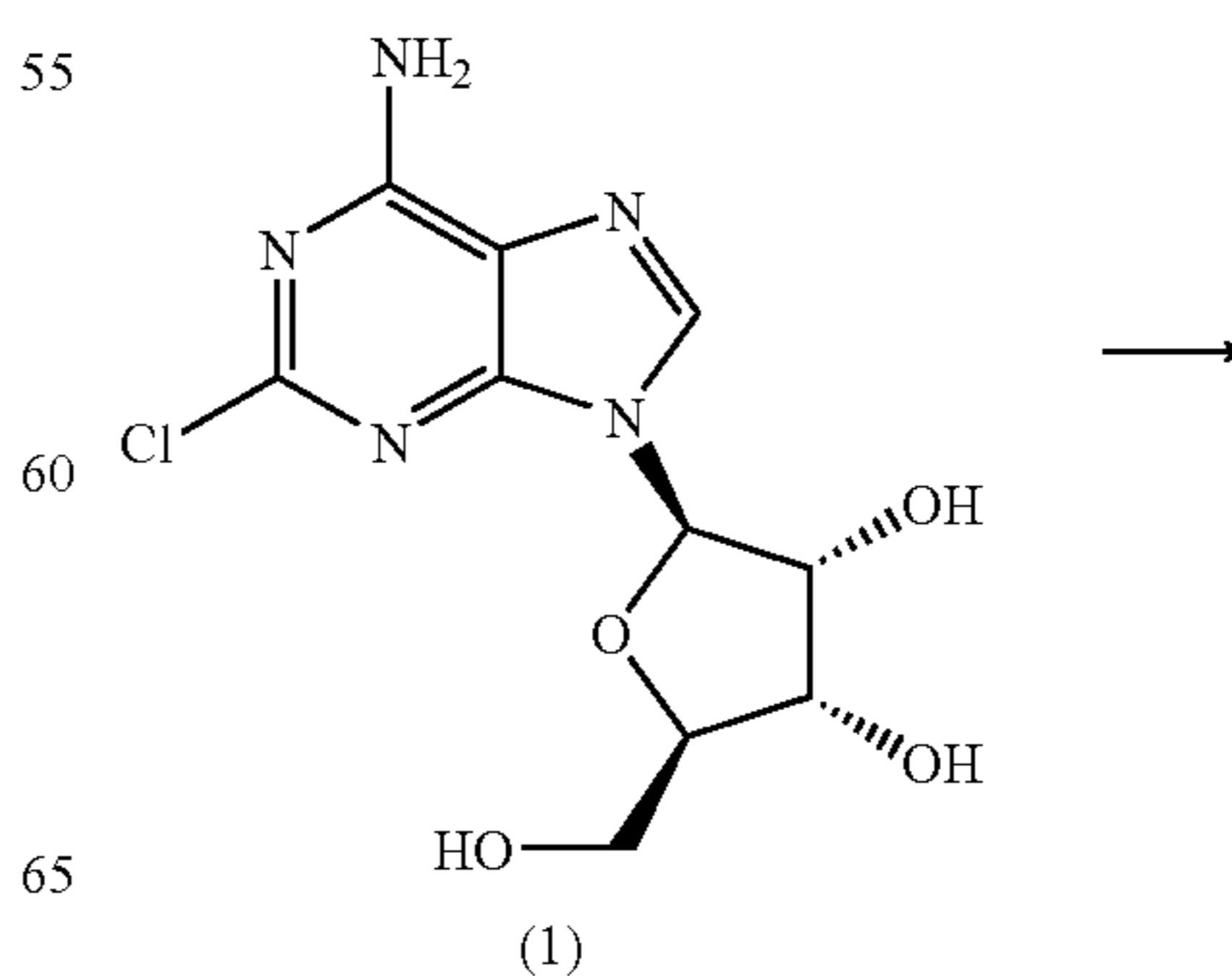
REACTION SCHEME III
