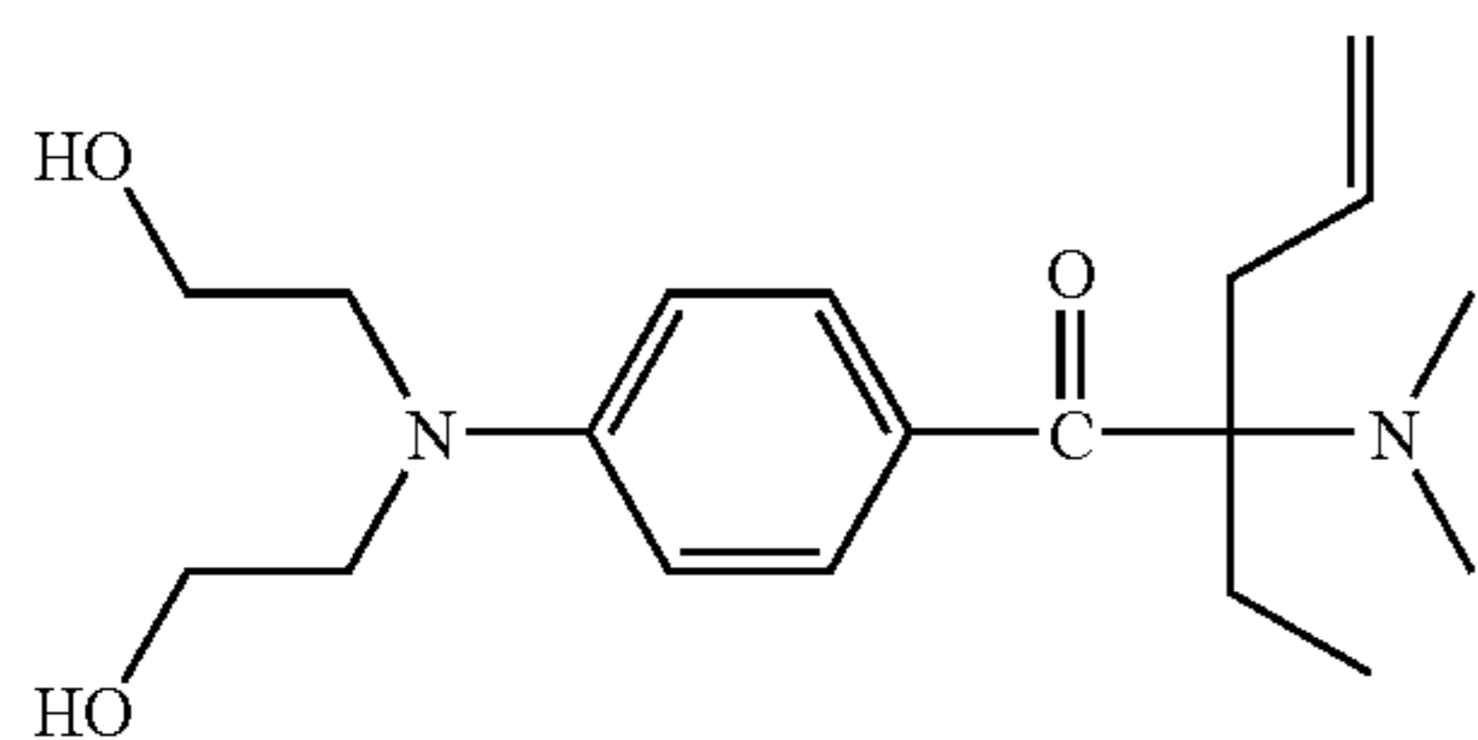
2-dimethylamino-1-[4-[bis(2-hydroxyethyl)amino]phenyl]-2-ethyl-1-pent-4-en-1-one
