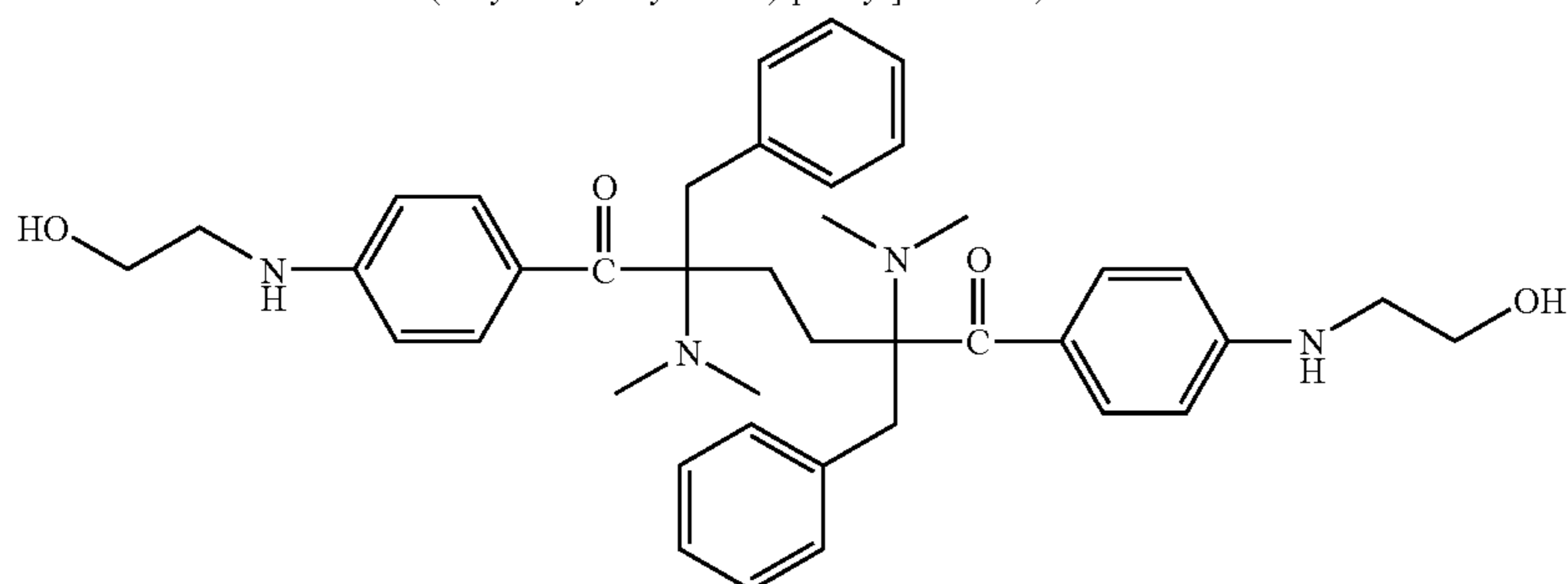
2,5-dibenzyl-2,5-bis-dimethylamino-1,6-bis-[4-(2-hydroxy-ethylamino)-phenyl]-hexan-1,6-dione
