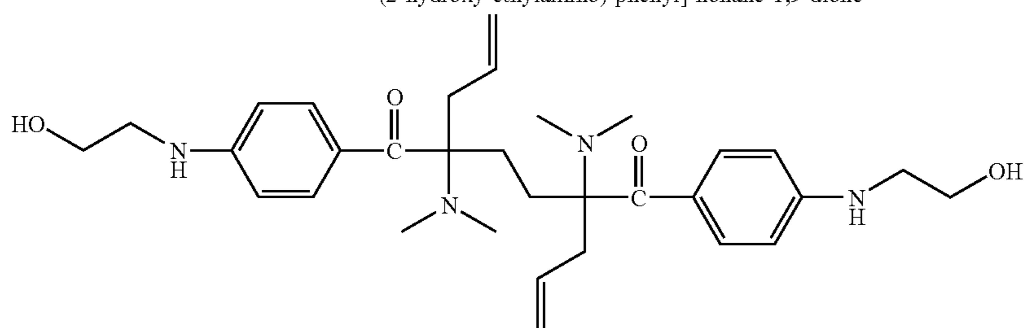
2,5-diallyl-2,5-bis-dimethylamino-1,6-bis-[4-(2-hydroxy-ethylamino)-phenyl]-hexan-1,6-dione
