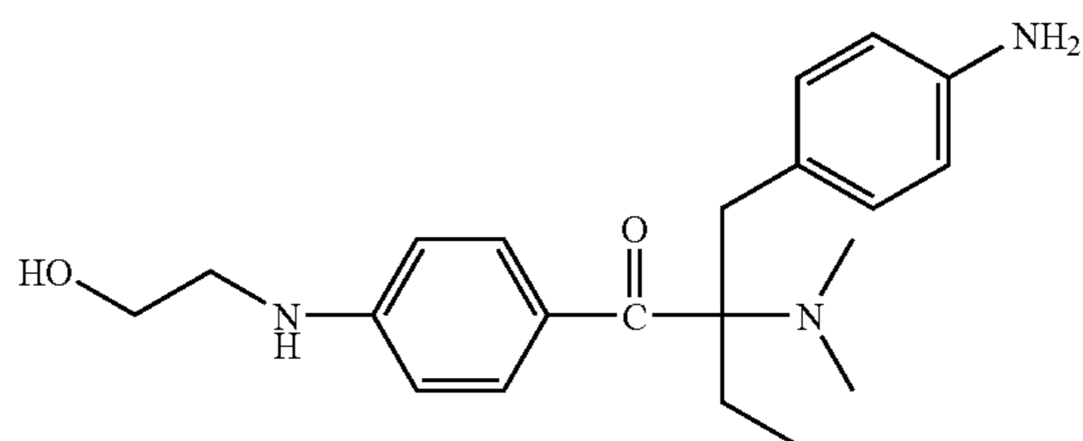
2-[(4-aminophenyl)methyl]-1-[4-(2-hydroxyethylamino)phenyl]-2-dimethylamino-1-butanone
