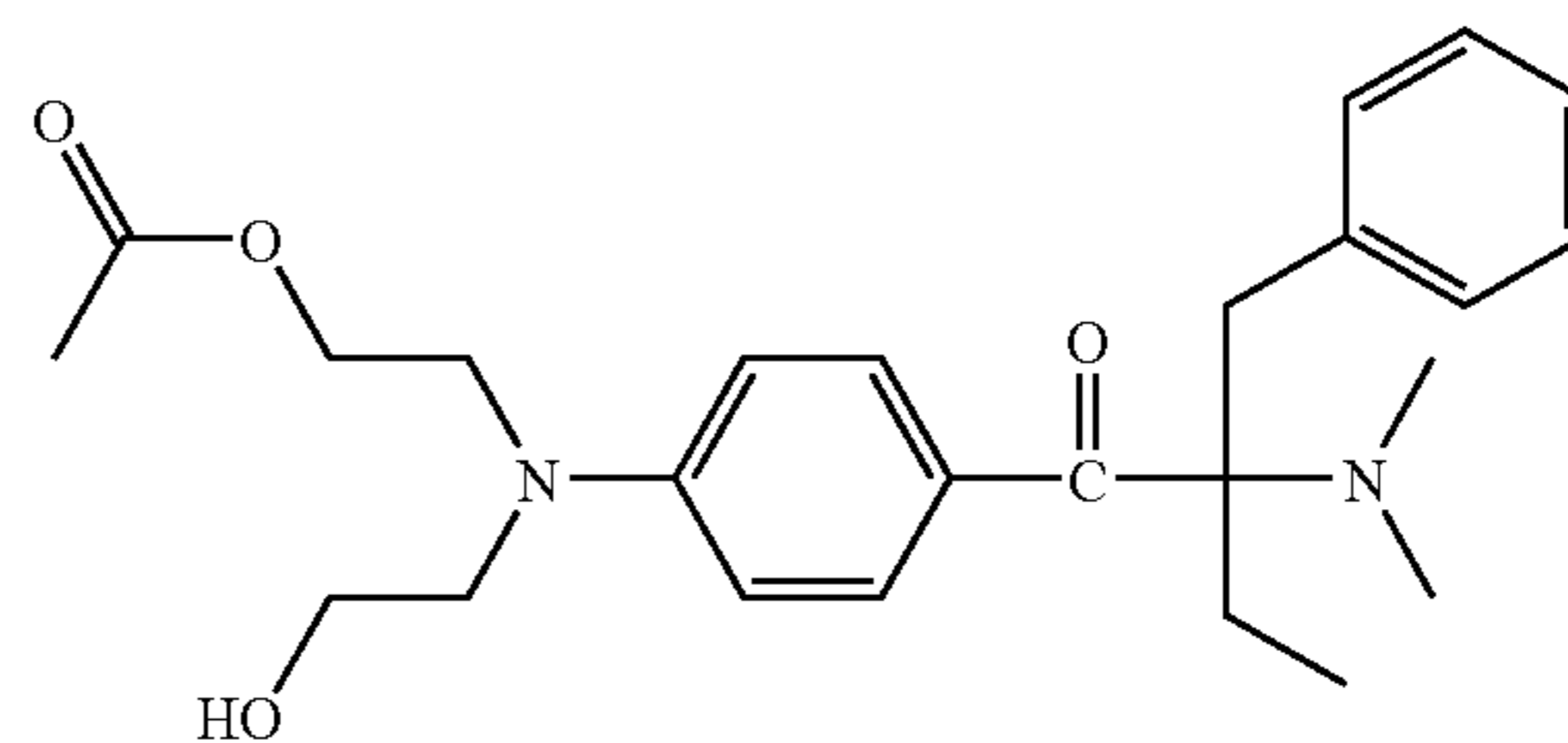
2-benzyl-2-dimethylamino-1-[4-(2-acetoxyethyl-2-hydroxyethyl-amino)phenyl]-1-butanone
