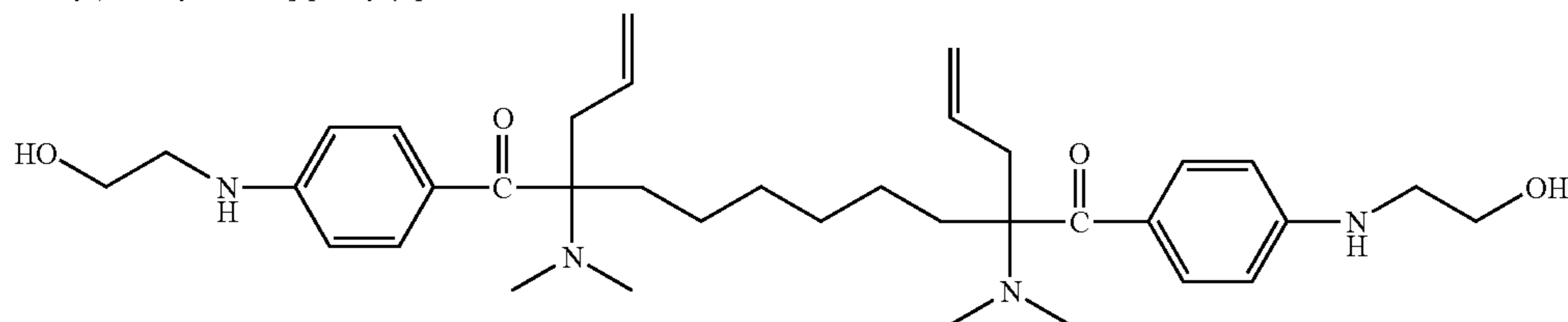
2,8-diallyl-2,8-bis-dimethylamino-1,9-bis-[4-(2-hydroxy-ethylamino)-phenyl]-nonane-1,9-dione
