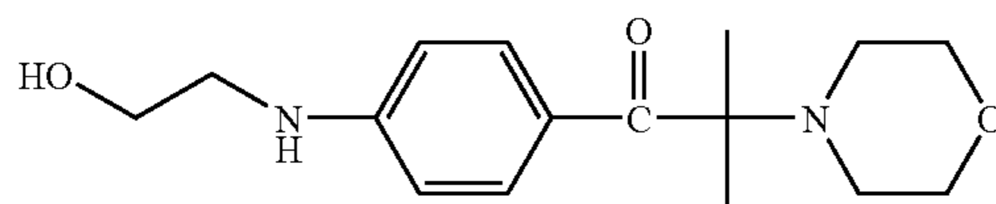
1-[4-(2-hydroxyethylamino)phenyl]-2-methyl-2-(morpholin-4-yl)-1-propanone
