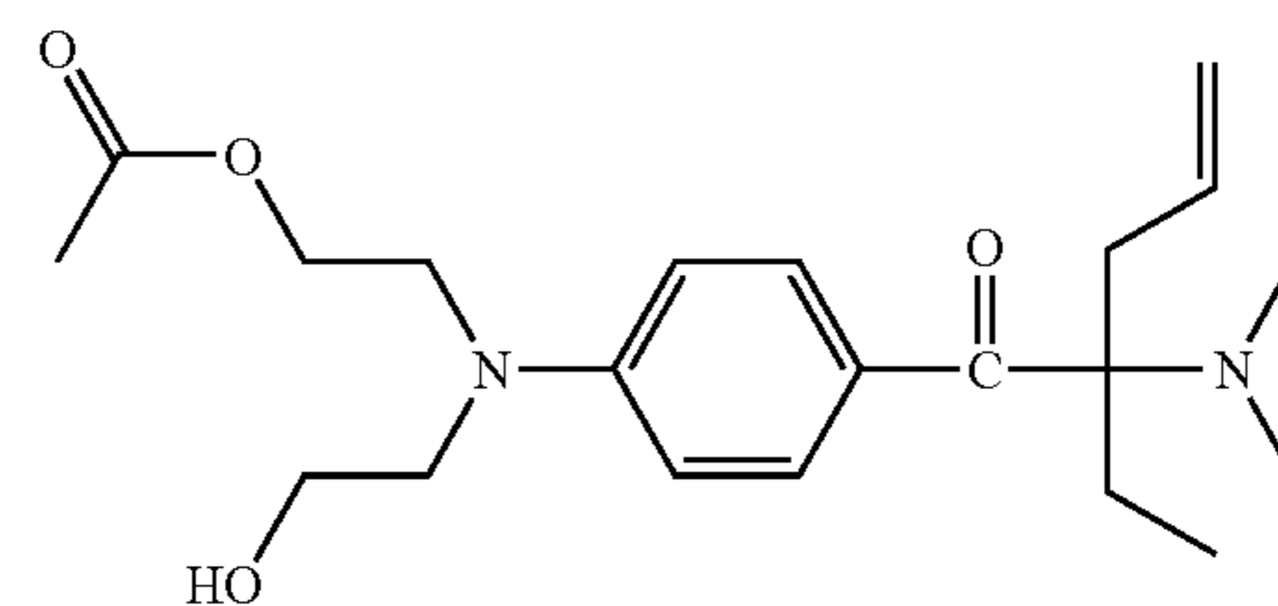
2-dimethylamino-1-[4-(2-acetoxyethyl-2-hydroxyethyl-amino)phenyl]-2-ethyl-1-pent-4-en-1-one
