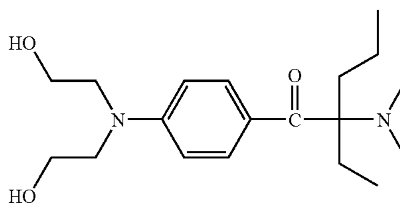
2-dimethylamino-1-[4-[bis(2-hydroxyethyl)amino]phenyl]-2-ethyl-1-pentan-1-one
