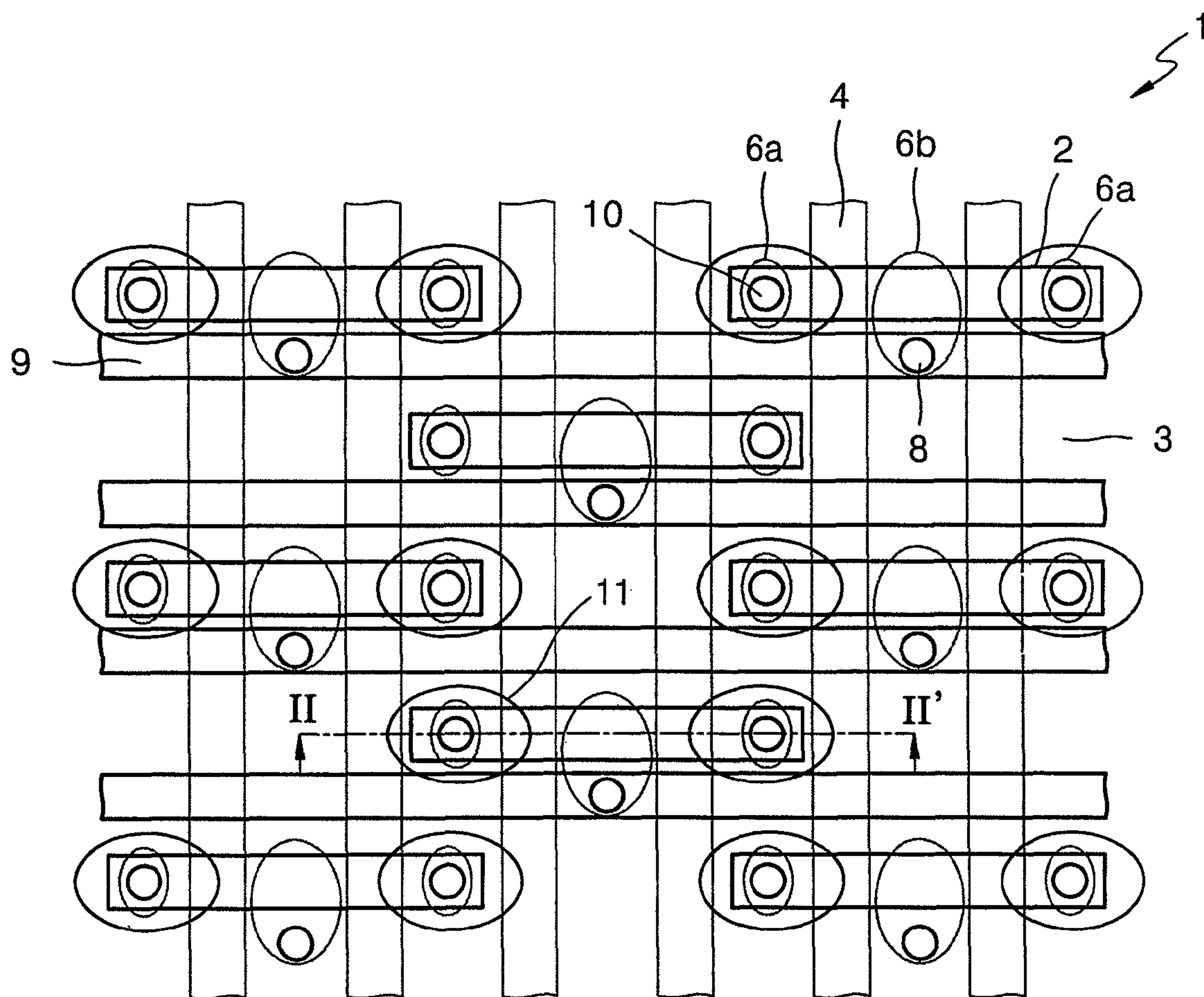
FIG. 1 (PRIOR ART)
