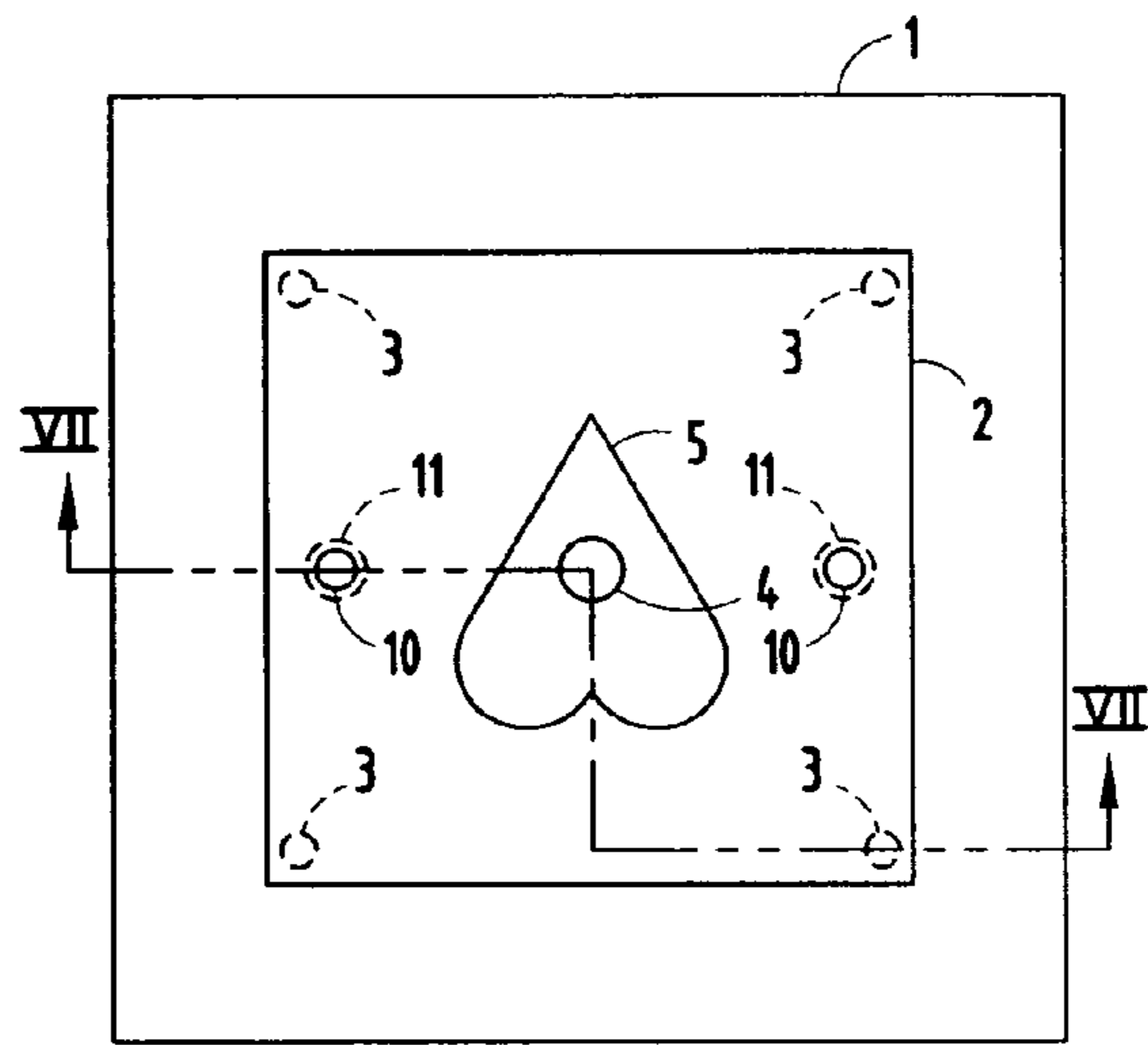
FIG. 6 PRIOR ART
