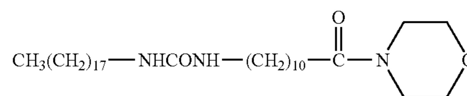
Structural Formula 5
