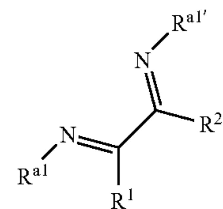
Structure 1f
