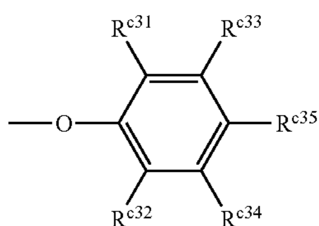
Structure 14c
