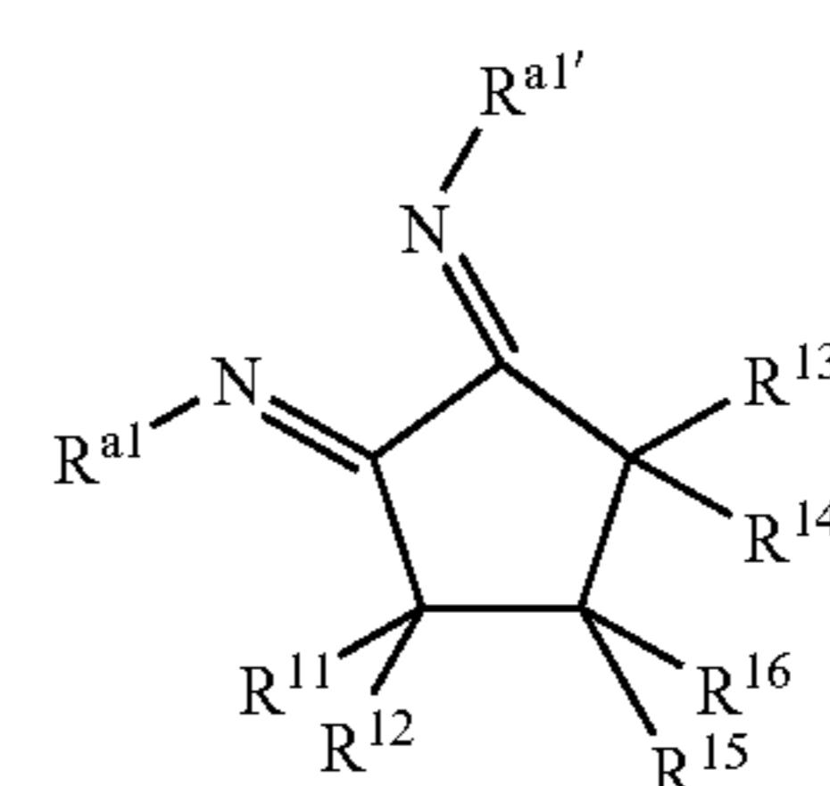
Structure 4f
