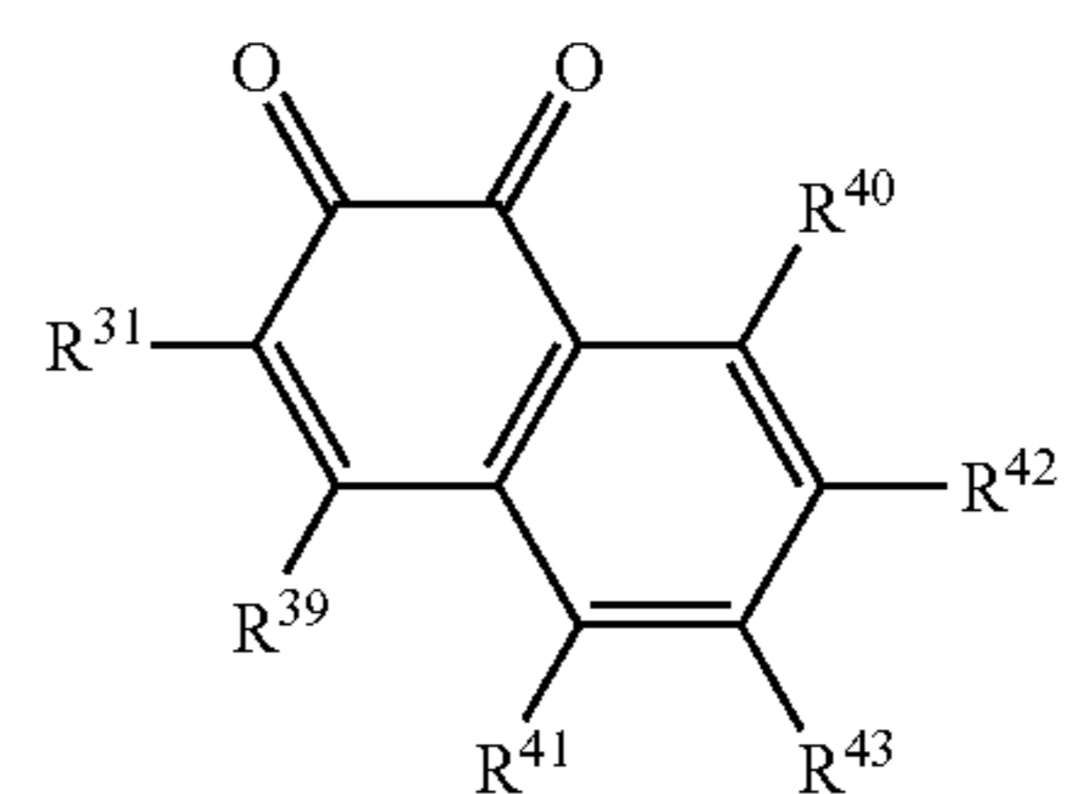
Structure 9
