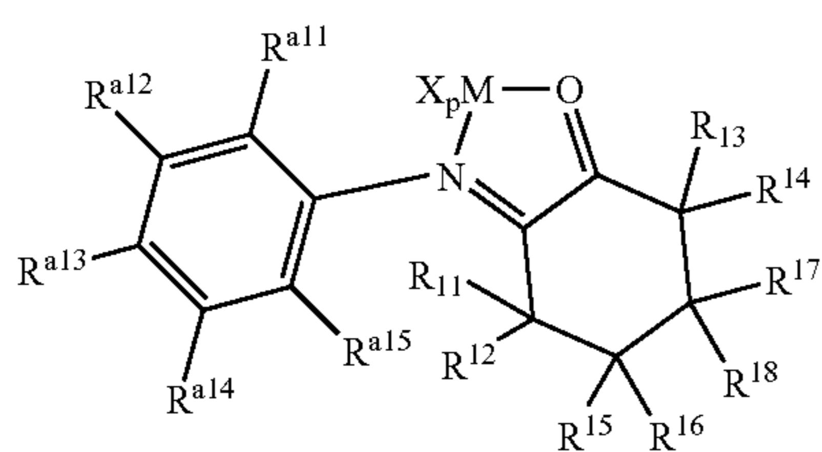
Structure 31d
