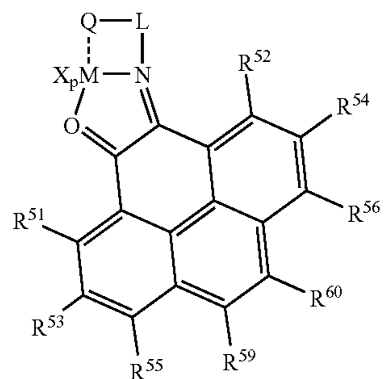
Structure 26d
