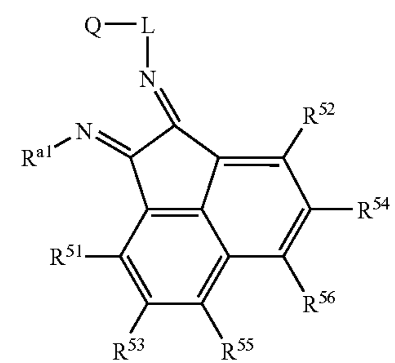
Structure 24f
