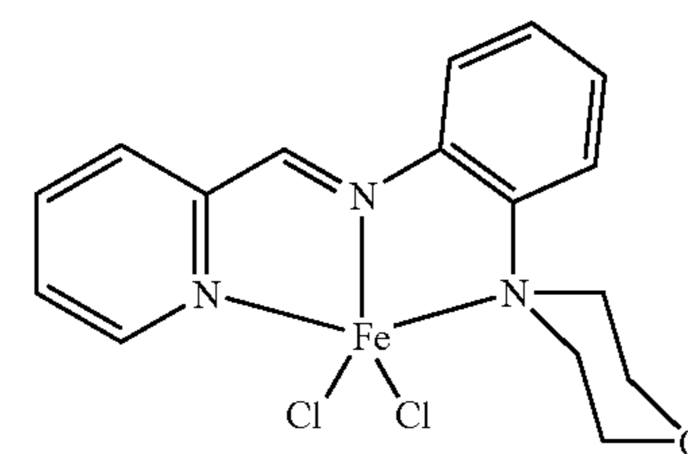
Structure XIX
