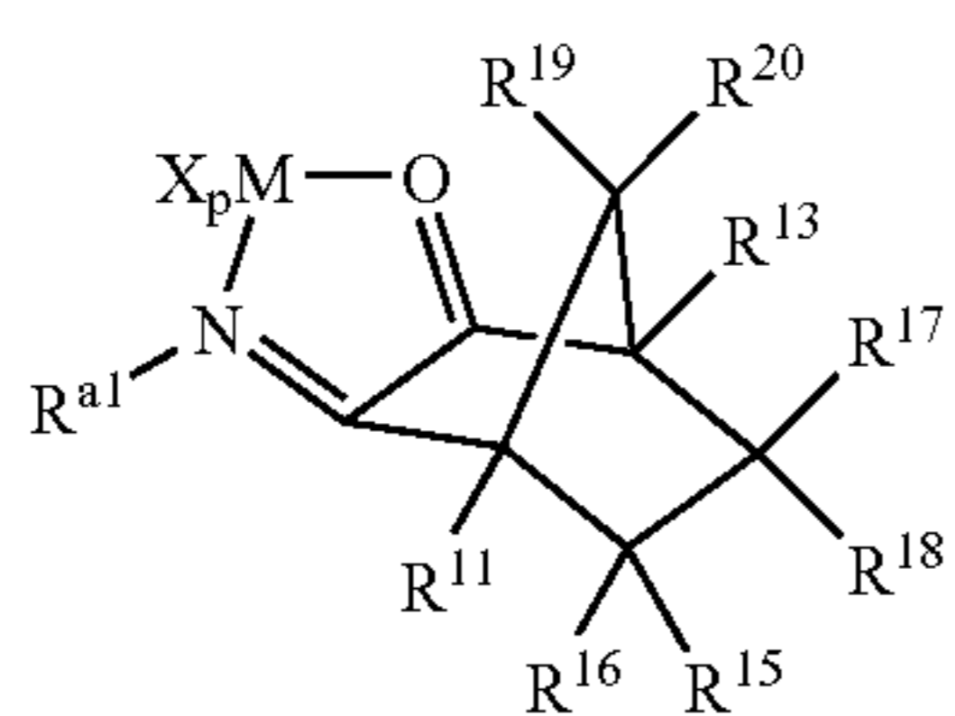
Structure 6d
