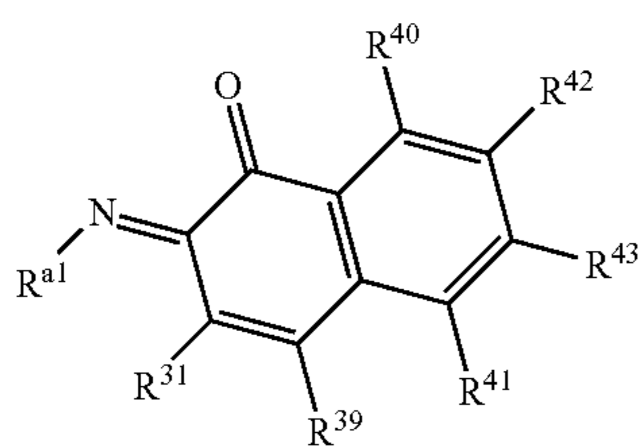
Structure 9b
