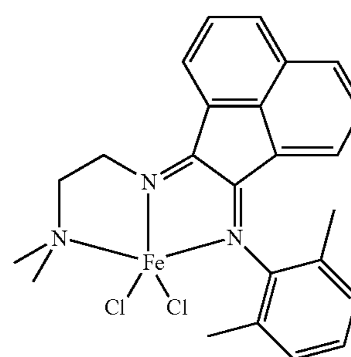
Structure XII
