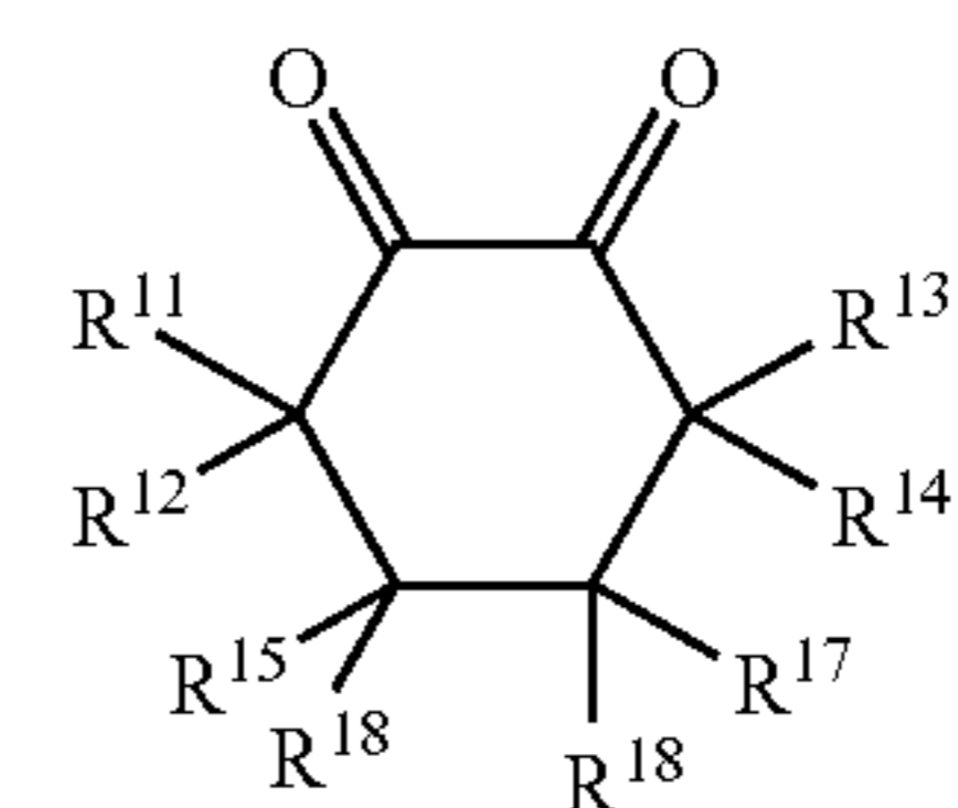
Structure 5
