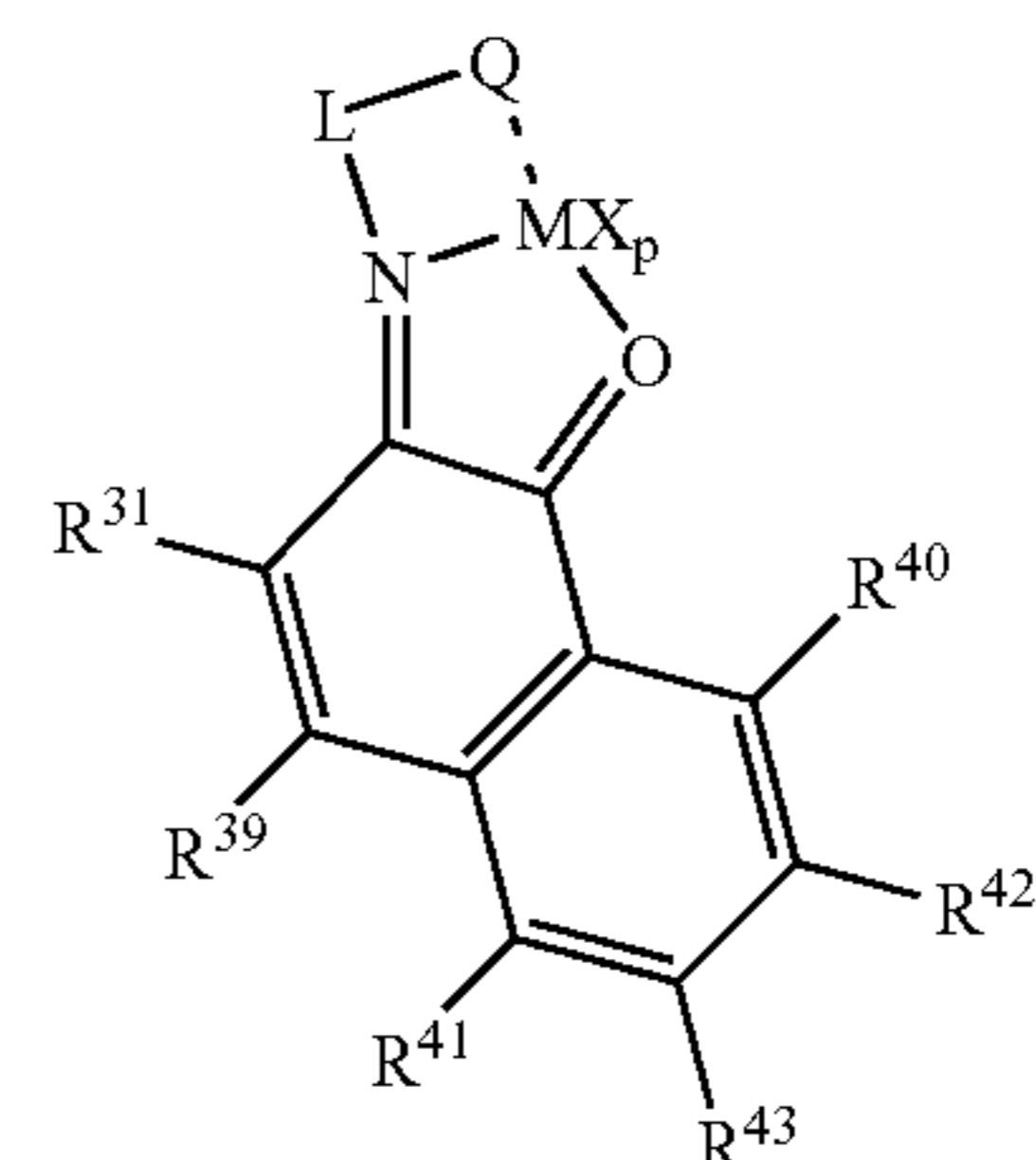
Structure 23d
