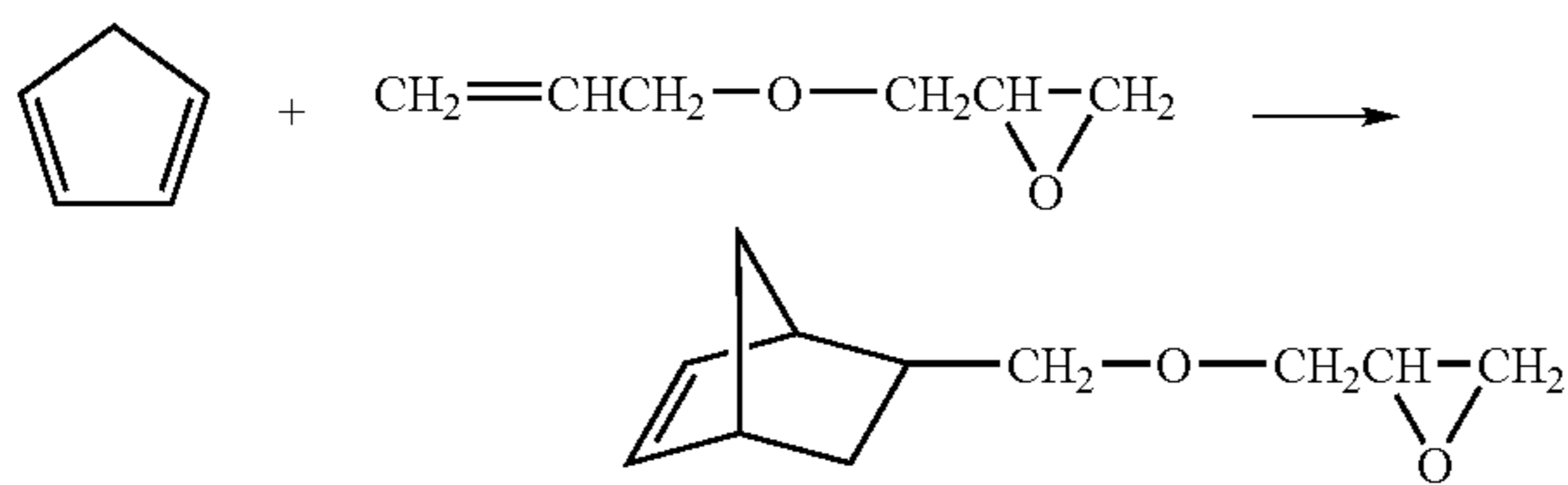
FIG. 1 was a scheme shown the process to prepare various cross-linked hybrid materials from norbornene compound with cross-linkable groups.
