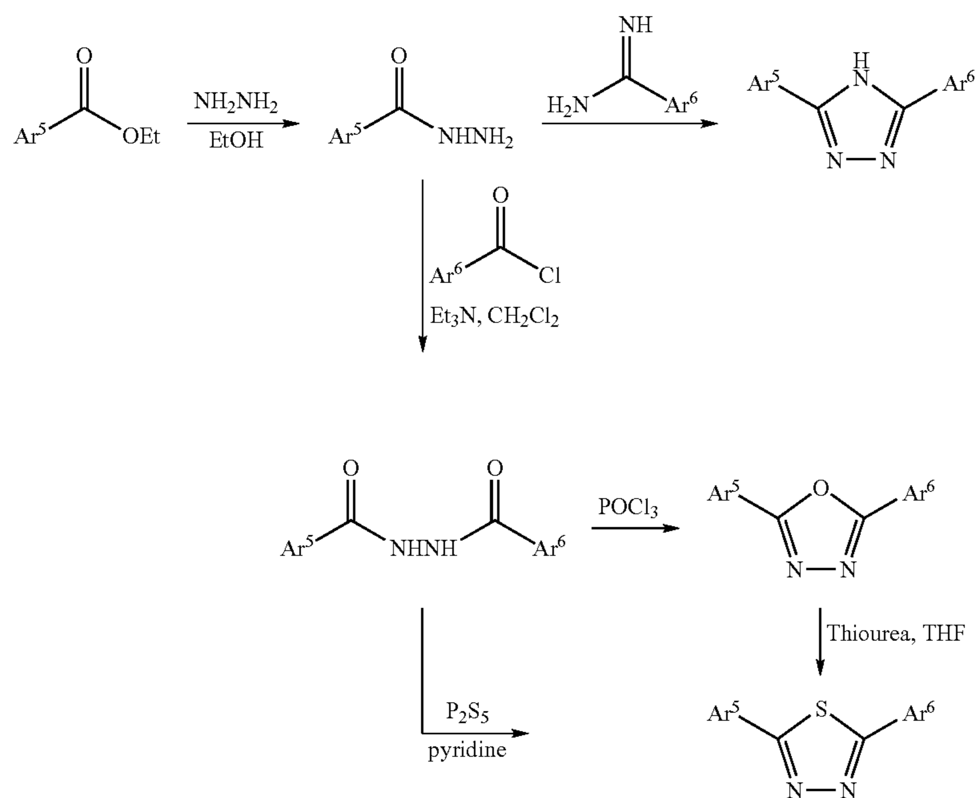
Reaction Scheme 3
