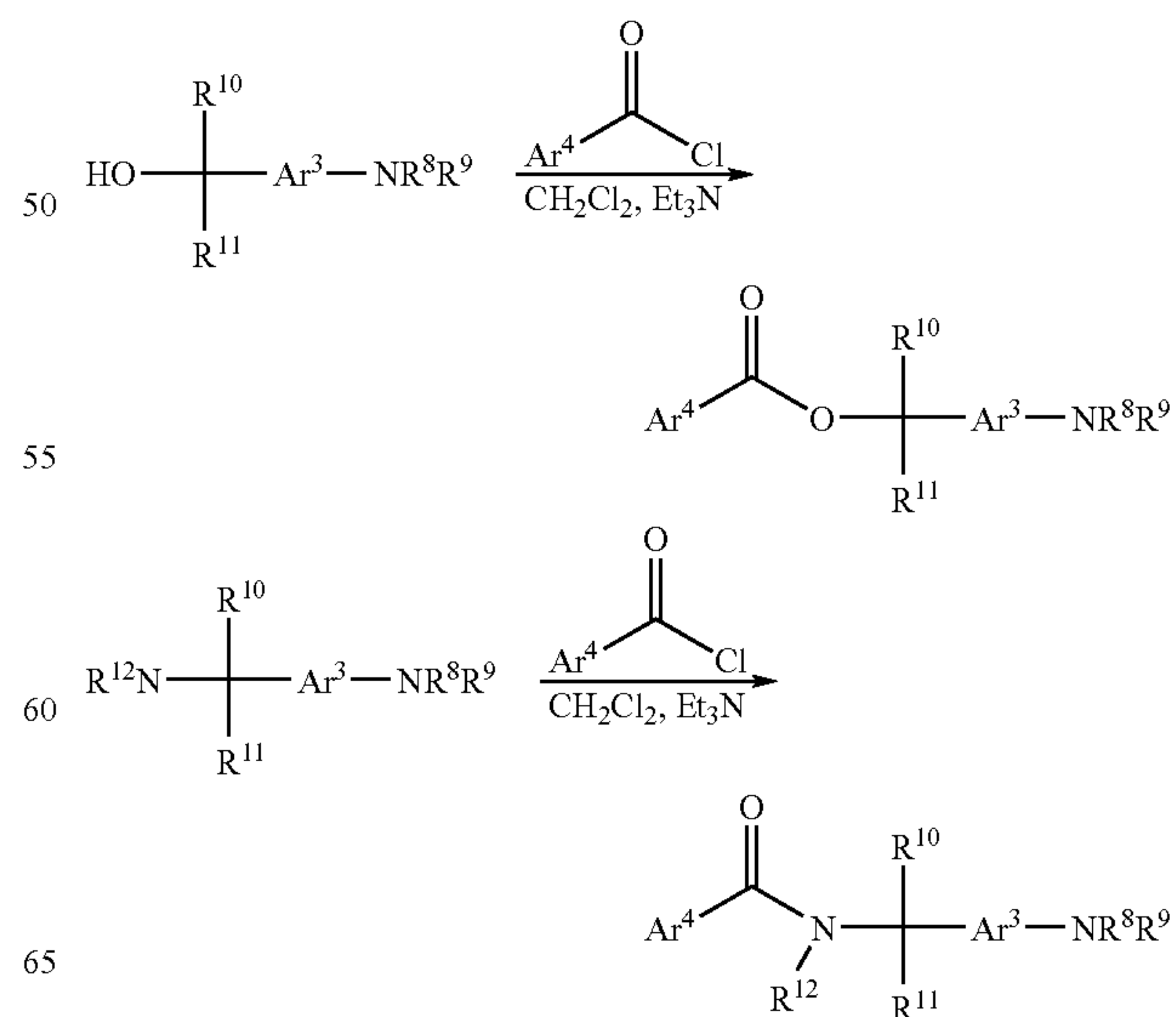
Reaction Scheme 2
