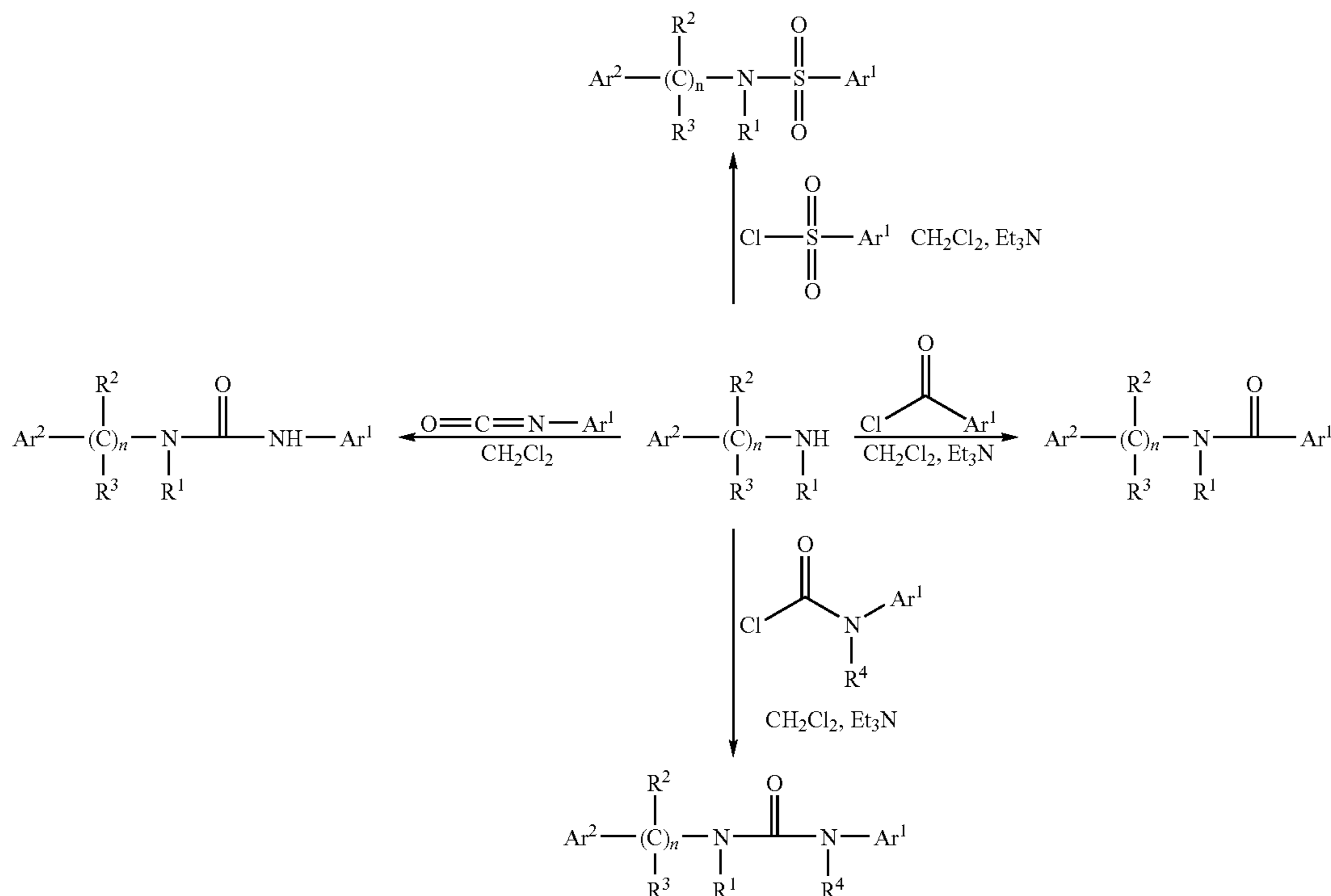
Reaction Scheme 1
