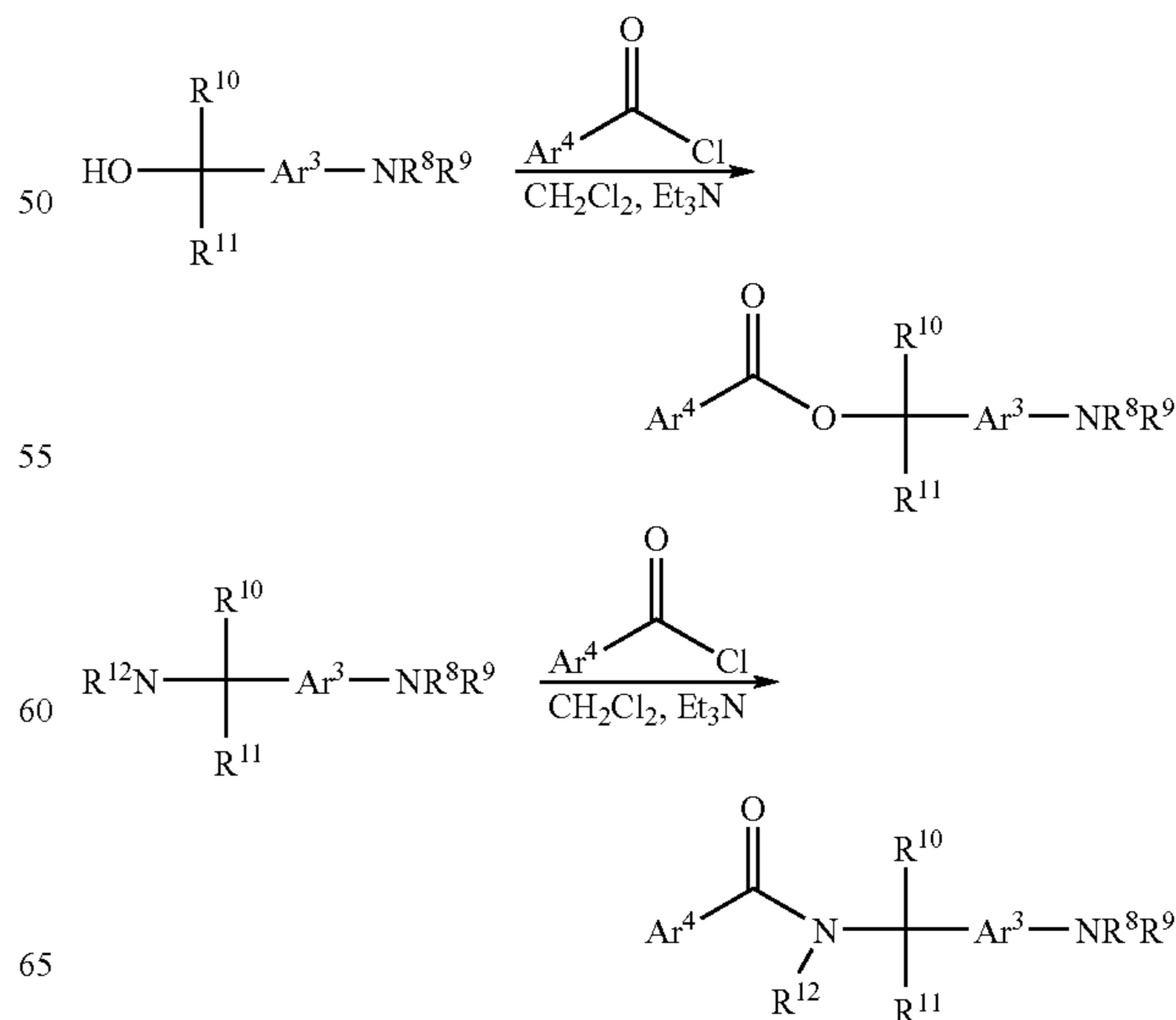
Reaction Scheme 2
