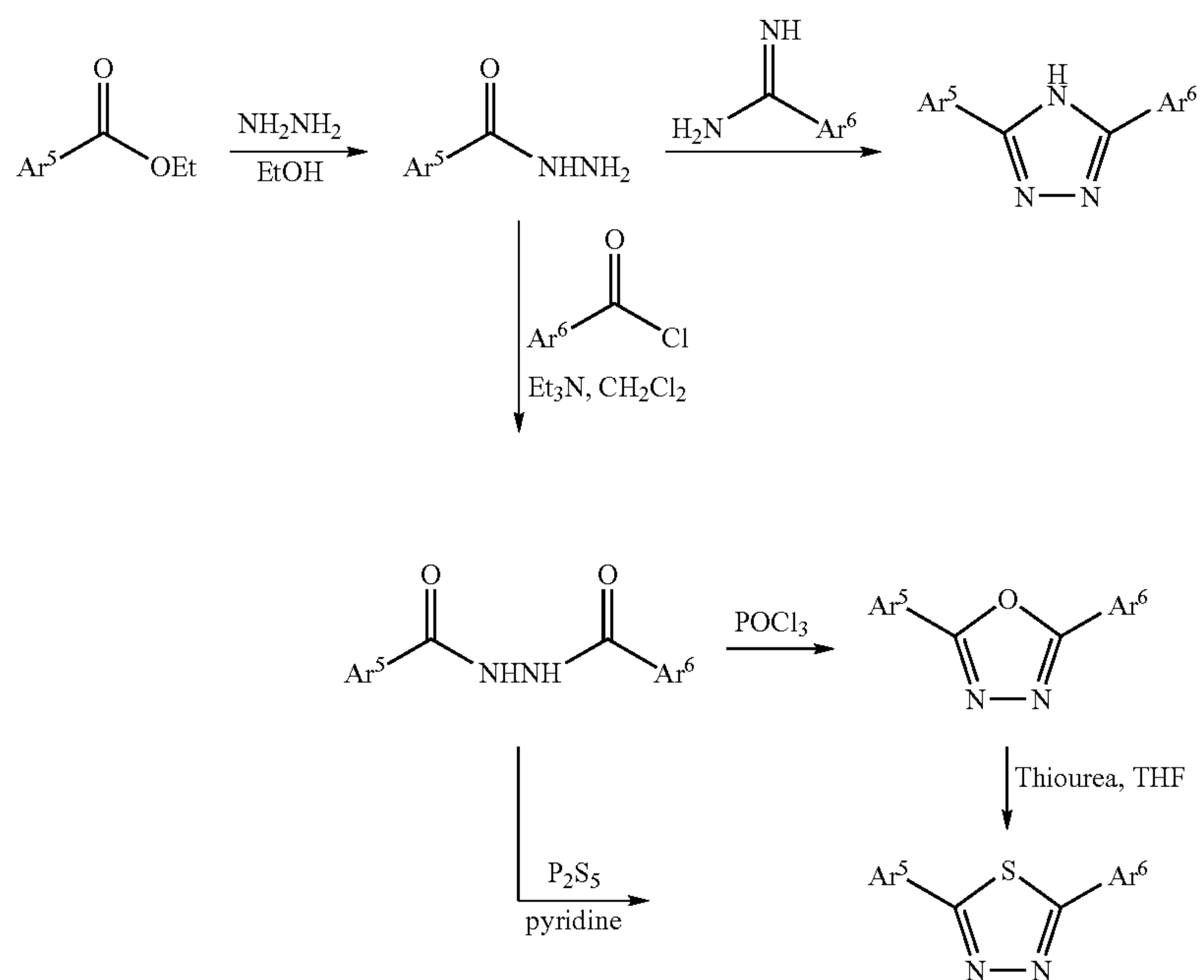
Reaction Scheme 3
