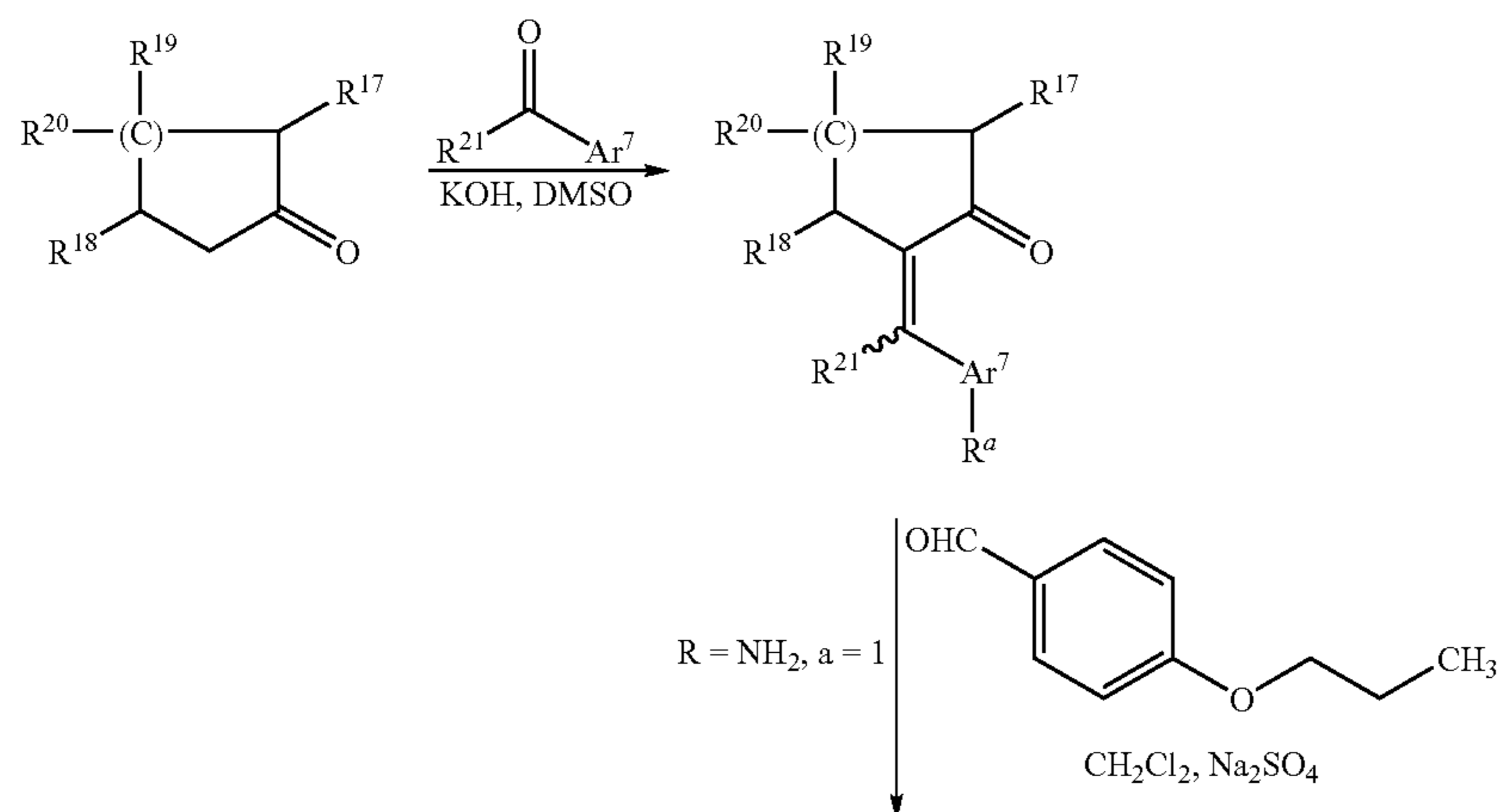
Reaction Scheme 4
