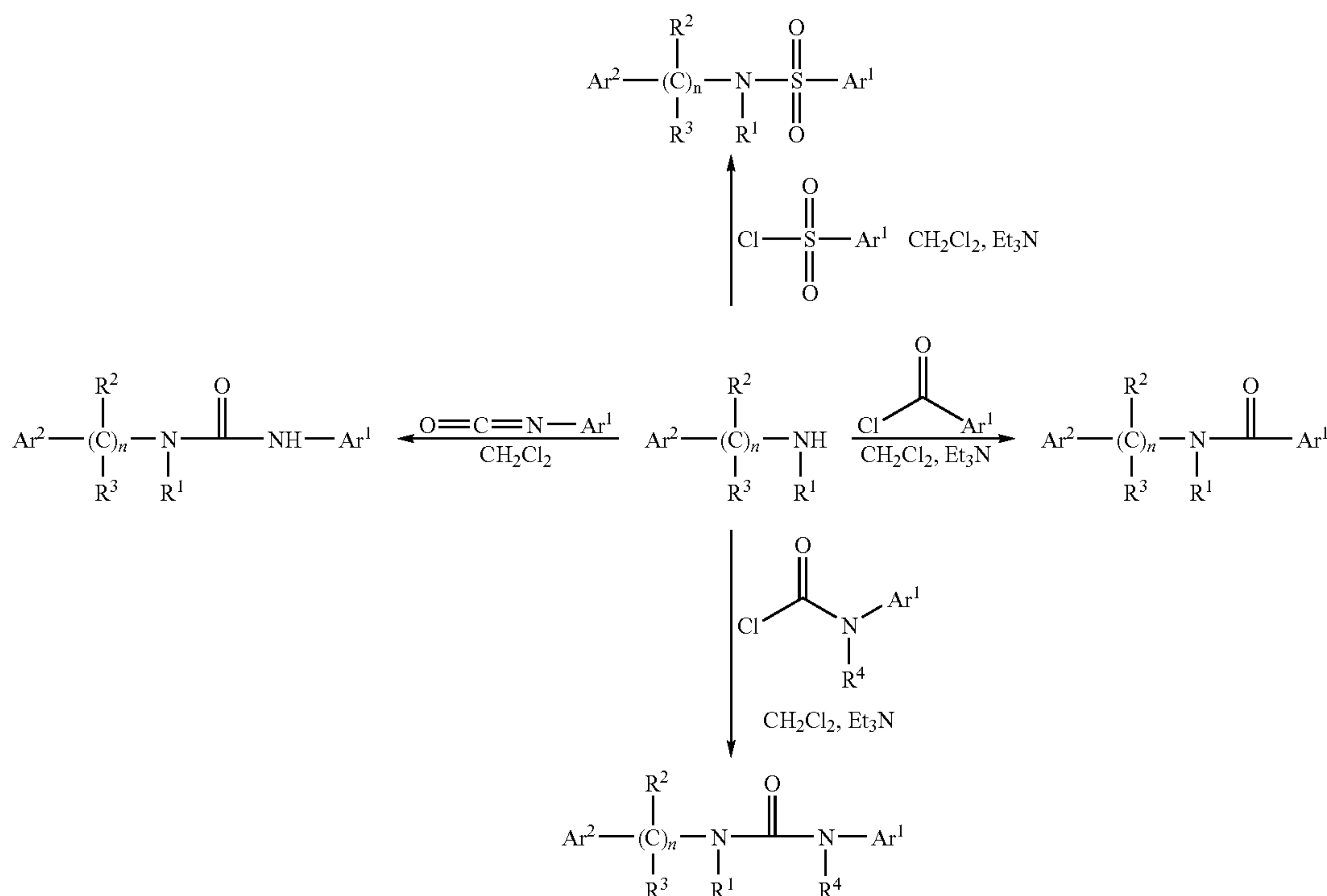
Reaction Scheme 1
