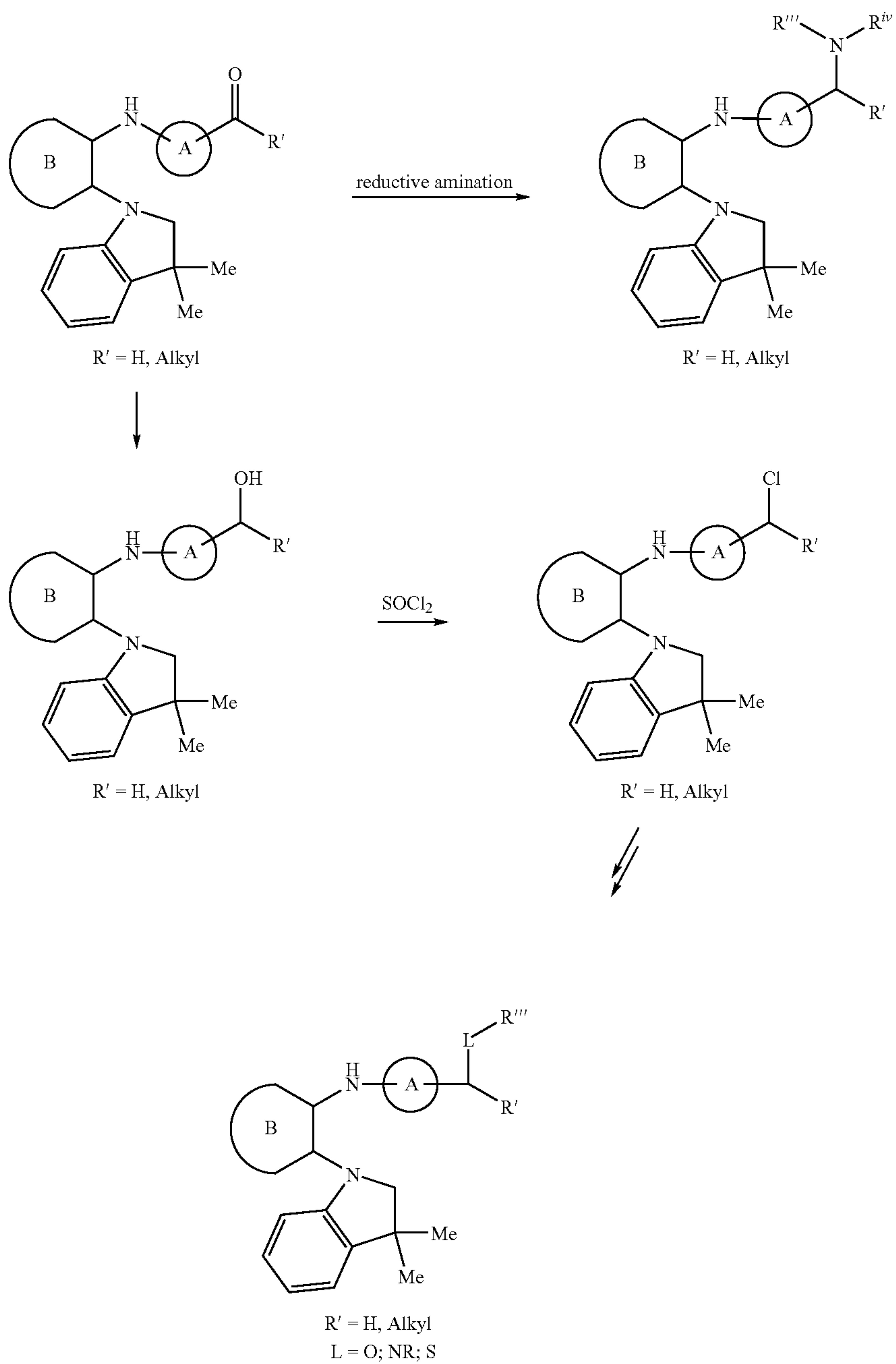
Scheme 24
