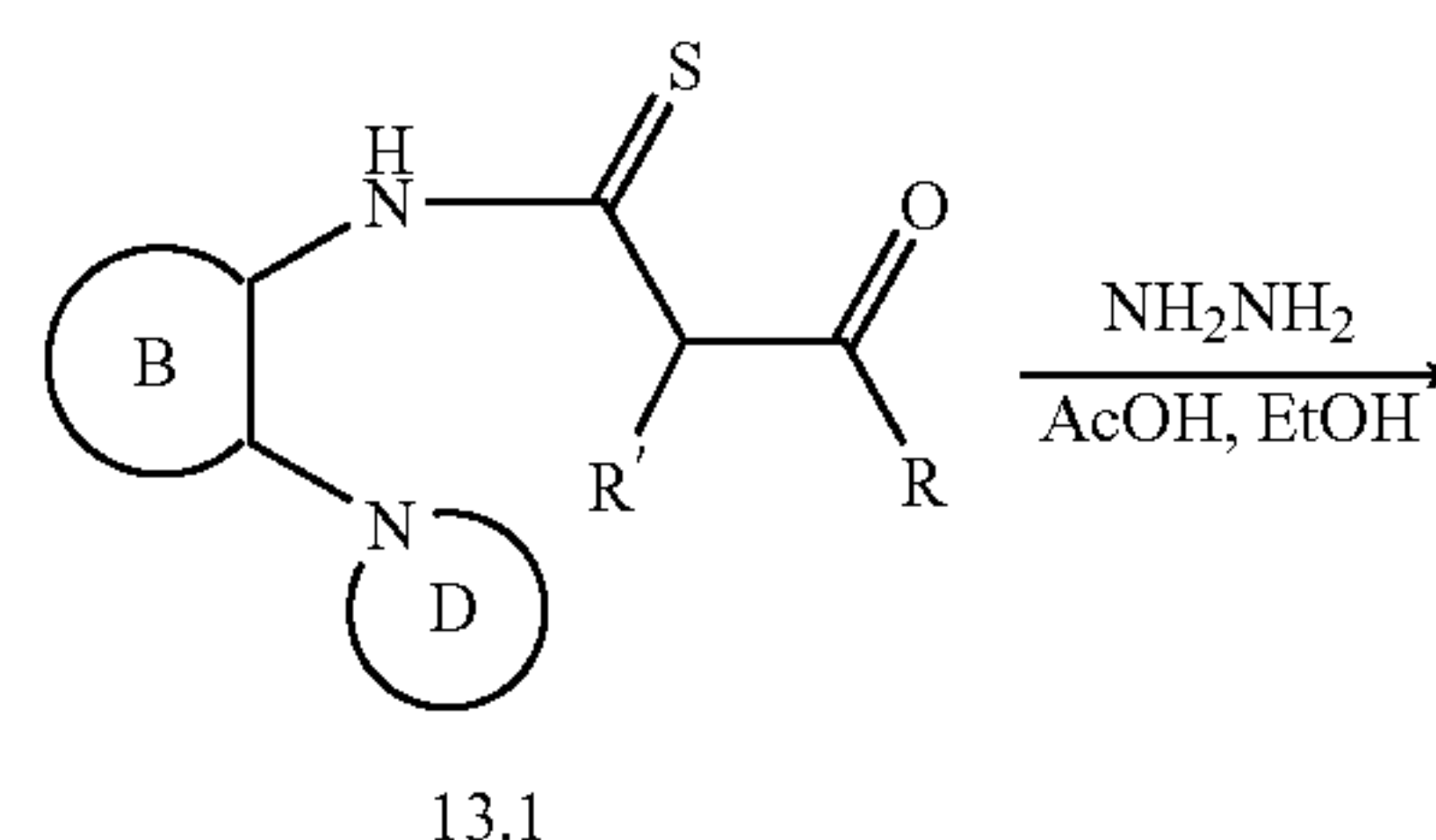
Scheme 13
