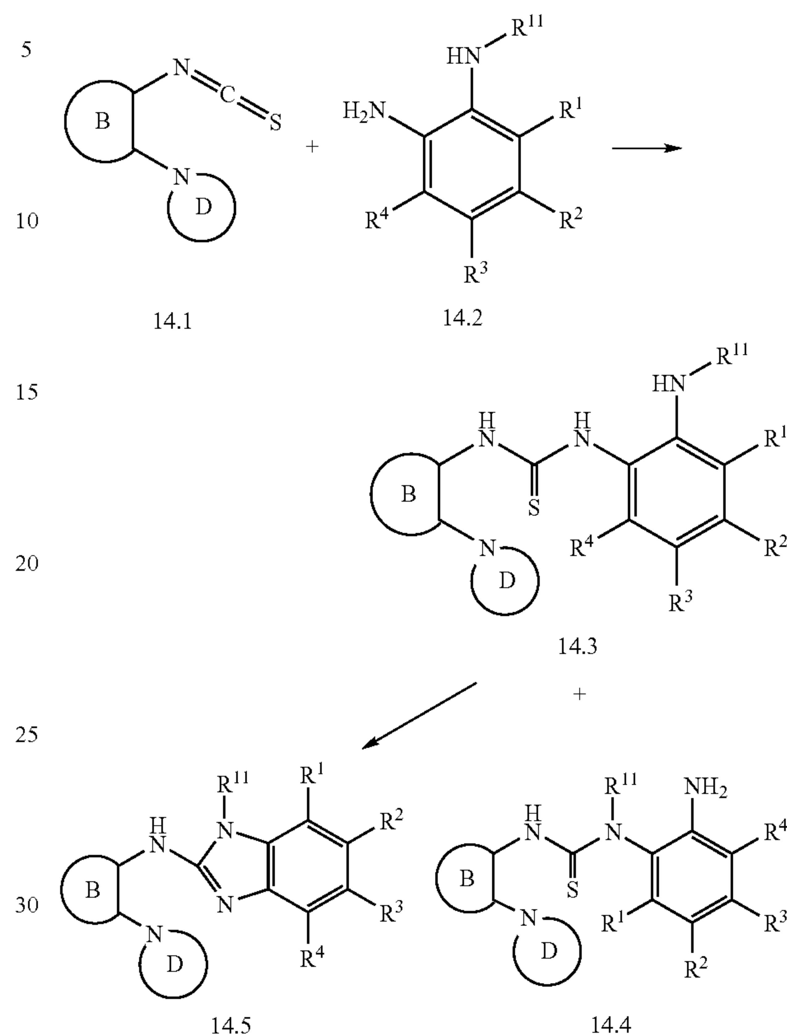
Scheme 14
