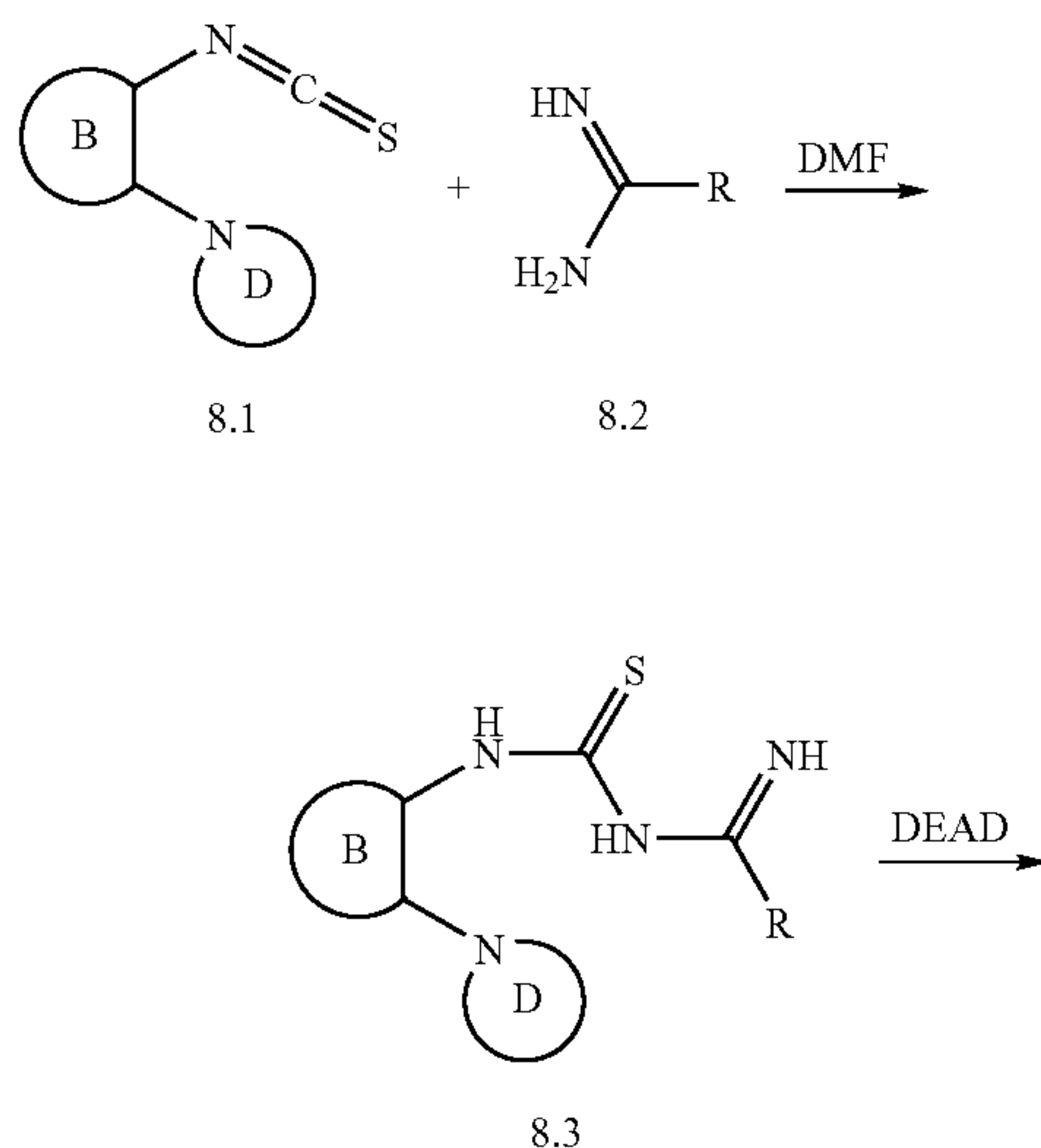
Scheme 8
