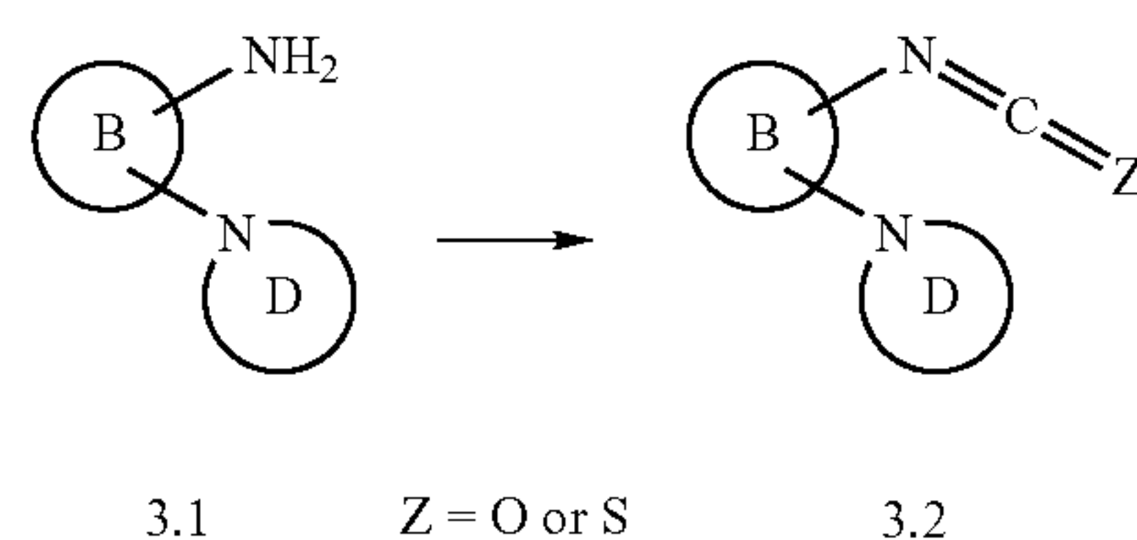
Scheme 3
