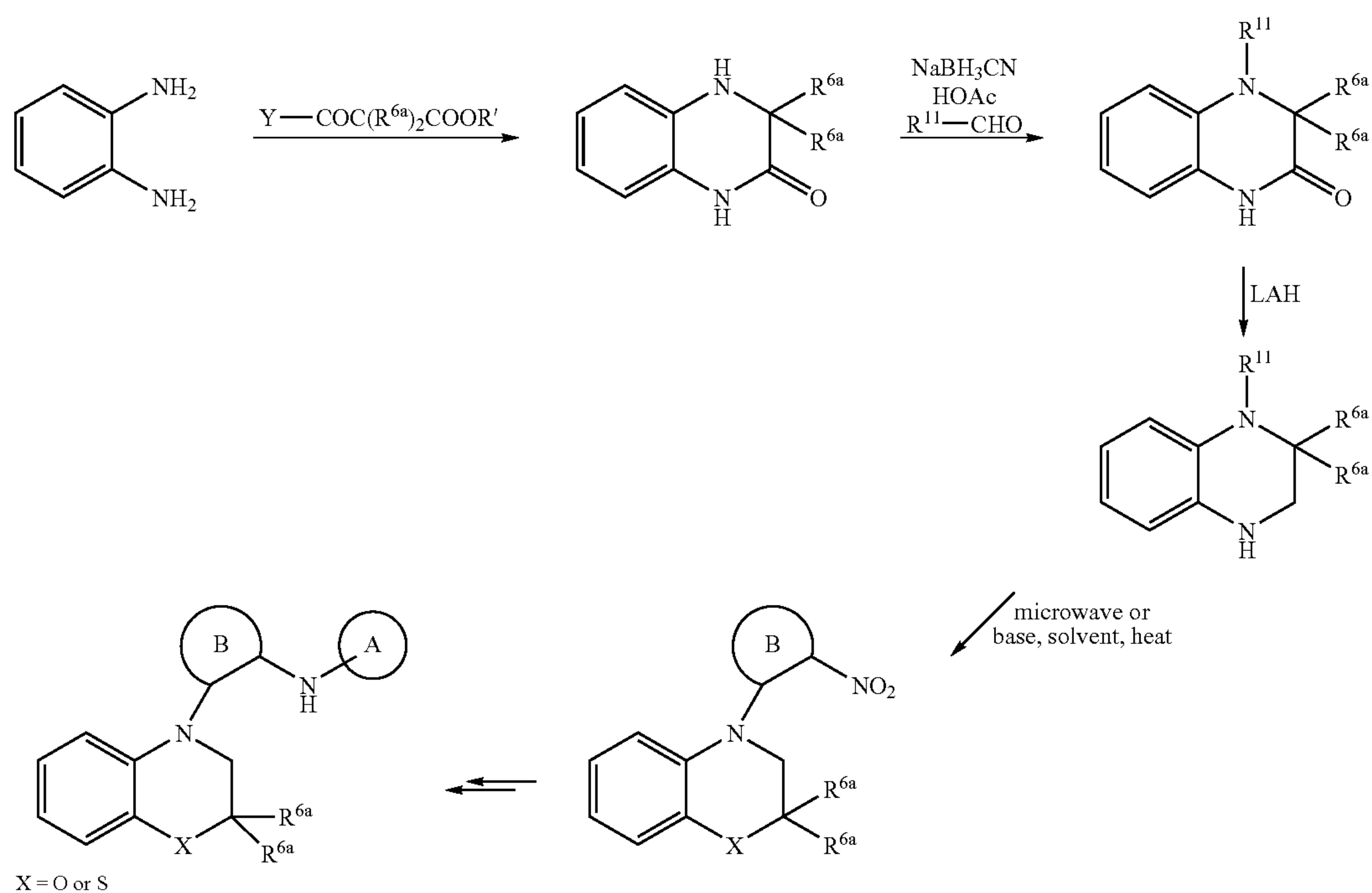
Scheme 27
