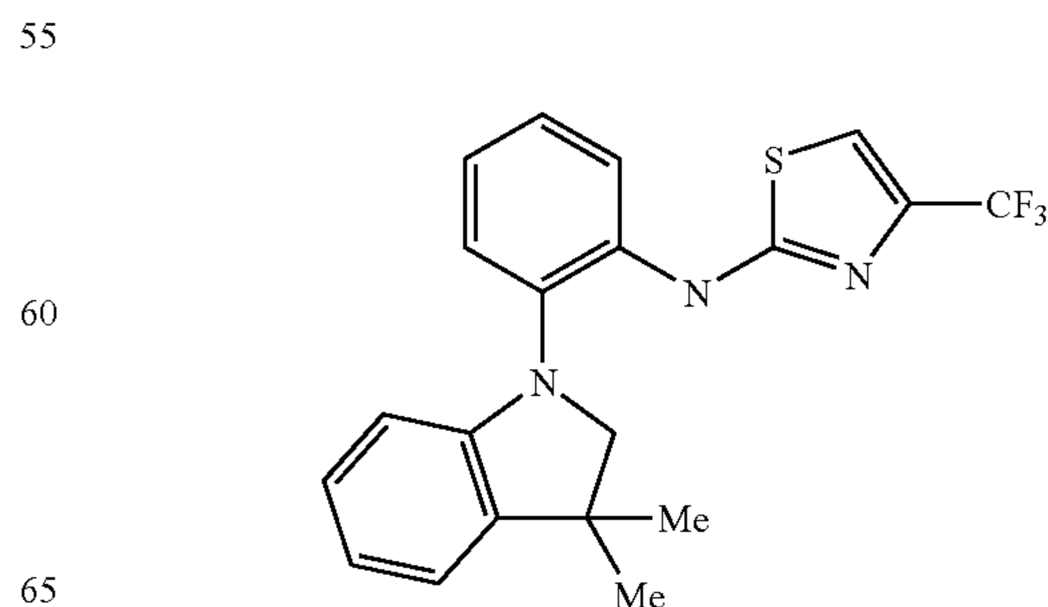
N-(2-(3,3-dimethylindolin-1-yl)phenyl)-4-(trifluoromethyl)thiazol-2-amine
