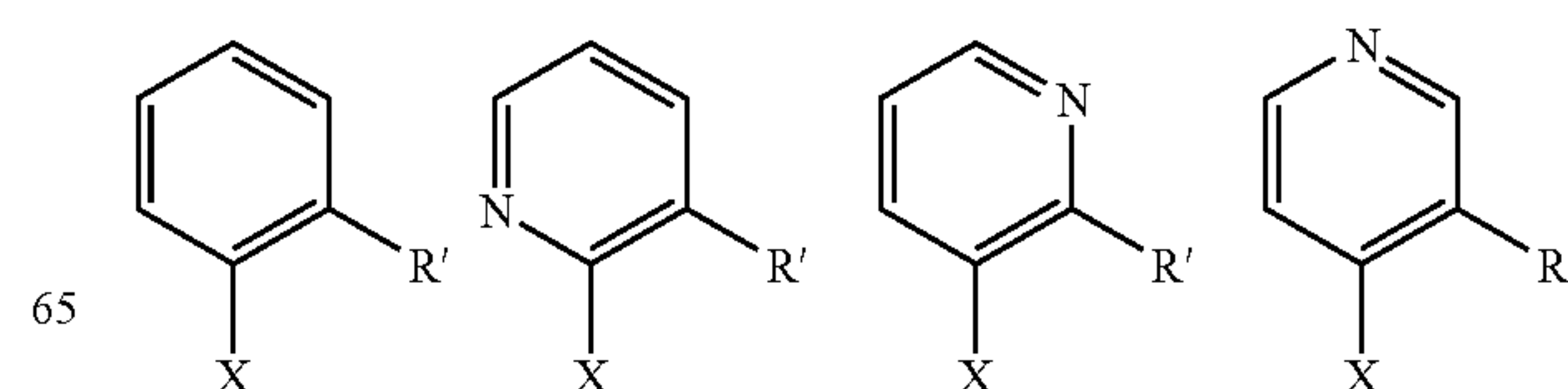
Scheme 17
