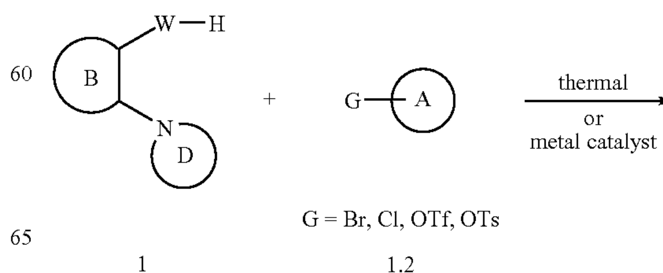
Scheme 1
