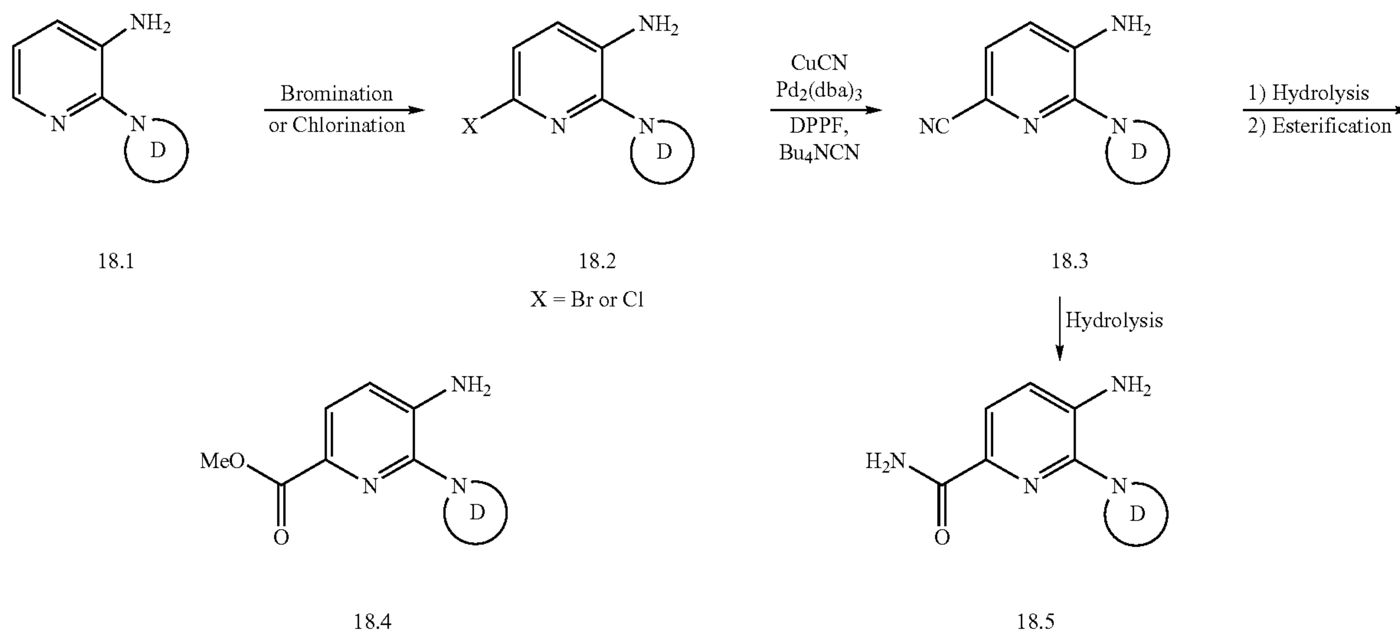
Scheme 18
