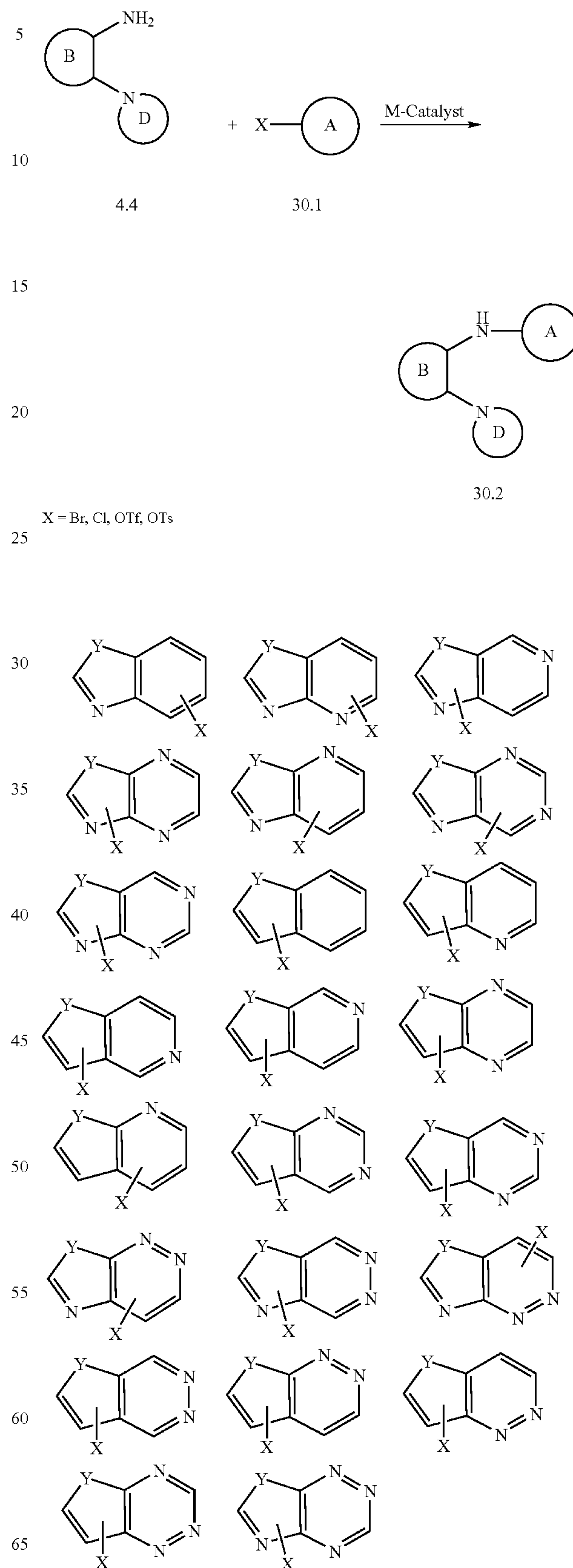
Scheme 30
