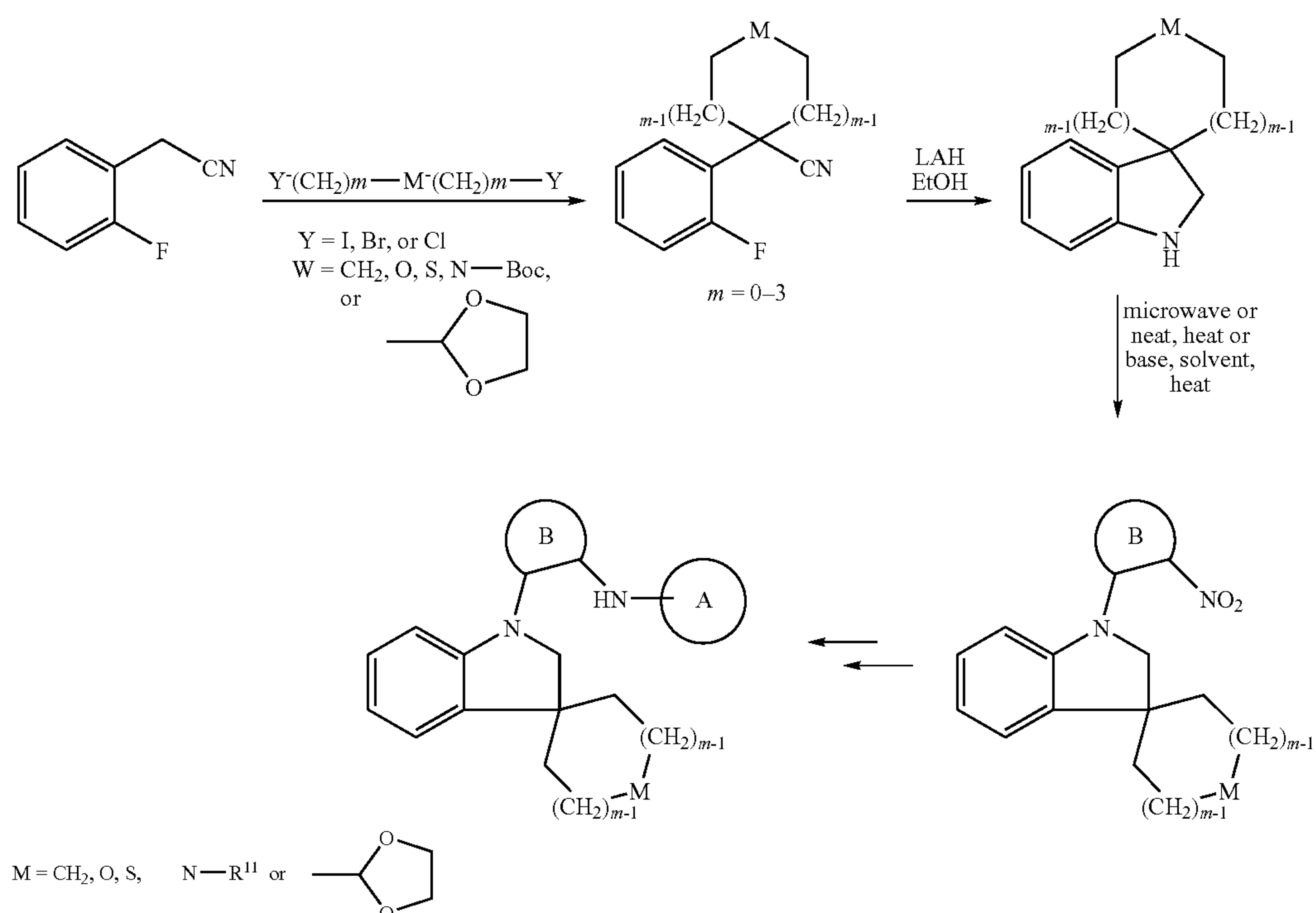
Scheme 28
