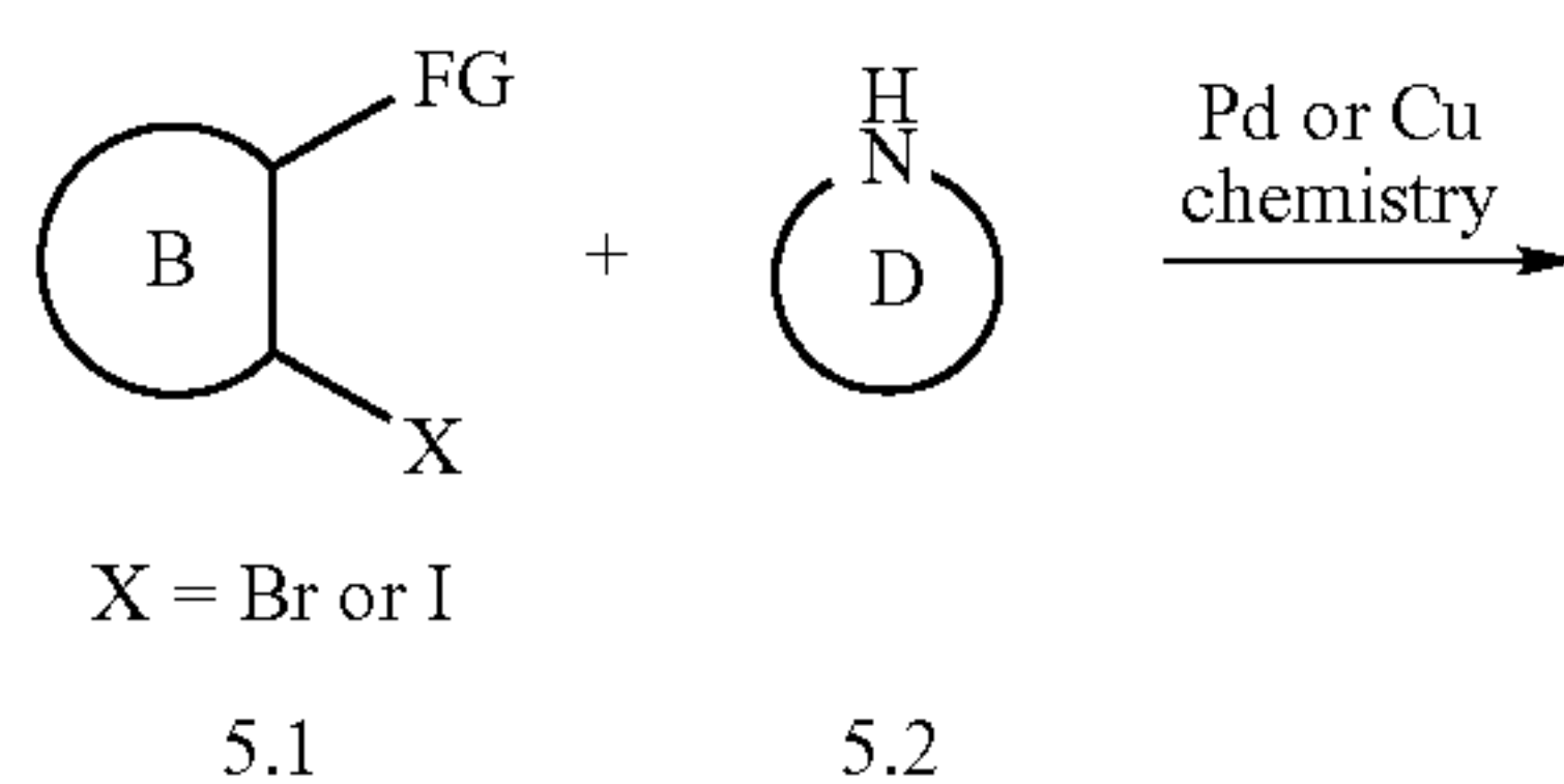
Scheme 5
