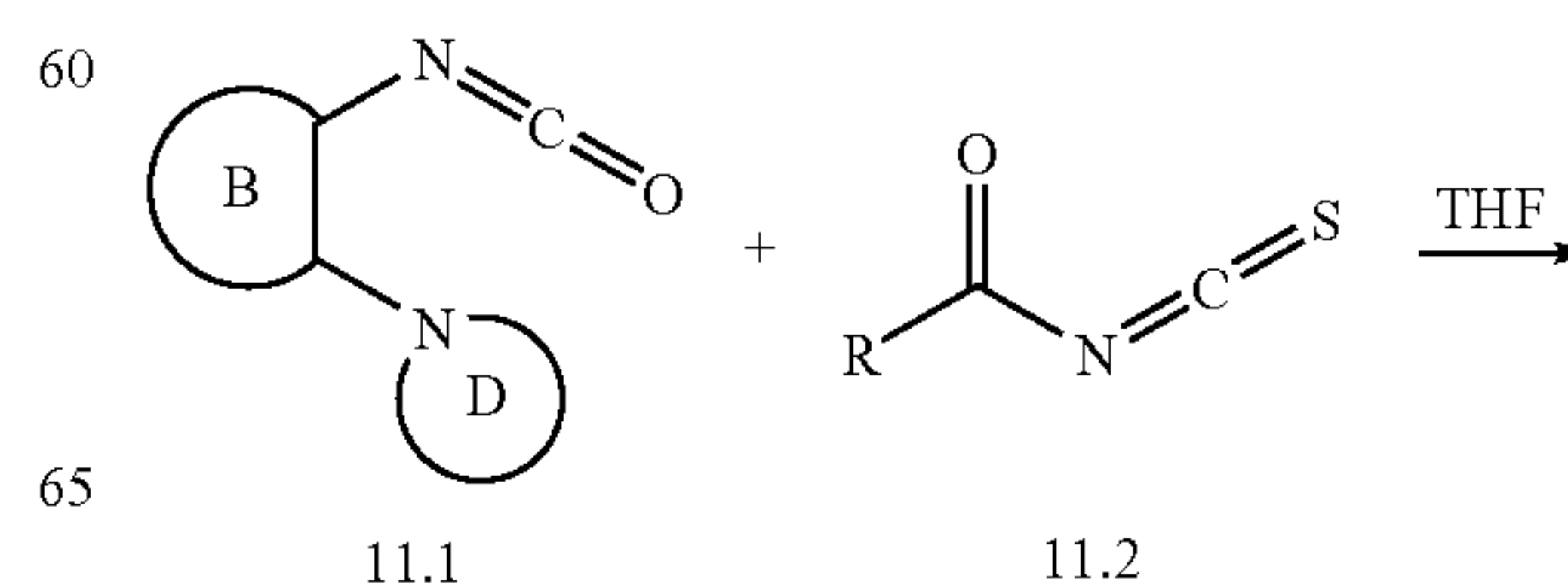
Scheme 11
