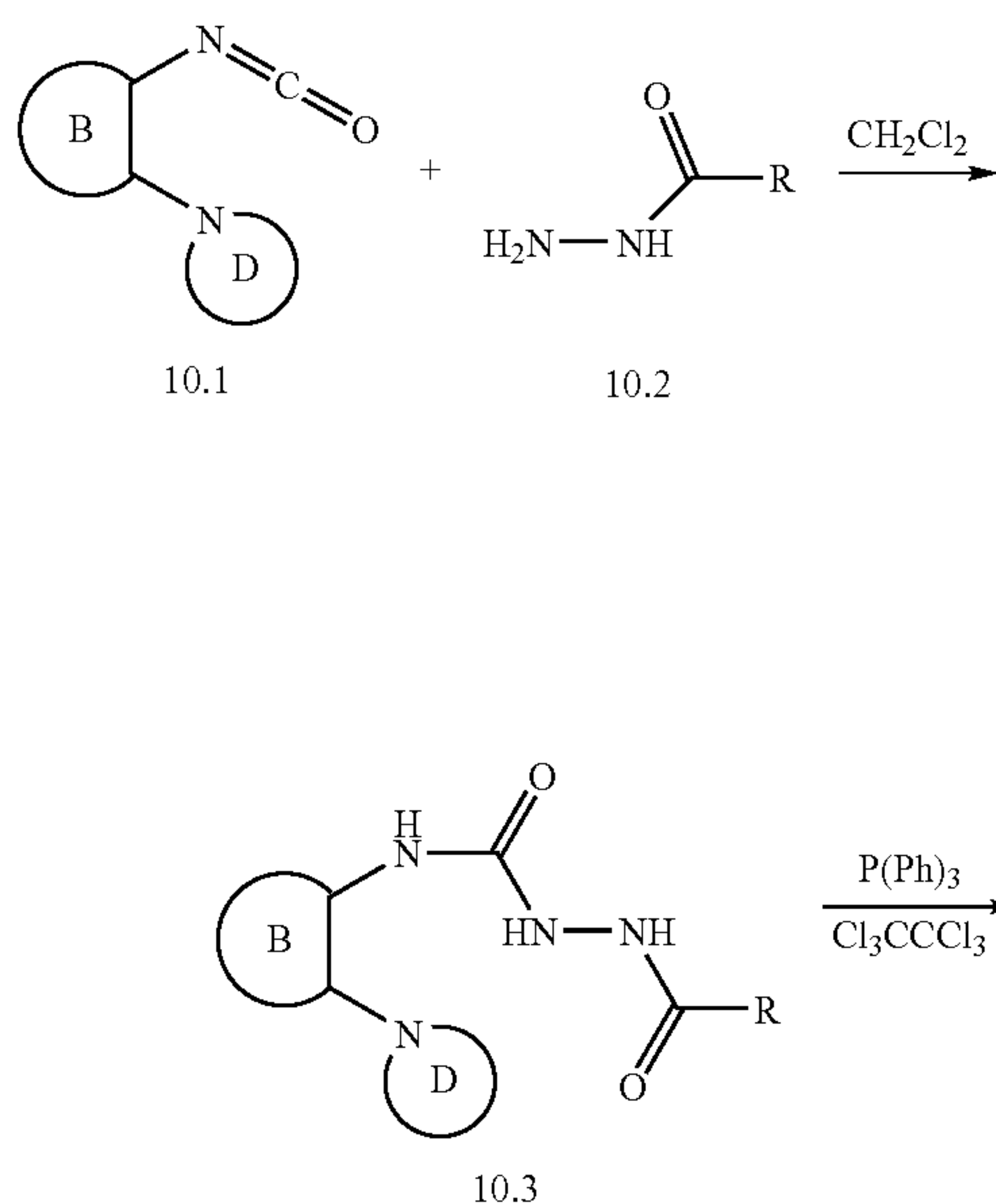
Scheme 10
