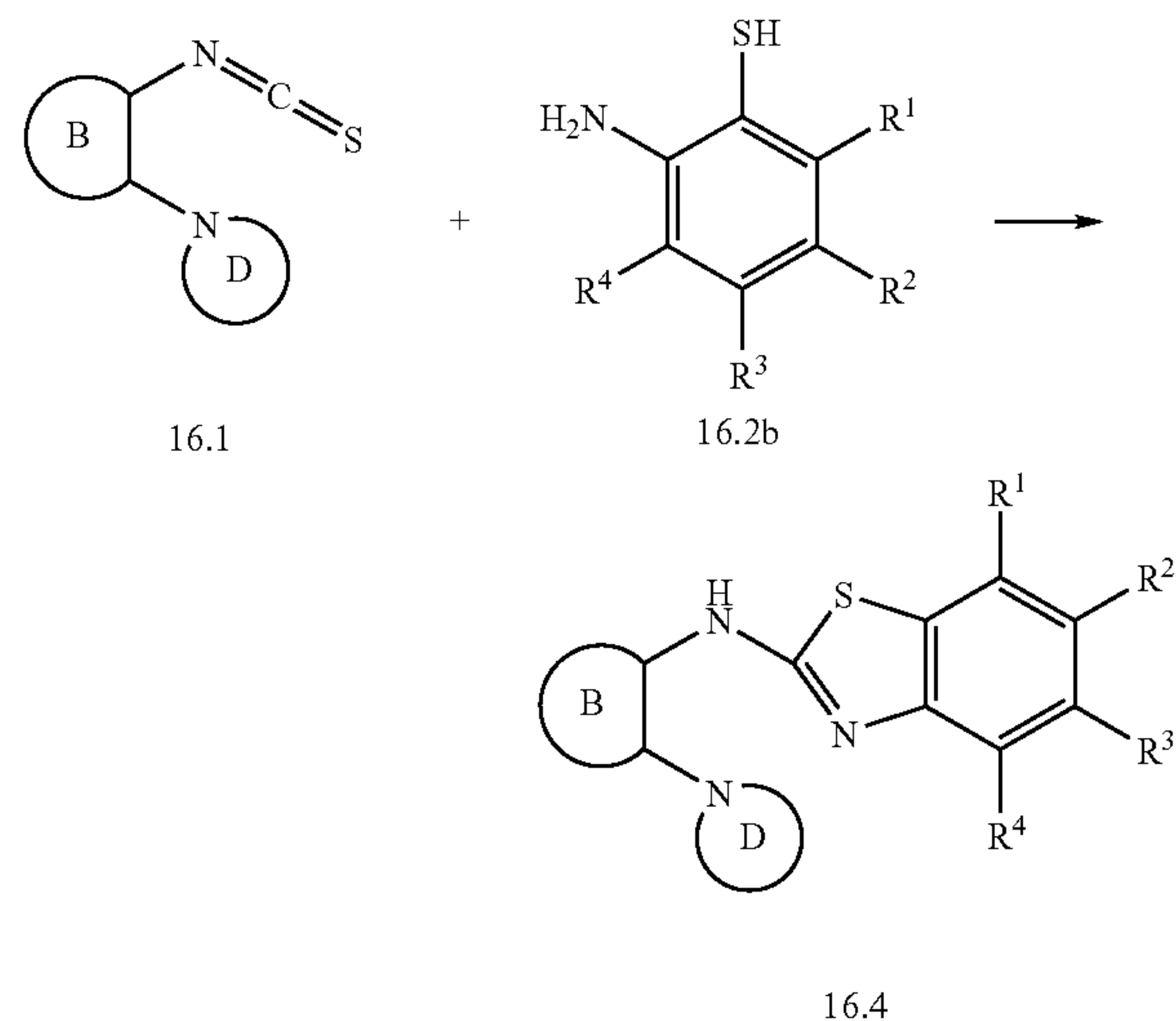
Scheme 16-b
