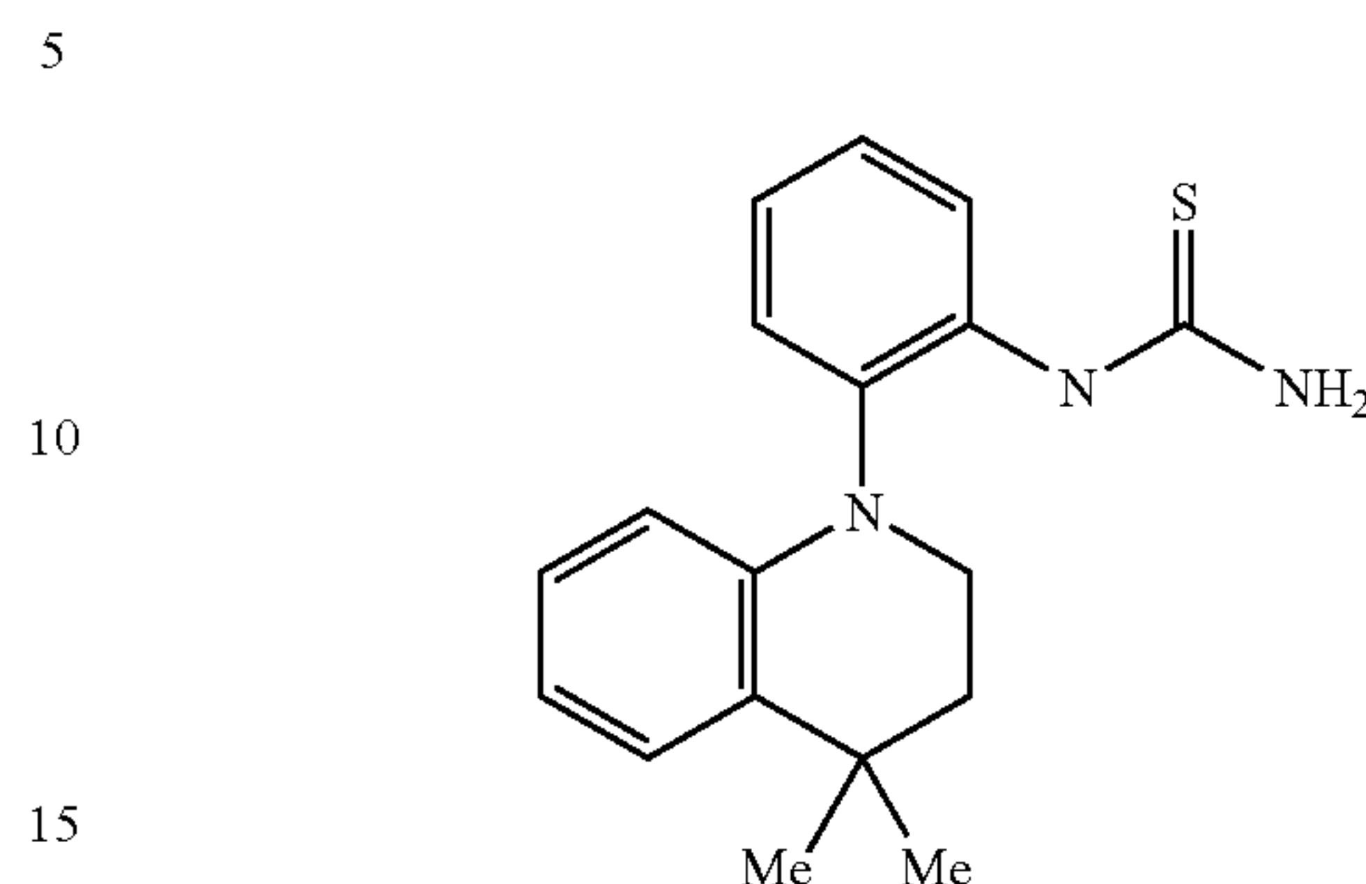
1f. 1-(2-(4,4-dimethyl-3,4-dihydroquinolin-1(2H)-yl)phenyl)thiourea
