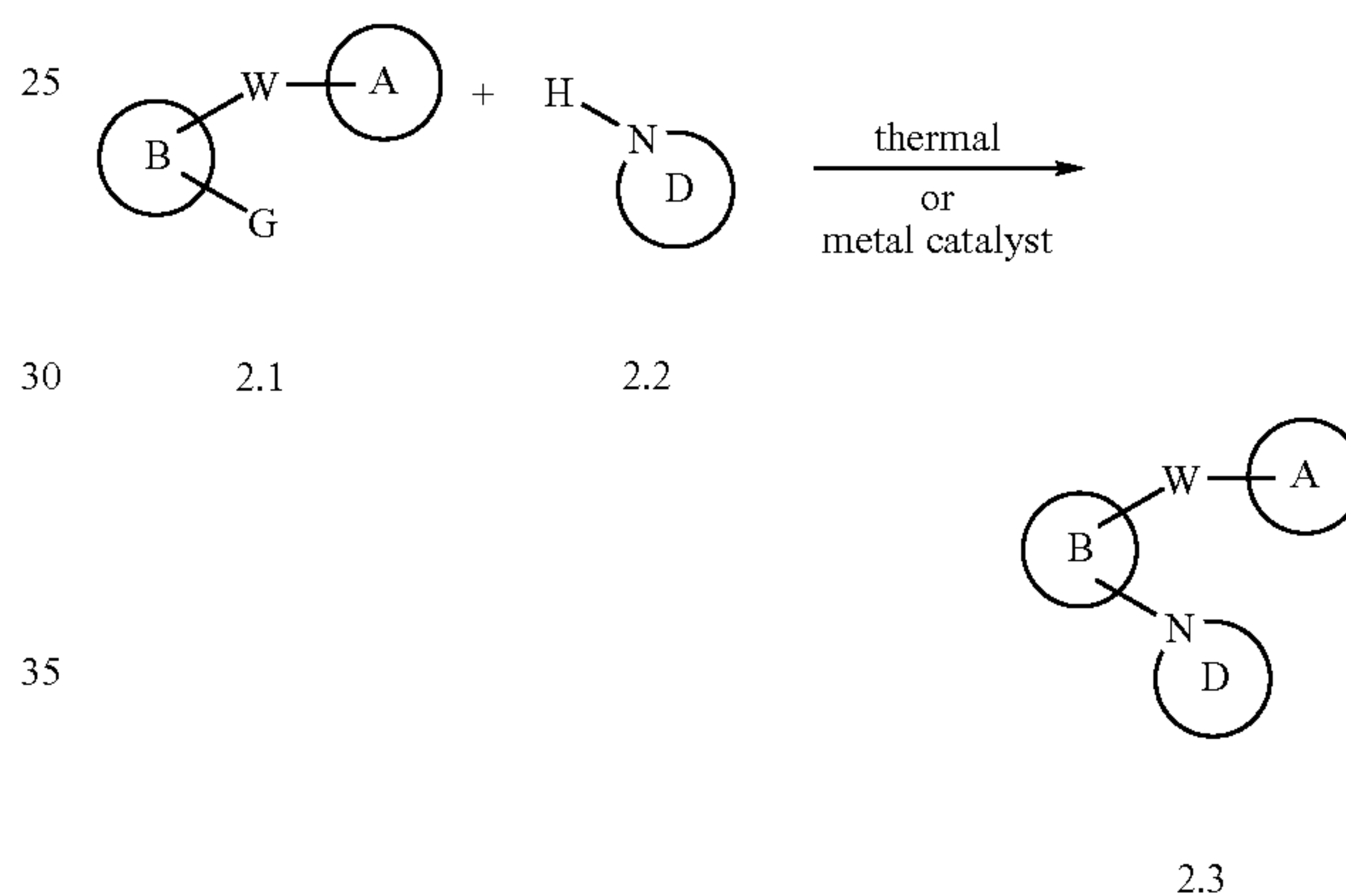
Scheme 2
