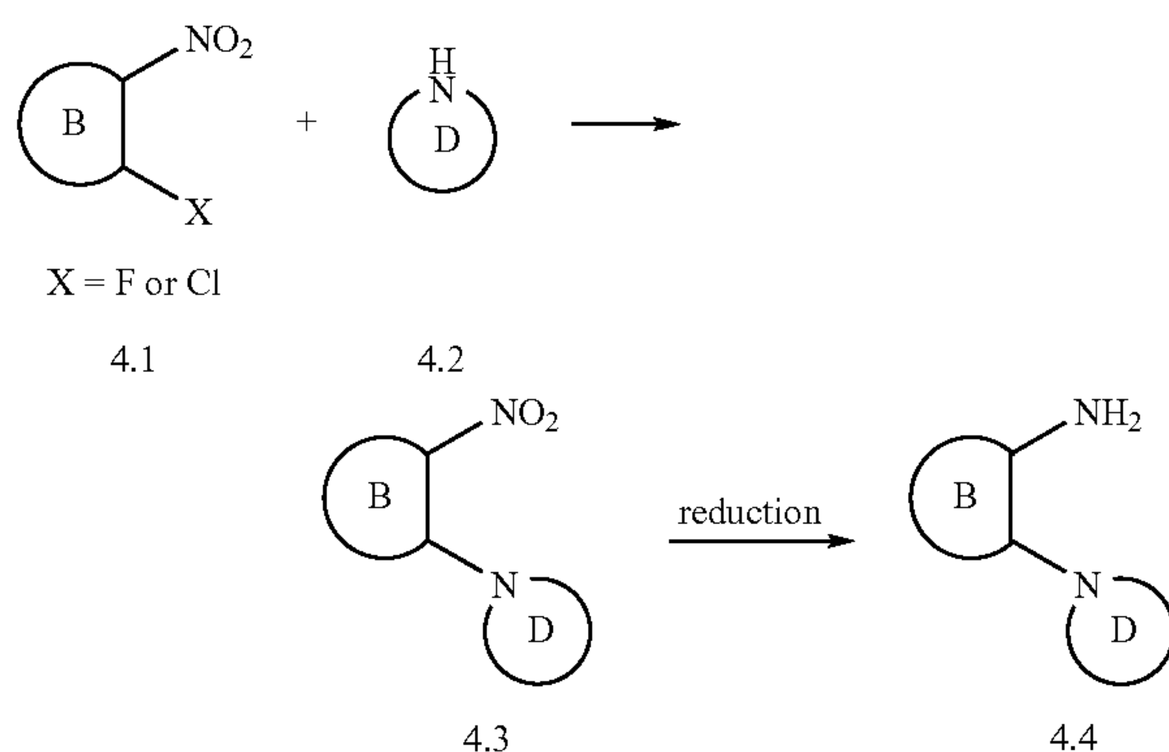
Scheme 4
