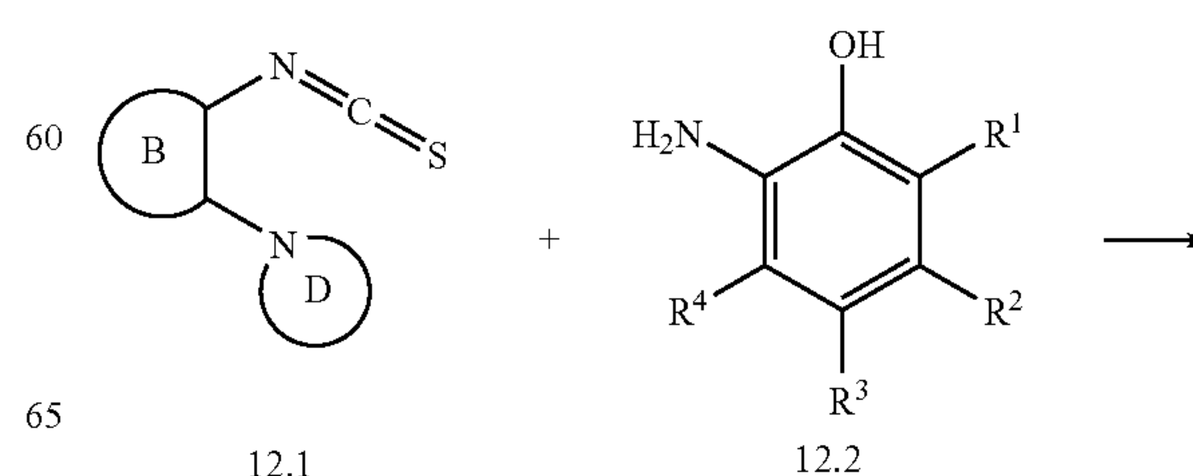
Scheme 15
