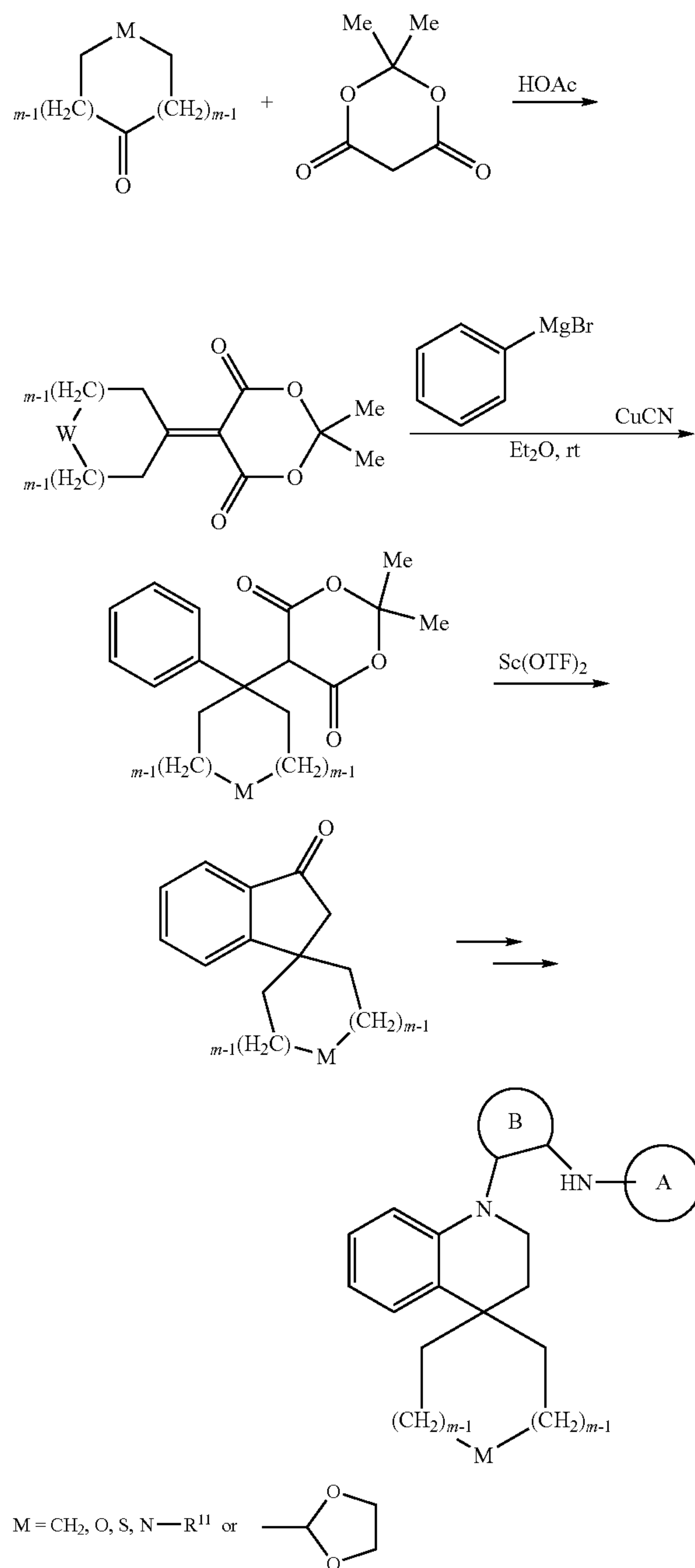
Scheme 29
