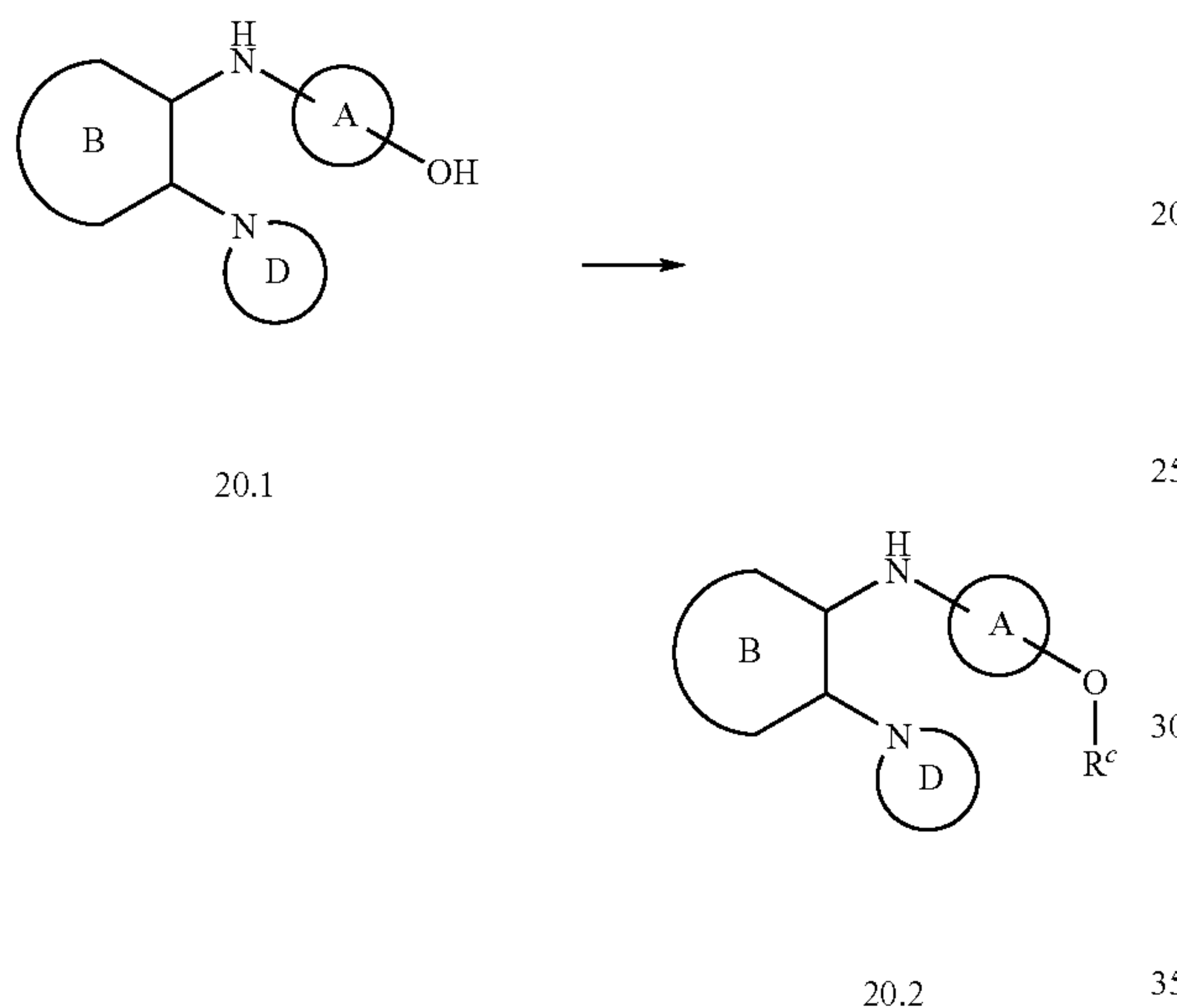
Scheme 20
