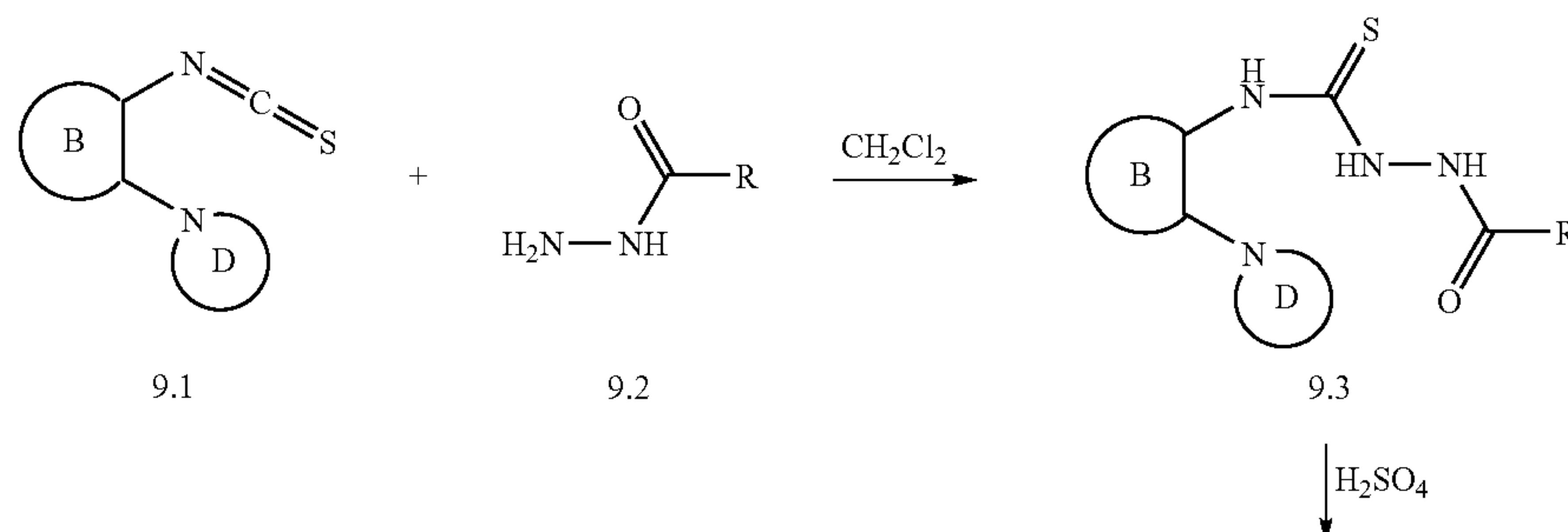
Scheme 9
