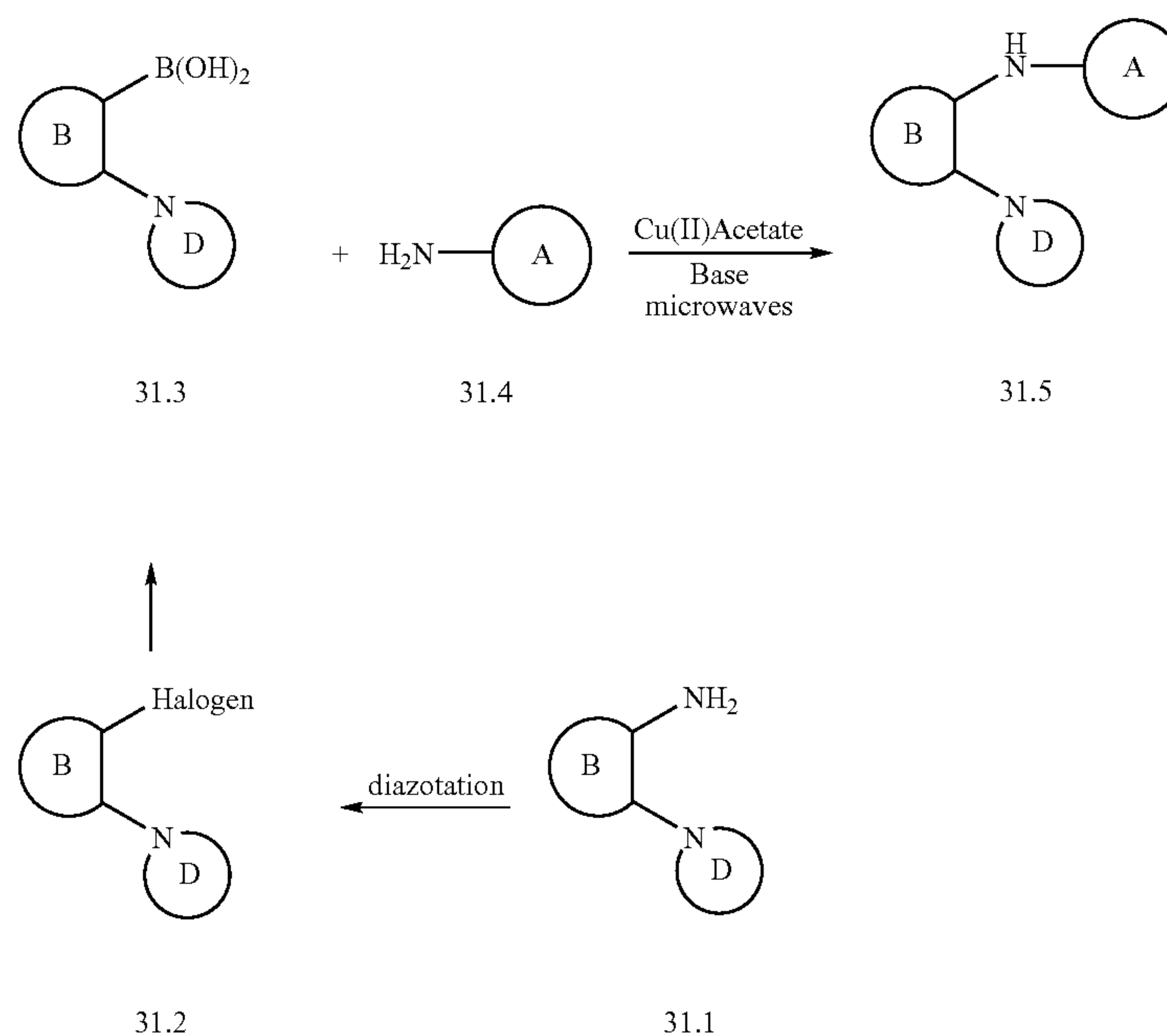
Scheme 31
