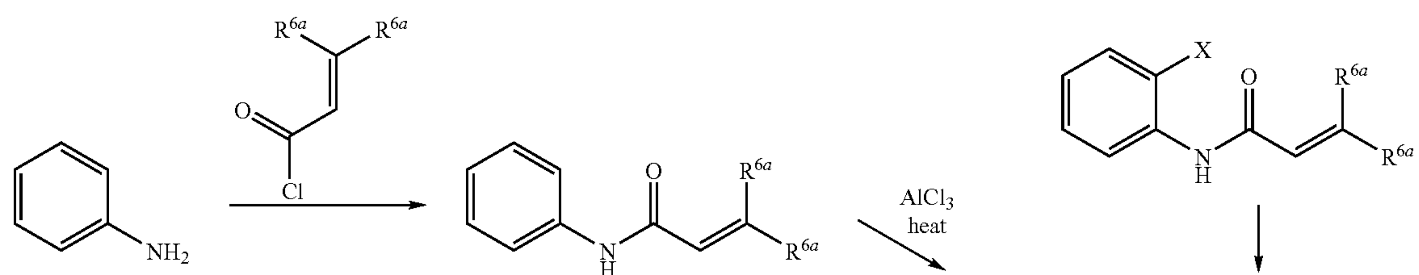
Scheme 25
