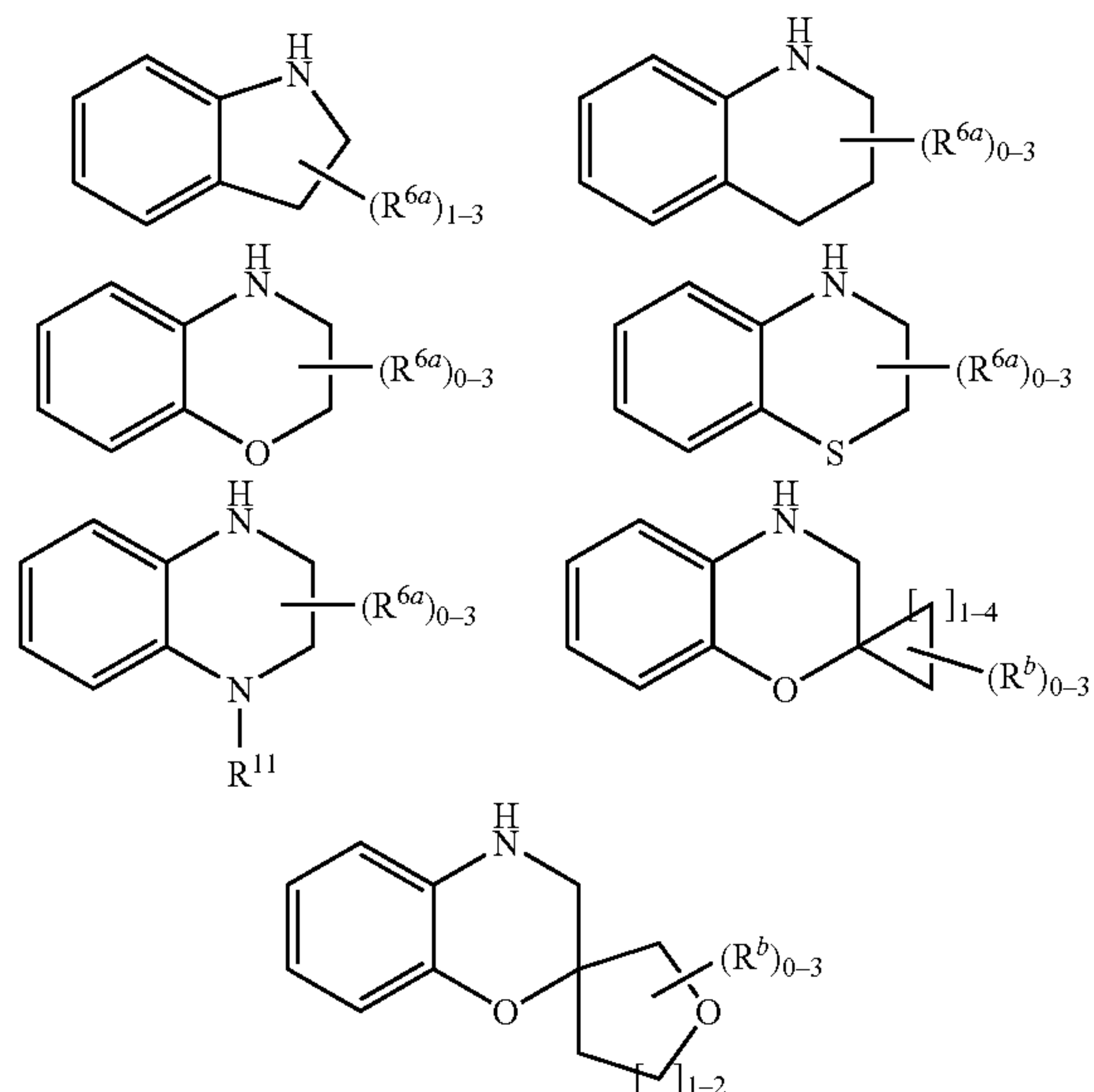
Scheme 21
