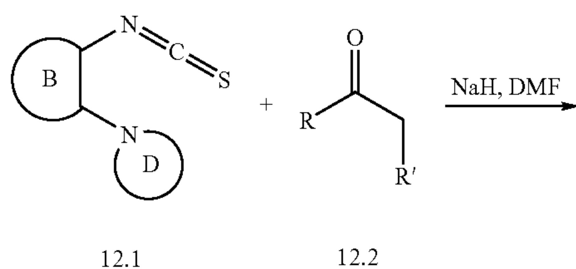
Scheme 12
