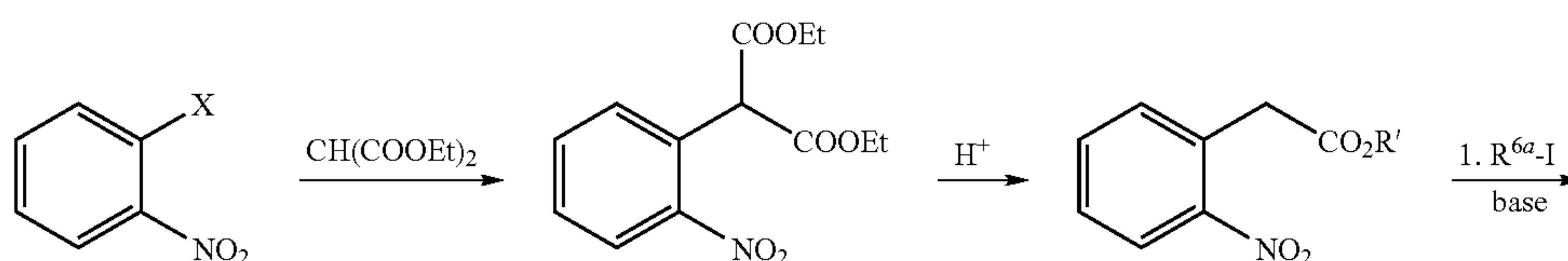
Scheme 22
