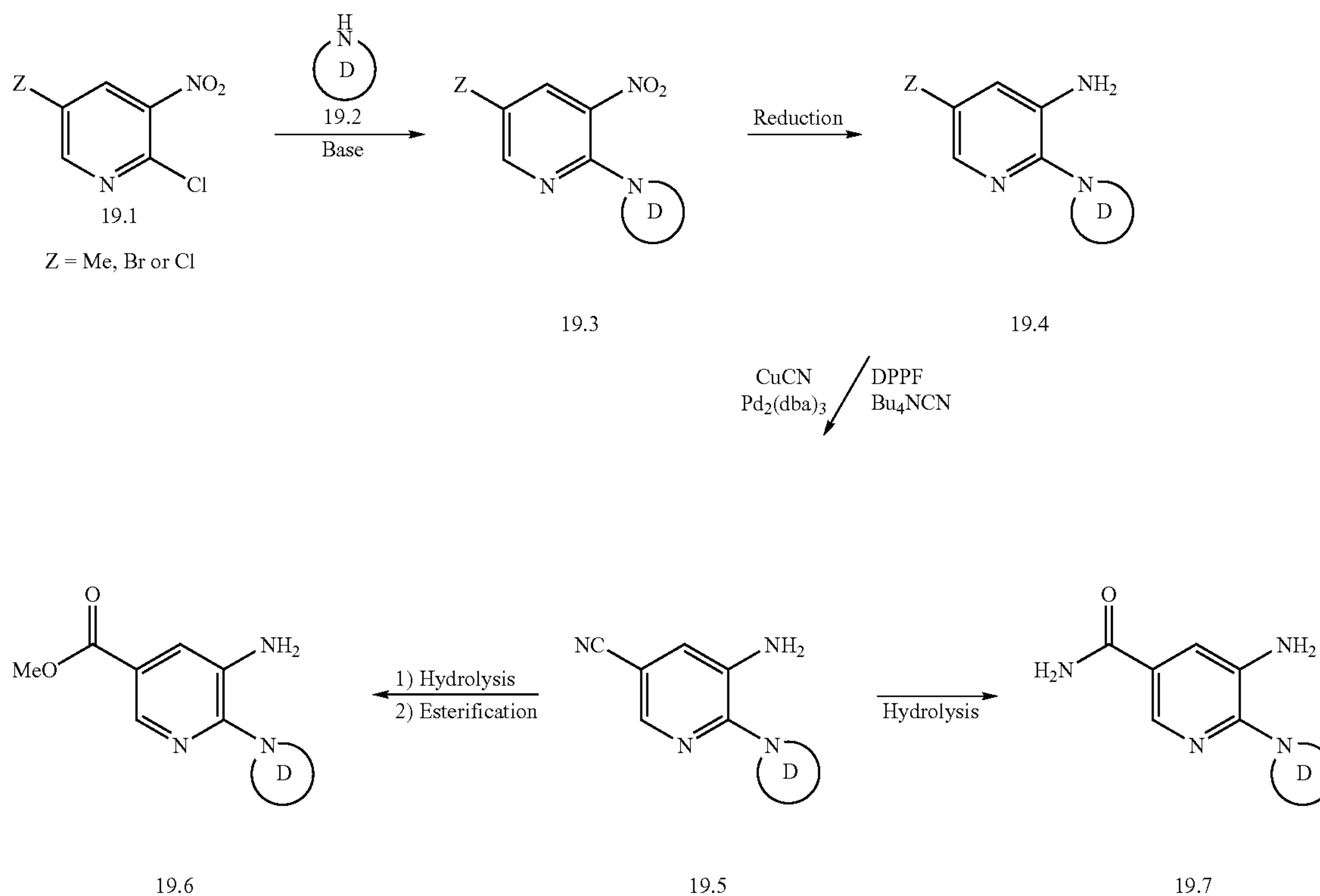
Scheme 19
