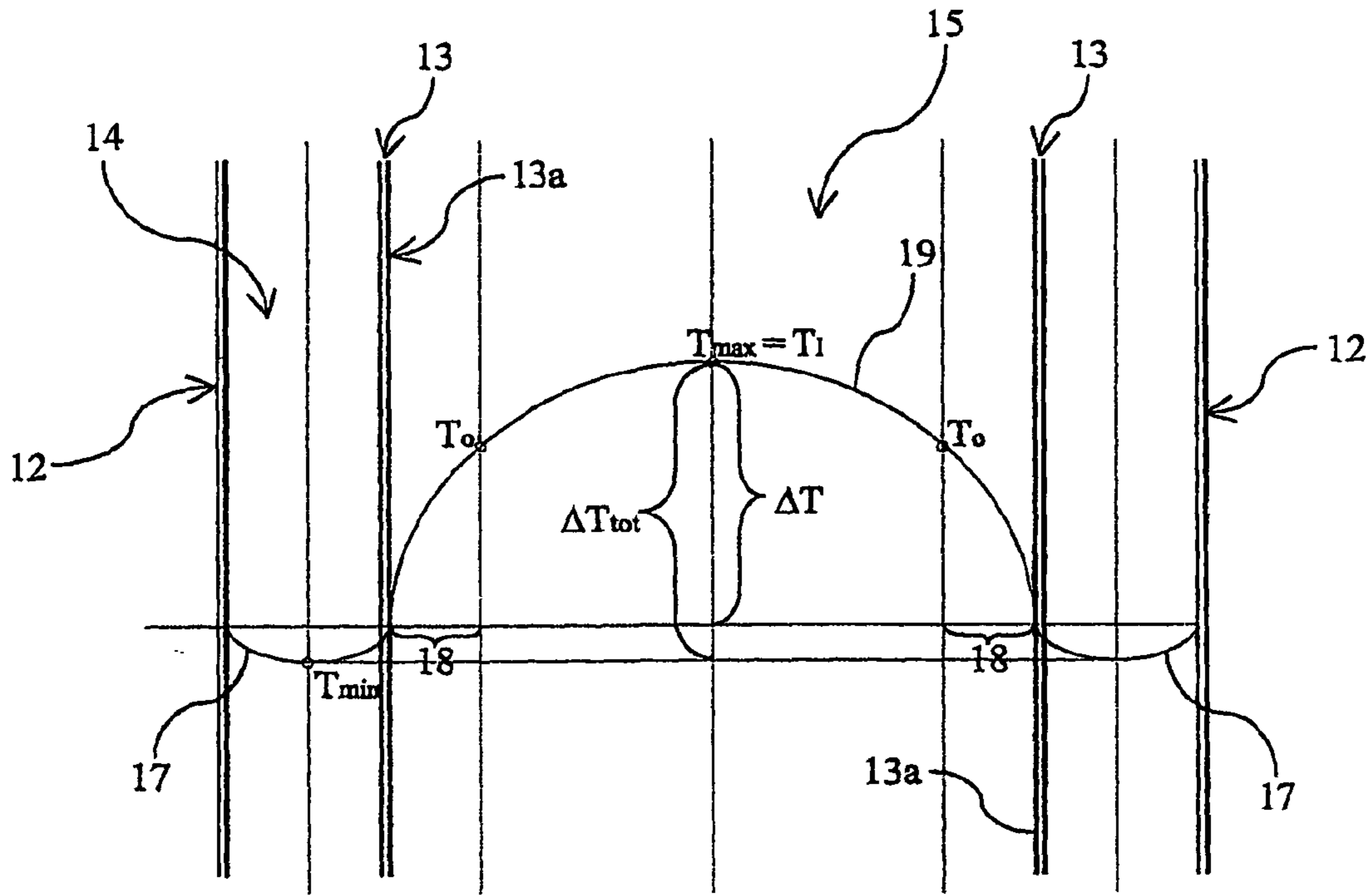
Fig 2 (Prior Art)
