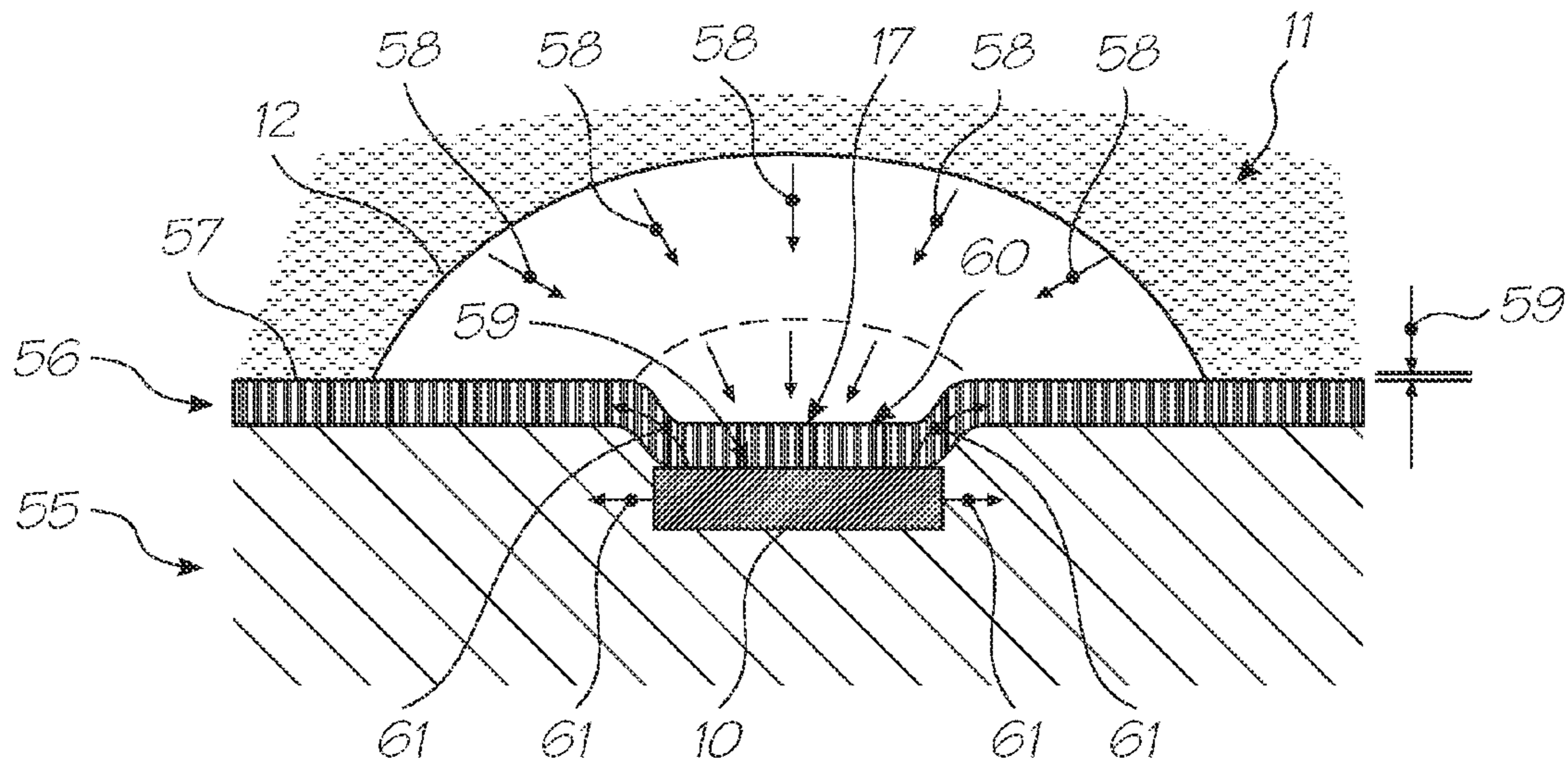
FIG. 47 (PRIOR ART)
