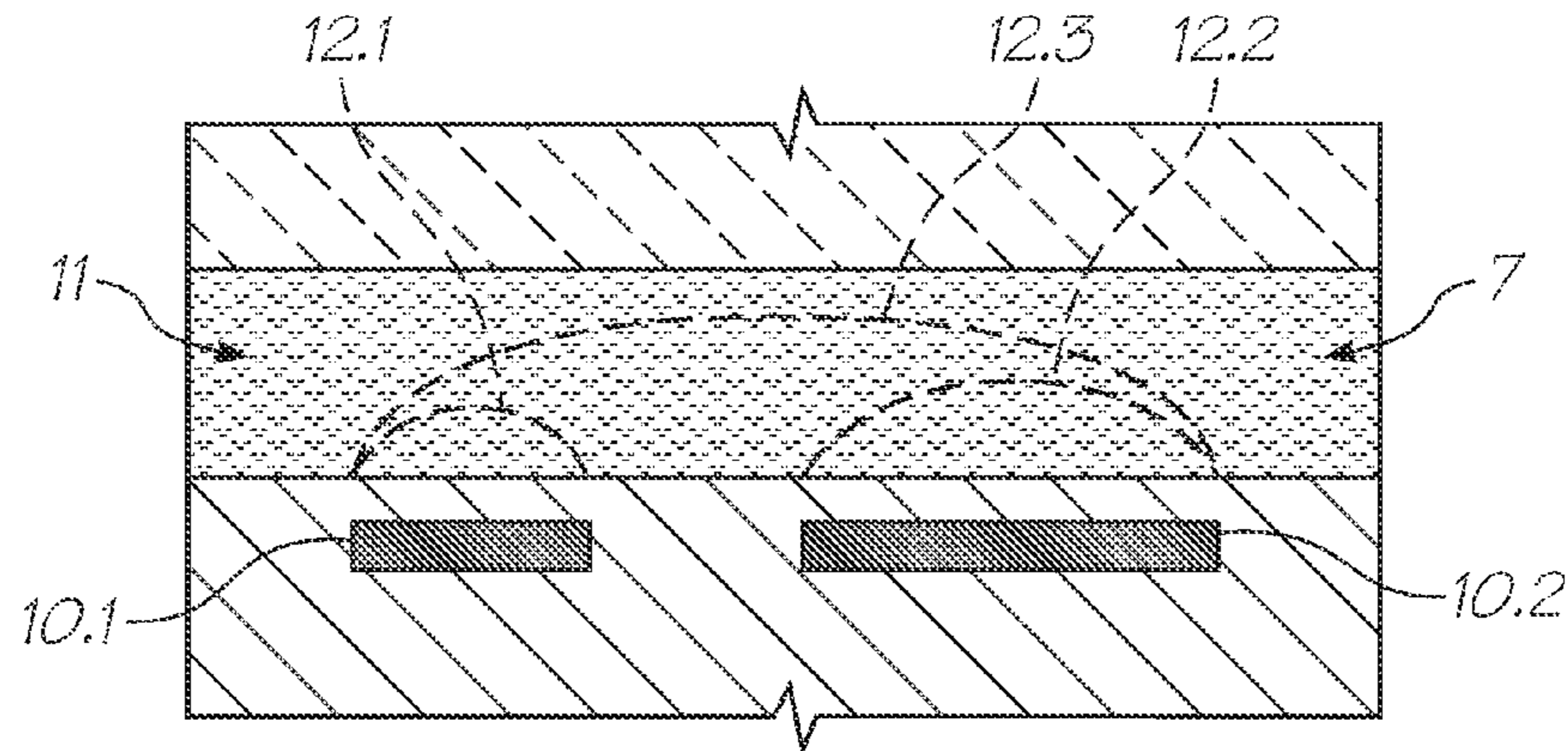
FIG. 52 (PRIOR ART)
