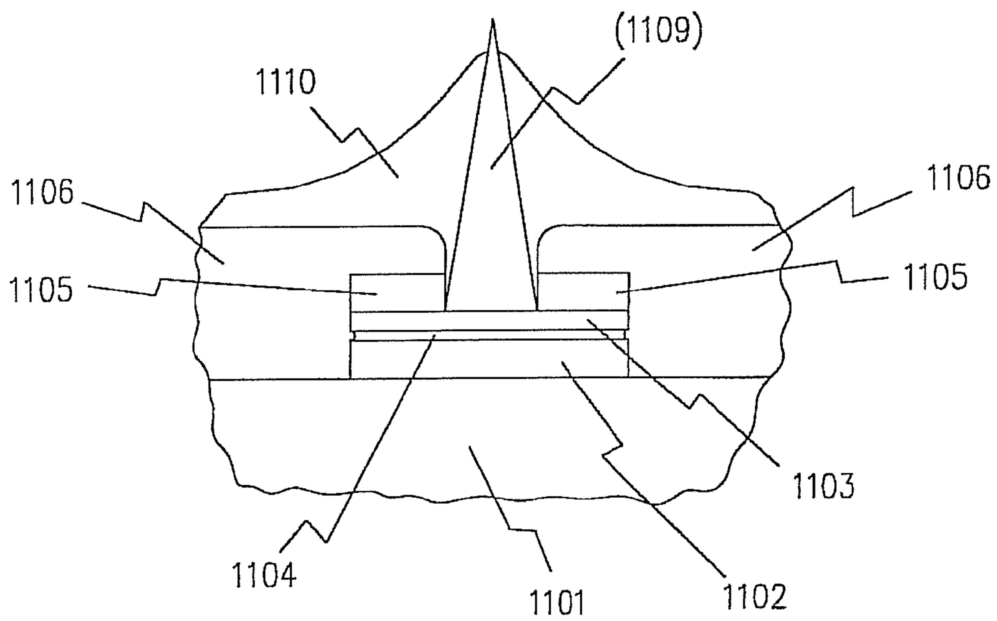
FIGURE 11b ELECTRODES
