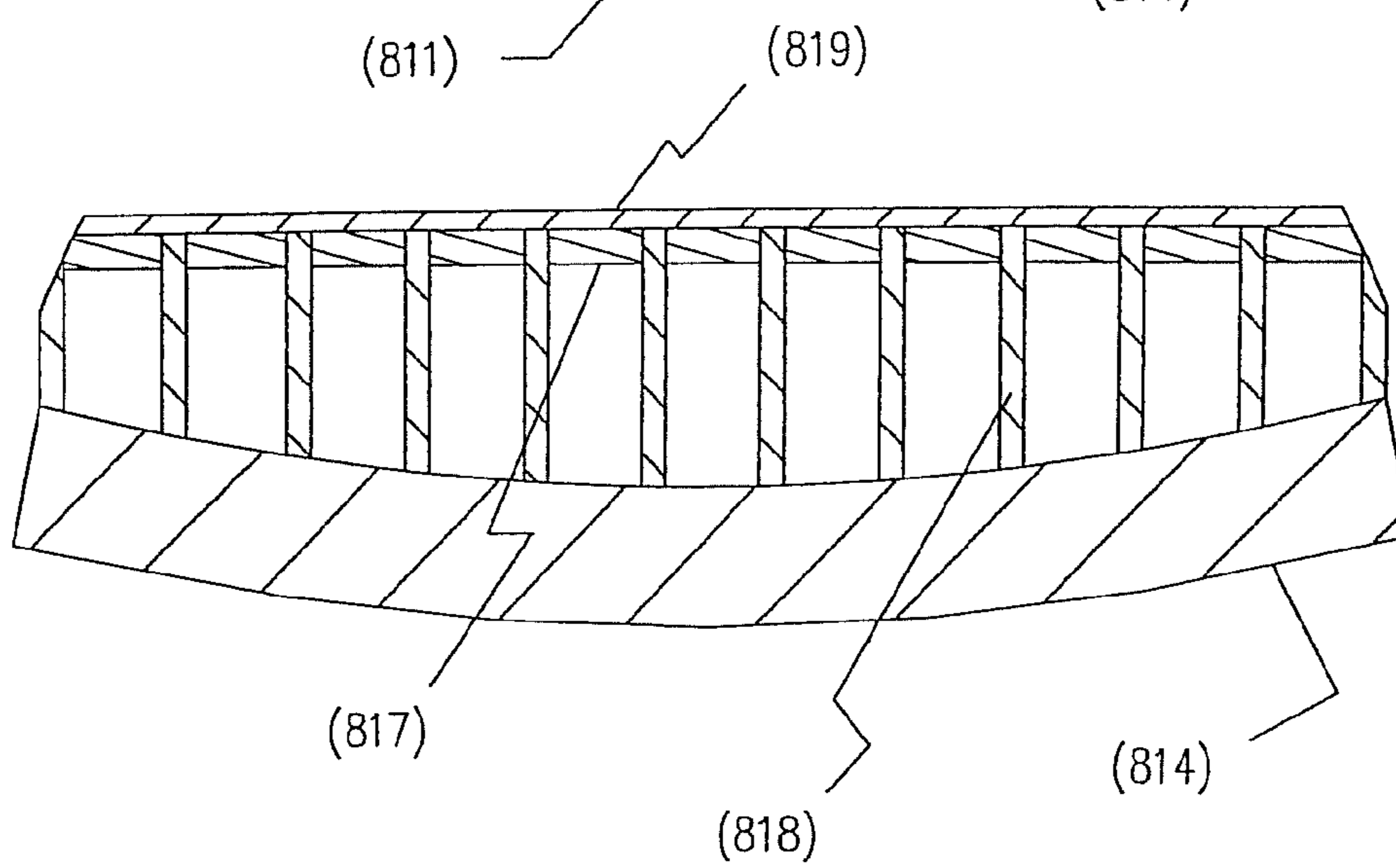
FIGURE 8b EPIRETINAL ELECTRODES - RECESSED
