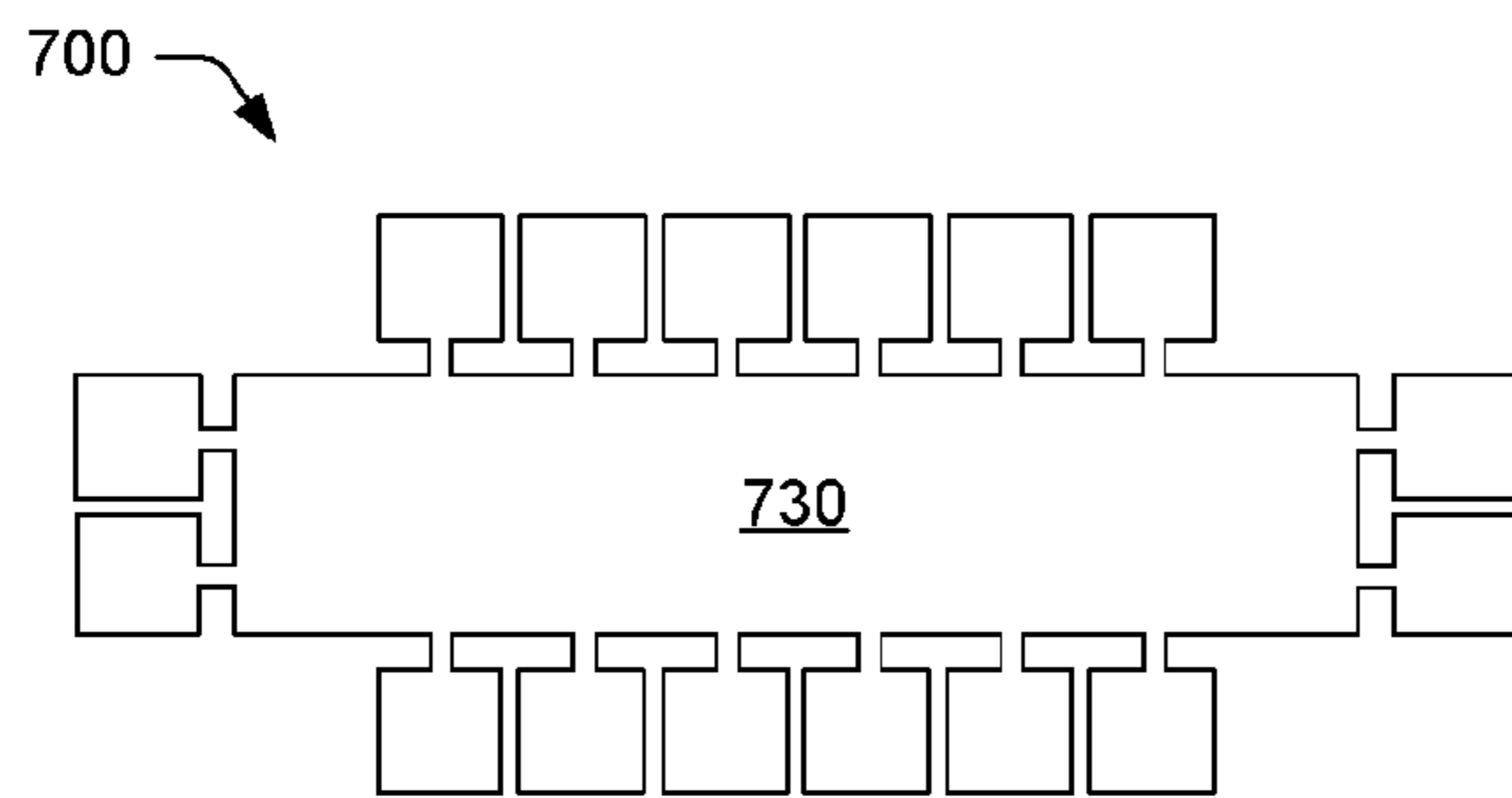
FIG. 7A UNFOLDED PATTERN
