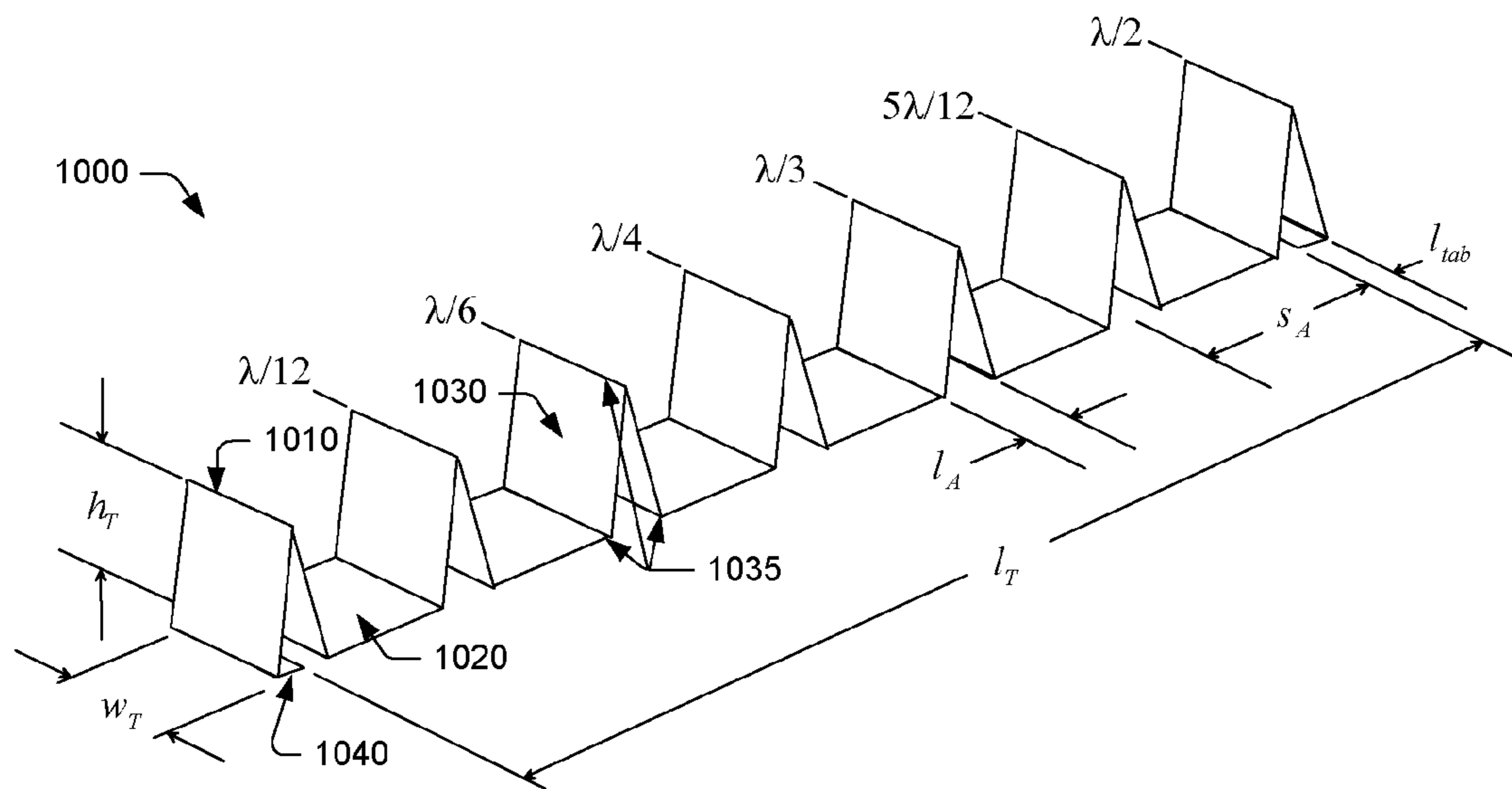
FIG. 10B FOLDED PATTERN
