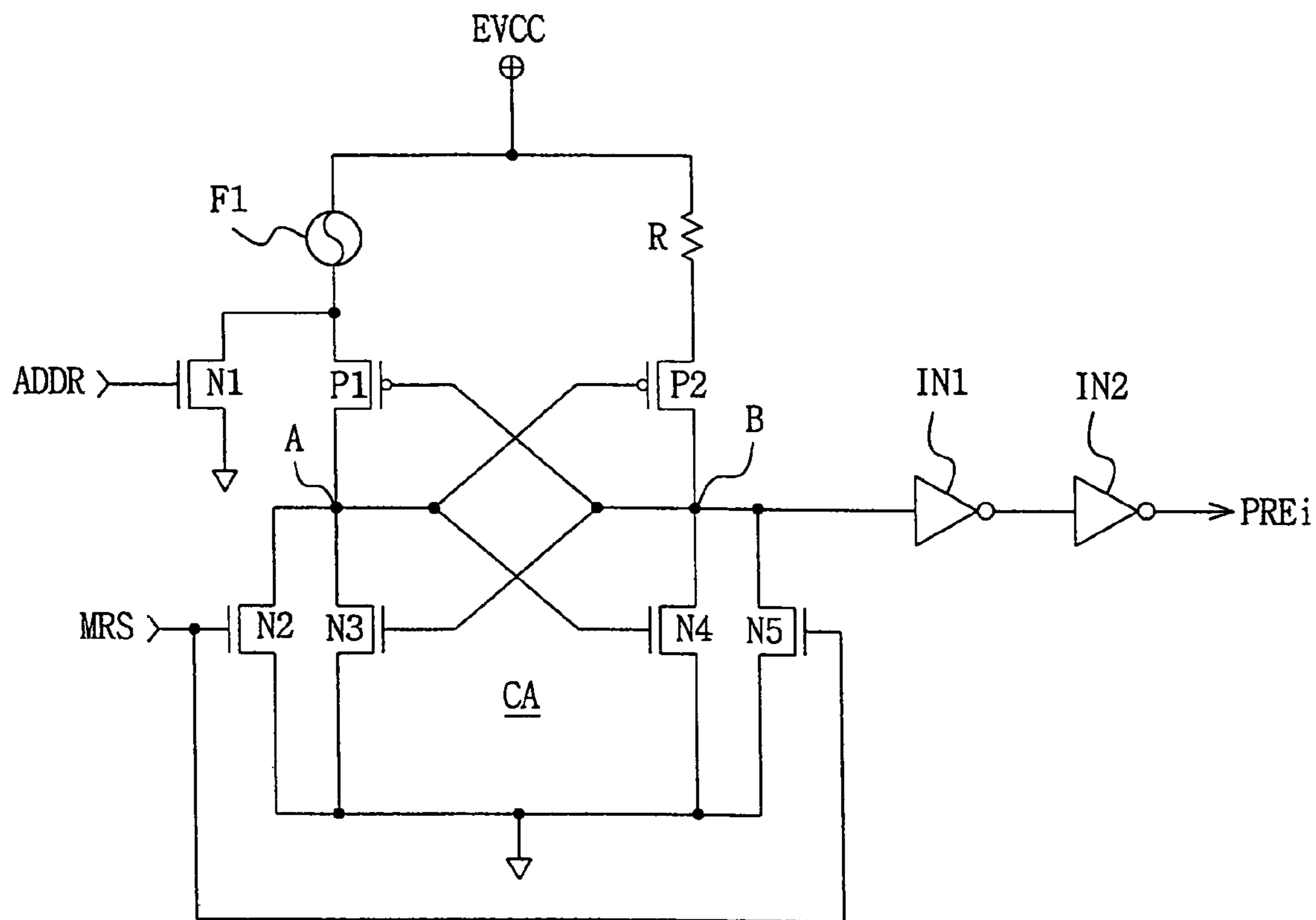
FIG. 1 (PRIOR ART)
