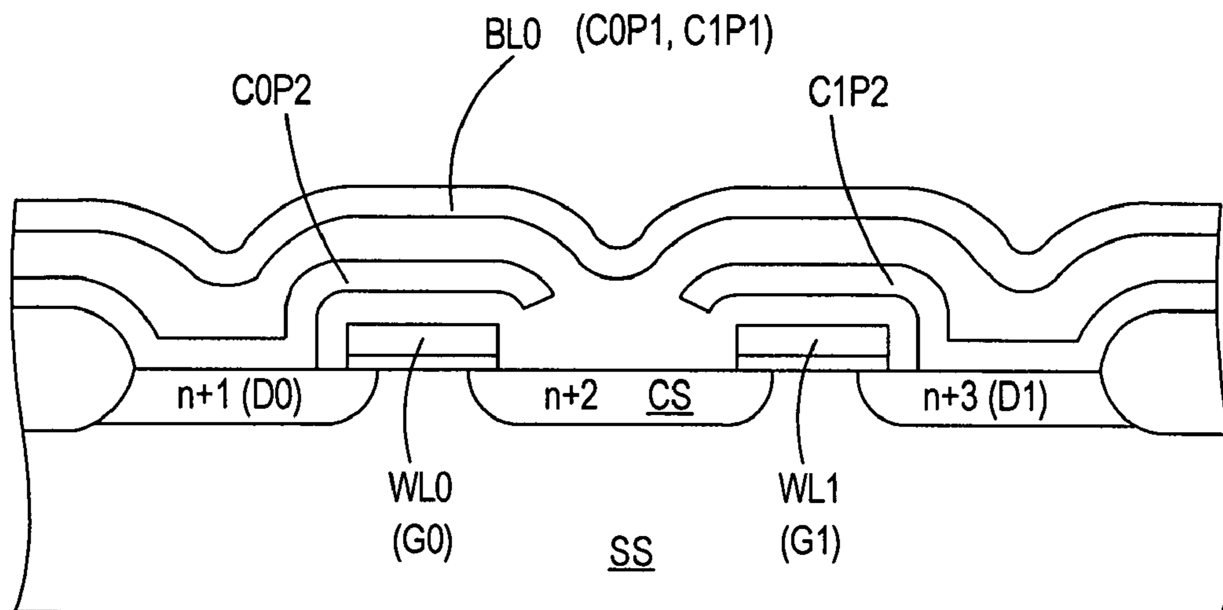
FIGURE 2 (PRIOR ART)
