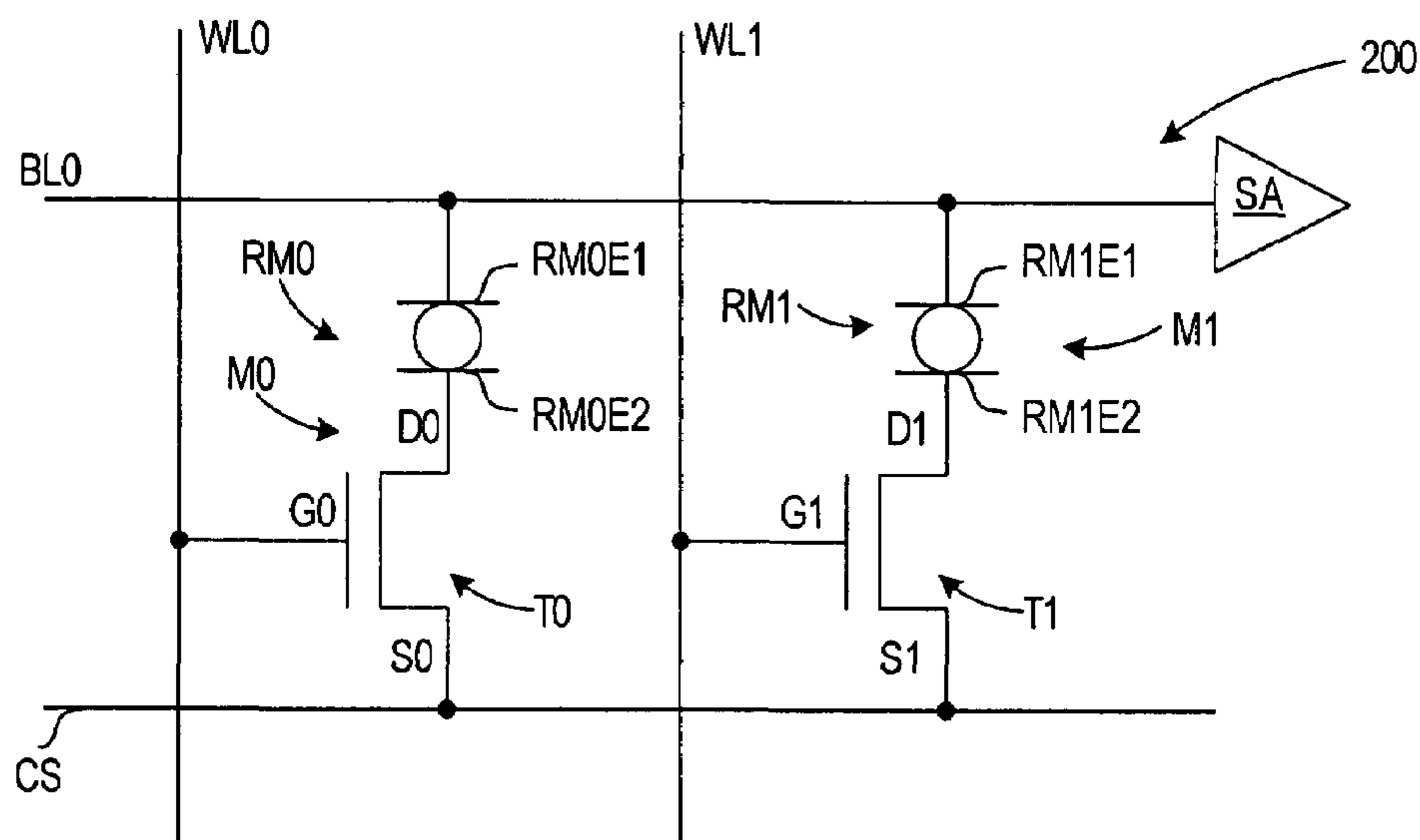
FIGURE 6 (PRIOR ART)
