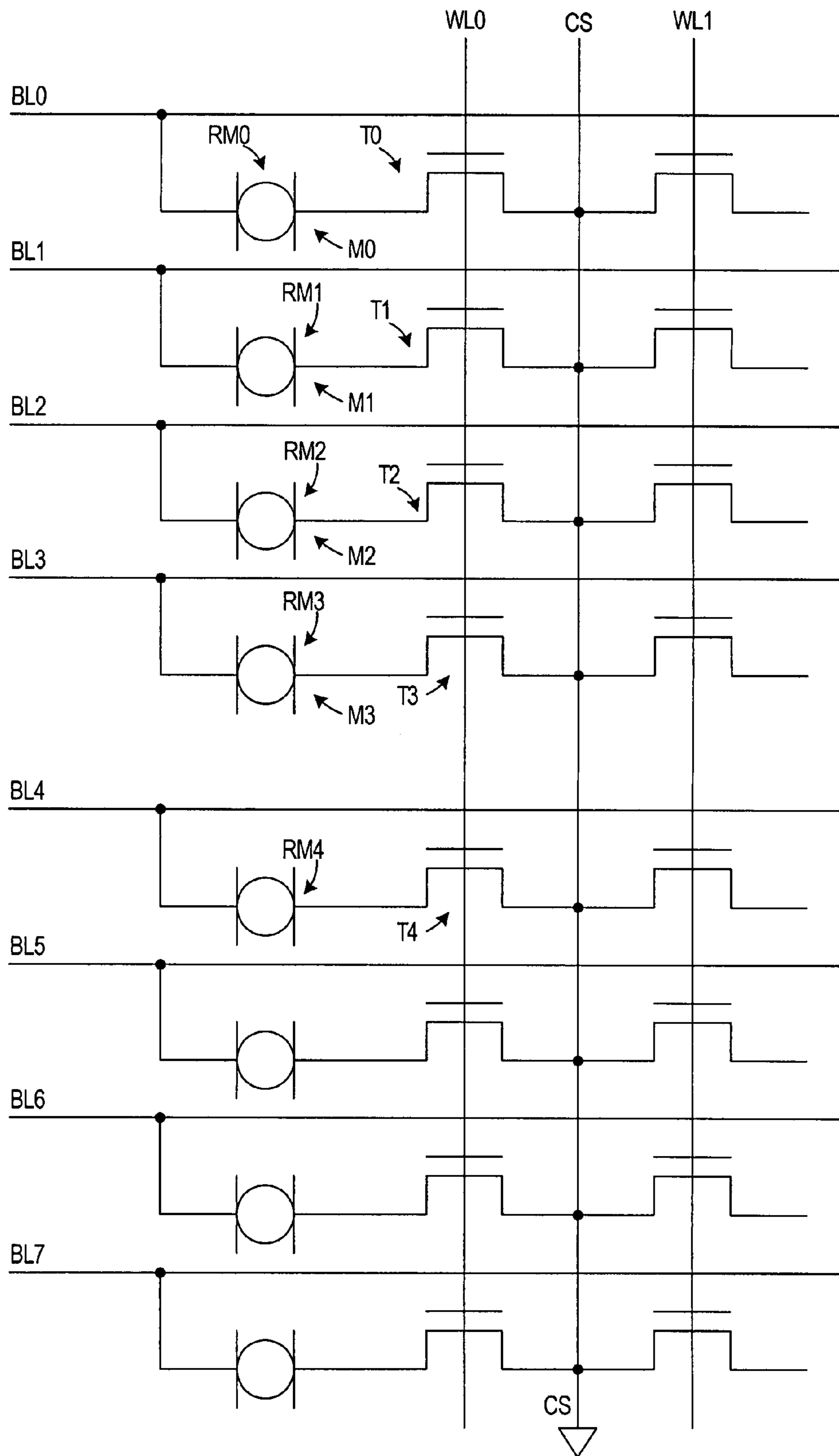
FIGURE 7 (PRIOR ART)
