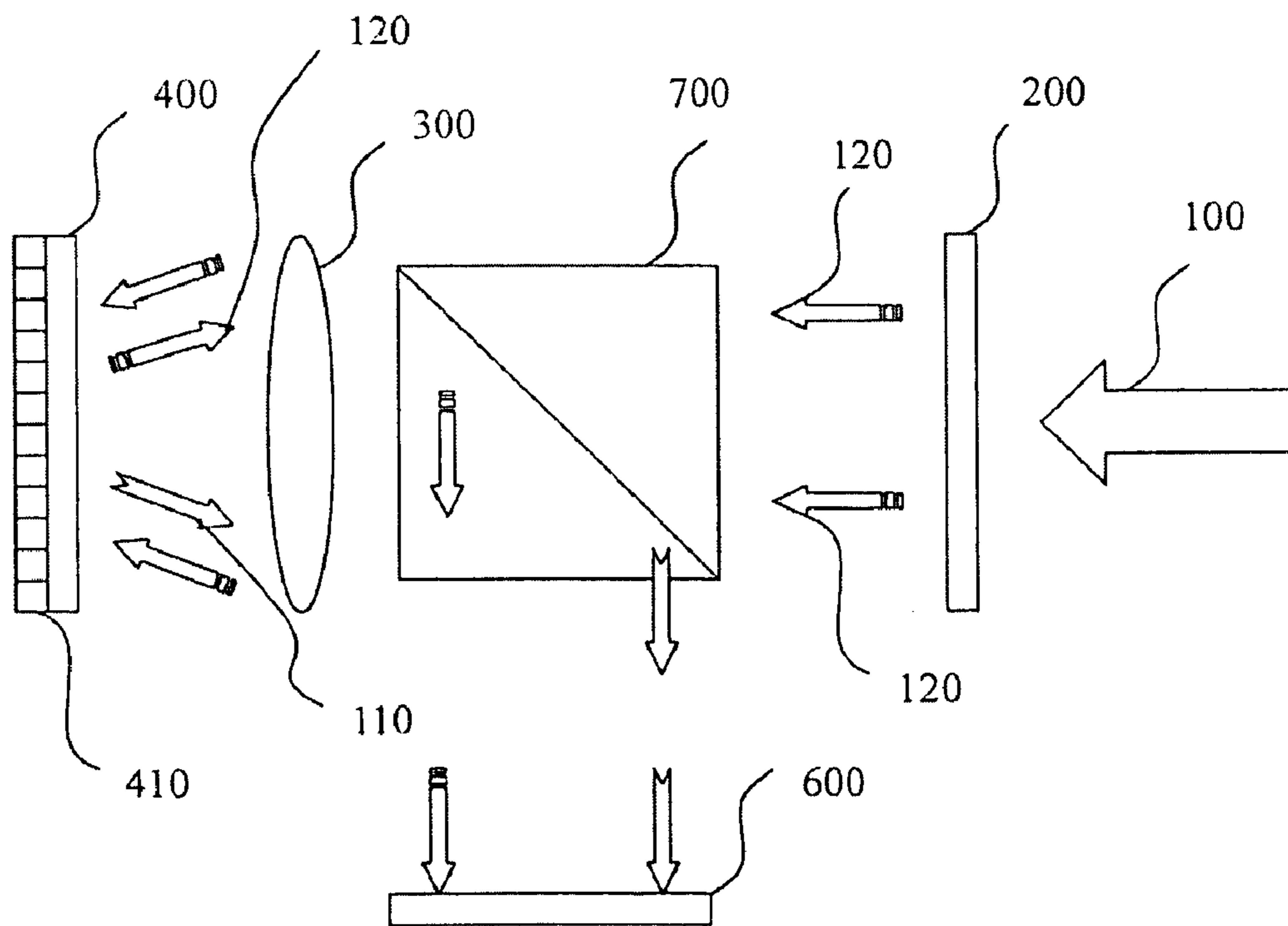
FIG. 2a(PRIOR ART)
