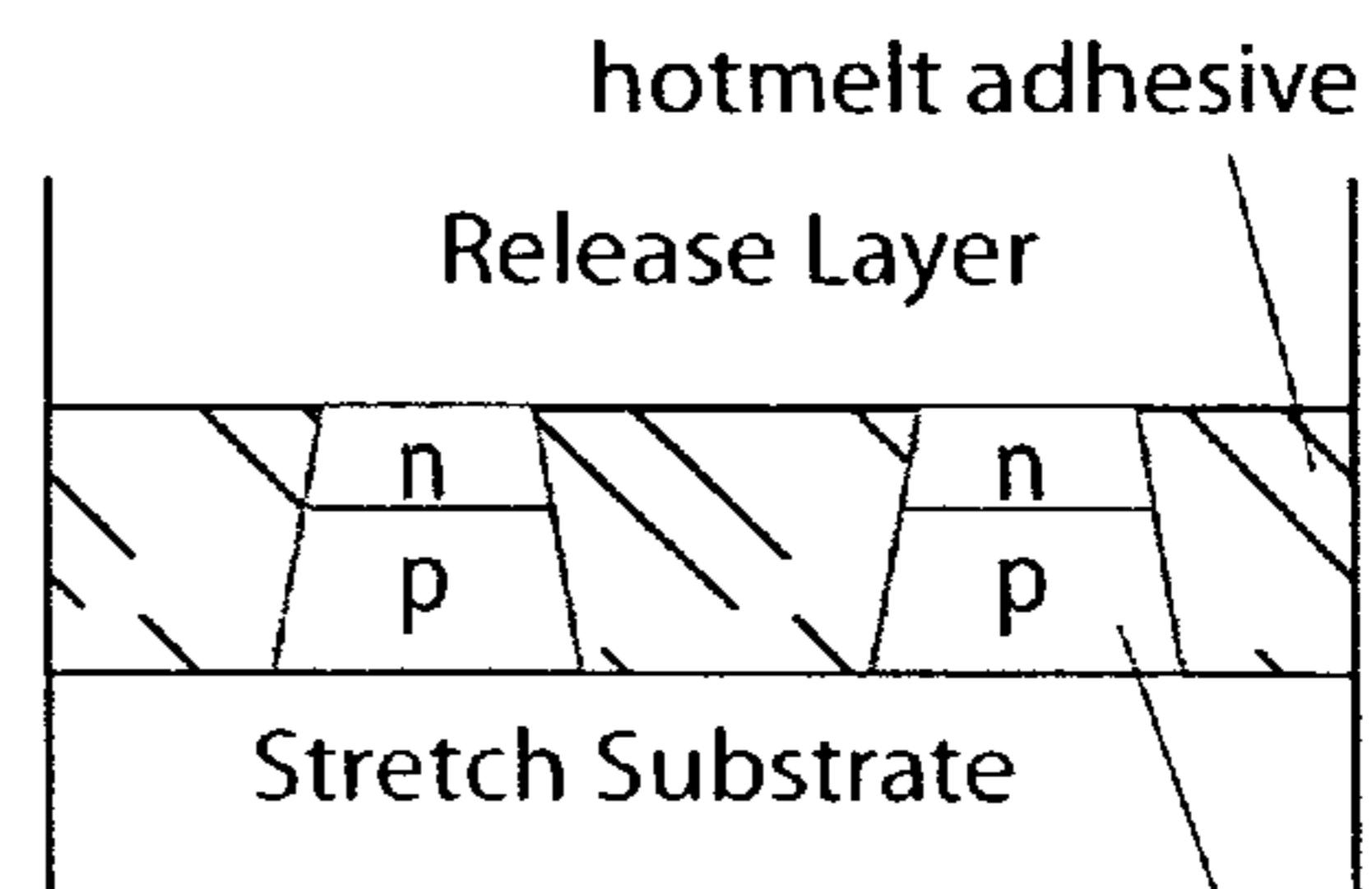
Figure 83(a) embedded LED chips
