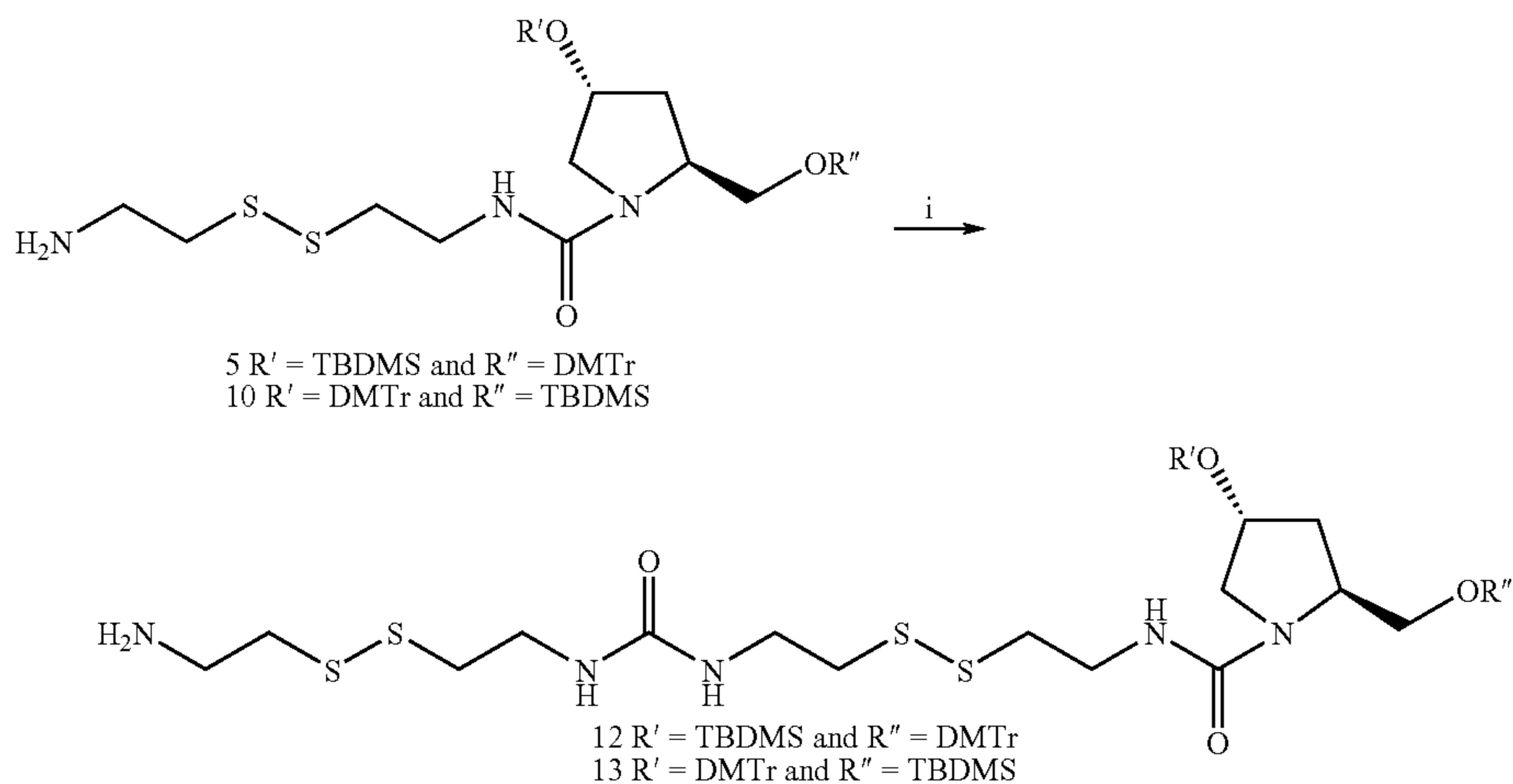
Scheme 2 a
