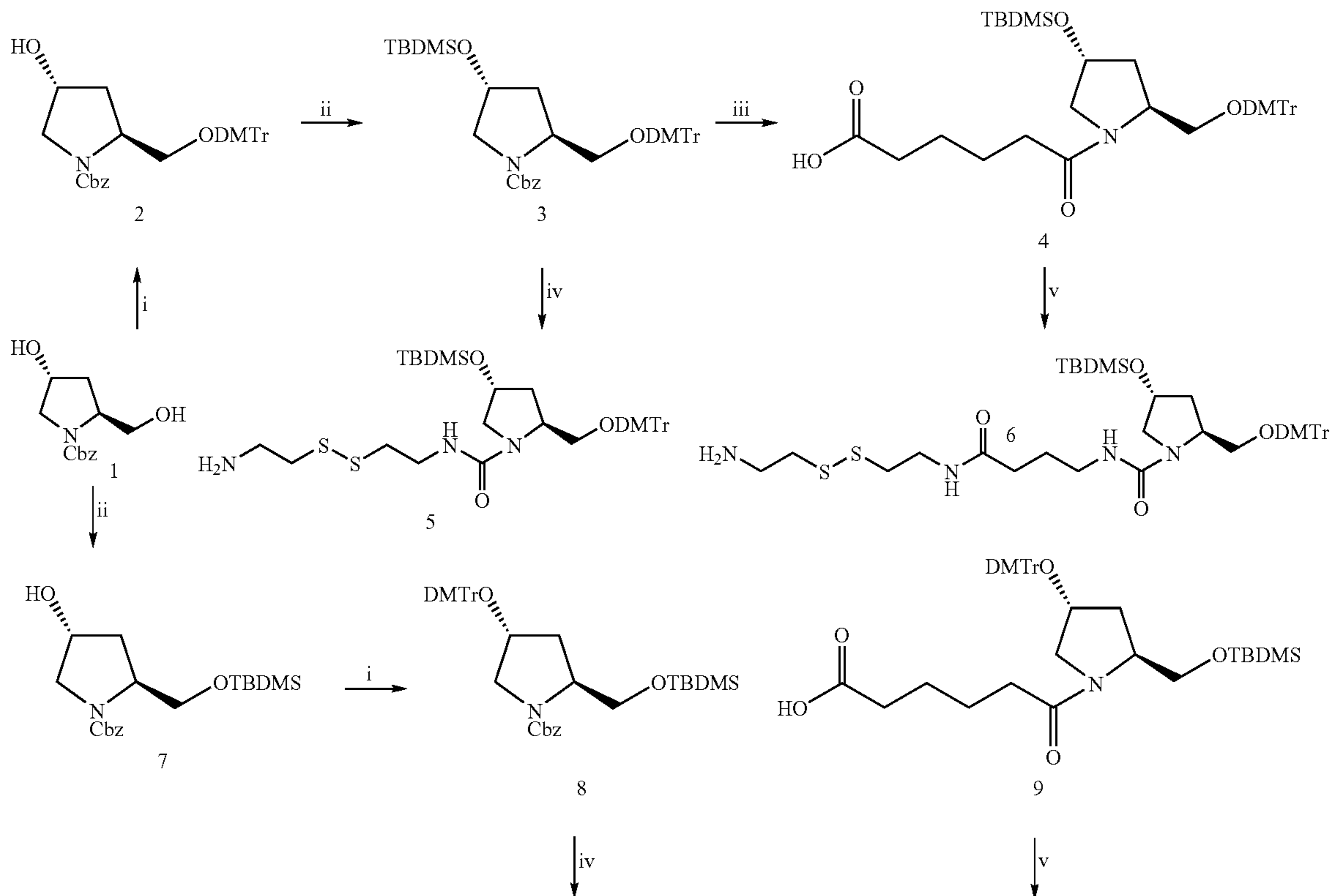
Scheme 1 a
