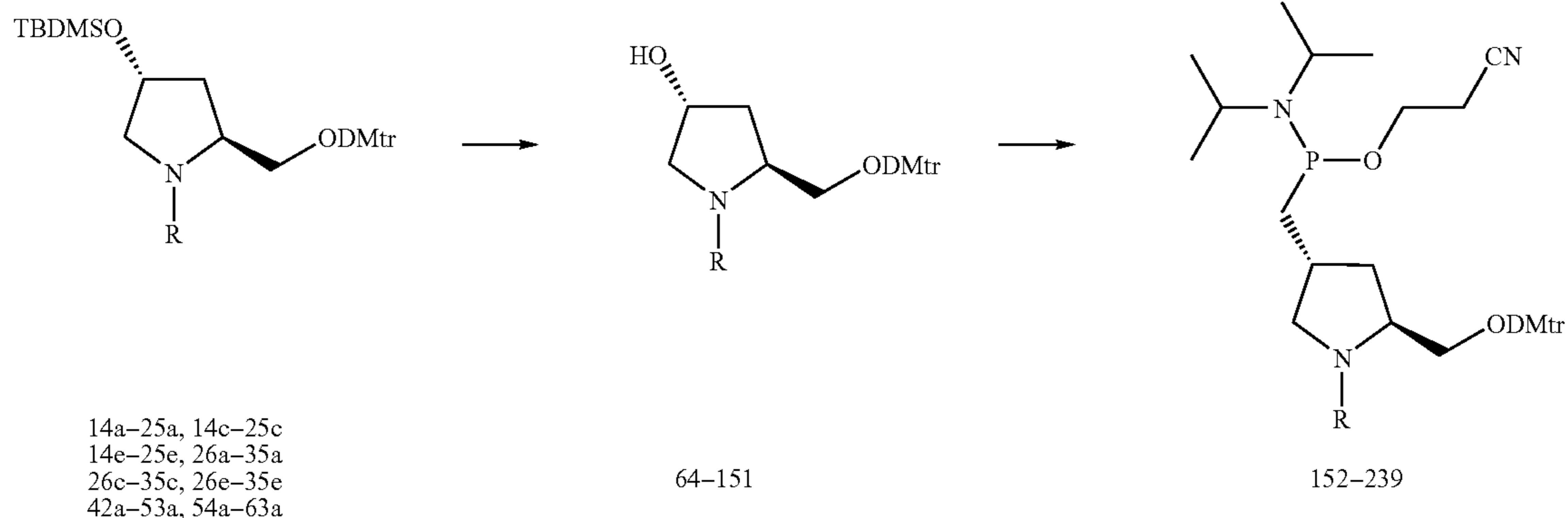
Scheme 8 a
