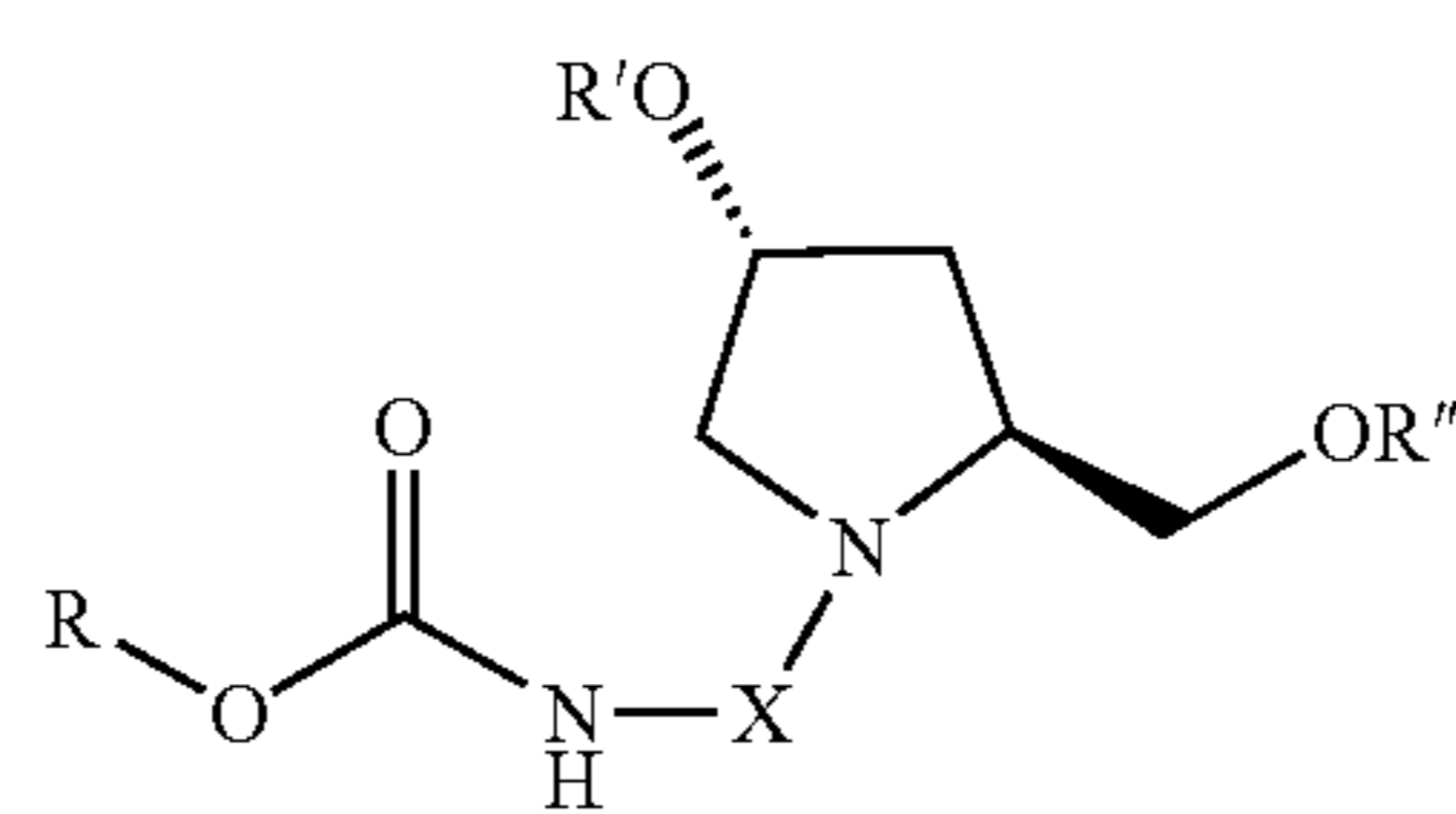
Scheme 4a
