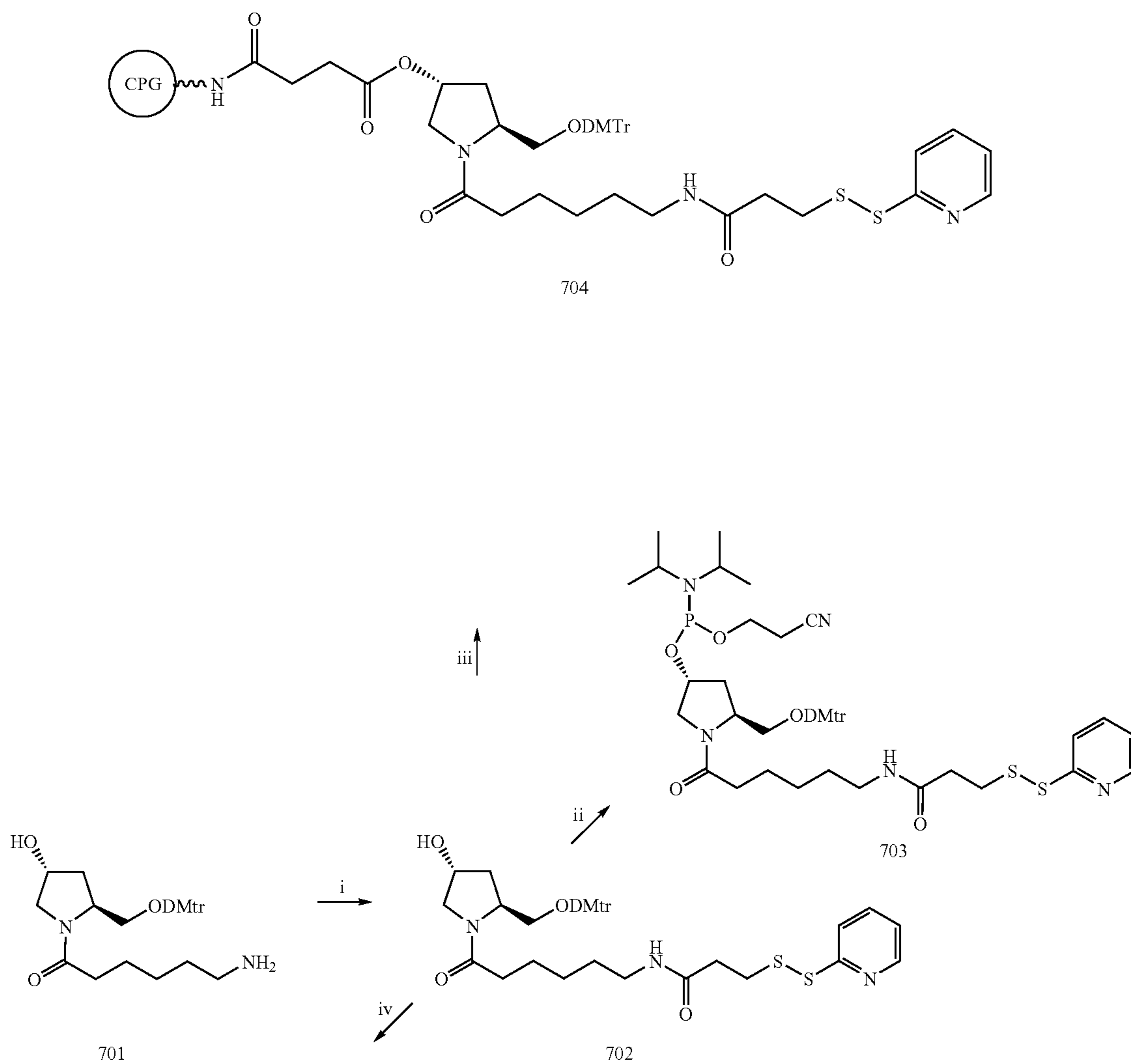
Scheme 10 a
