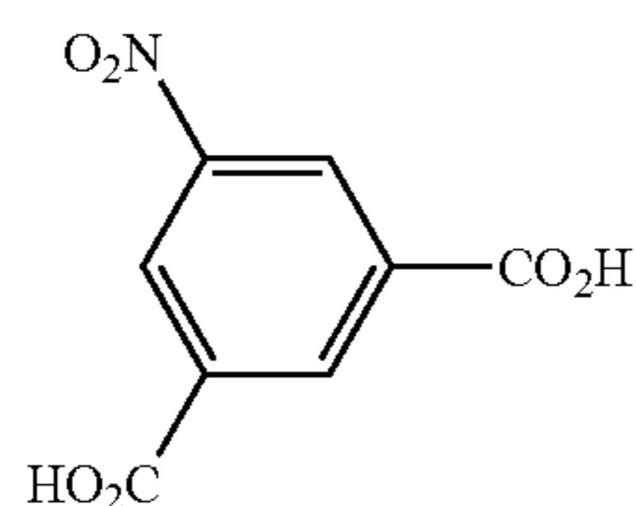
5-nitro-isophthalic acid
