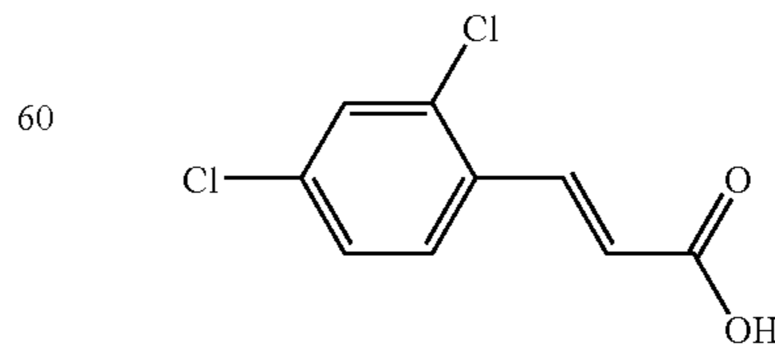
2,4-dichlorophenylacrylic acid
