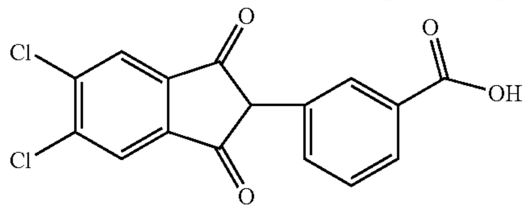
3-(4,5-dichlorophthaloylimido)benzoic acid
