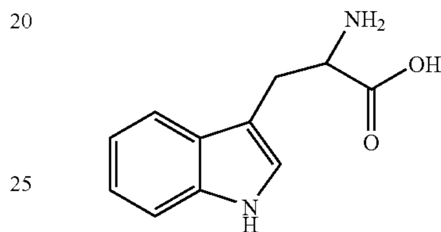
tryptophane
