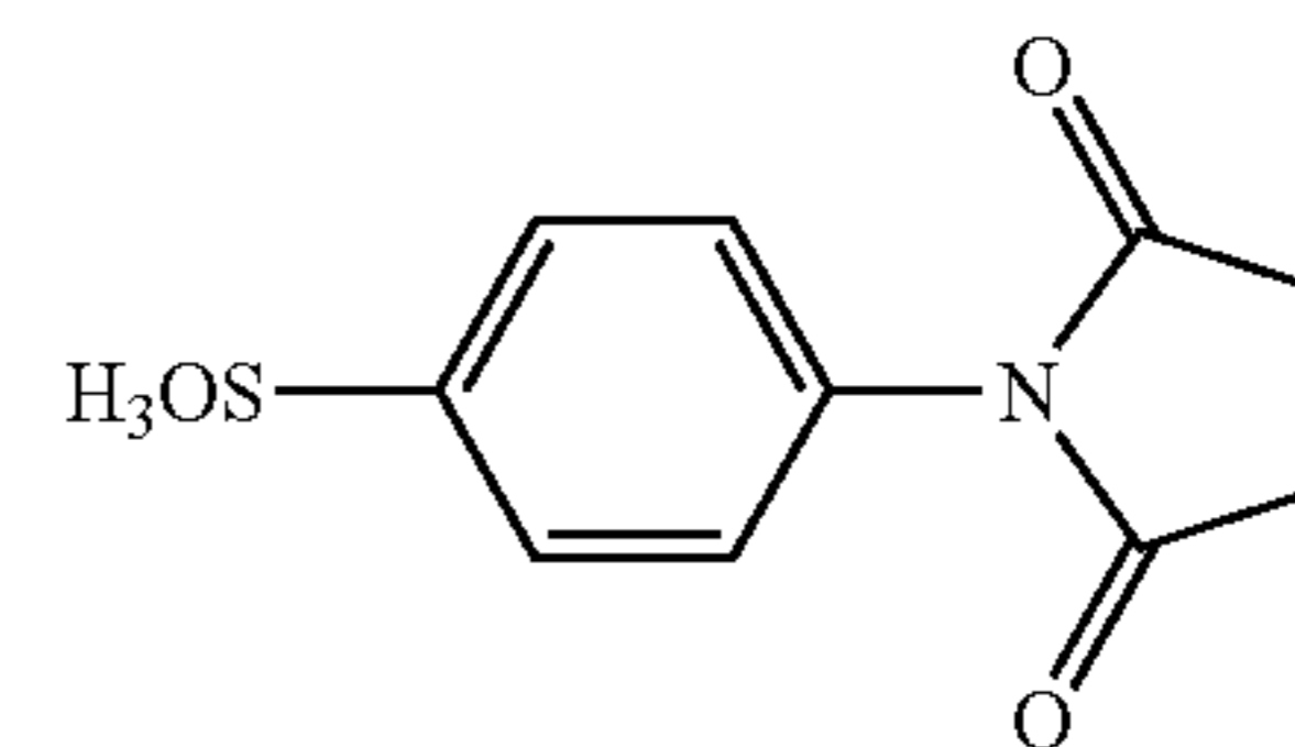
4-succinimidobenzenesulphonic acid
