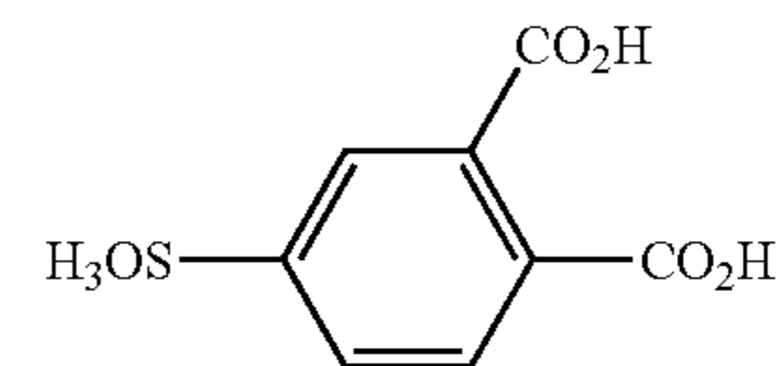
4-sulphoththalic acid
