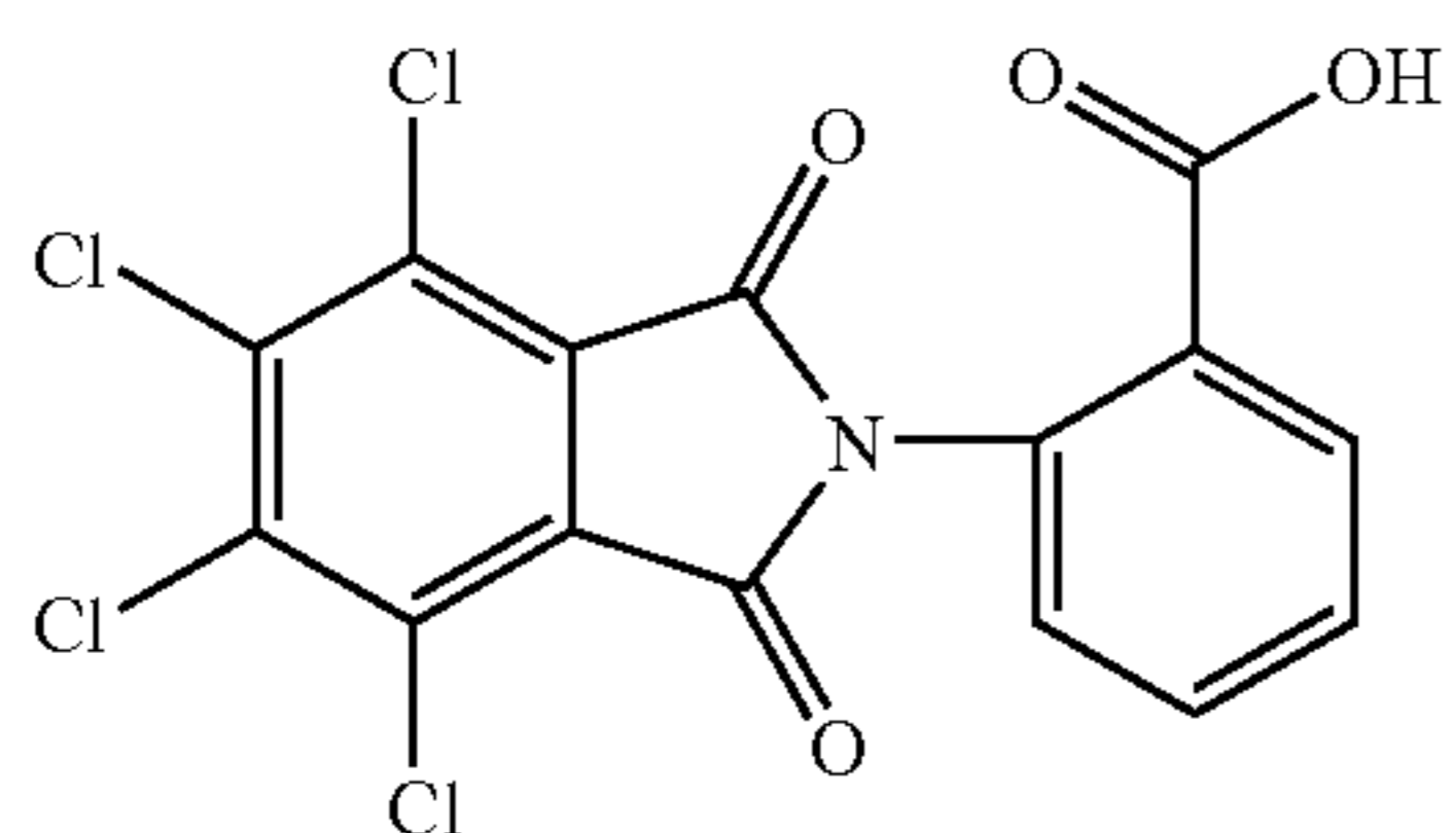
2-tetrachlorophthalimidobenzoic acid
