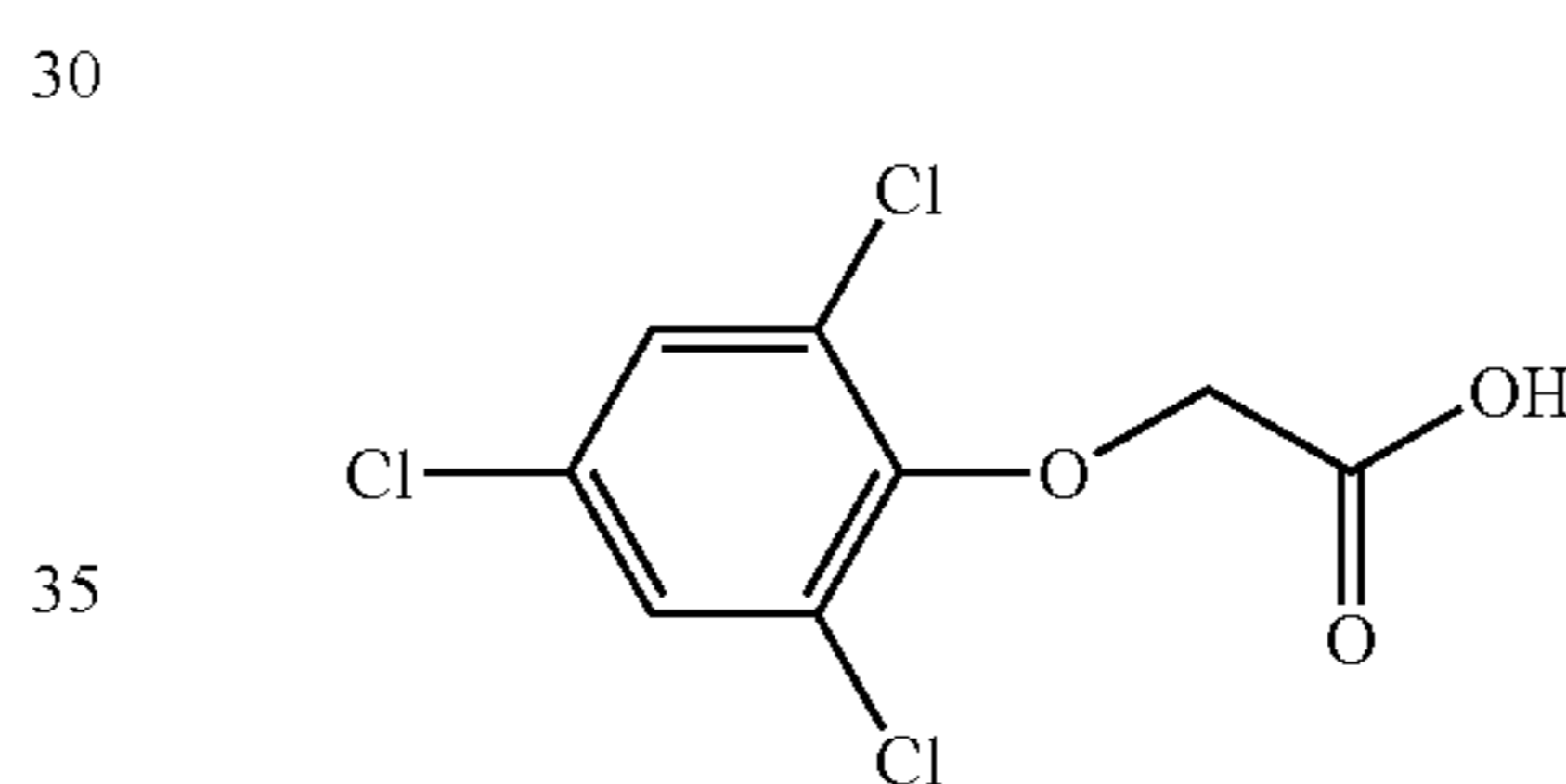
2,4,6-trichlorophenoxyacetic acid
