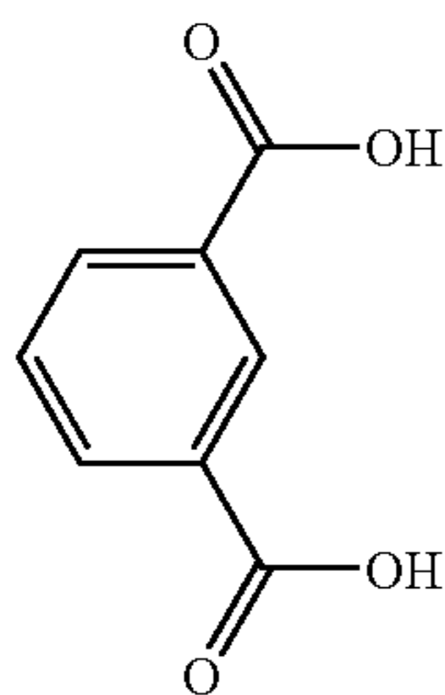
isophthalic acid
