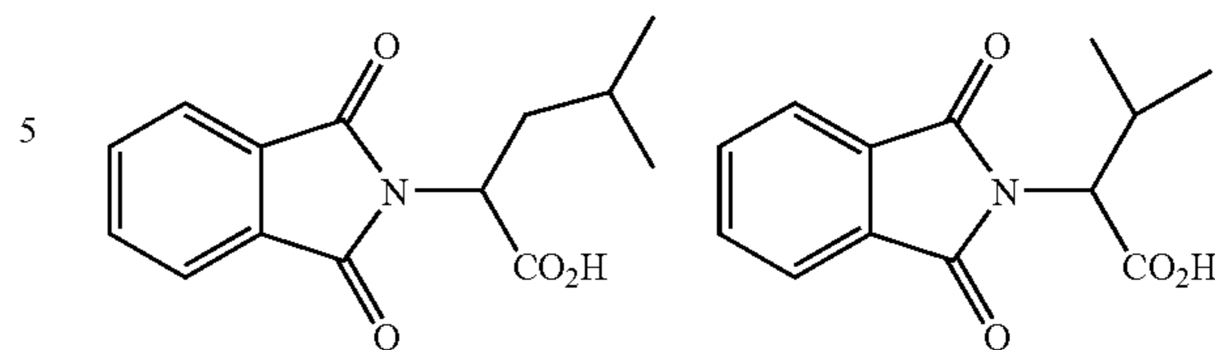
4-methyl-2-phthalimidovaleric acid
