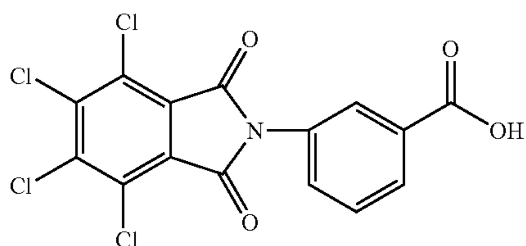
3-tetrachlorophthalimidobenzoic acid
