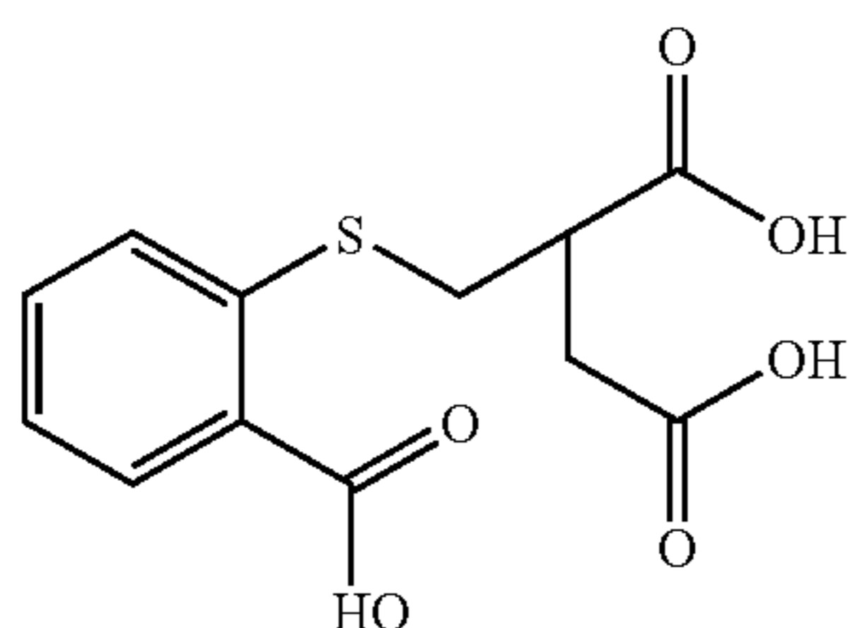
2-(2-carboxyphenylthiomethyl)succinic acid
