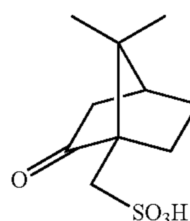
(+)-camphor-10-sulphonic acid
