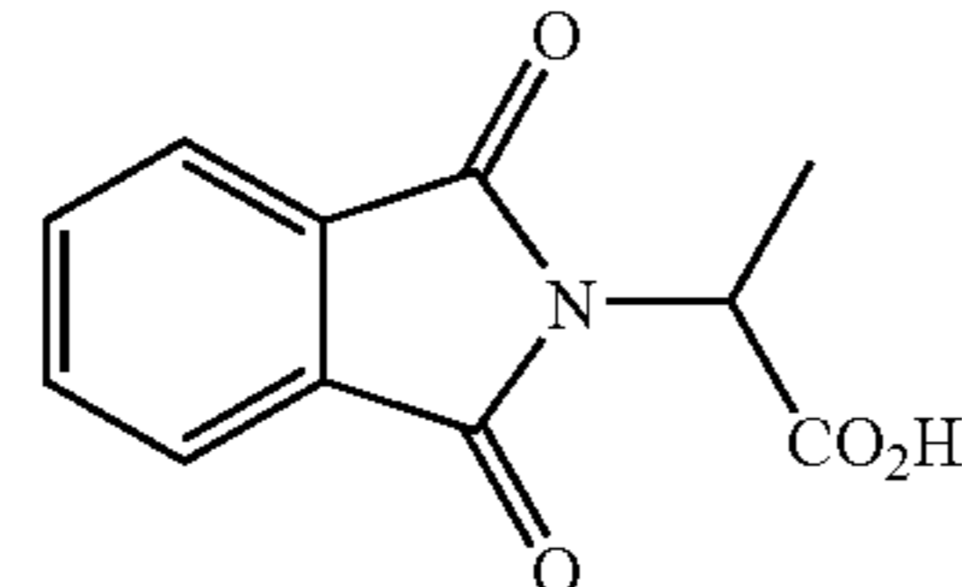
2-phthalimidopropionic acid
