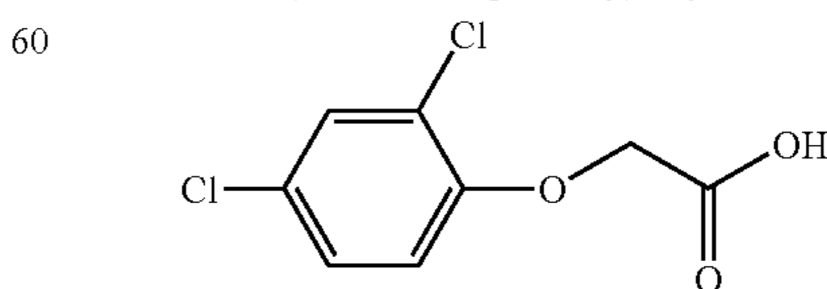
2,4-dichlorophenoxyacetic acid
