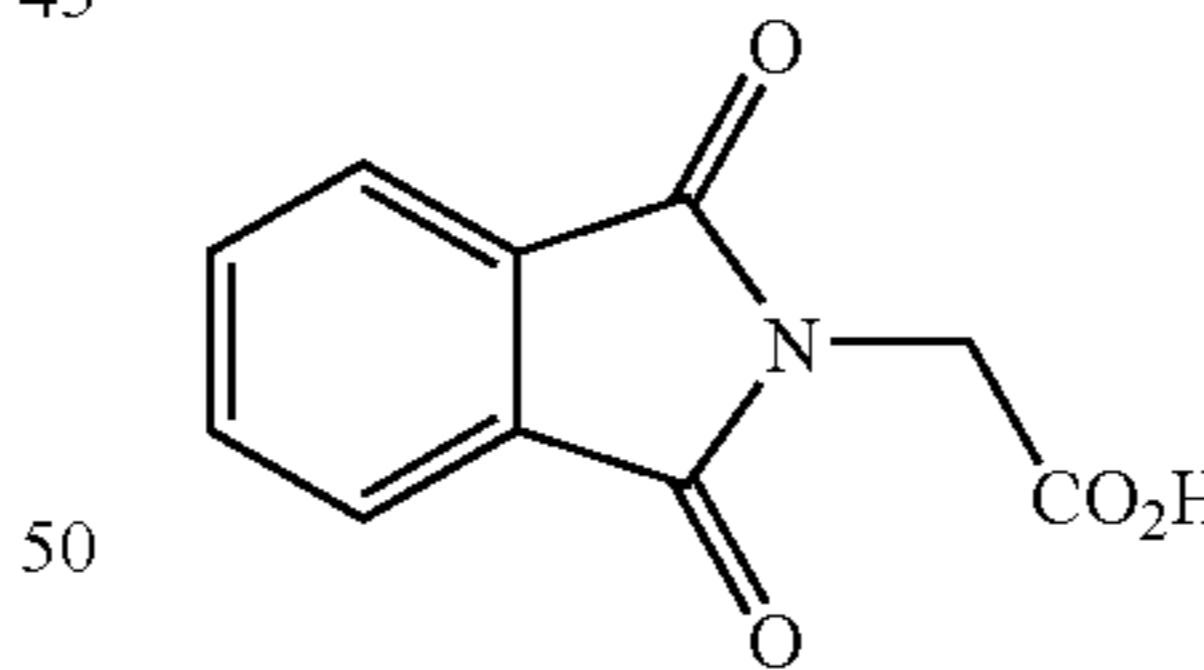
phthaloyl glycine
