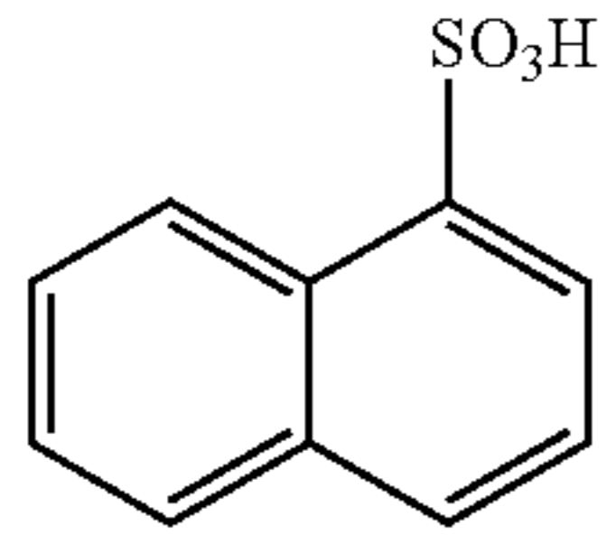
naphthalene-1-sulphonic acid
