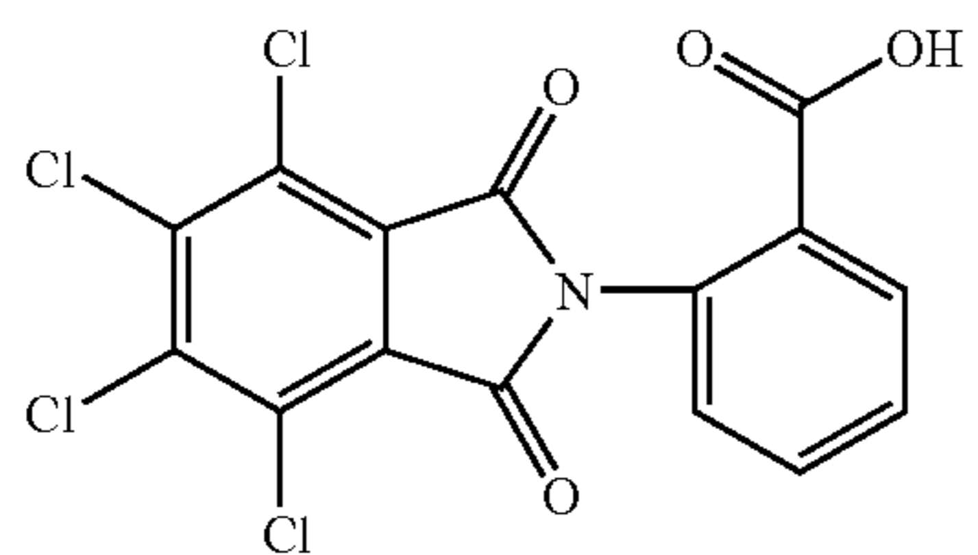
2-(3,4,5,6-tetrachlorophthaloylimido)benzoic acid
