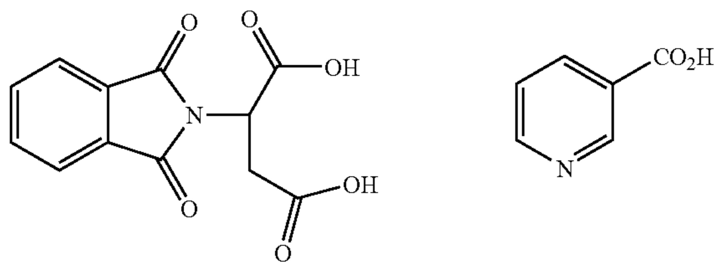
2-phthaloylimidosuccinic acid
