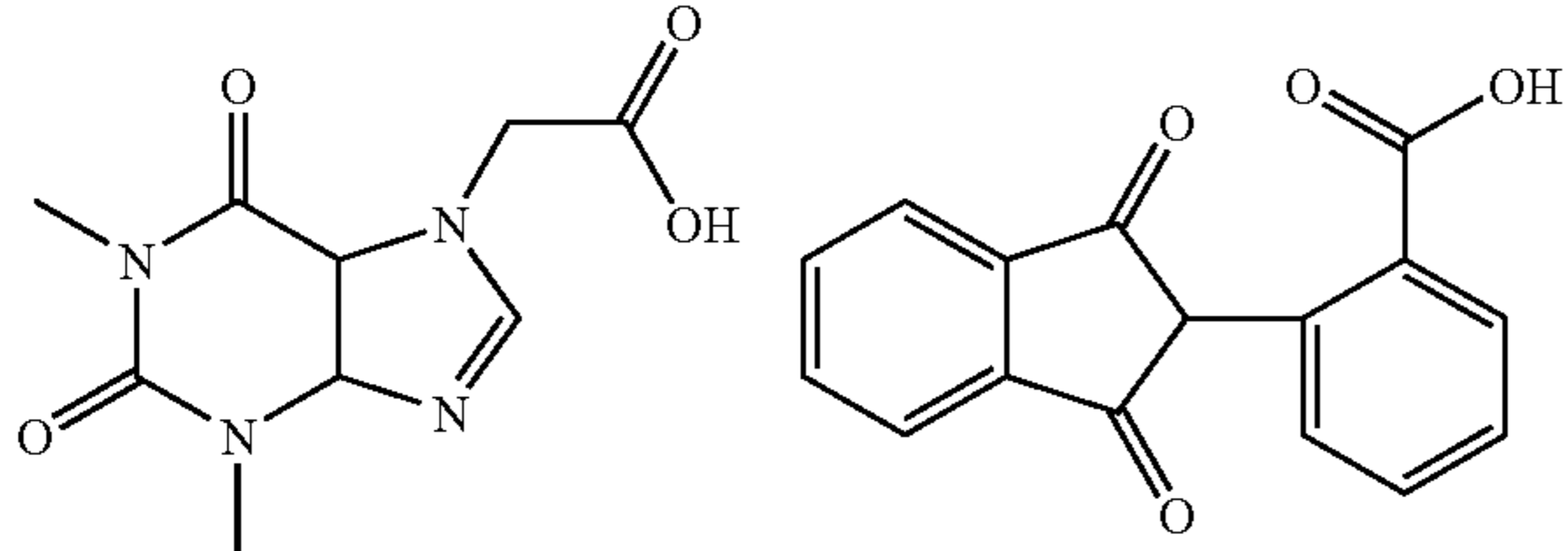
theophylline-7-acetic acid
