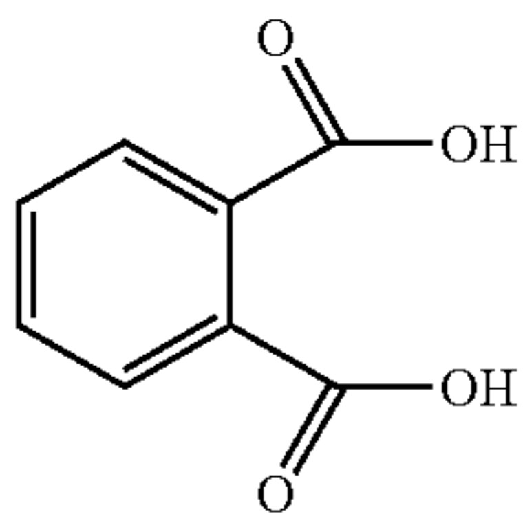
phthalic acid
