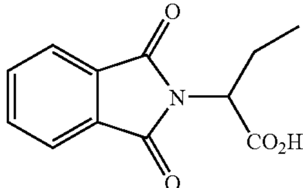
2-phthalimidobutyric acid
