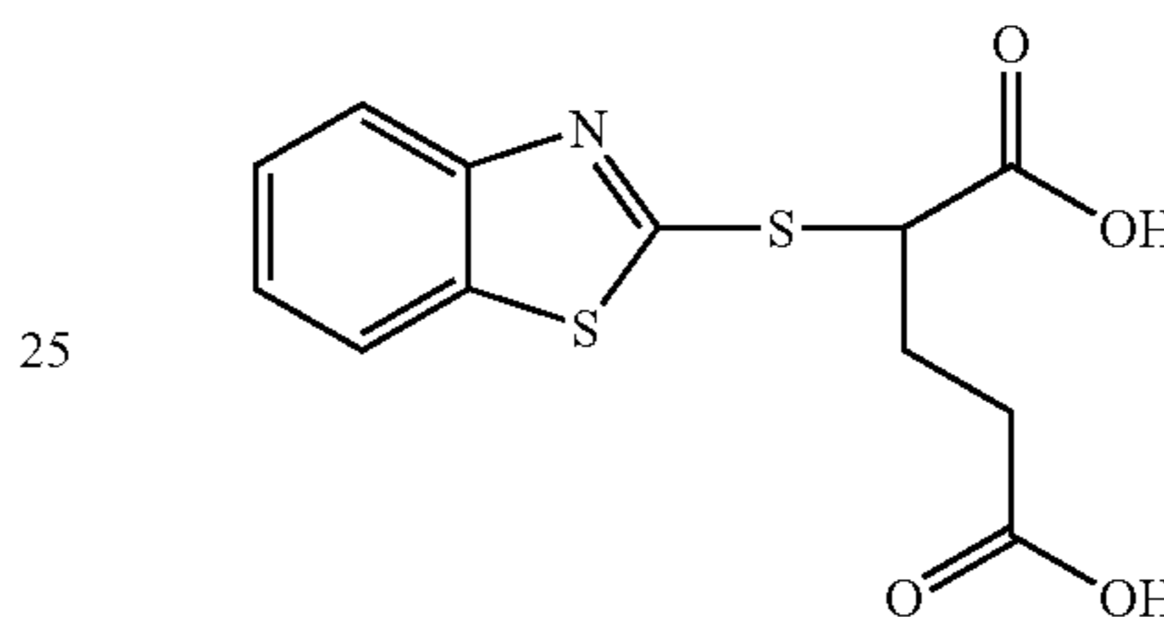
2-(2-benzothiazolylthio)succinic acid
