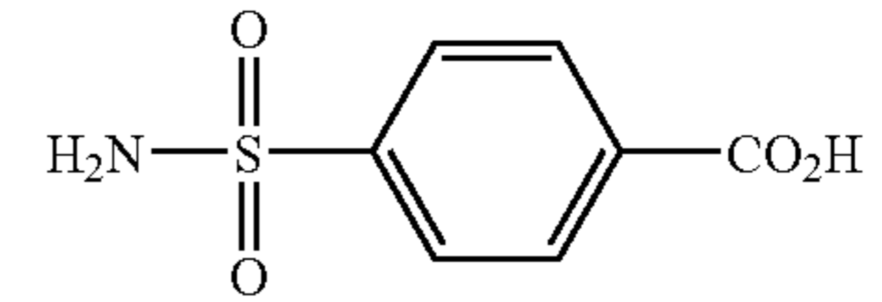
benzoic acid-4-sulphamide
