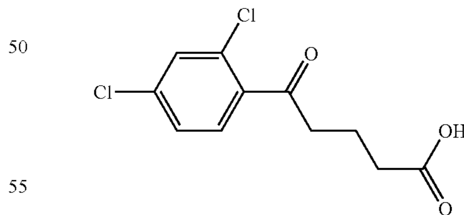
3-(2,4-dichlorobenzoyl)-butyric acid
