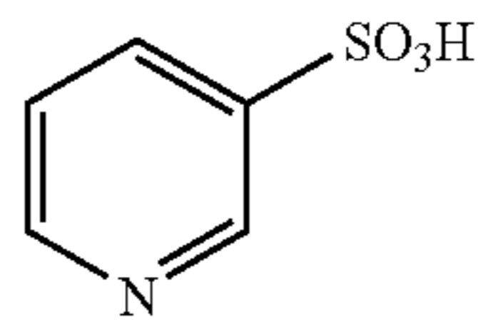
pyridine-3-sulphonic acid
