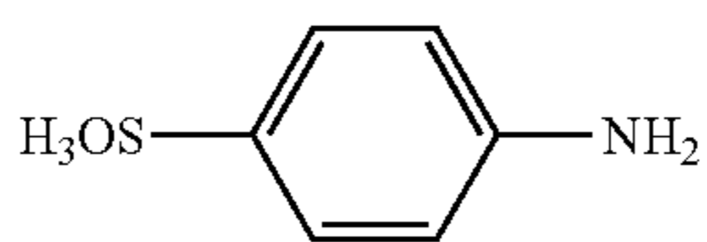
sulphanilic acid
