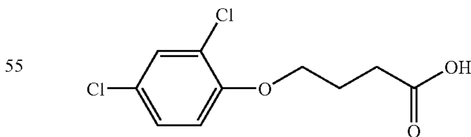
3-(2,4-dichlorophenoxy)butyric acid
