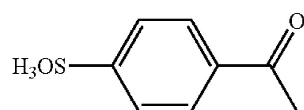
4-acetylsulphonic acid
