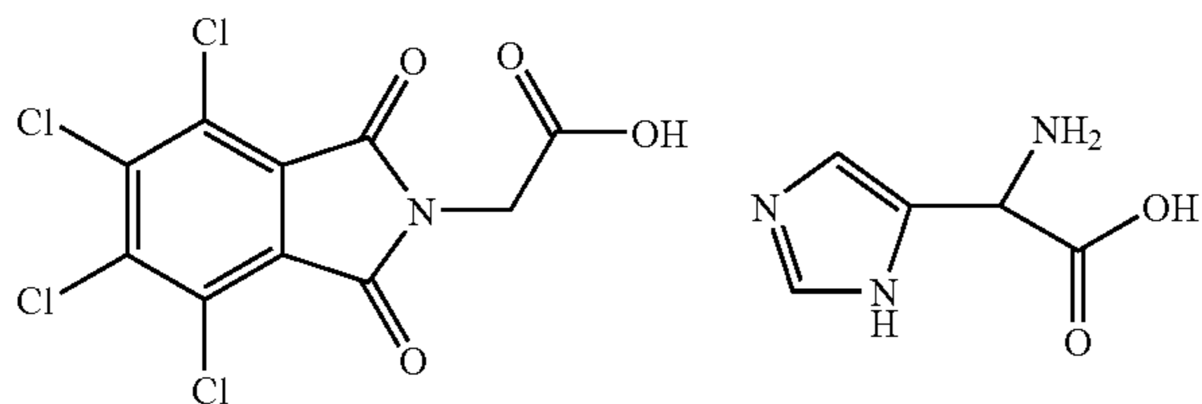
Histidine
