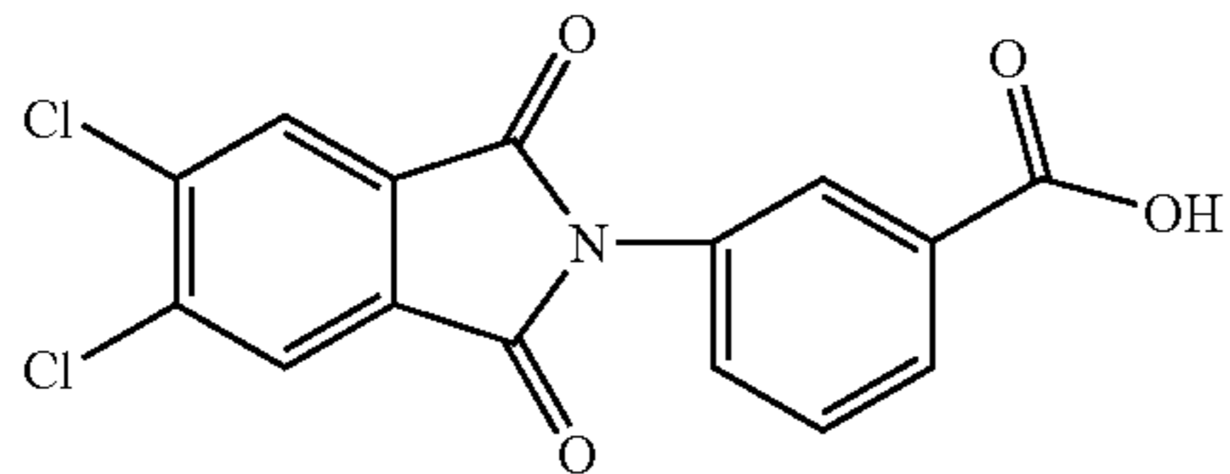
3(4,5-dichlorophthalimido)-benzoic acid
