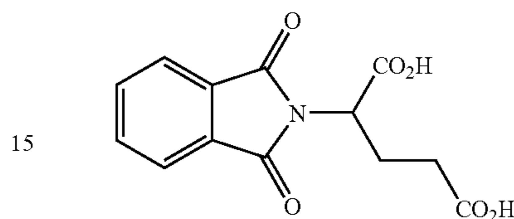
2-phthalimidoglutaric acid
