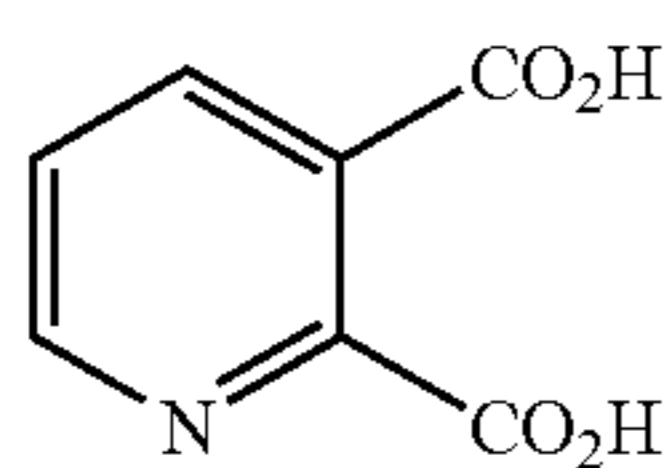
quinolinic acid
