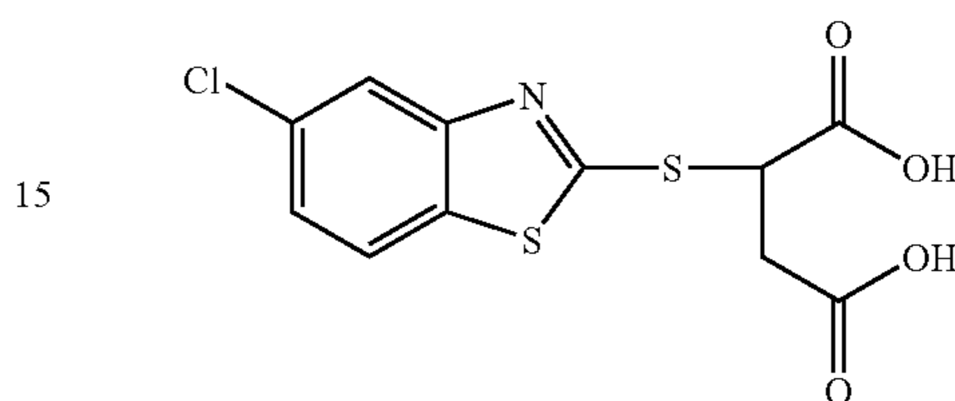
2-[2-(5-chlorobenzothiazolylthio)]succinic acid
