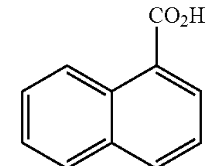
1-naphtholic acid
