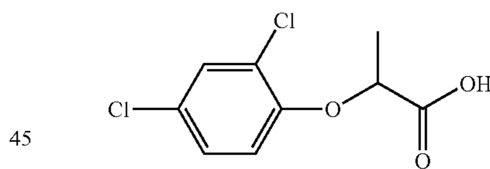
2-(2,4-dichlorophenoxy)-propionic acid
