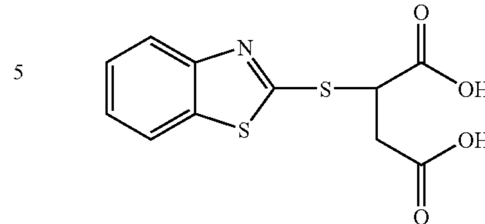
2-(2-benzothiazolylthio)succinic acid
