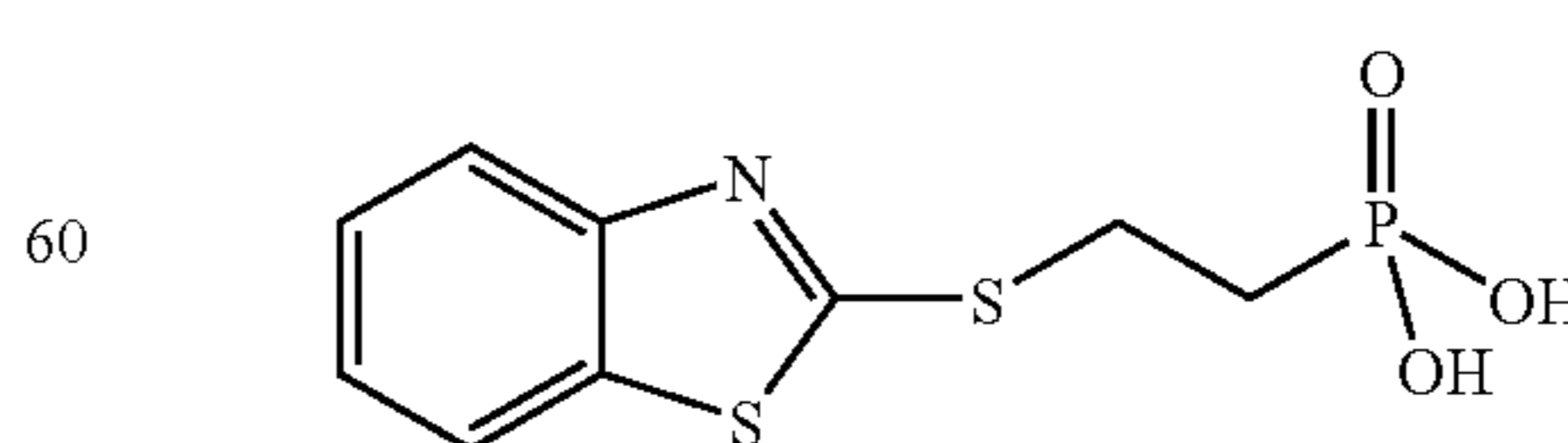
3-(2-benzothiazolylthio)propanephosphonic acid
