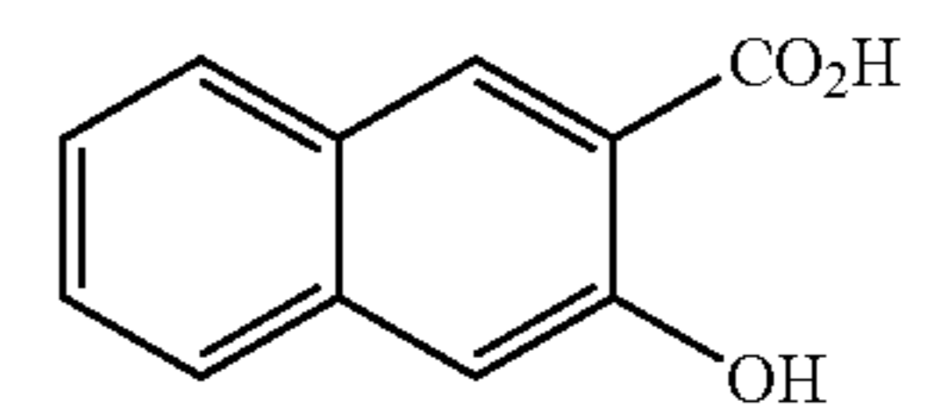
3-hydroxynaphtholic acid
