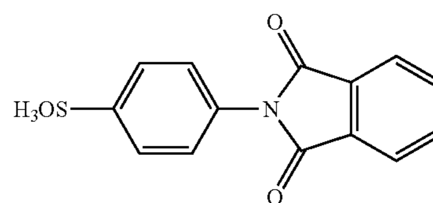
4-phthalimidobenzenesulphonic acid
