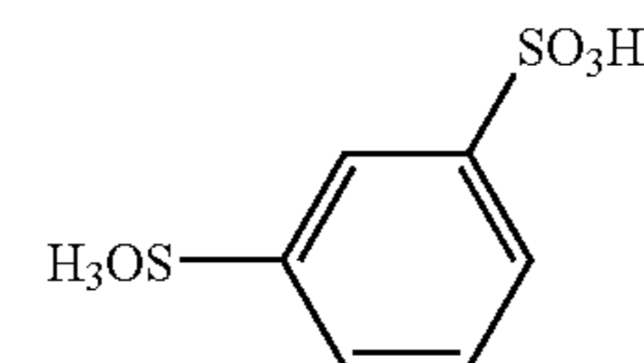
benzene-1,3-disulphonic acid
