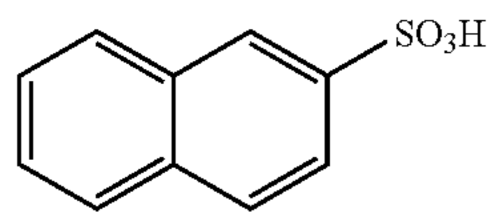
naphthalene-2-sulphonic acid
