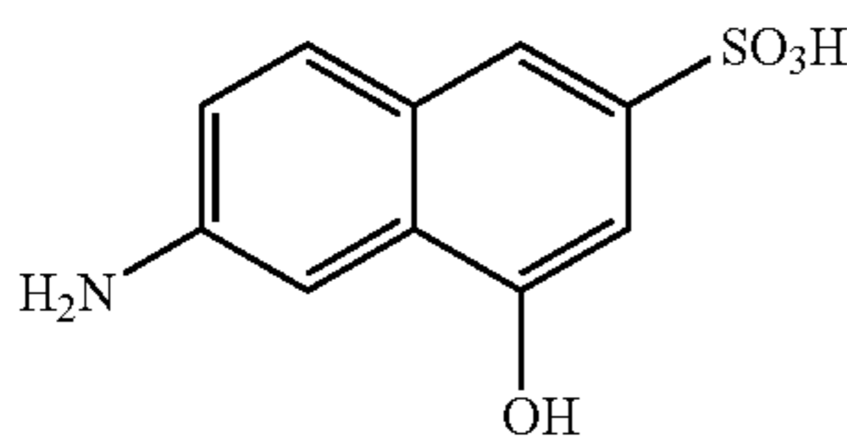
7-amino-1-naphthol-3-sulphonic acid
