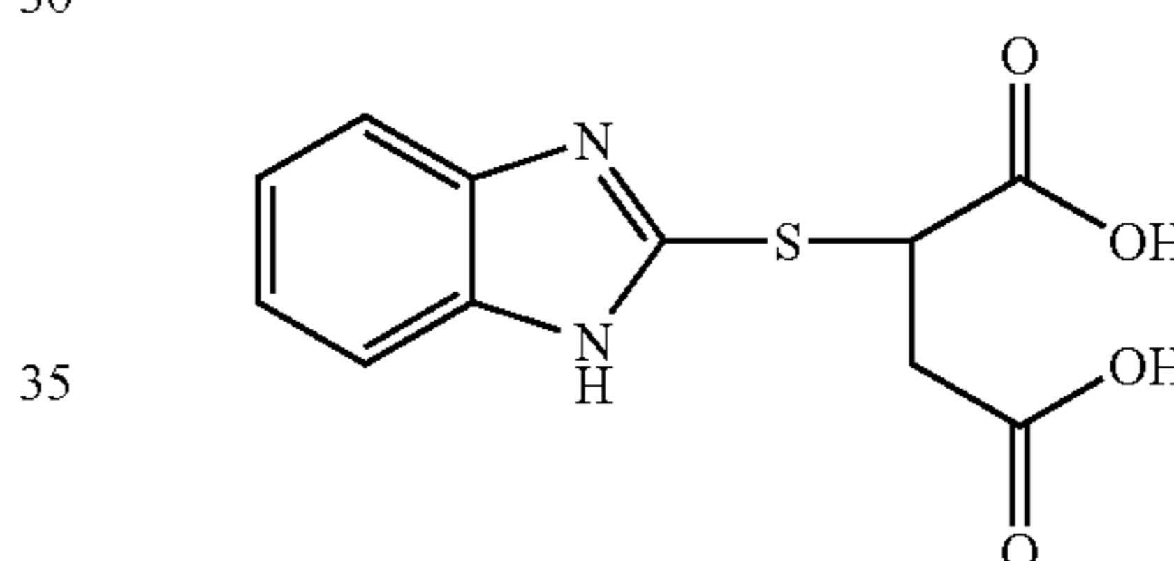
2-(2-benzimidazolylthio)succinic acid
