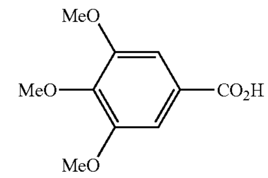
3,4,5-trimethoxybenzoic acid
