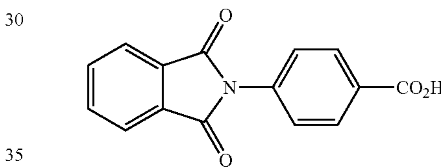
N-(4-carboxylphenyl)phthalimide
