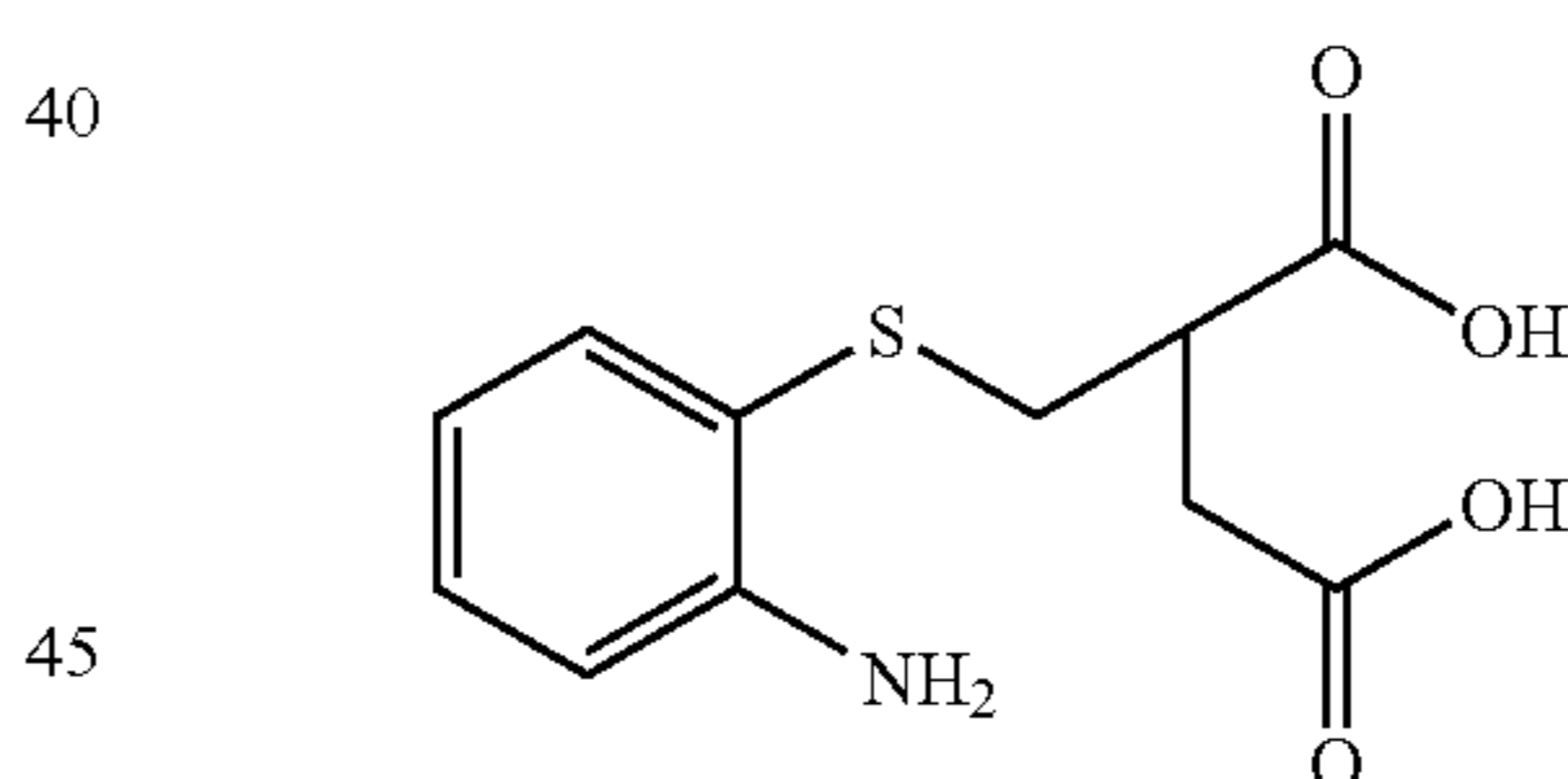
2-(2-aminophenylthiomethyl)succinic acid
