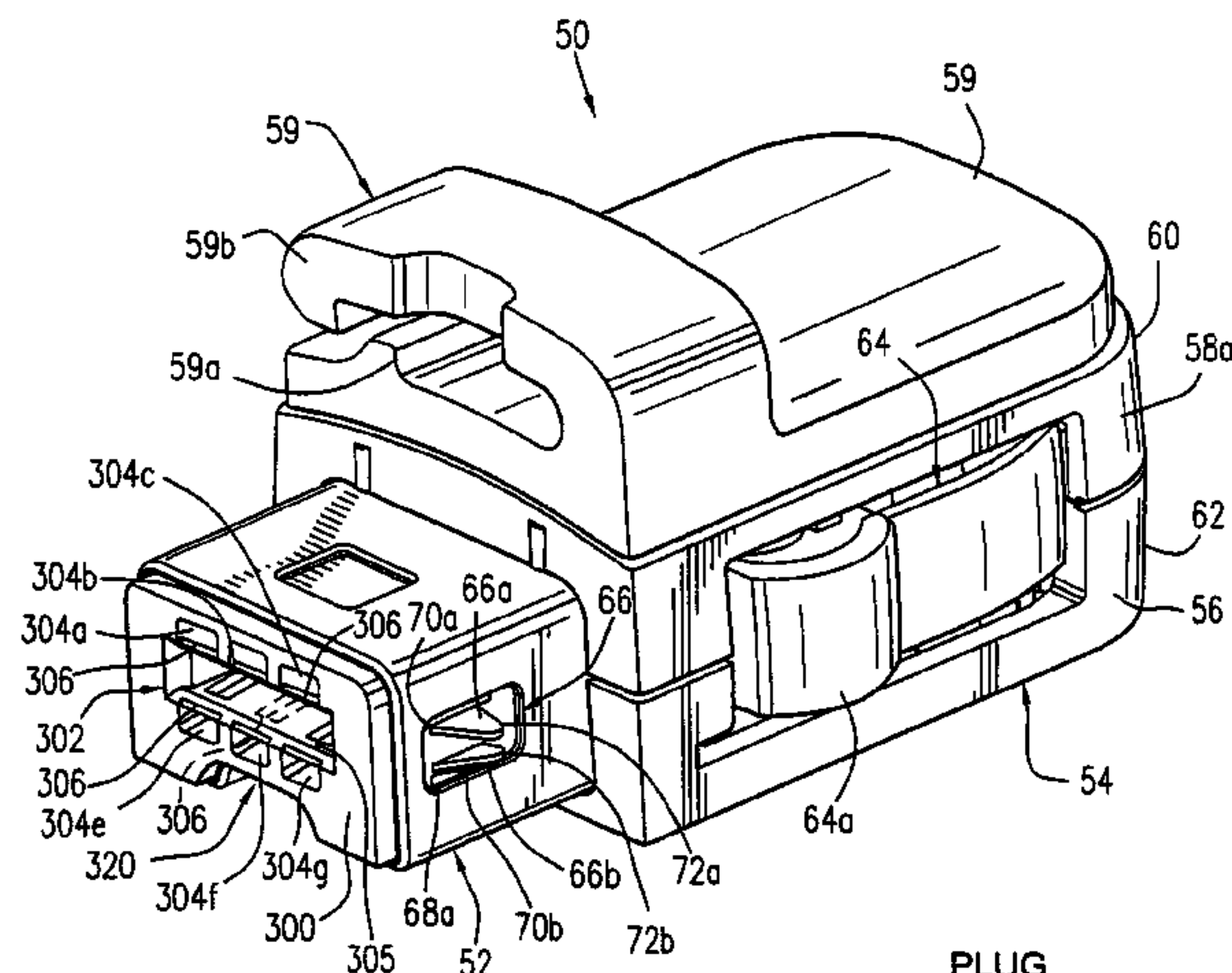
PLUG
