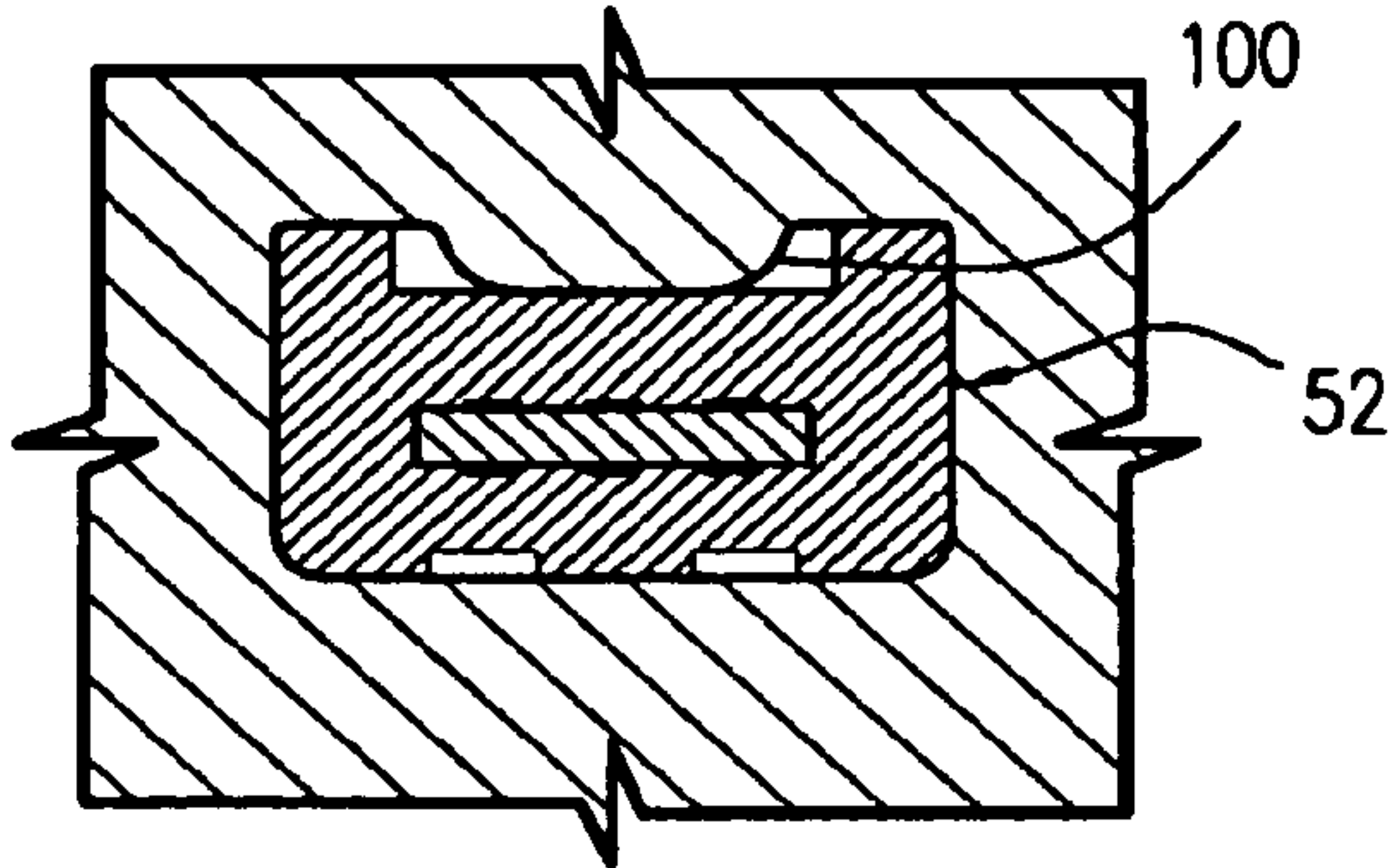
FIG. 18I PLUG
