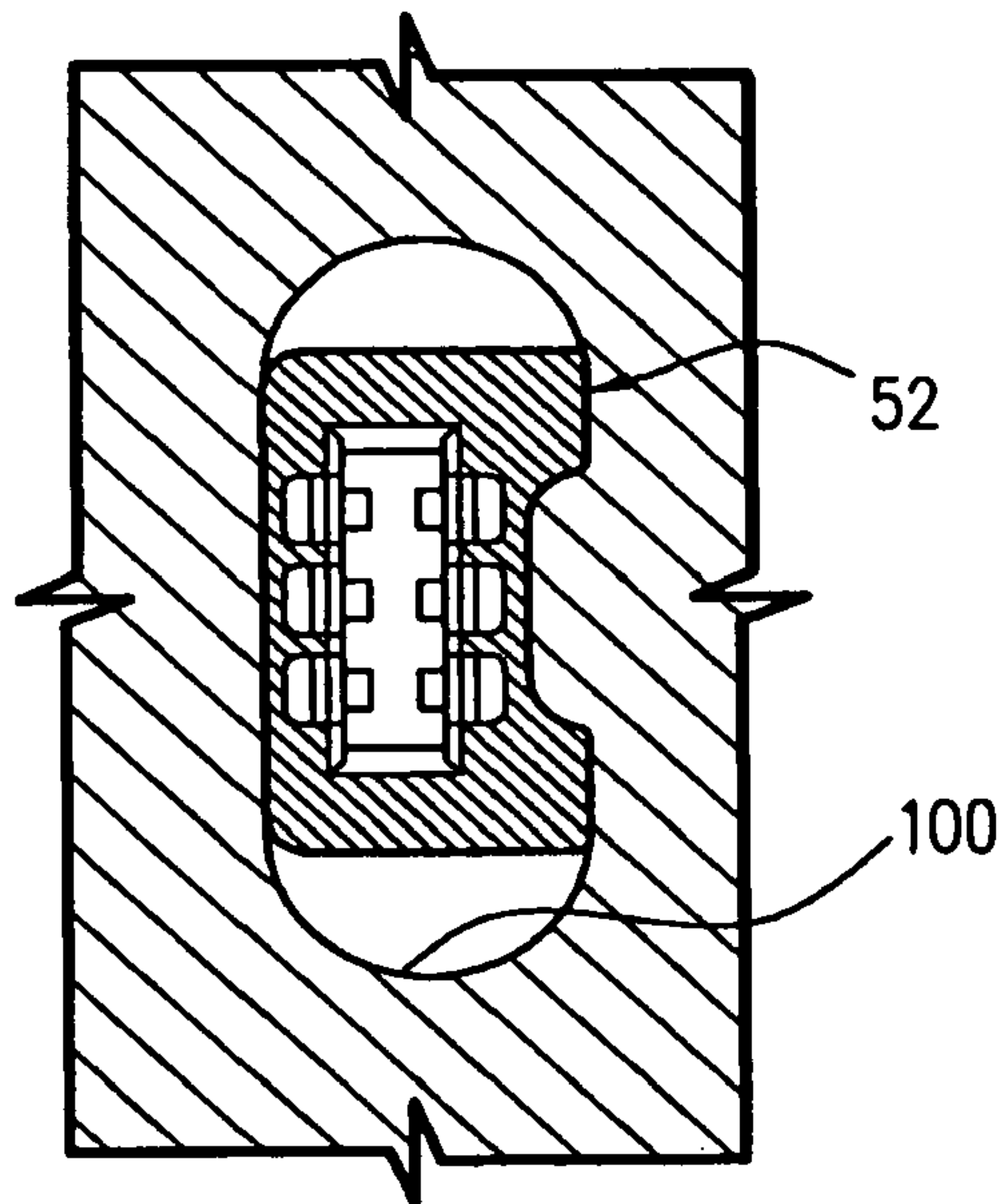
FIG. 17I SOCKET
