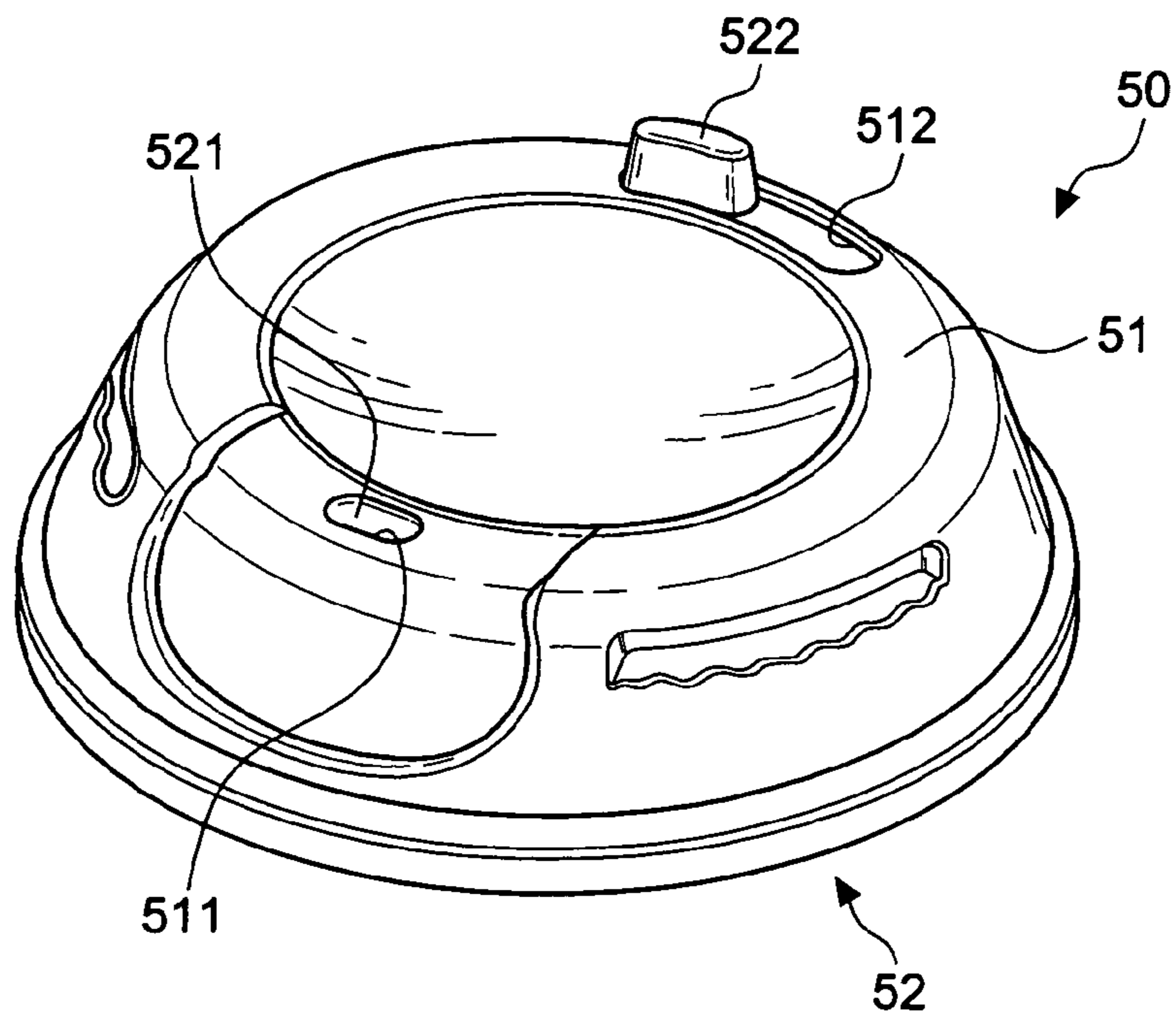
FIG. 2 PRIOR ART
