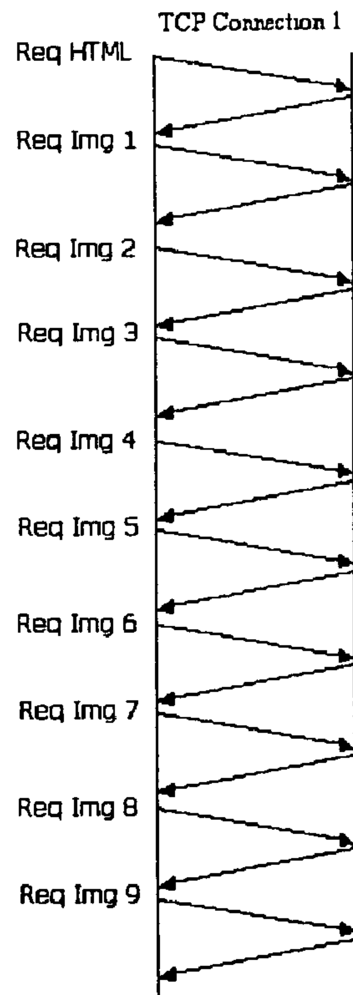
HTTP/1.1 persistent connection
