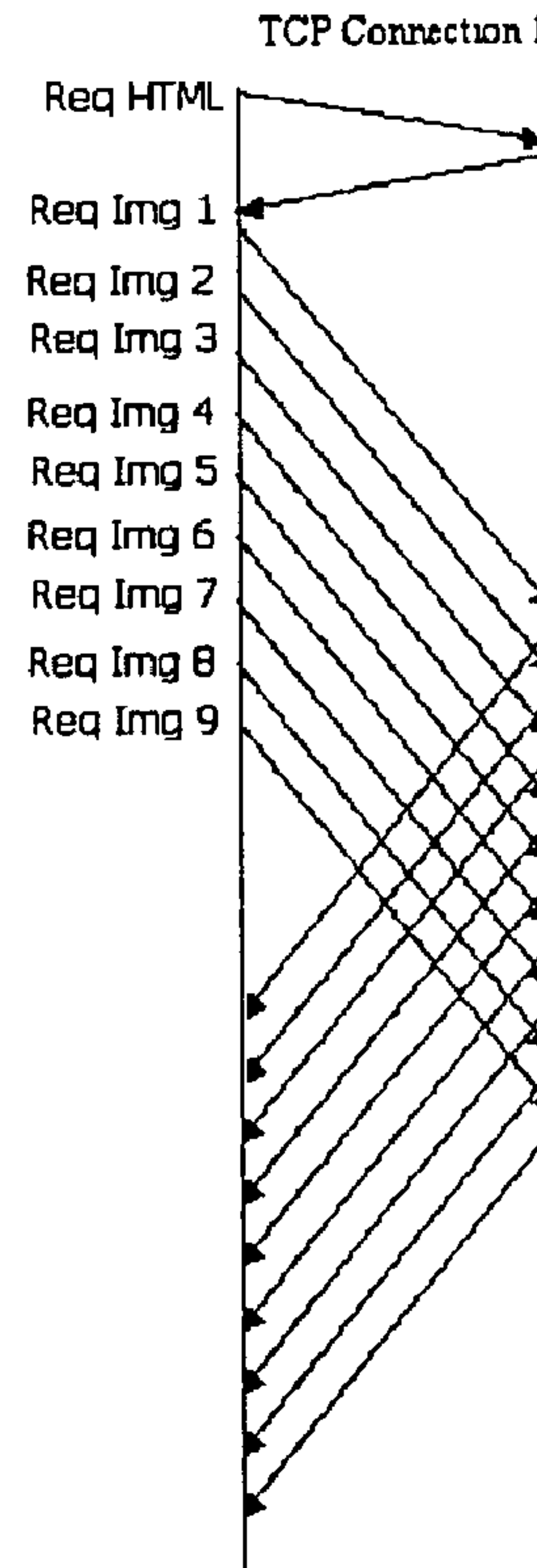
HTTP/1.1 persistent, pipelined connection
