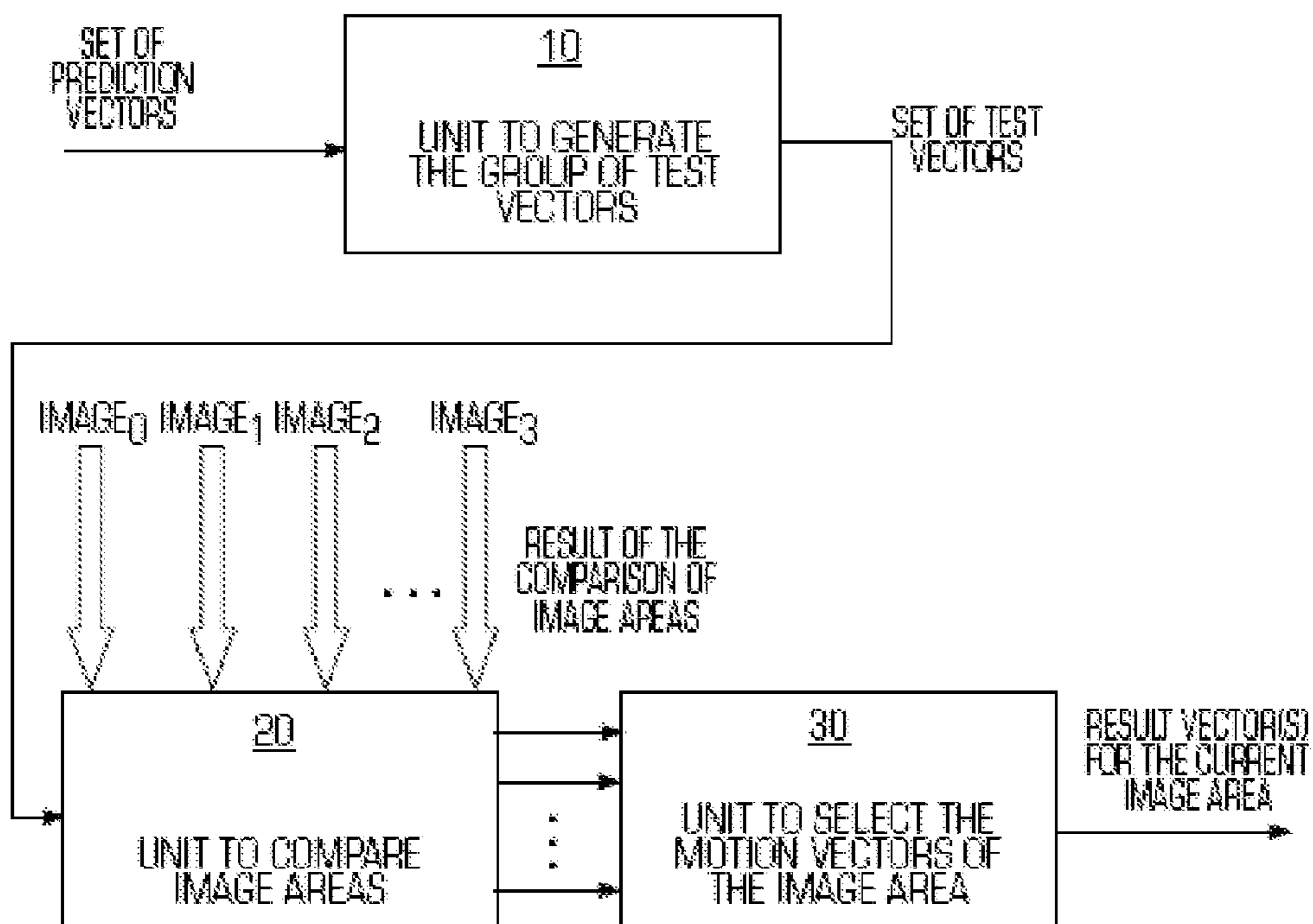
FIG. 2 (PRIOR ART)
