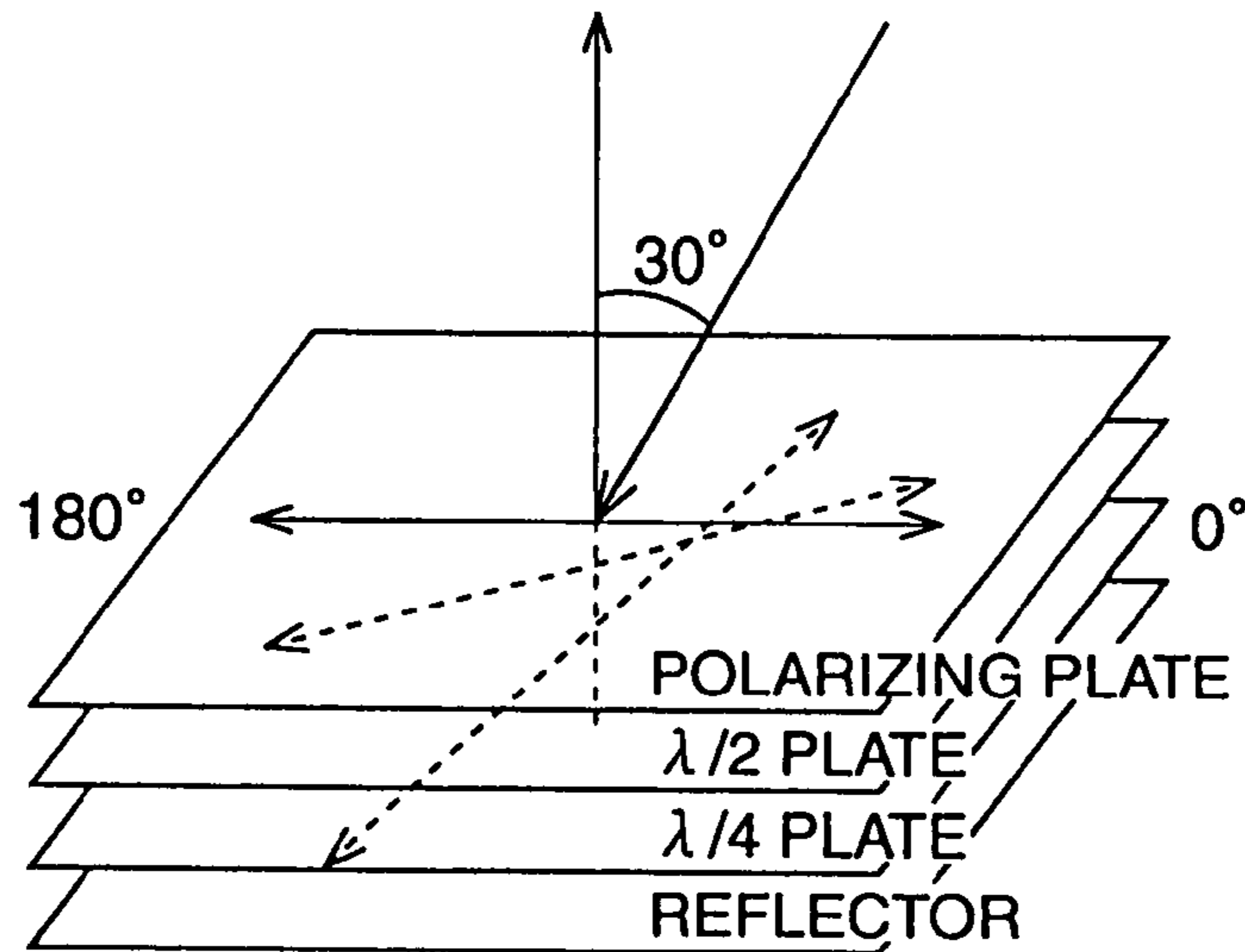
CONFIGURATION OF POLARIZING PLATE + BROADBAND \lambda/4 AND MEASUREMENT METHOD
