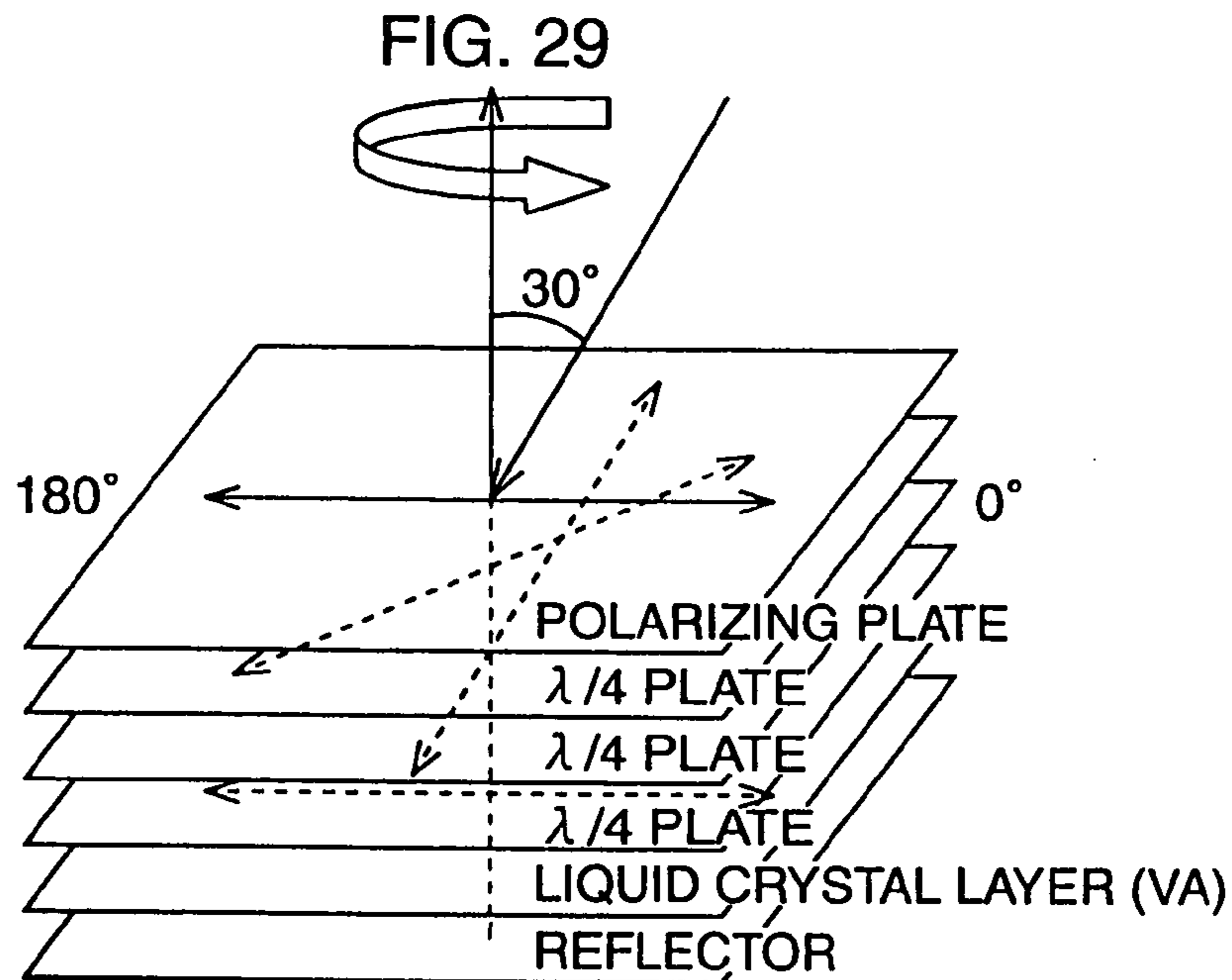
CONFIGURATION OF POLARIZING PLATE+ λ/4+COMPENSATION PLATE AND MEASUREMENT METHOD
