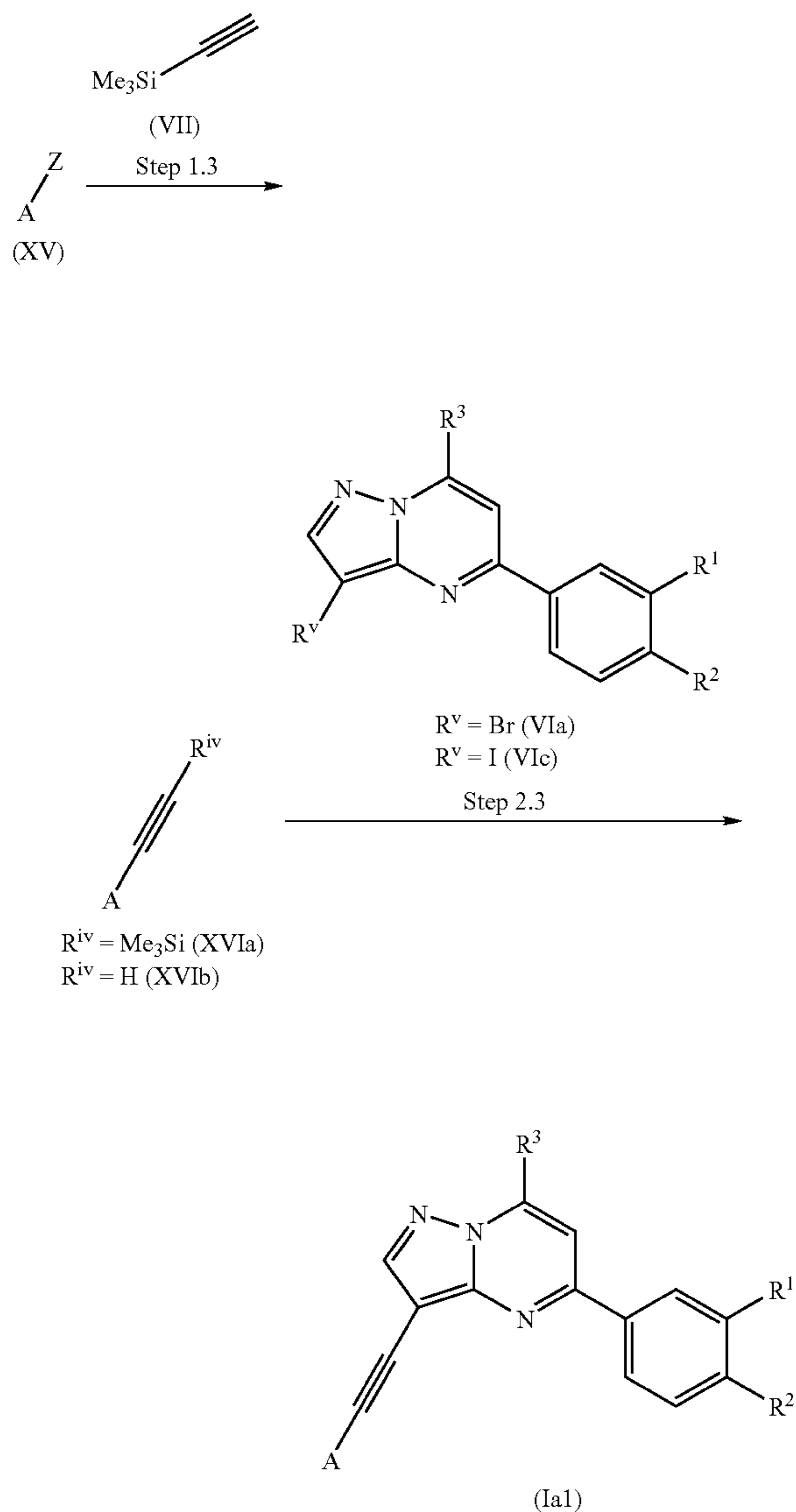
Scheme 3
