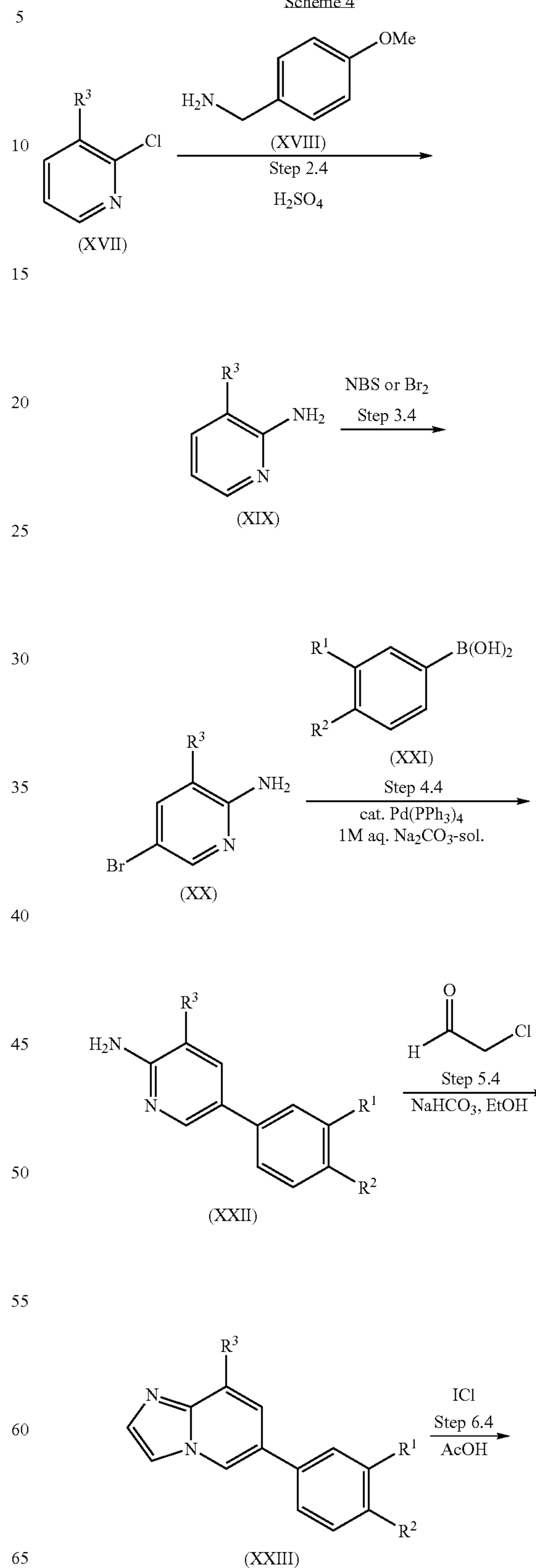
Scheme 4
