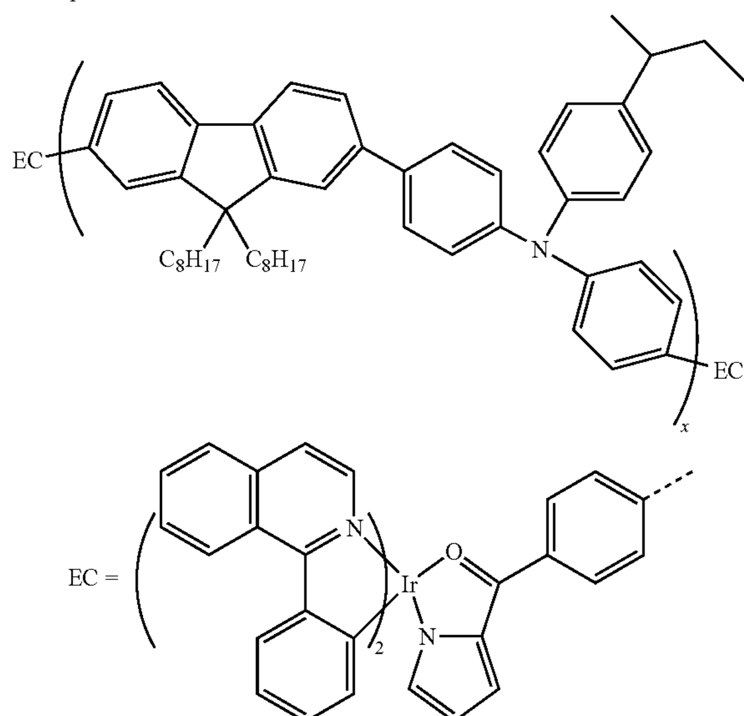
Poly(9,9-dioctylfluorene-triarylamine) End-capped Organic Iridium Complex XLVII: A solution of N,N-4,4'-
