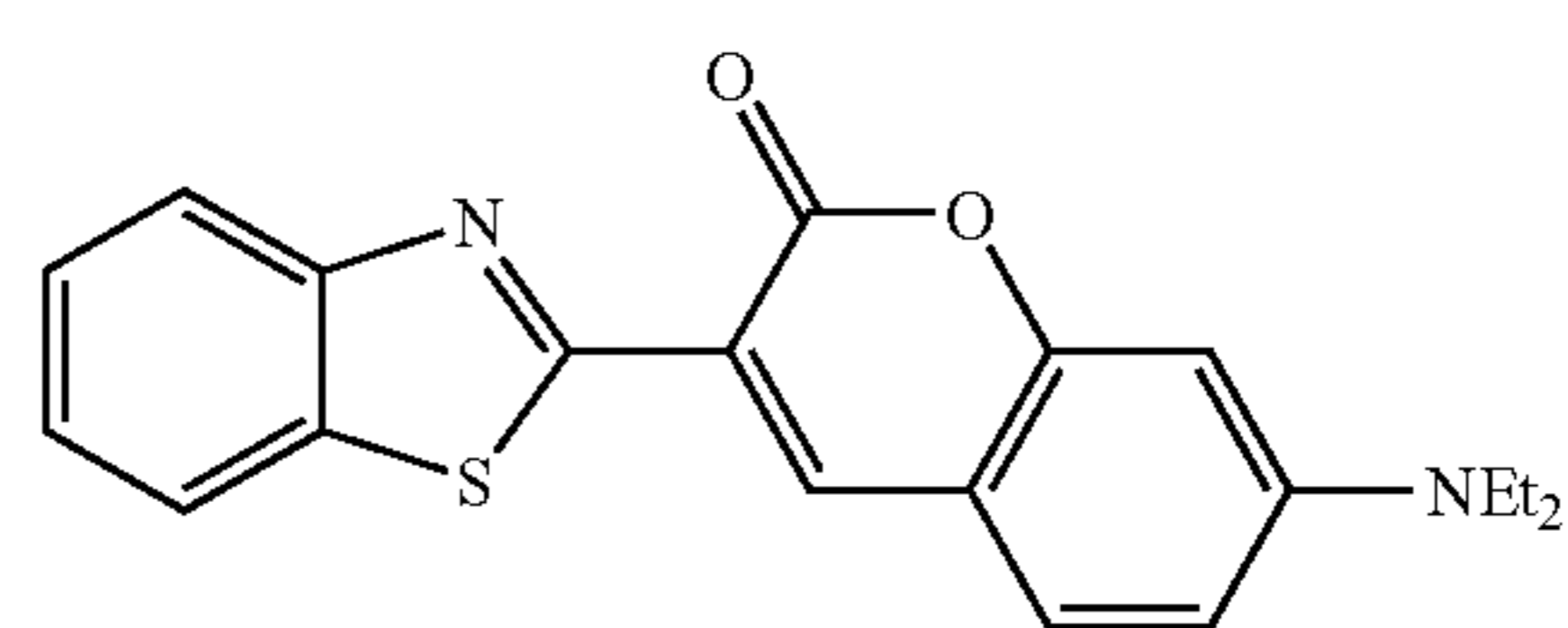
"coumarin 6"
